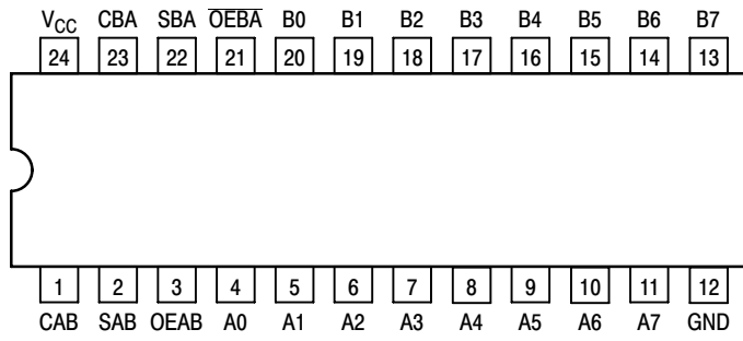
Figure 2. 24-Lead Pinout (Top View)
