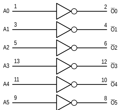
LOGIC DIAGRAM
