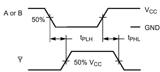
Figure 4. Switching Waveforms
