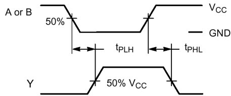
Figure 4. Switching Waveforms
