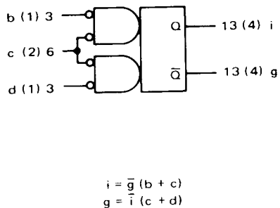
MC906 Half-Shift Register (without inverter)
