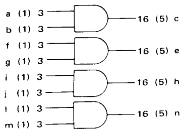
MC9813 Quad 2-Input AND Gate
