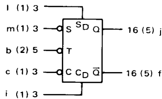
MC826, MC926 J-K Flip-Flop
