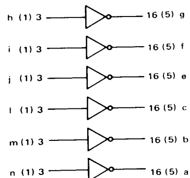
MC889, MC989 Hex Inverter
