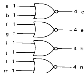
MC817, MC917 Quad 2-Input NOR Gate
