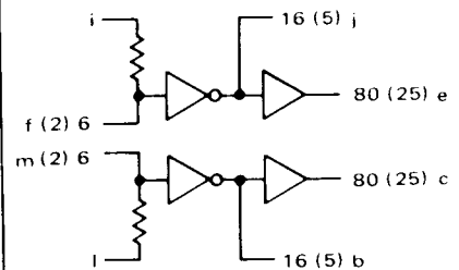
MC899/MC999 Dual Buffer
