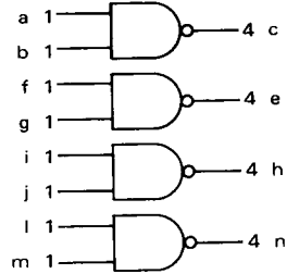
MC9824 Quad 2-Input NAND Gate
