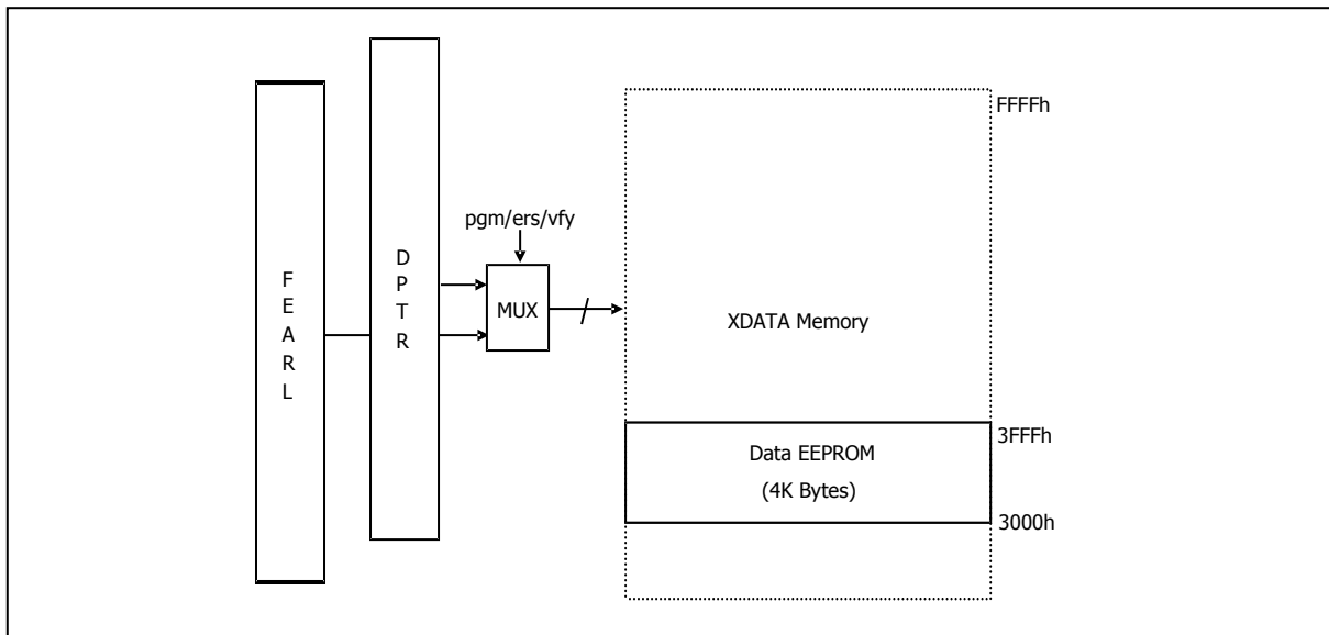
Figure 15-3 Data EEPROM memory map
