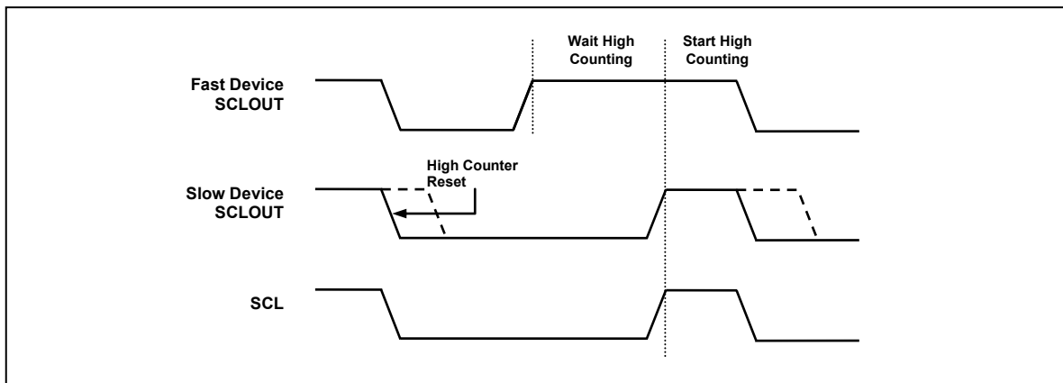
Figure 11-40 Clock Synchronization during Arbitration Procedure
