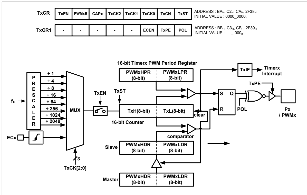
Figure 11-20 PWM Mode
