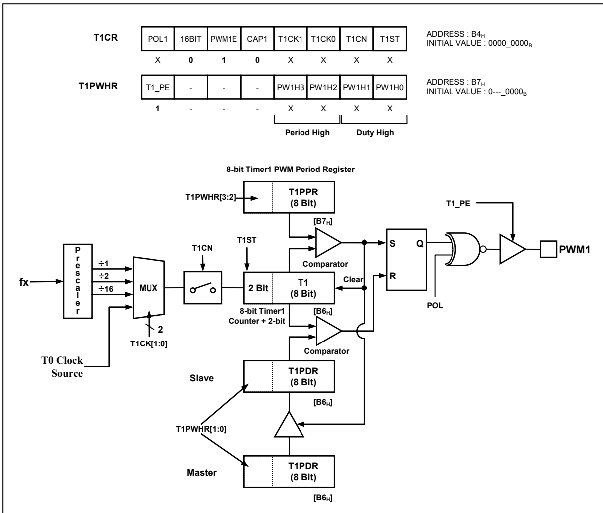
Figure 11-15 PWM Mode
