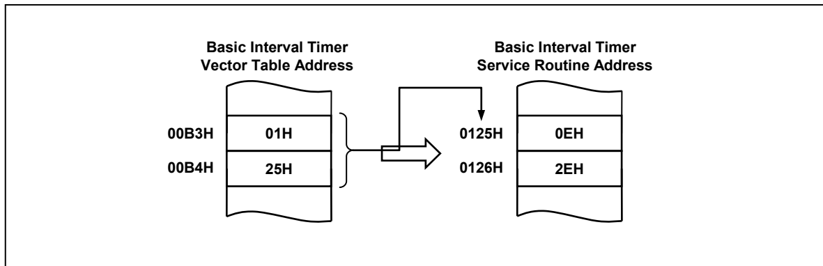
Figure 10-7 Correspondence between vector Table address and the entry address of ISP
