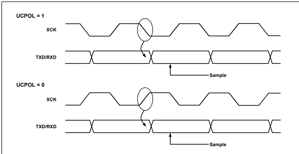
Figure 11-25 Synchronous Mode XCKn Timing
