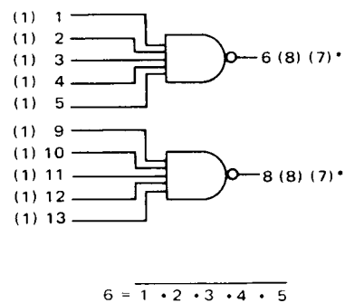
MC1800/MC1900 MC1801/MC1901 Dual 5-Input NAND Gate
