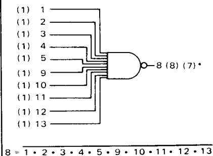
MC1804/MC1904 MC1805/MC1905 10-Input NAND Gate
