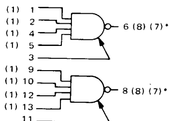
MC830/MC930 MC861/MC961 Expandable Dual 4-Input NAND Gate
