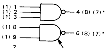
MC830G/MC930G MC861G/MC961G Expandable Dual 3-2 Input NAND Gate
