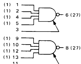
MC844/MC944 Expandable Dual 4-Input Power NAND Gate
