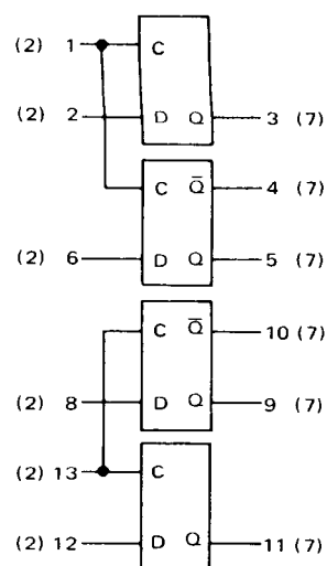
MC1814/MC1914 Quad Latch
