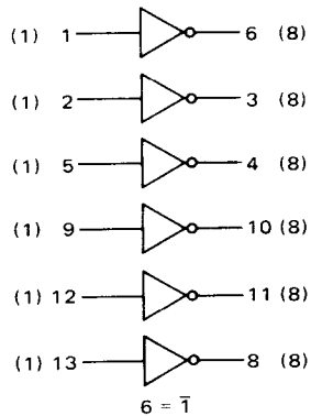
MC840/MC940 Hex Inverter (Without Input Diodes)
