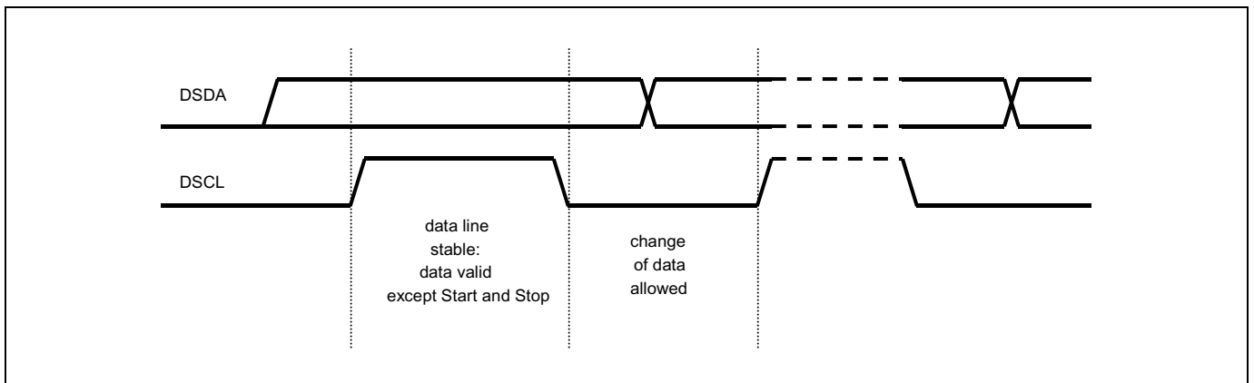
Figure 13.16 Bit Transfer on the Serial Bus
