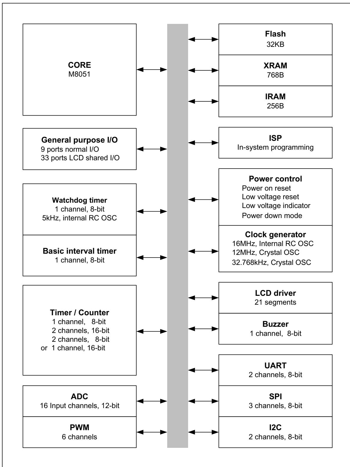
Figure 2.1 Block diagram of MC96F6432S
