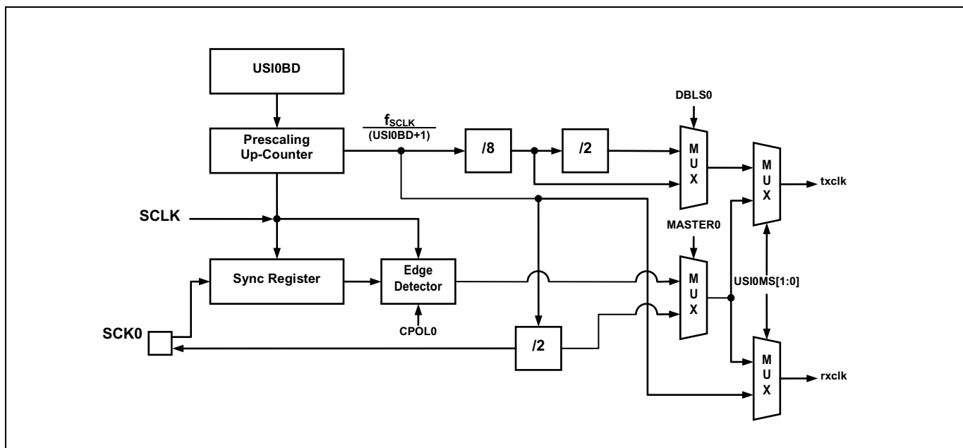
Figure 11.58 Clock Generation Block Diagram (USI0)
