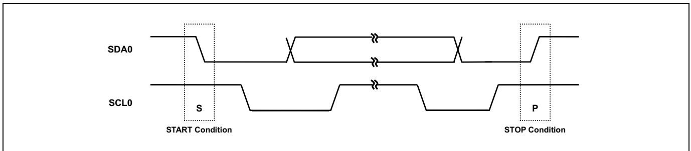
Figure 11.68 START and STOP Condition (USI0)
