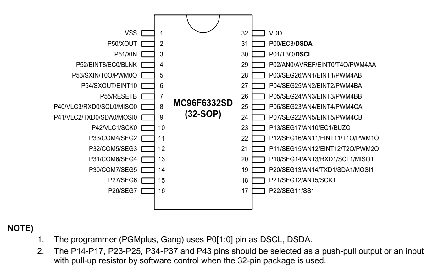
Figure 3.2 MC96F6332SD 32SOP pin assignment
