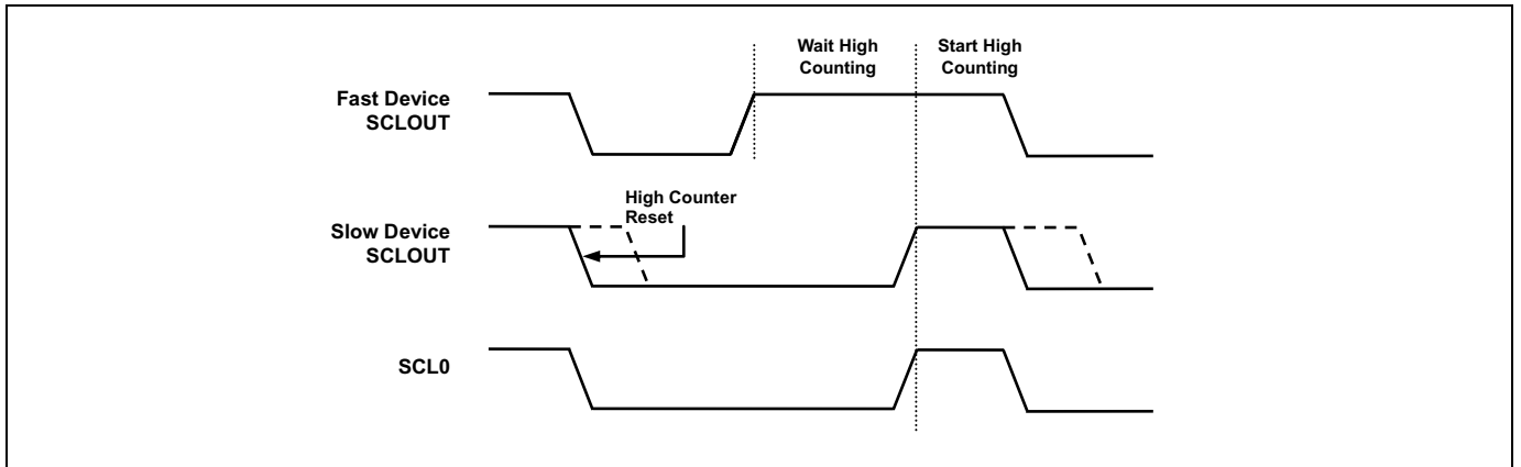
Figure 11.71 Clock Synchronization during Arbitration Procedure (USI0)
