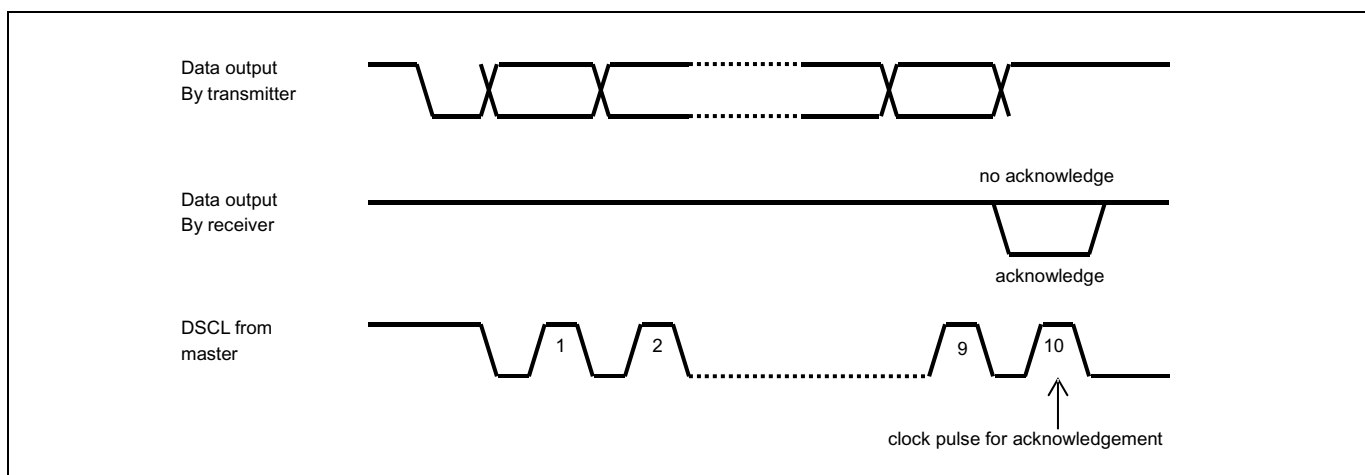
Figure 13.18 Acknowledge on the Serial Bus
