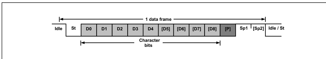
Figure 11.60 Frame Format(USI0)
