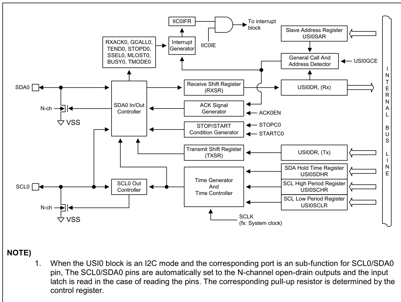
Figure 11.73 USI0 I2C Block Diagram
