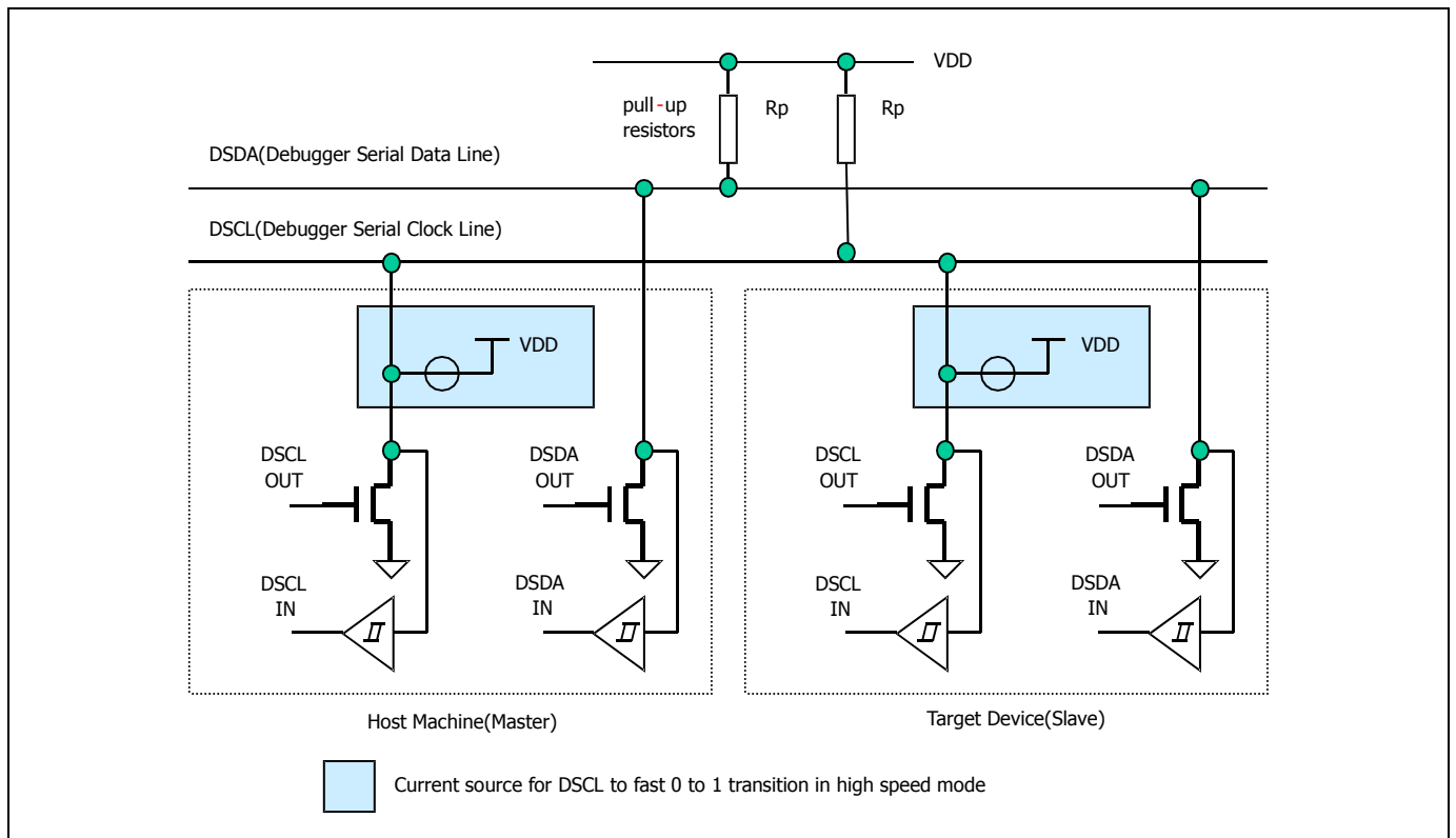
Figure 13.20 Connection of Transmission
