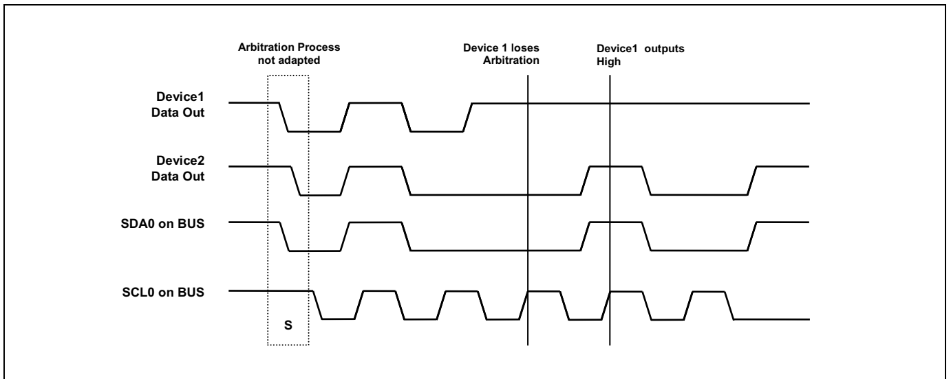
Figure 11.72 Arbitration Procedure of Two Masters (USI0)
