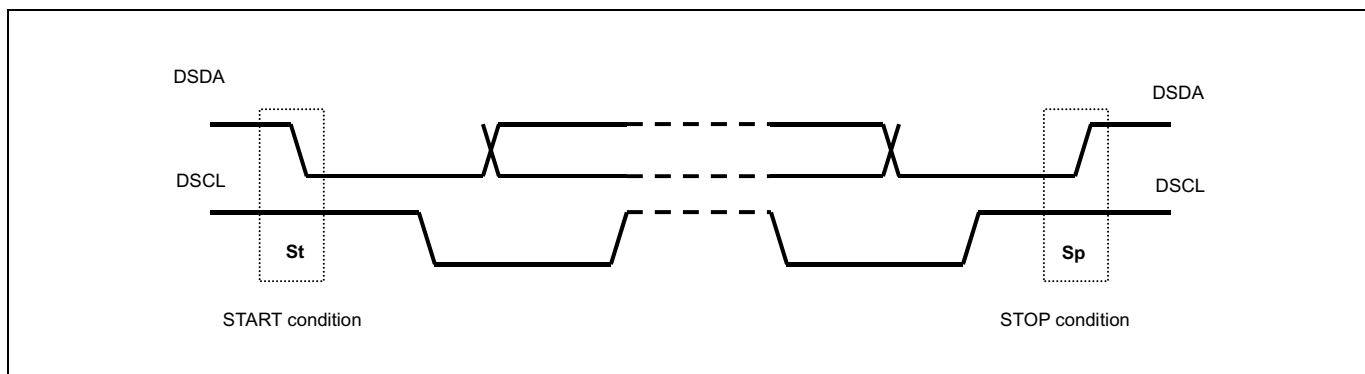
Figure 13.17 Start and Stop Condition
