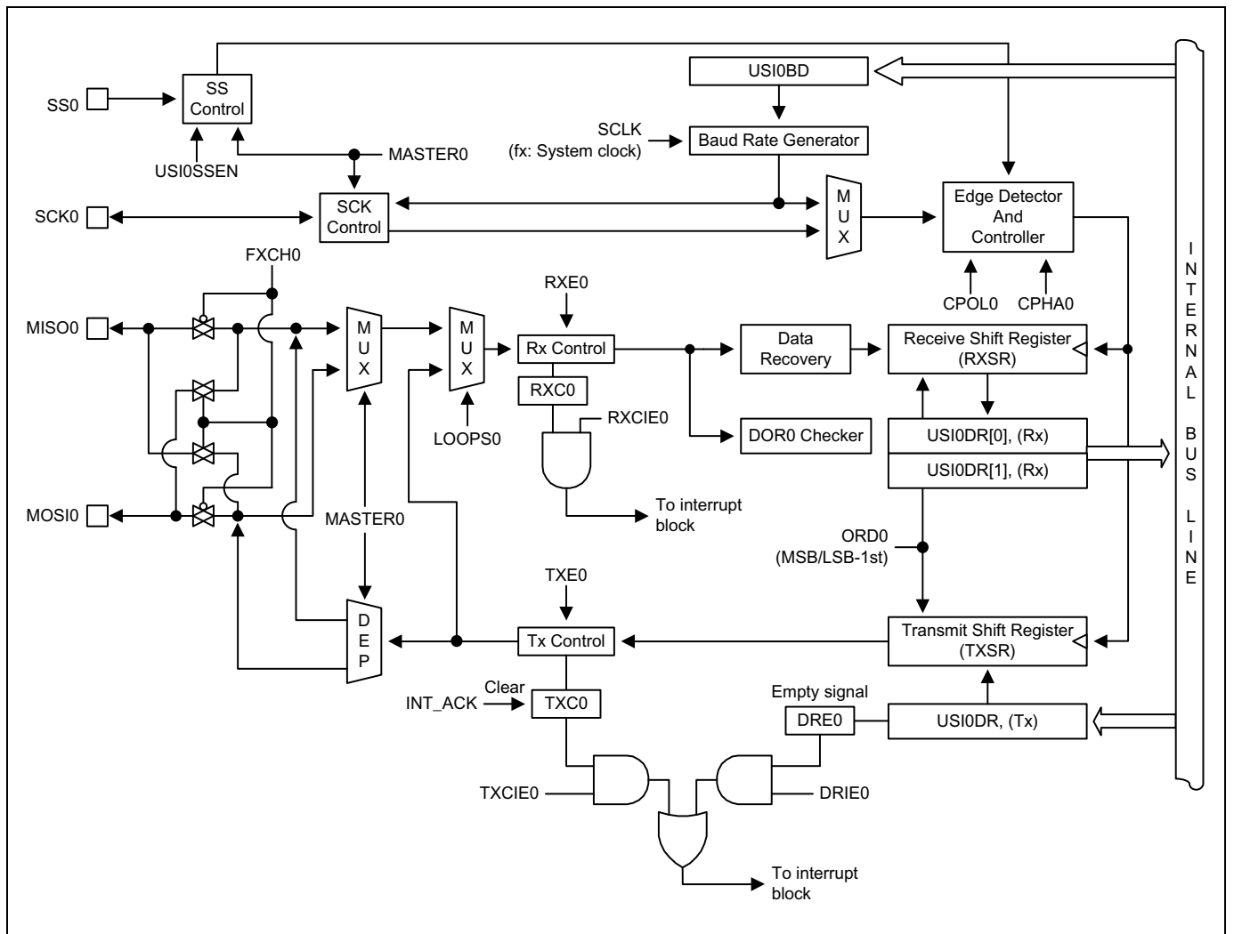
Figure 11.66 USI0 SPI Block Diagram
