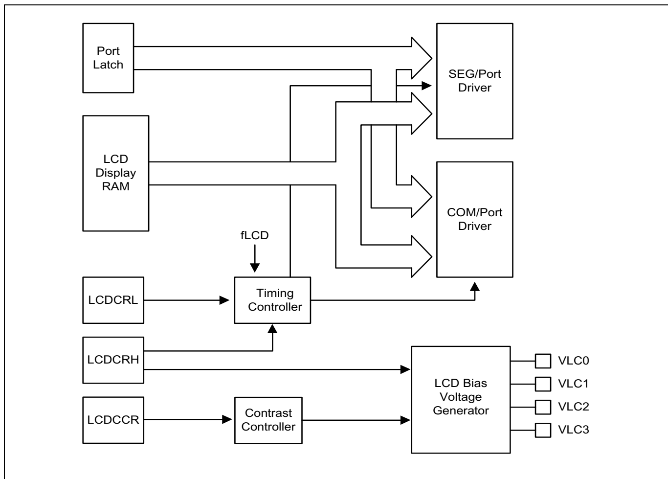
Figure 11.81 LCD Circuit Block Diagram
