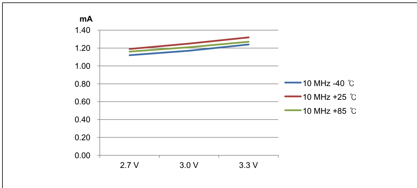
Figure 7.16 IDLE (IDD2) Current
