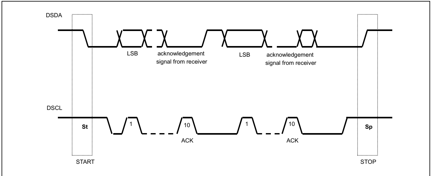
Figure 13.15 Data Transfer on the Twin Bus
