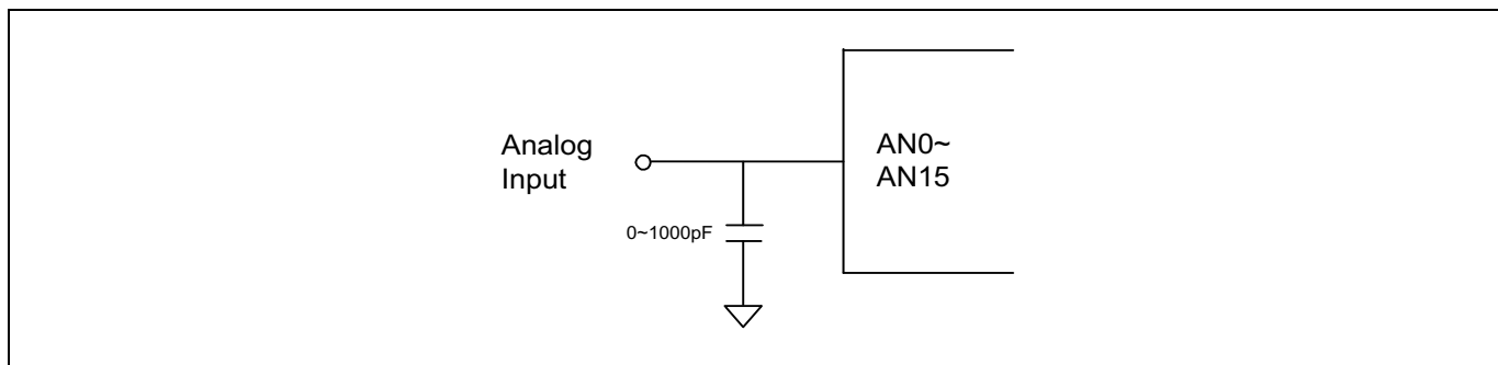
Figure 11.53 A/D Analog Input Pin with Capacitor
