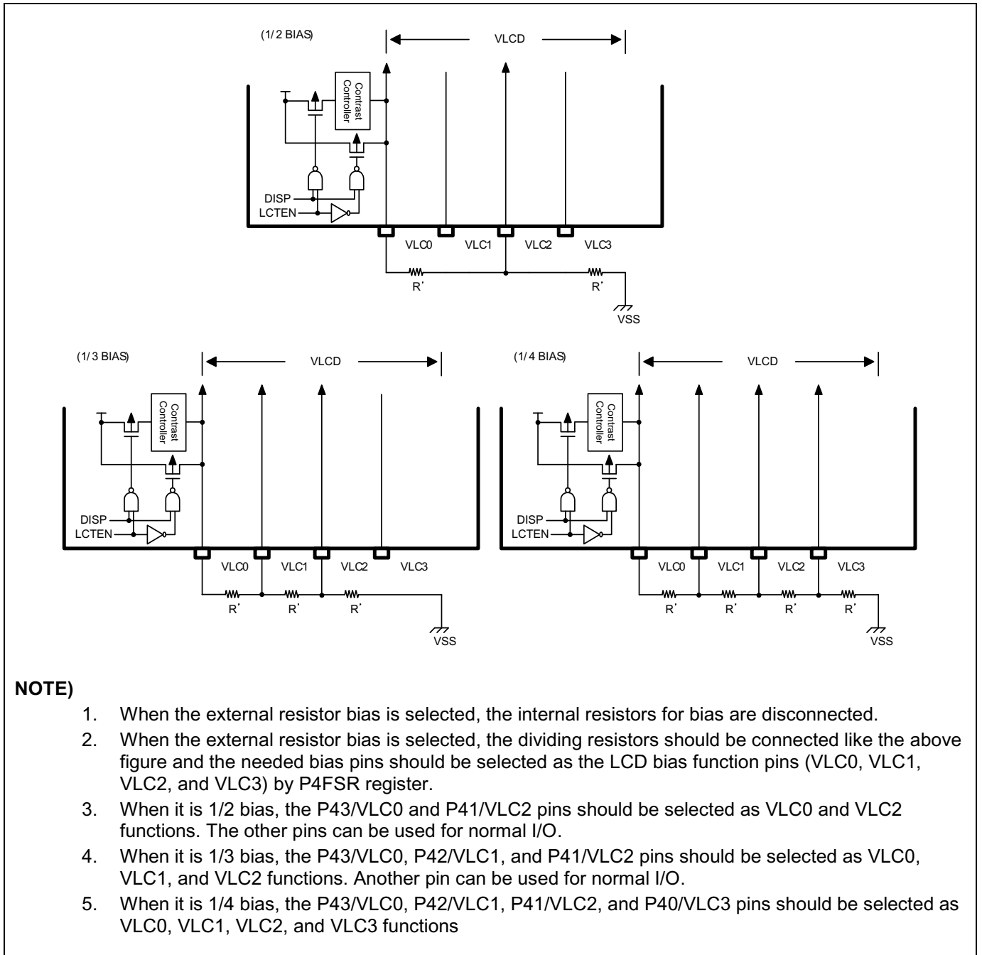
Figure 11.80 External Resistor Bias Connection
