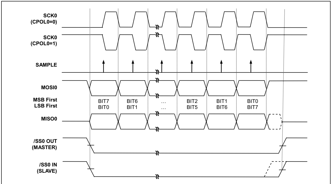
Figure 11.64 USI0 SPI Clock Formats when CPHA0=0
