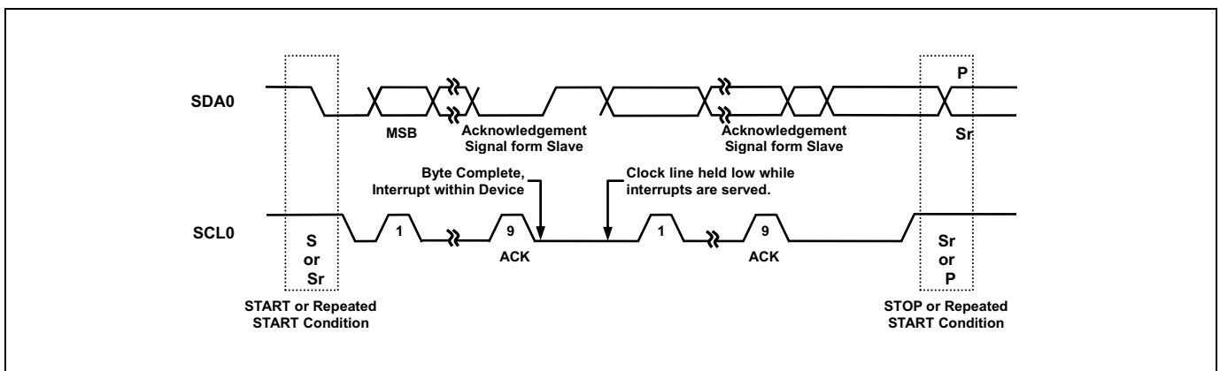
Figure 11.69 Data Transfer on the I2C-Bus (USI0)
