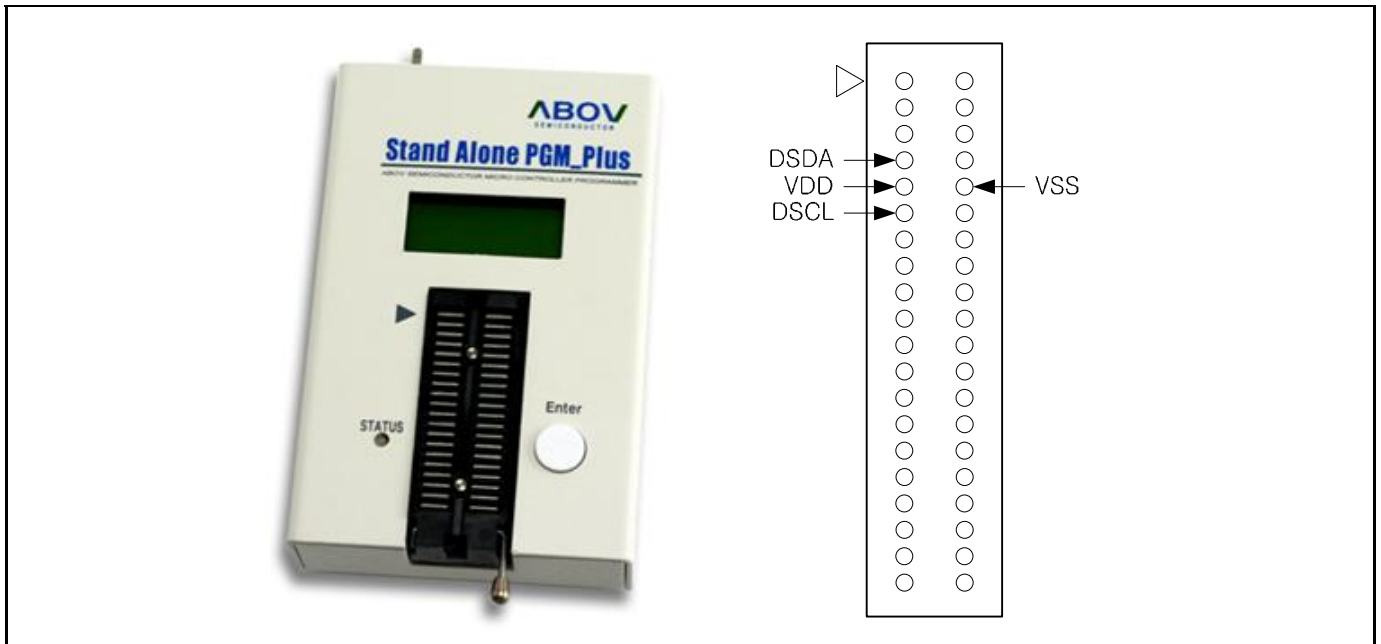
Figure 1.5 Standalone PGMplus(Single writer)
