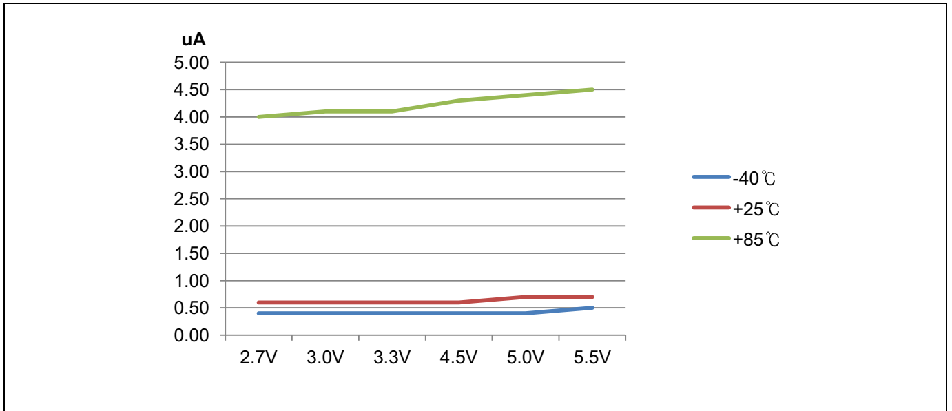
Figure 7.19 STOP (IDD5) Current
