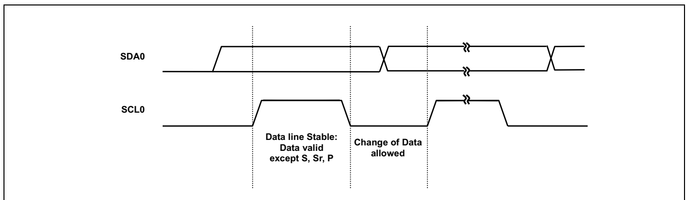
Figure 11.67 Bit Transfer on the I2C-Bus (USI0)
