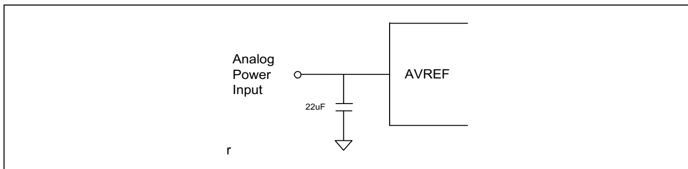
Figure 11.54 A/D Power (AVREF) Pin with Capacitor
