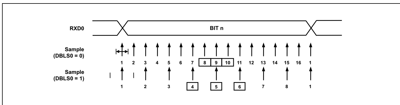
Figure 11.62 Asynchronous Sampling of Data and Parity Bit (USI0)
