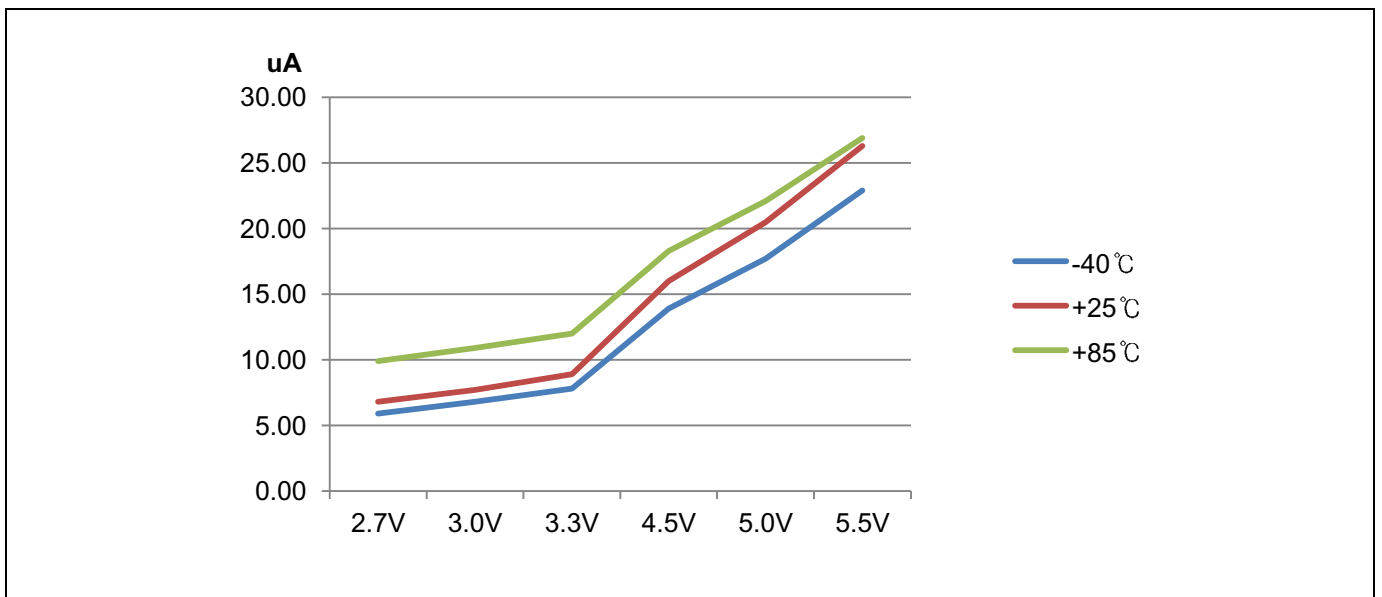
Figure 7.18 SUB IDLE (IDD4) Current
