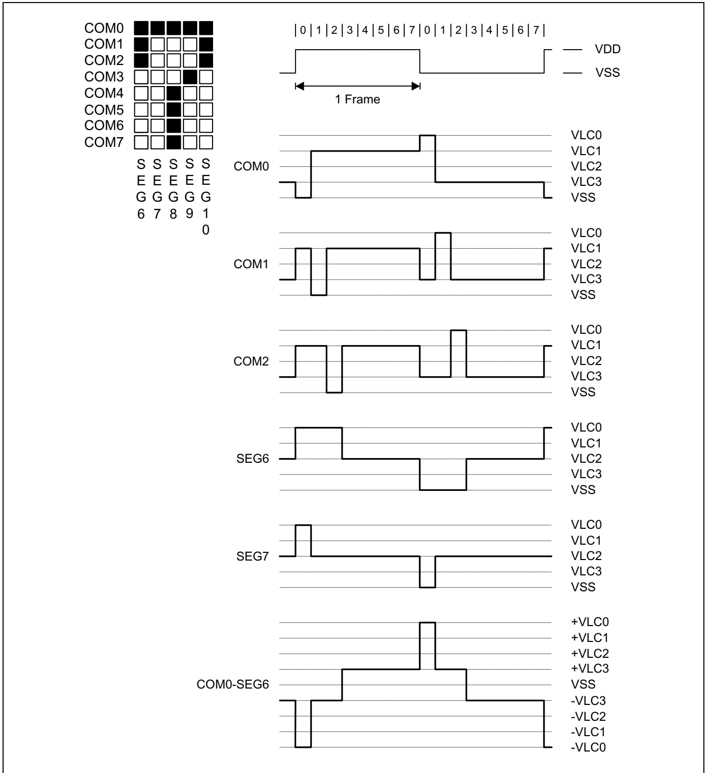
Figure 11.78 LCD Signal Waveforms (1/8Duty, 1/4Bias)
