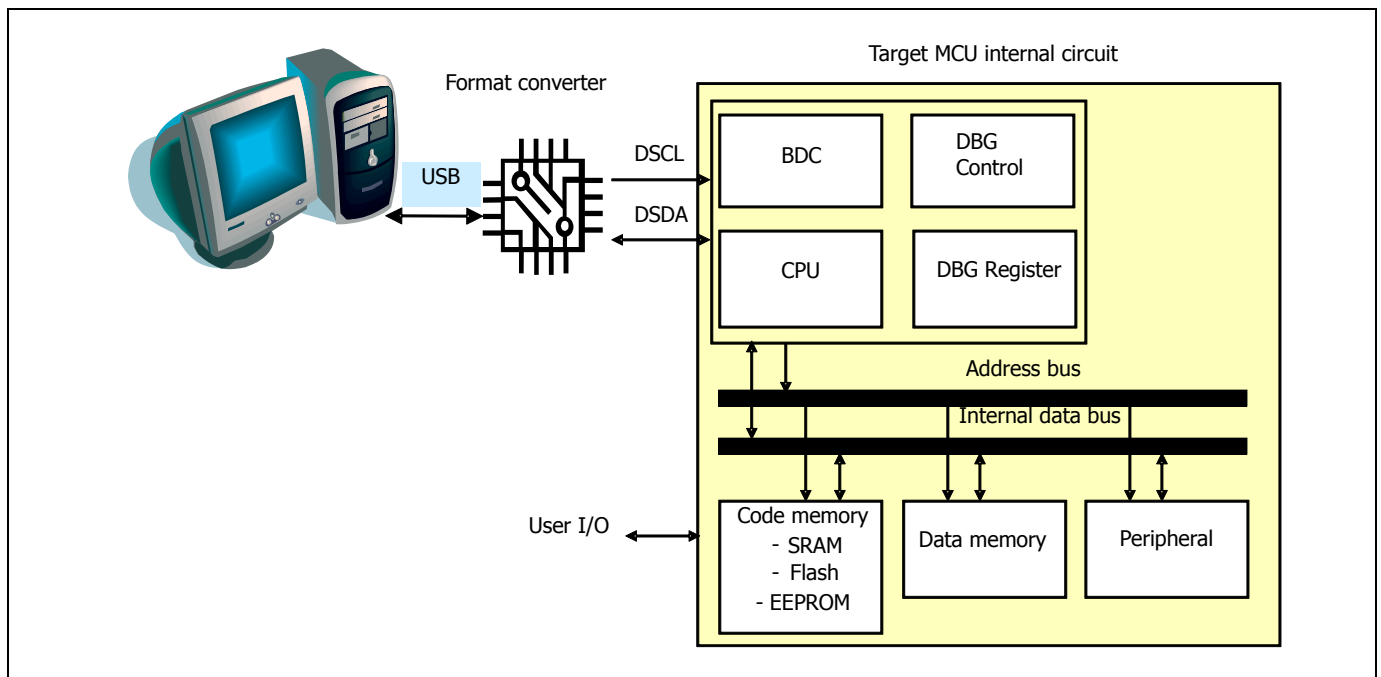
Figure 13.13 Block Diagram of On-Chip Debug System
