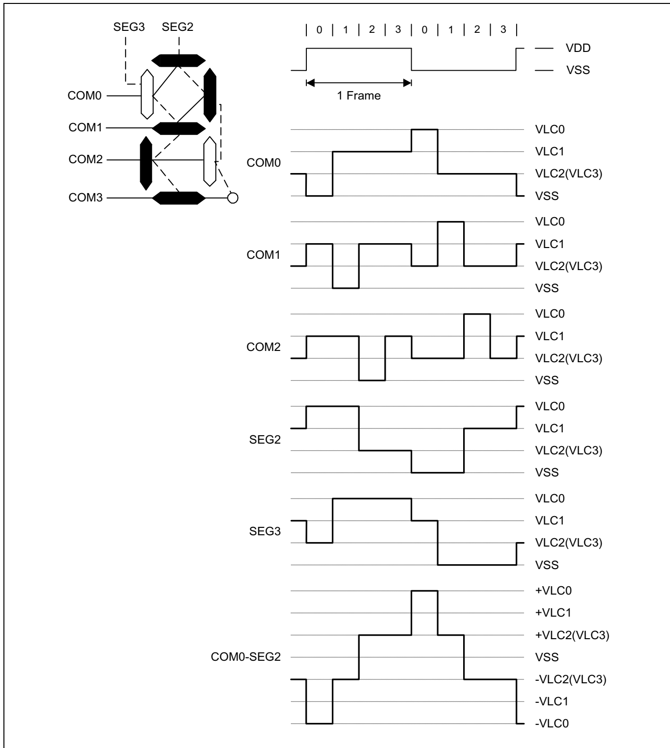
Figure 11.77 LCD Signal Waveforms (1/4Duty, 1/3Bias)
