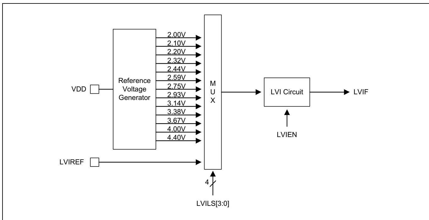
Figure 13.12 LVI Diagram
