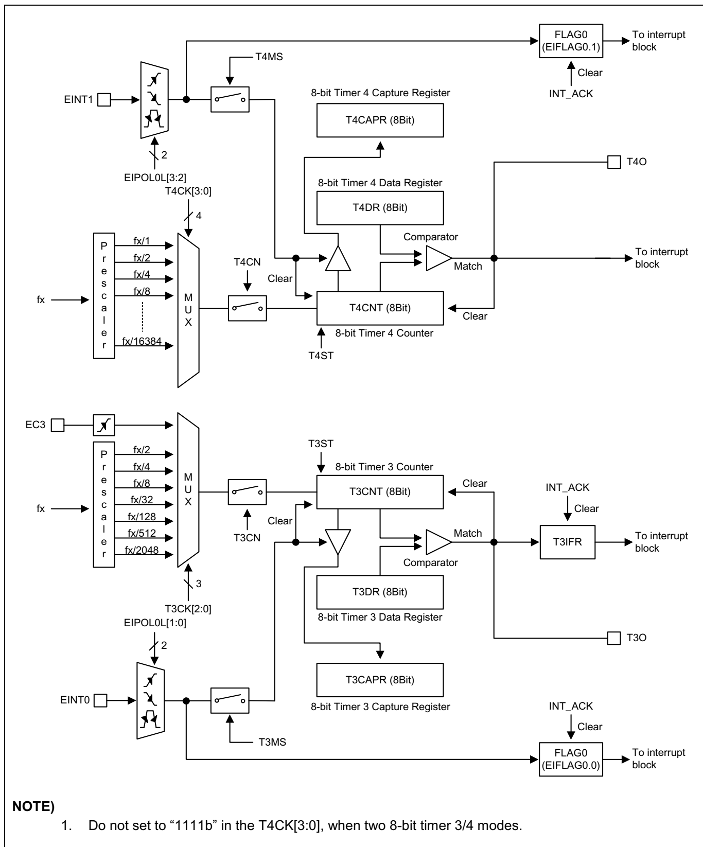
Figure 11.45 Two 8-bit Timer 3, 4 Block Diagram
