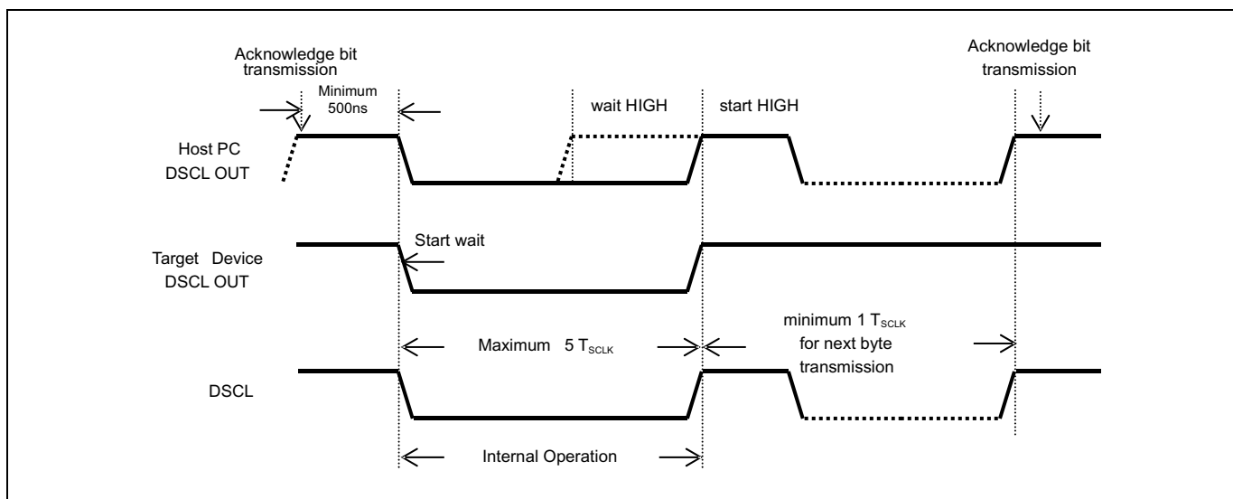
Figure 13.19 Clock Synchronization during Wait Procedure
