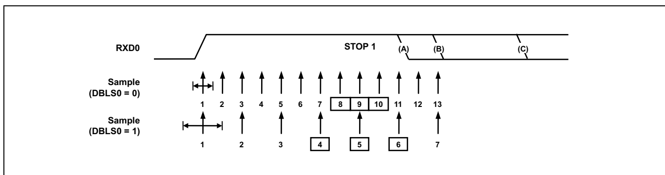
Figure 11.63 Stop Bit Sampling and Next Start Bit Sampling (USI0)
