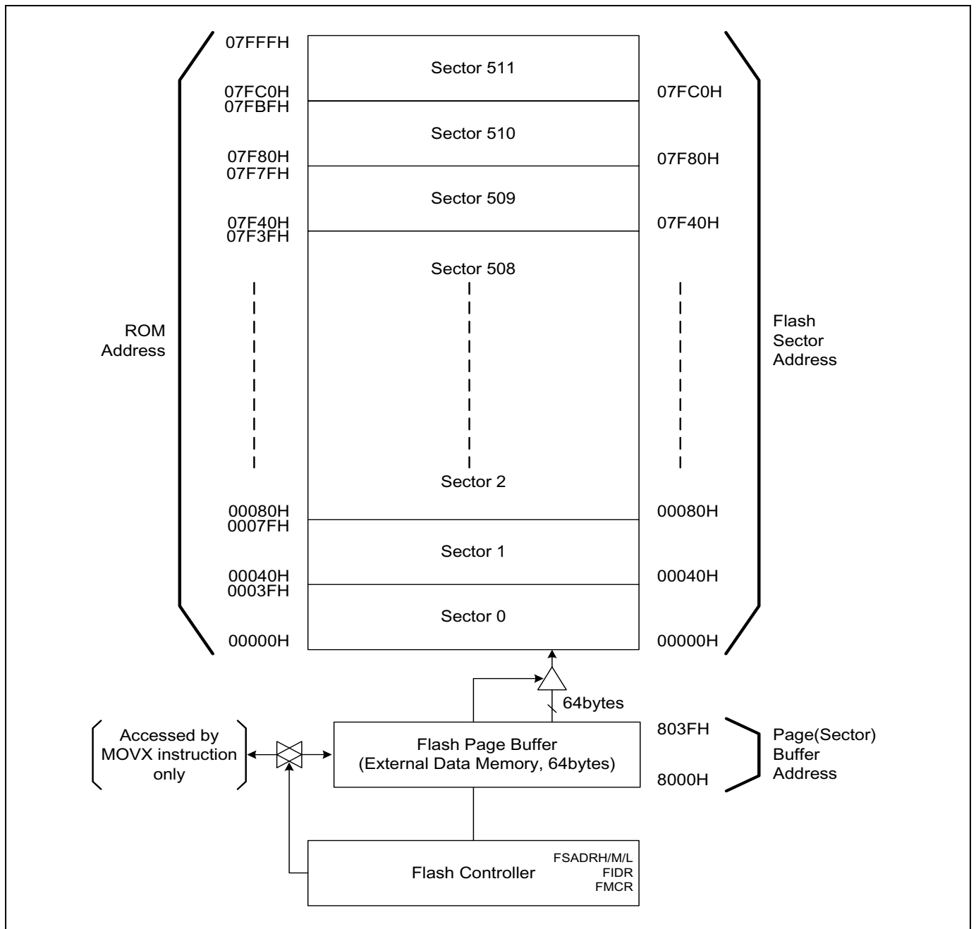
Figure 14.1 Flash Program ROM Structure
