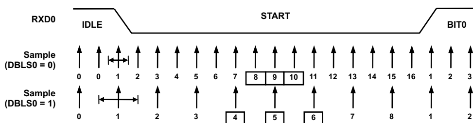
Figure 11.61 Asynchronous Start Bit Sampling (USI0)
