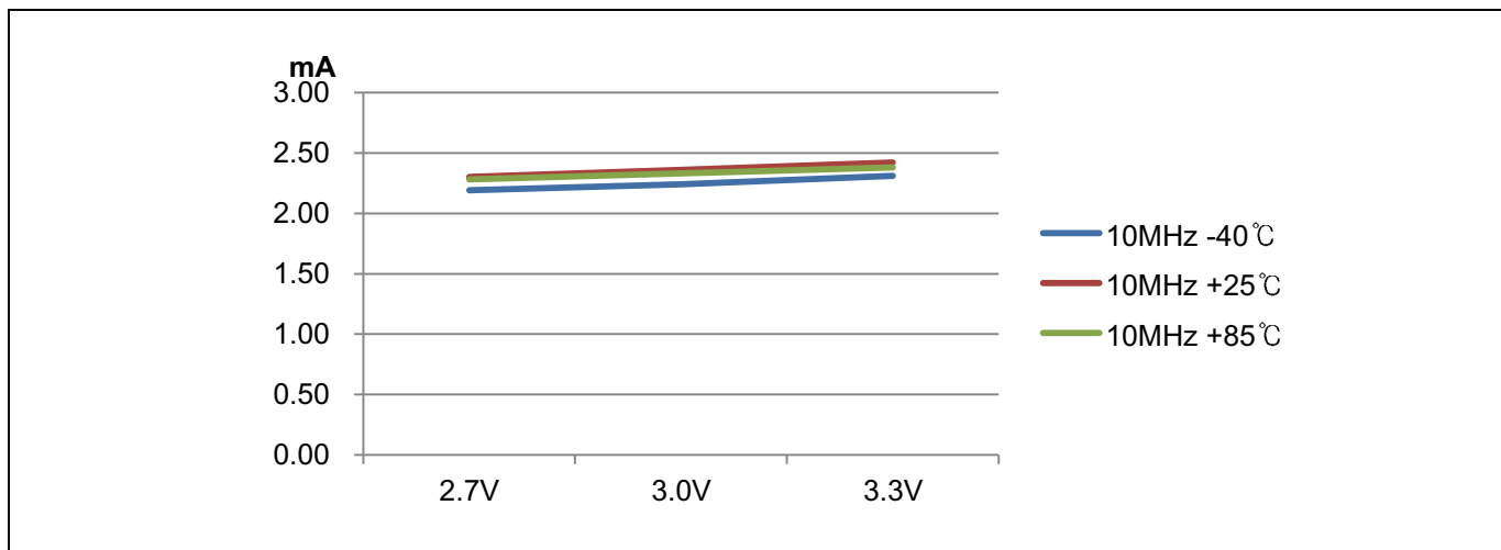
Figure 7.15 RUN (IDD1) Current
