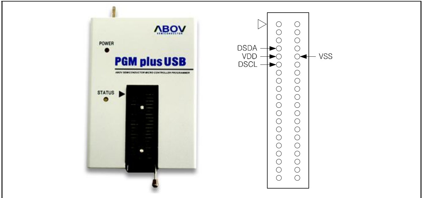
Figure 1.4 PGMplusUSB(Single writer)
