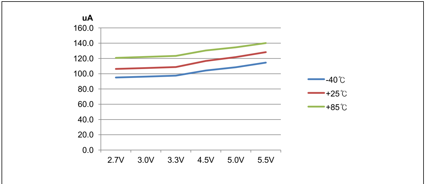
Figure 7.17 SUB RUN (IDD3) Current
