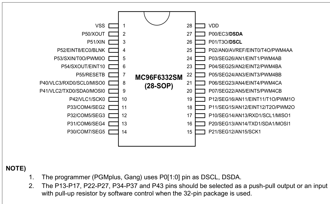
Figure 3.3 MC96F6332SM 28SOP pinassignment
