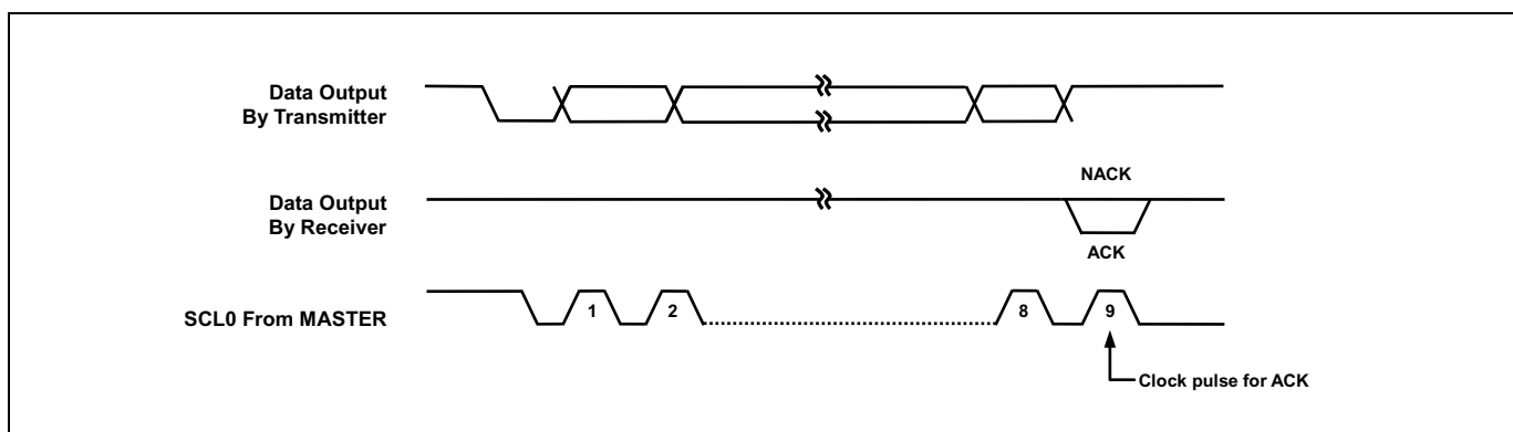
Figure 11.70 Acknowledge on the I2C-Bus (USI0)
