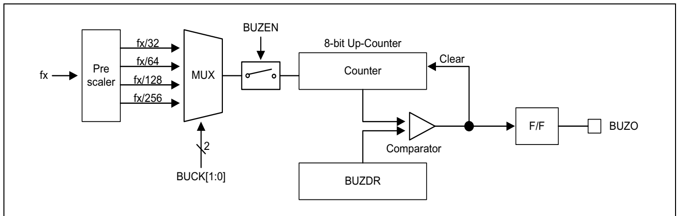
Figure 11.48 Buzzer Driver Block Diagram
