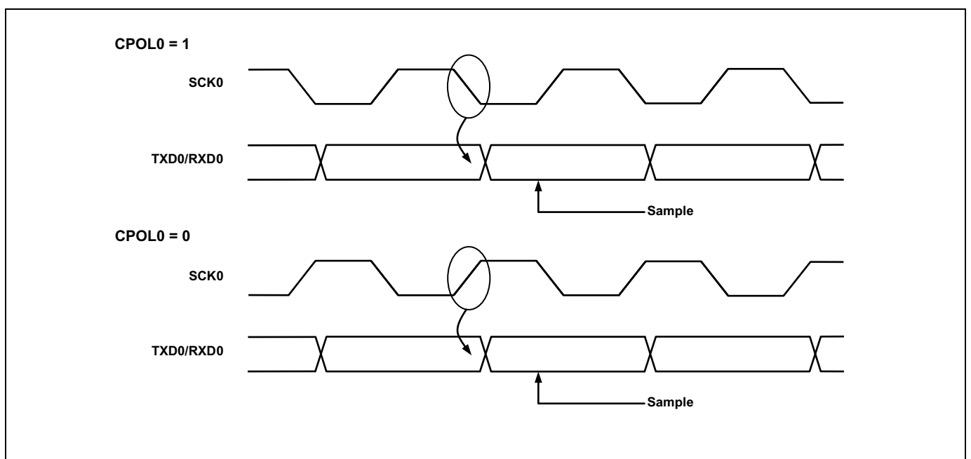
Figure 11.59 Synchronous Mode SCK0 Timing (USI0)
