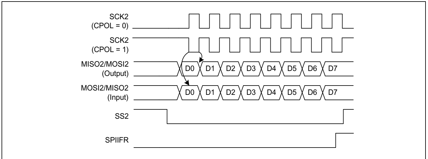
Figure 11.50 SPI 2 Transmit/Receive Timing Diagram at CPHA = 0
