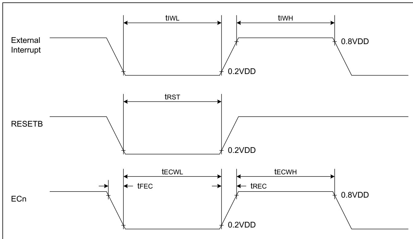
Figure 7.1 AC Timing
