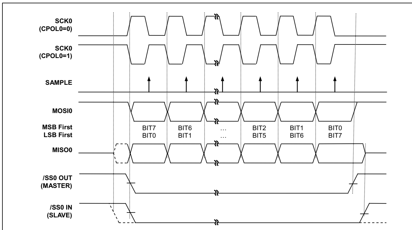
Figure 11.65 USI0 SPI Clock Formats when CPHA0=1
