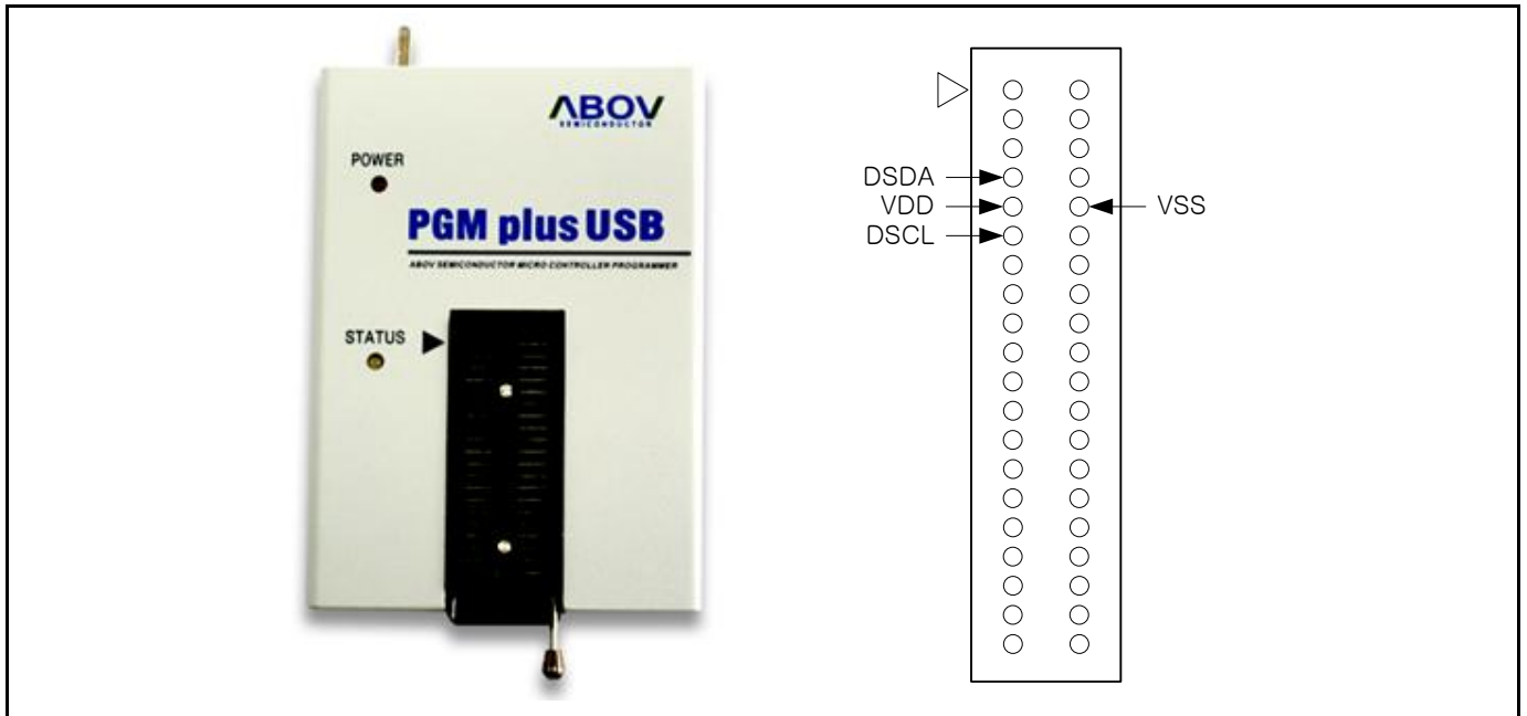
Figure 1-1. PGMplusUSB(Single writer)
