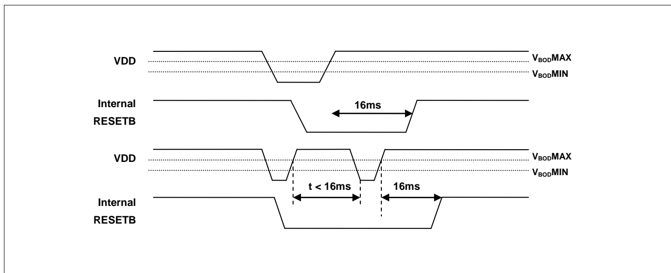
Figure 13-10. Internal Reset at the power fail situation
