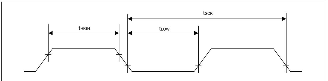
Figure 7-4. Input Timing for RESETB
