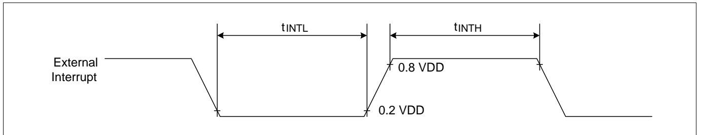
Figure 7-1. Input Timing for External Interrupts
