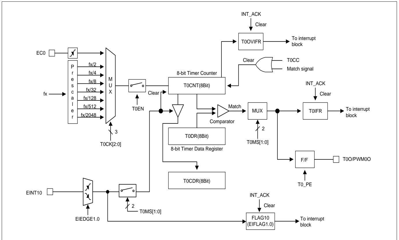
Figure 11-13. 8-Bit Timer 0 Block Diagram
