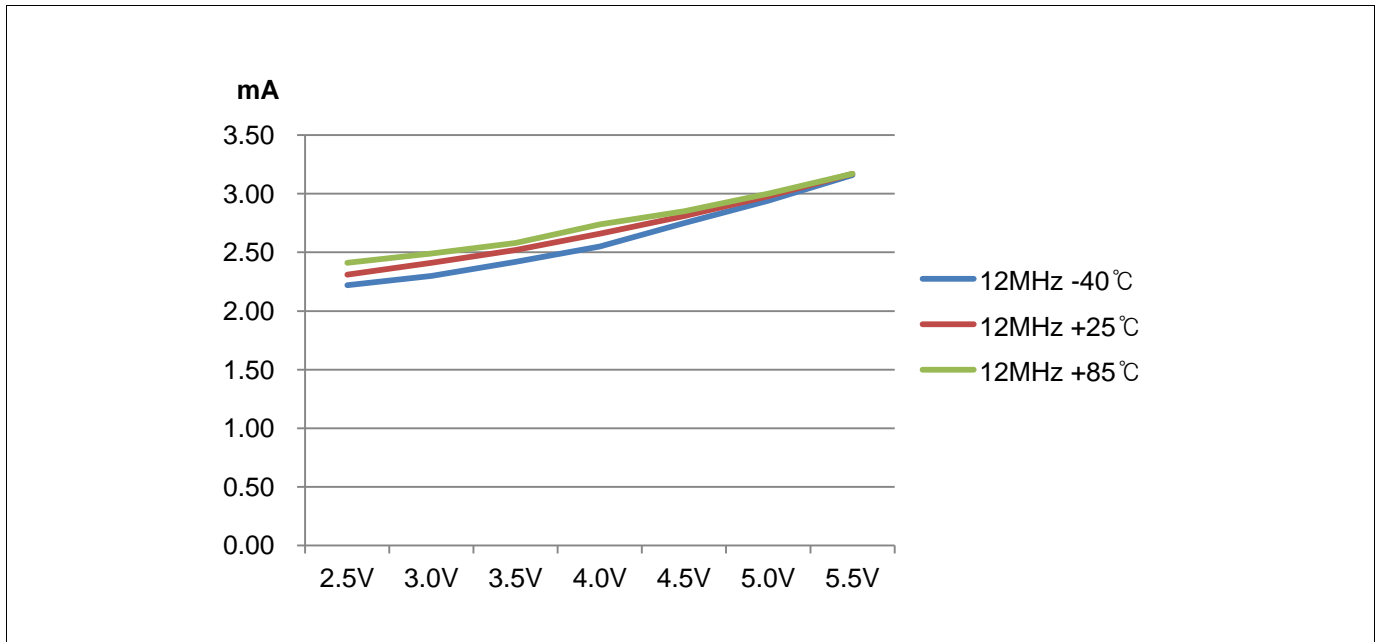
Figure 7-16. RUN (IDD1) Current
