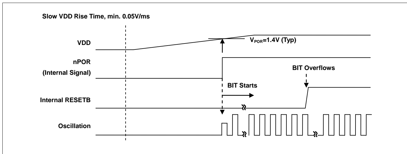
Figure 13-4. Internal RESET Release Timing On Power-Up
