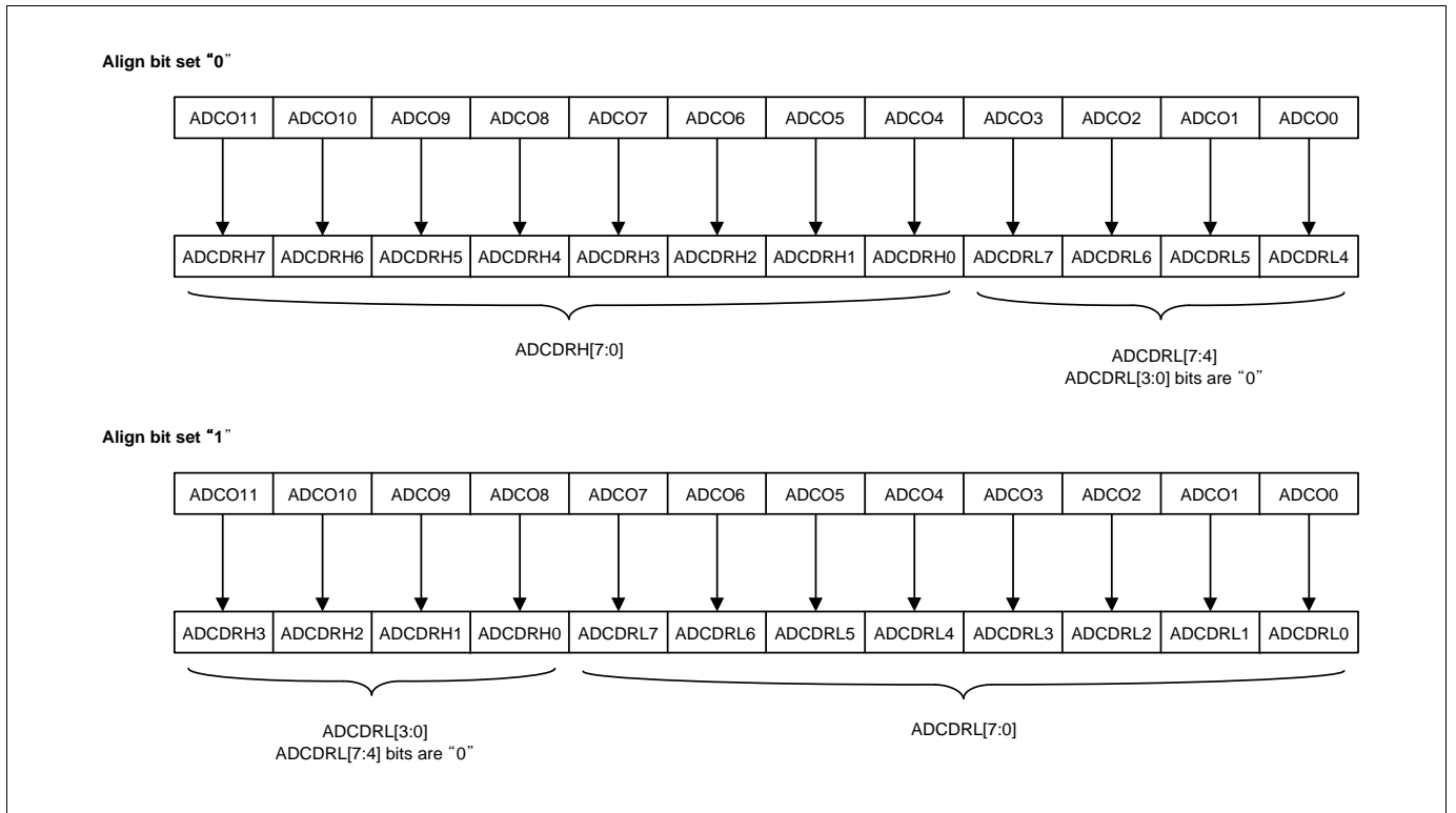
Figure 11-33. ADC Operation for Align Bit
