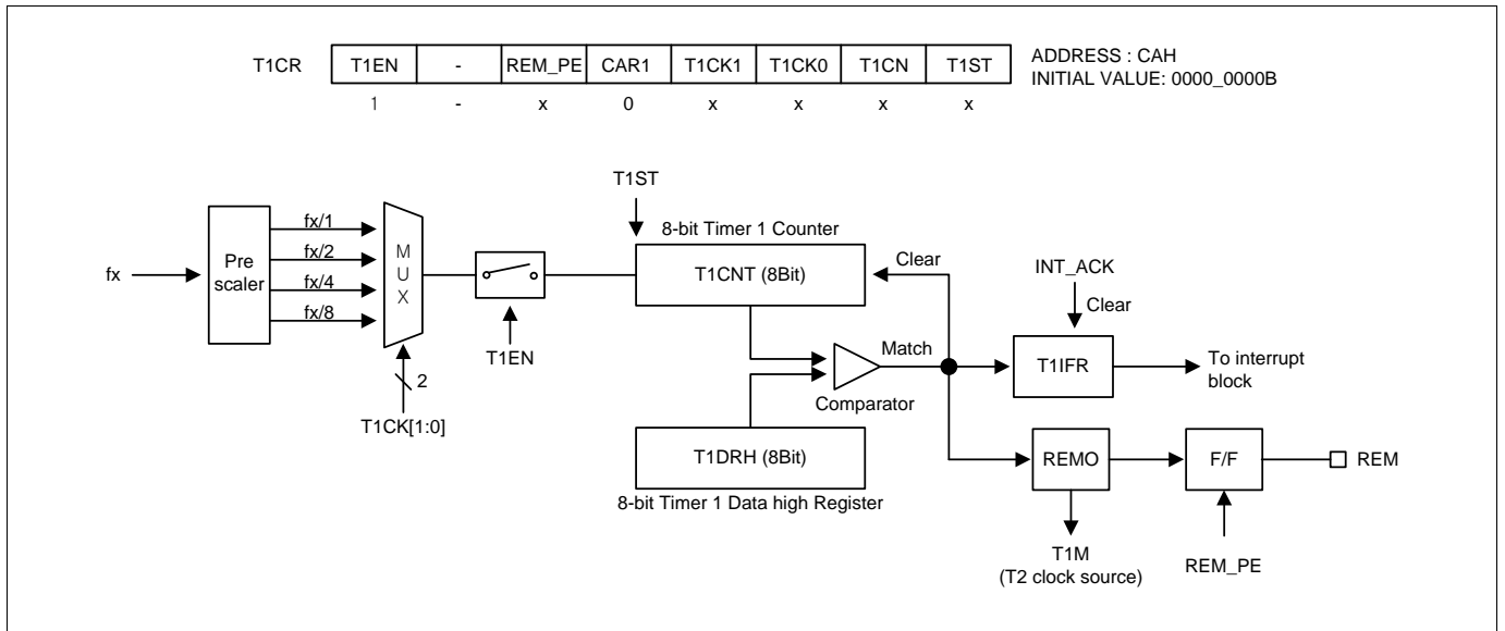
Figure 11-14. 8-Bit Timer/Counter Mode for Timer 1
