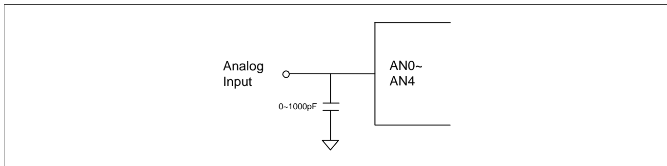
Figure 11-31. A/D Analog Input Pin with Capacitor
