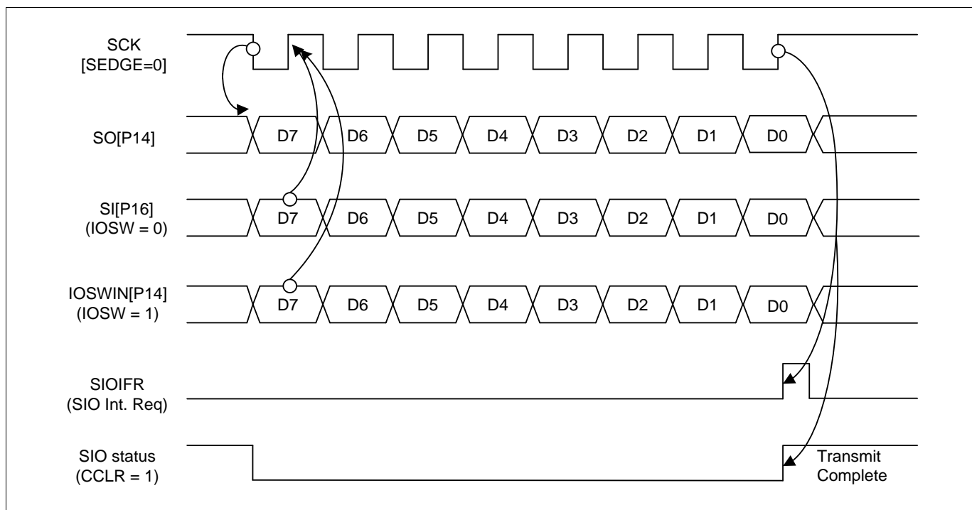
Figure 11-28. SIO Timing Diagram at SEDGE=0
