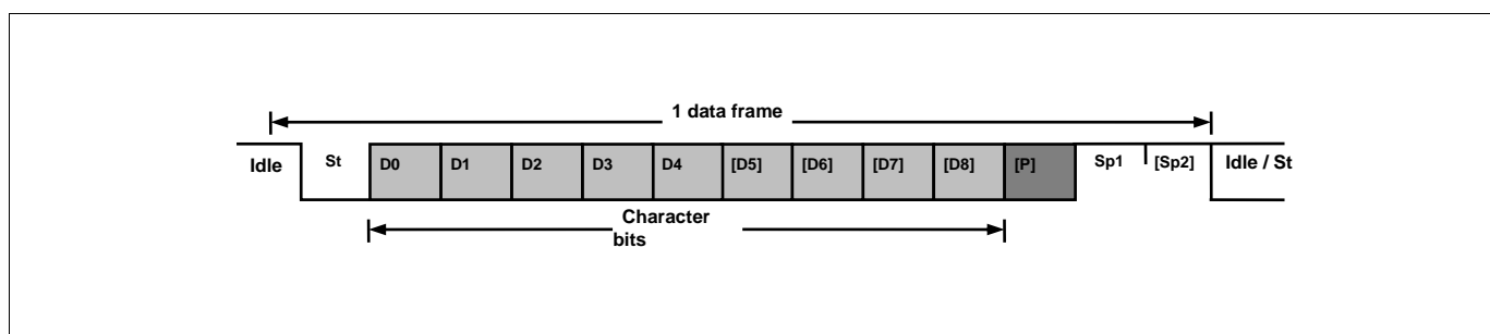
Figure 11-38. Frame Format
