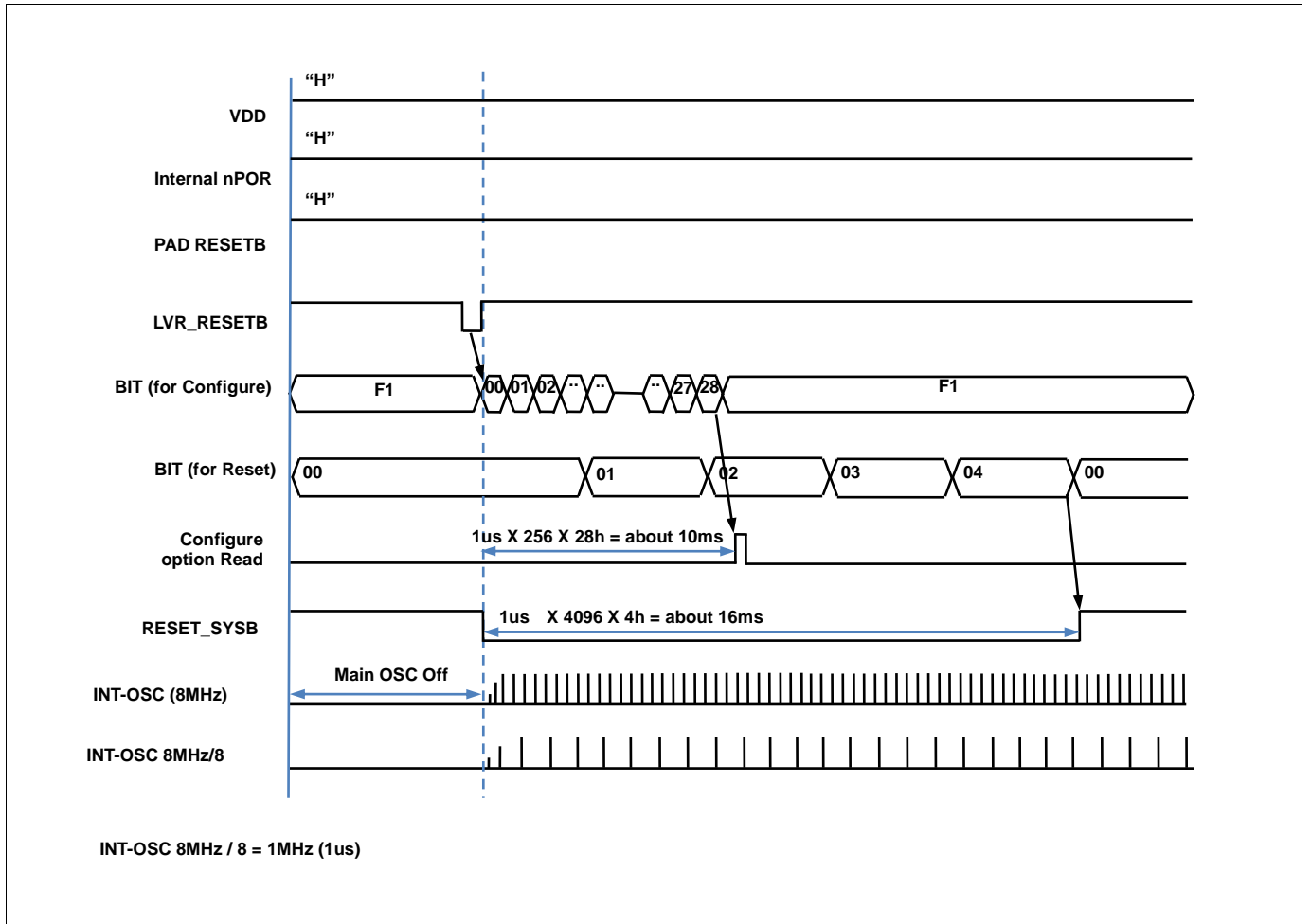
Figure 13-11. Configuration timing when BOD RESET
