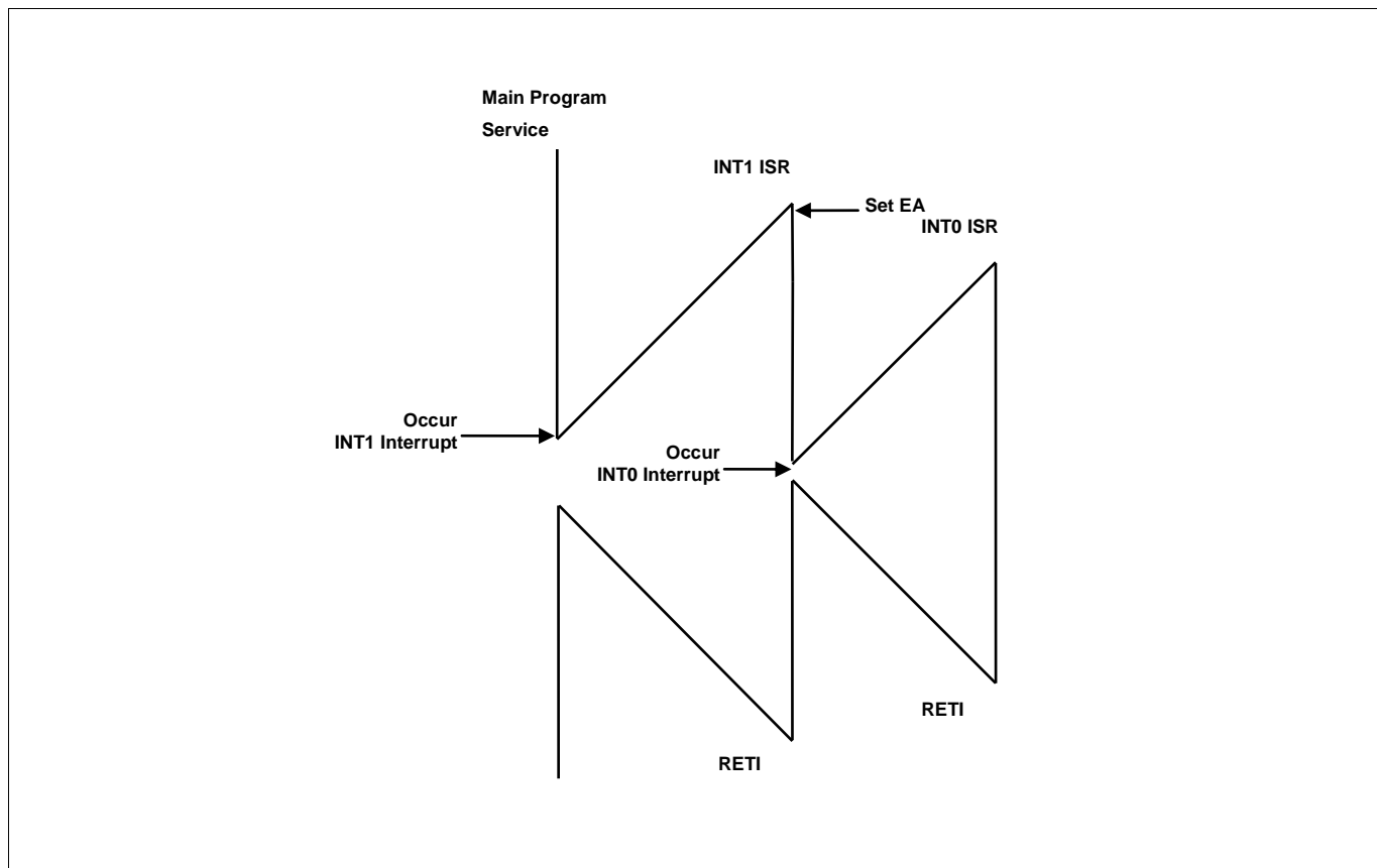
Figure 10-6. Effective Timing of Interrupt
