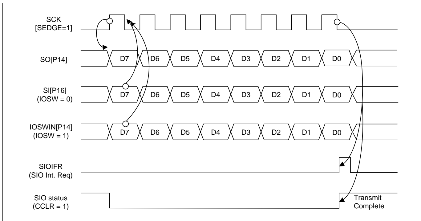
Figure 11-29. SIO Timing Diagram at SEDGE=1
