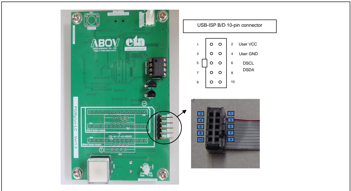
Figure 1-3. PGMplusLC writer
