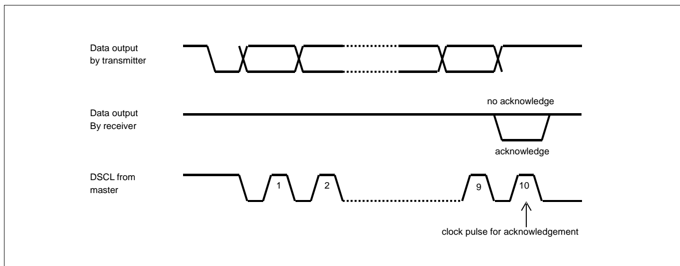
Figure 14-6. Acknowledge on the Serial Bus
