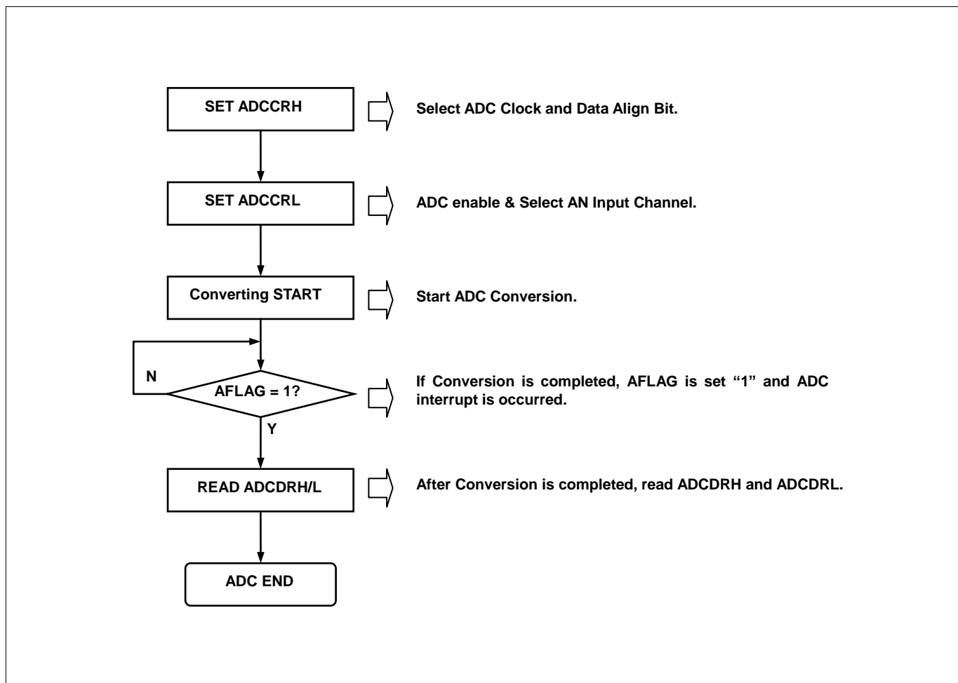
Figure 11-34. A/D Converter Operation Flow
