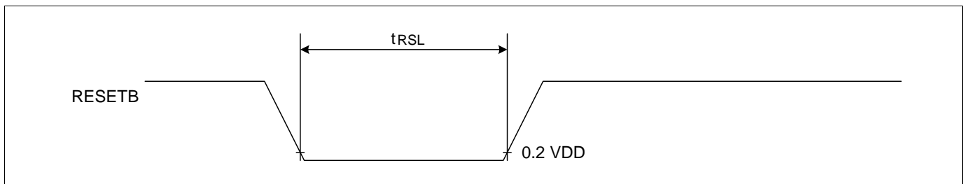
Figure 7-2. Input Timing for RESETB
