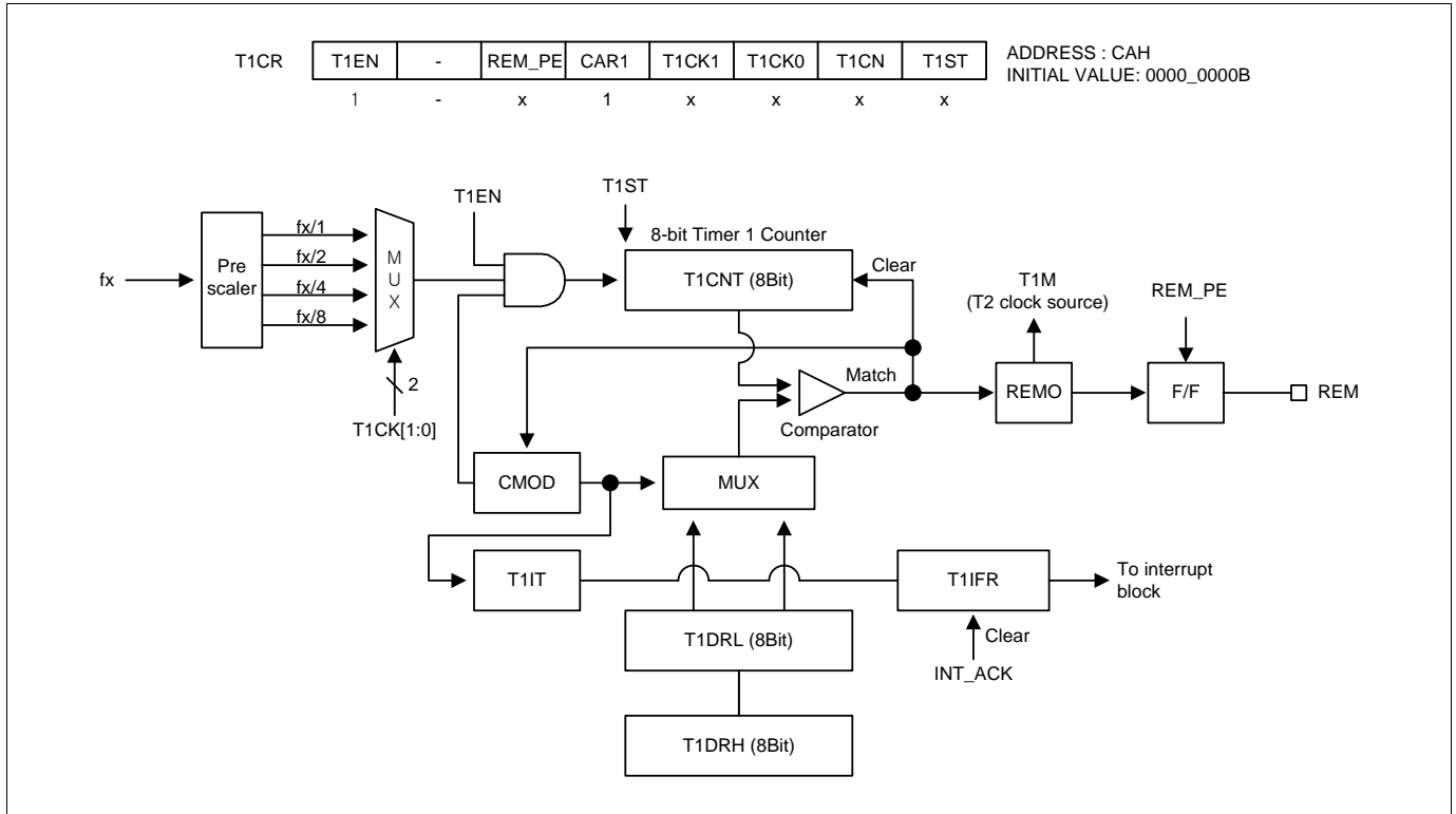
Figure 11-17. Carrier Mode for Timer 1
