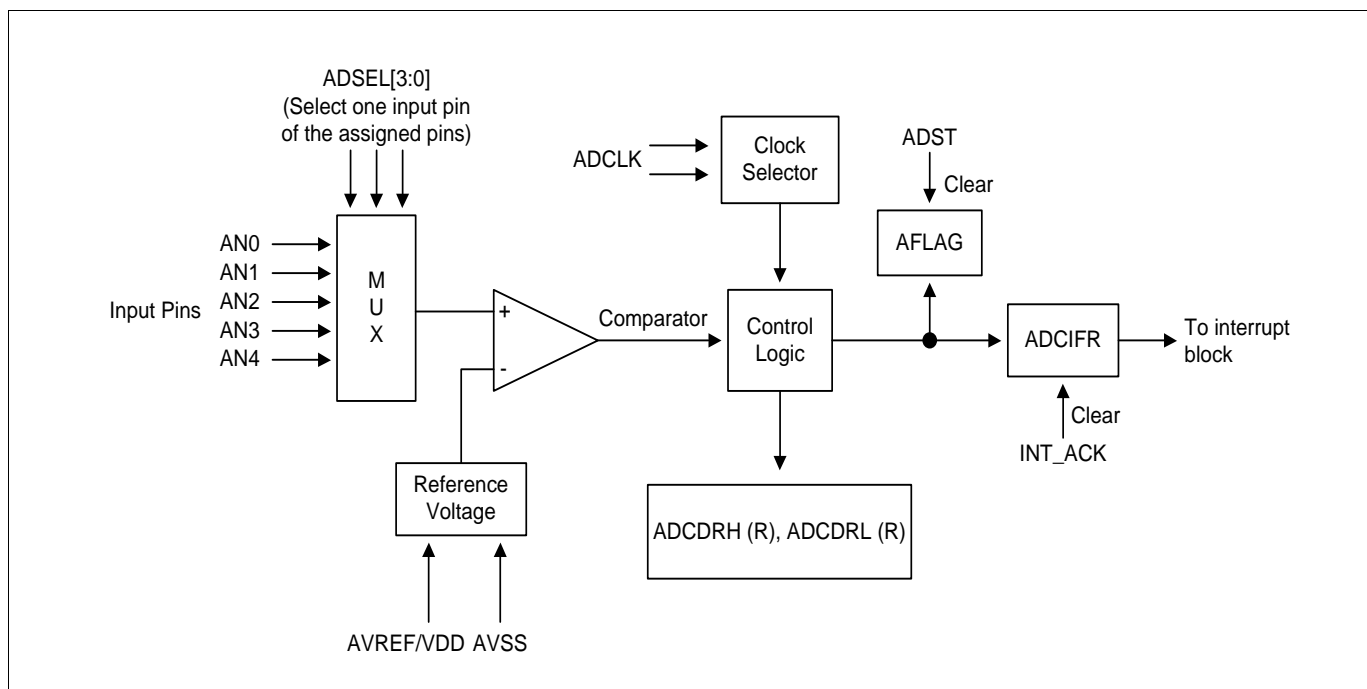
Figure 11-30. 12-bit ADC Block Diagram
