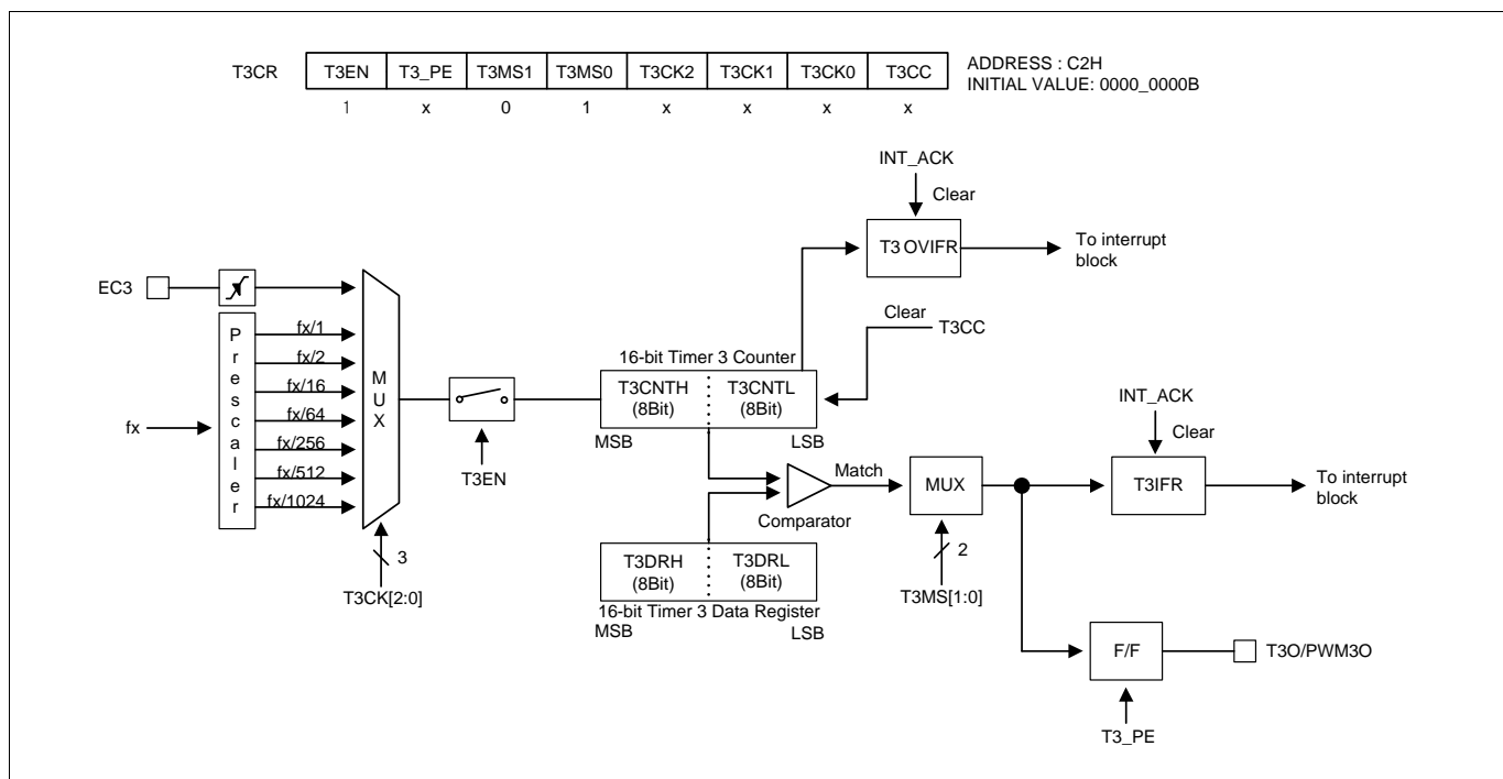
Figure 11-22. 16-Bit PWM Mode for Timer 3
