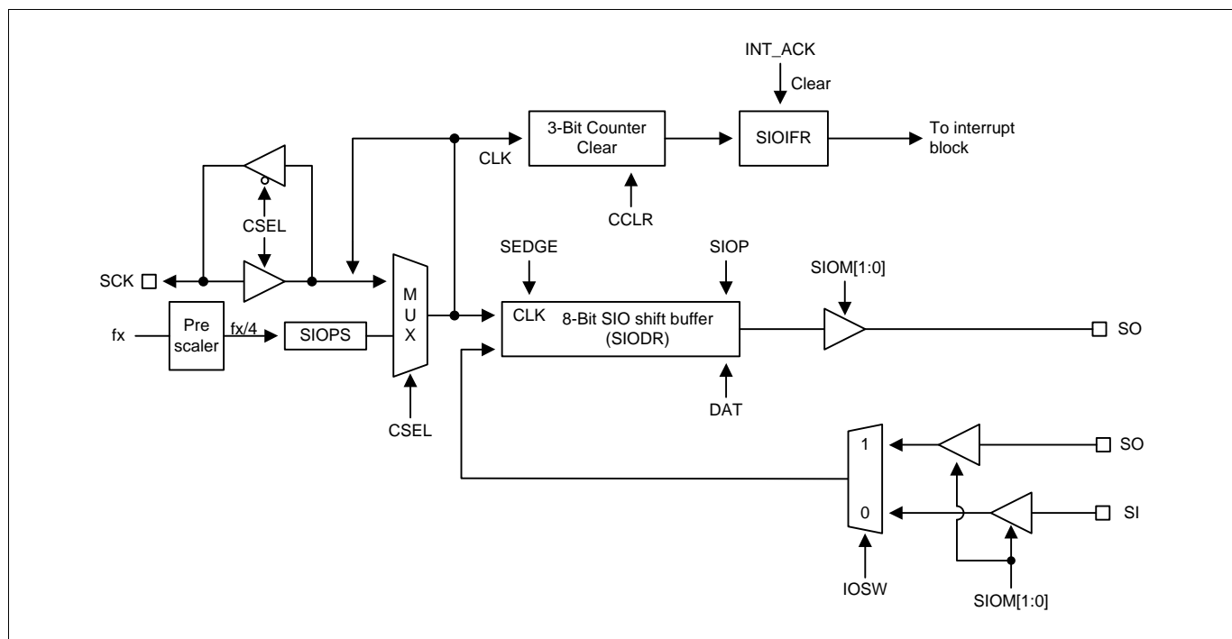
Figure 11-26. SIO Block Diagram
