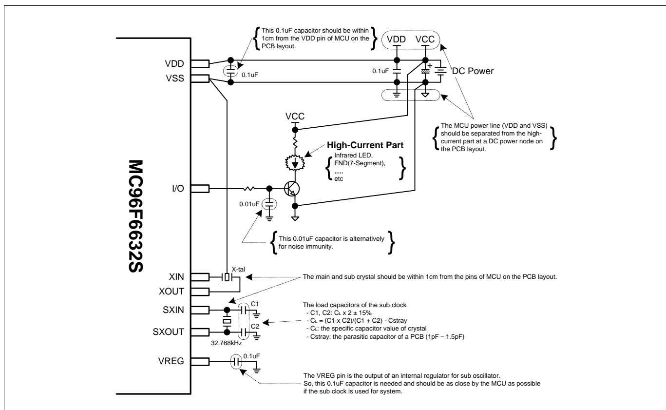
Figure 7-15. Recommended Circuit and Layout
