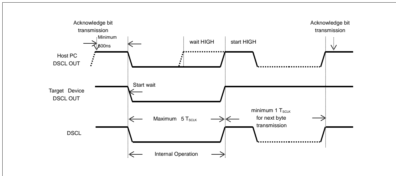
Figure 14-7. Clock Synchronization during Wait Procedure
