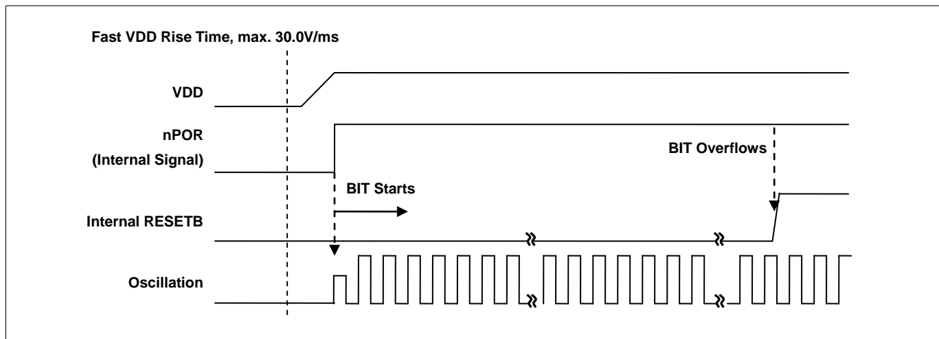
Figure 13-3. Fast VDD Rising Time
