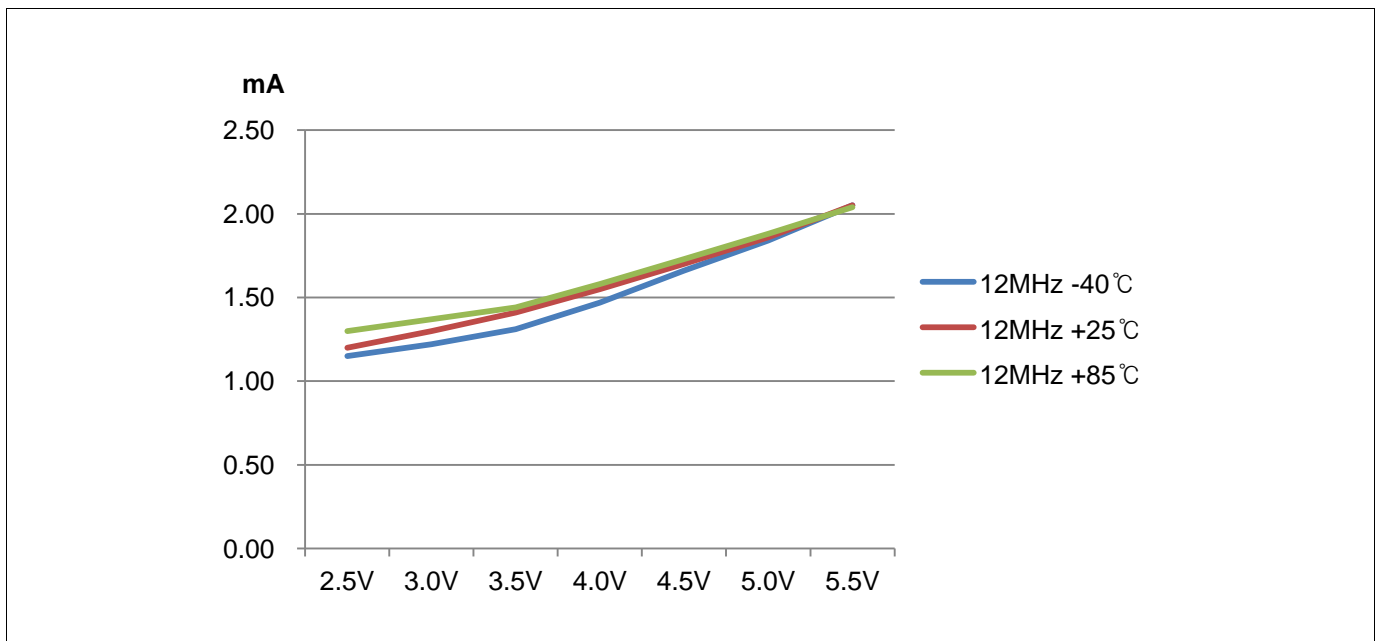
Figure 7-17. IDLE (IDD2) Current
