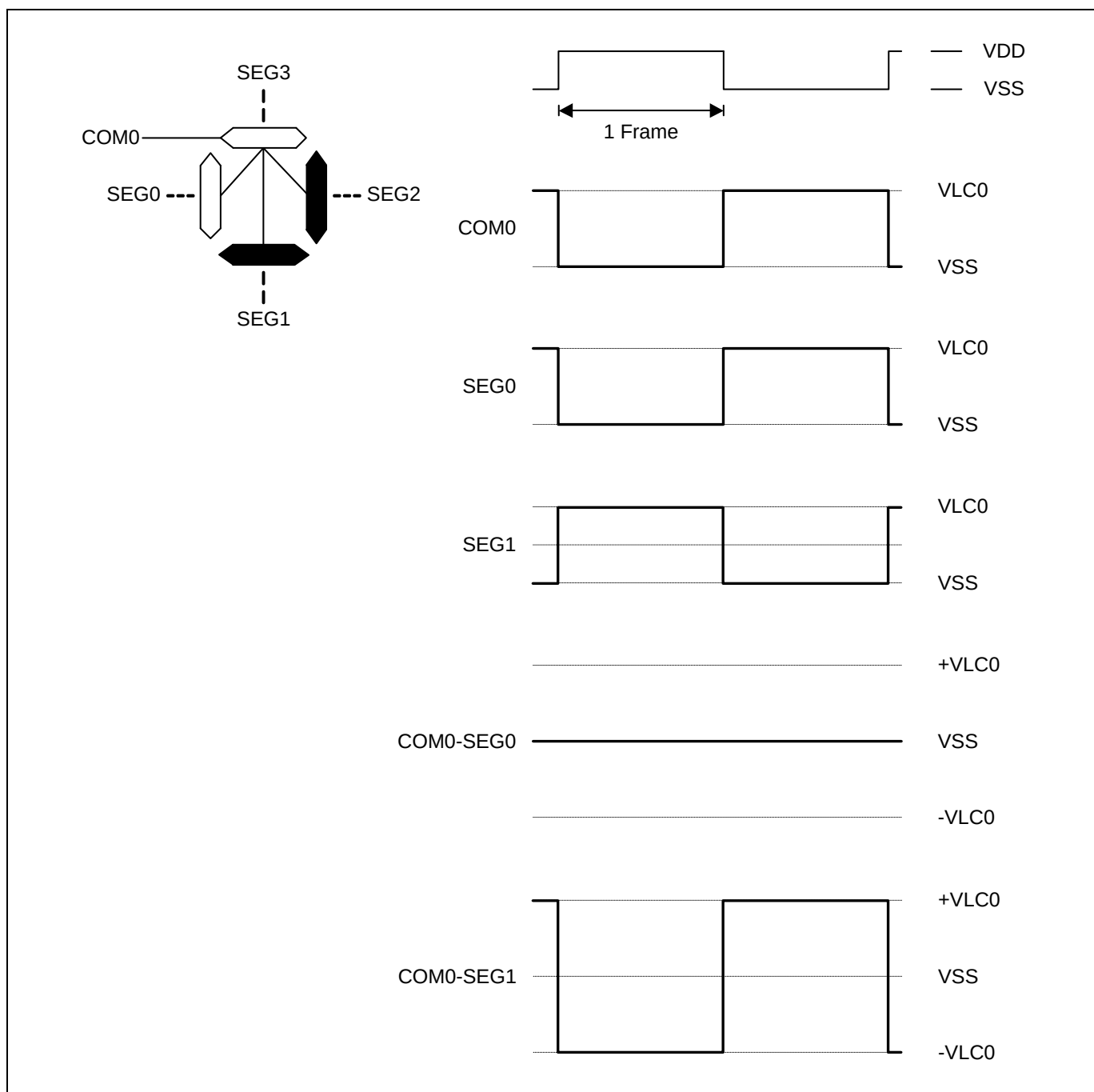
Figure 11.34 LCD Signal Waveforms (Static)
