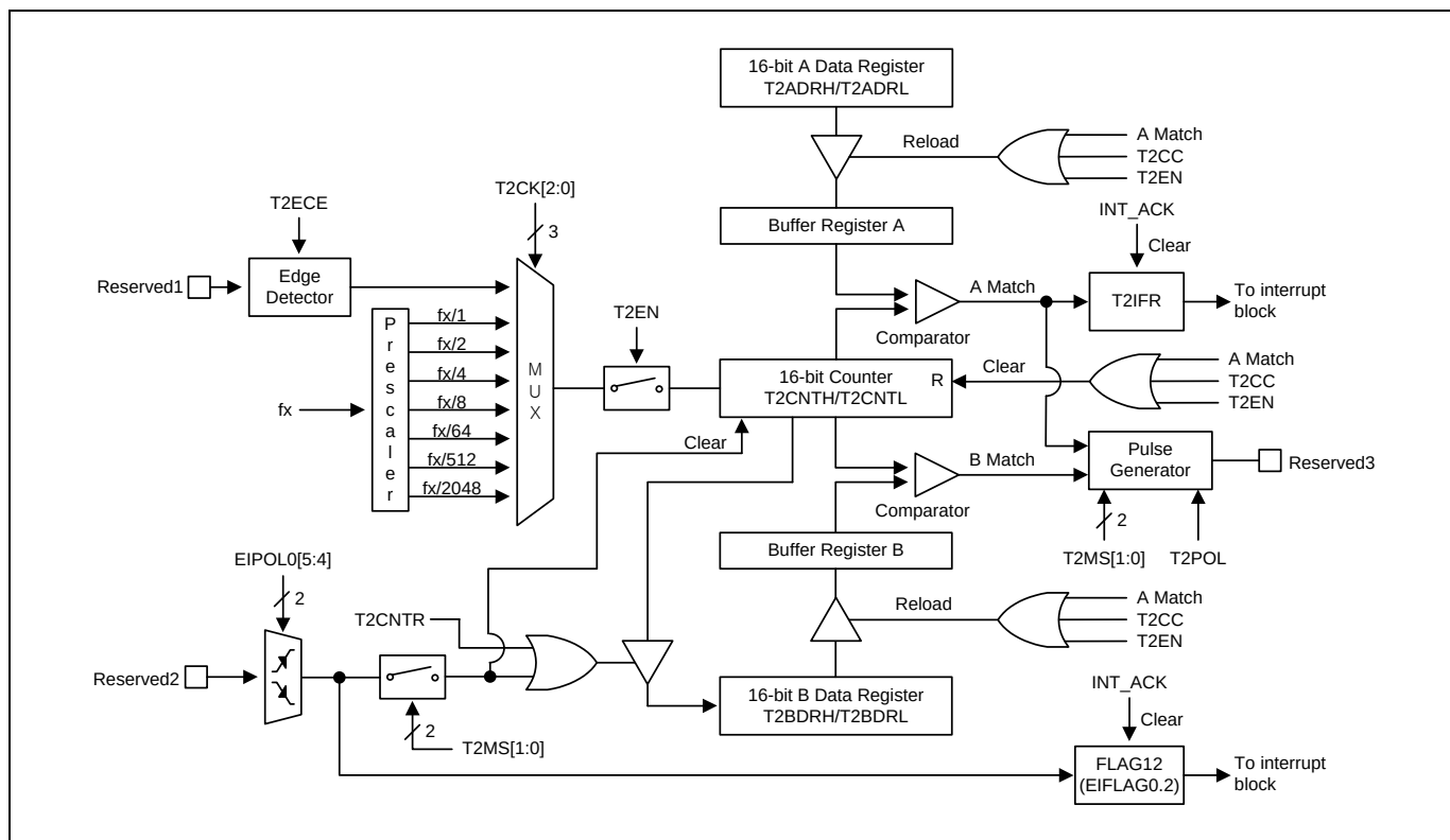
Figure 11.20 16-bit Timer 2 Block Diagram
