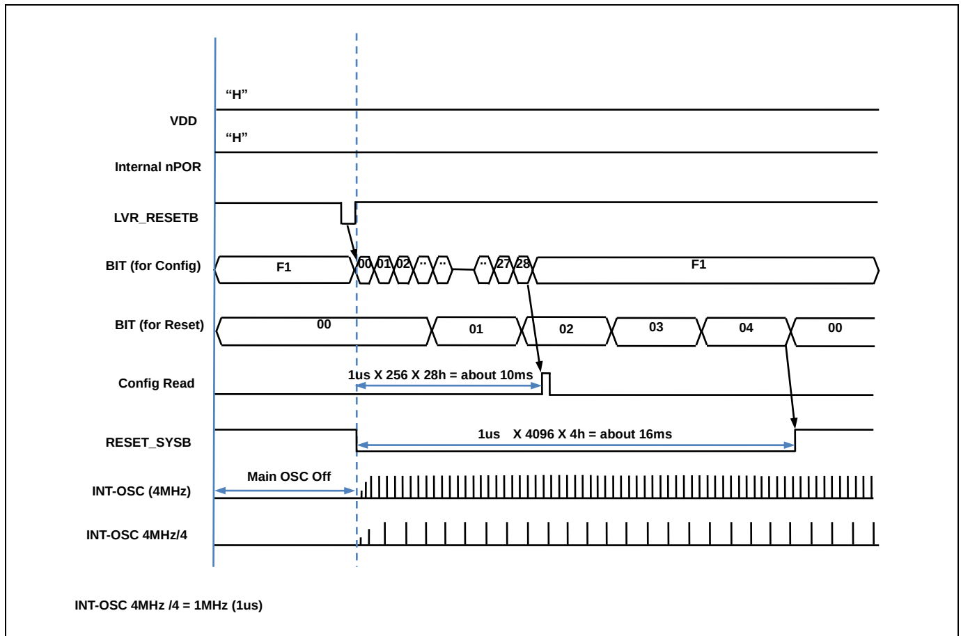
Figure 13.9 Configuration timing when BOD RESET
