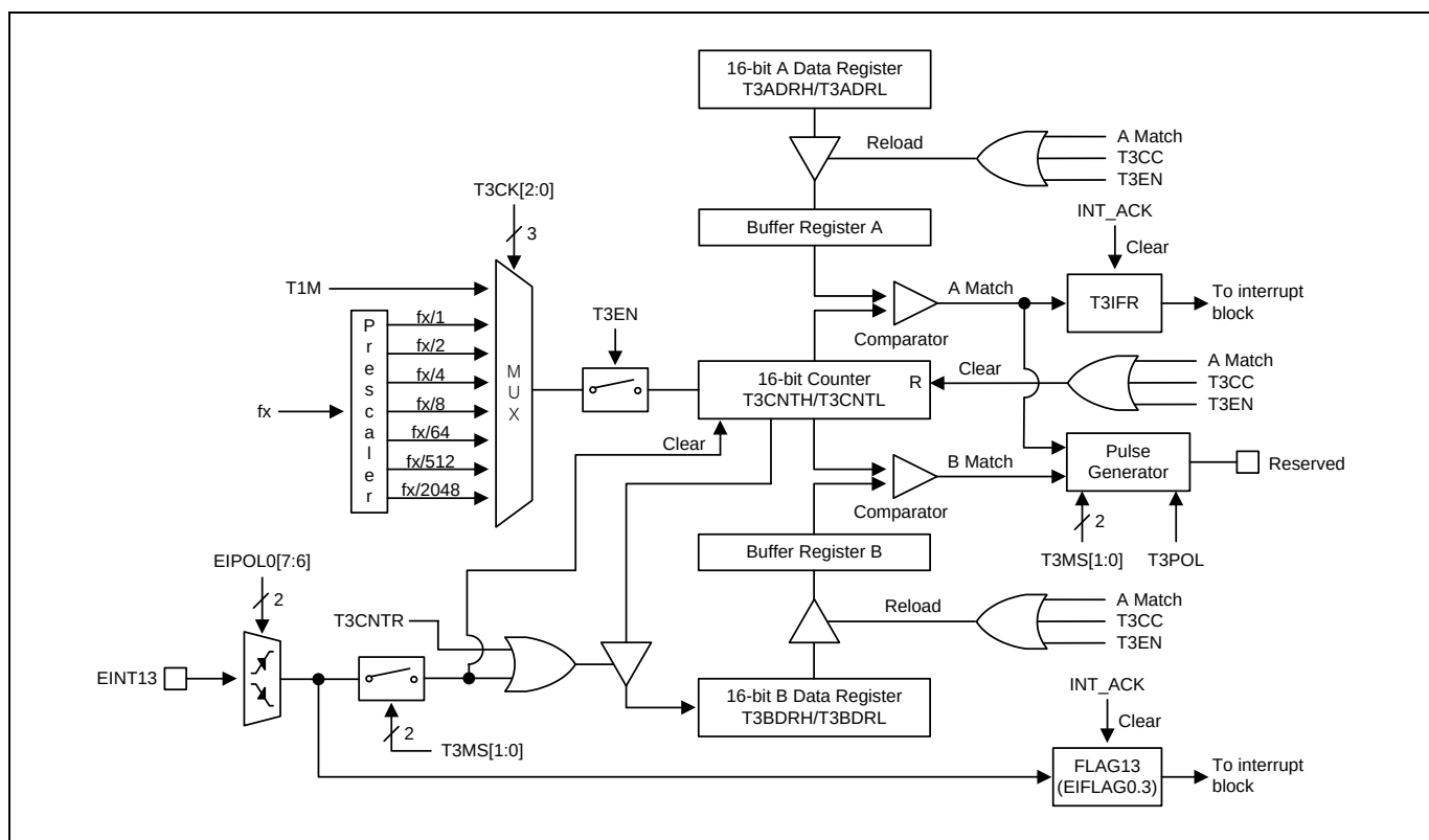
Figure 11.26 16-bit Timer 3 Block Diagram
