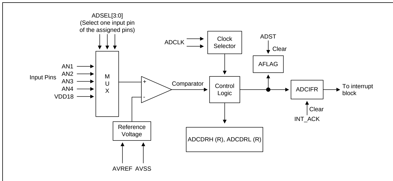
Figure 11.28 12-bit ADC Block Diagram
