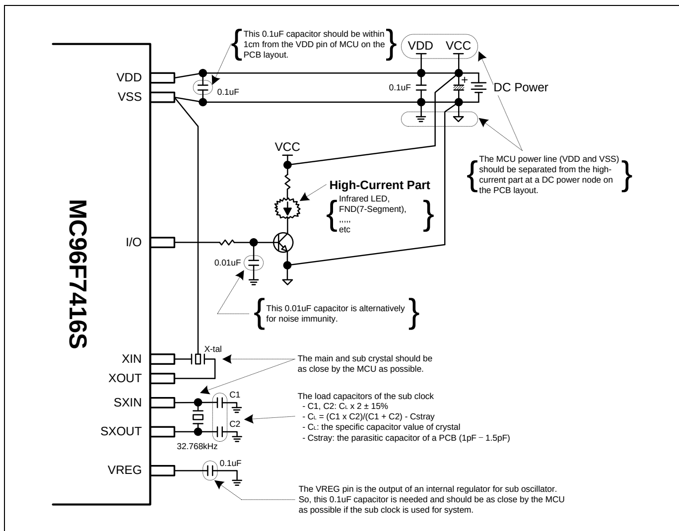
Figure 7.11 Recommended Circuit and Layout
