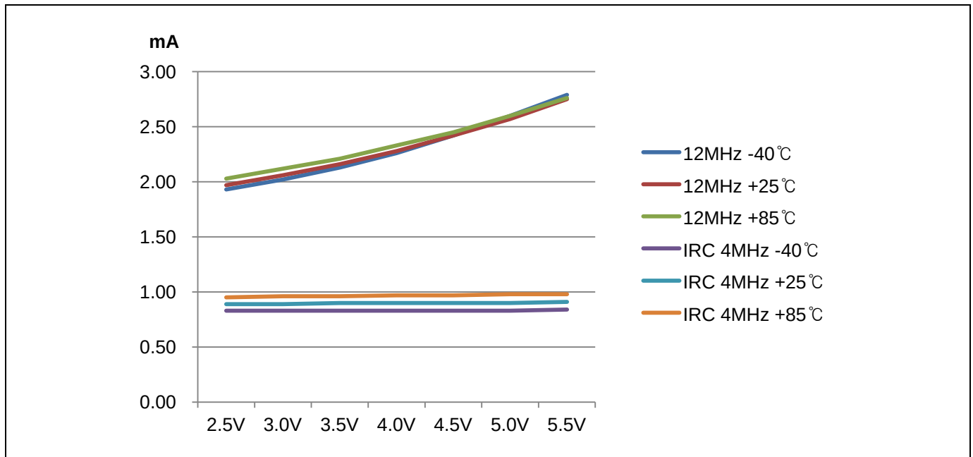
Figure 7.12 RUN (IDD1) Current
