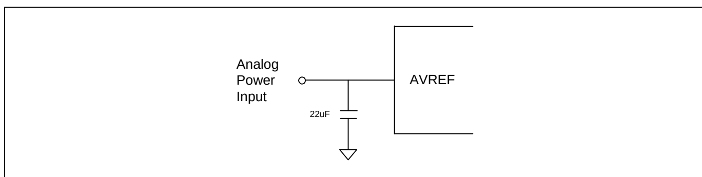
Figure 11.30 A/D Power (AVREF) Pin with Capacitor
