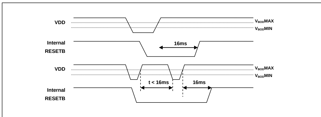
Figure 13.8 Internal Reset at the power fail situation
