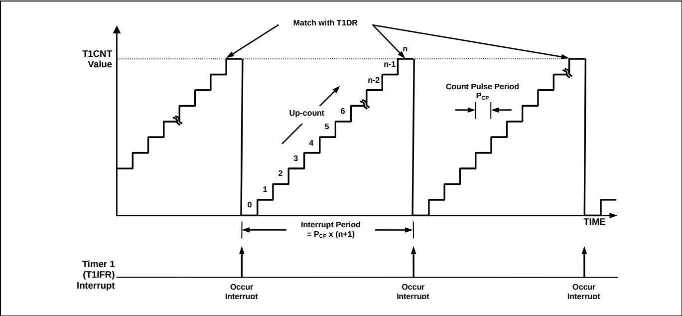
Figure 11.13 8-bit Timer/Counter 1 Example
