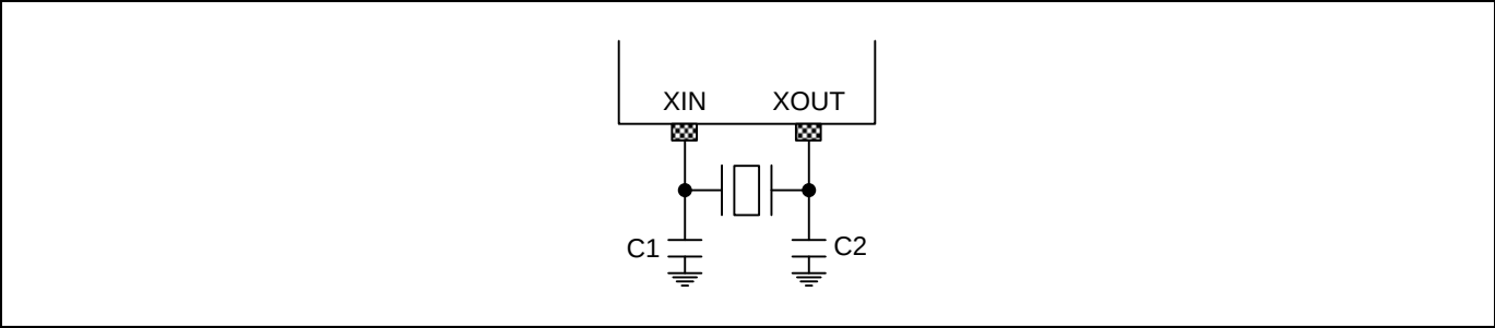
Figure 7.3 Crystal/Ceramic Oscillator
