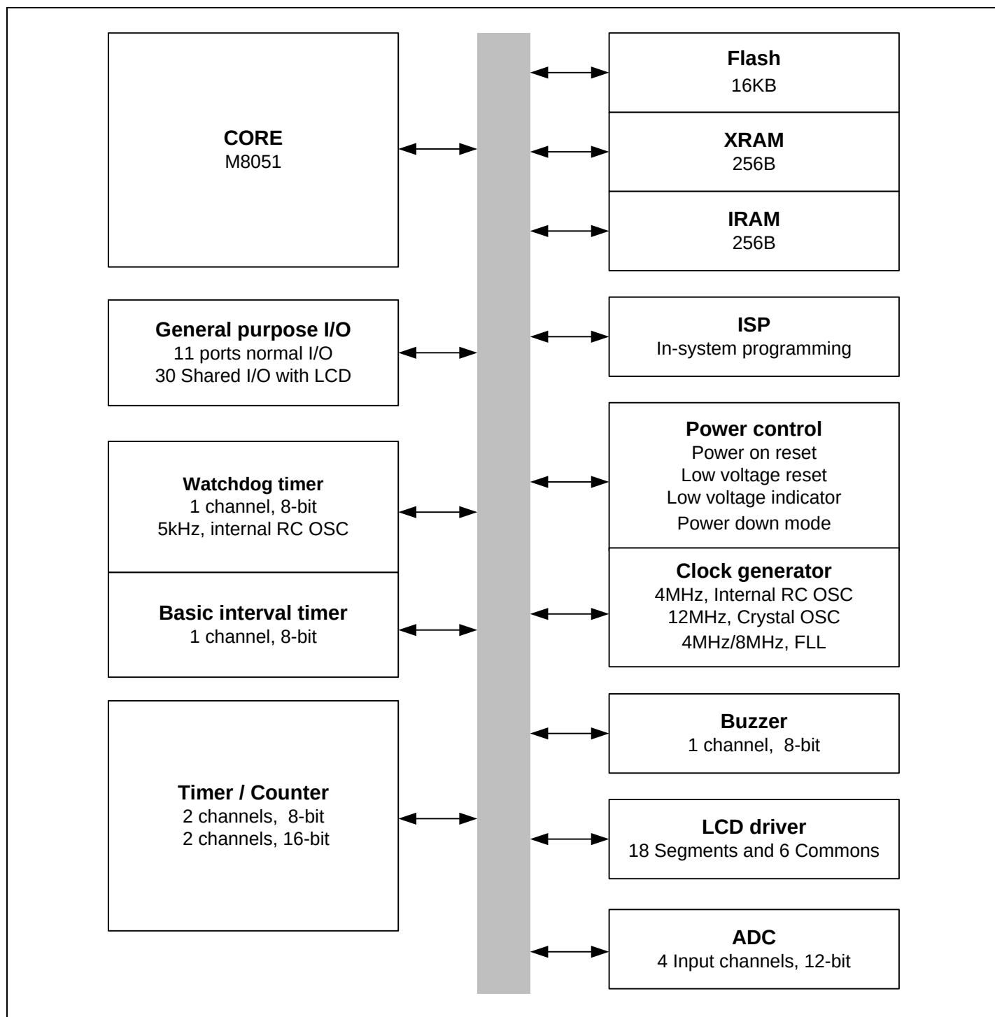
Figure 2.1 Block diagram of MC96F7416S
