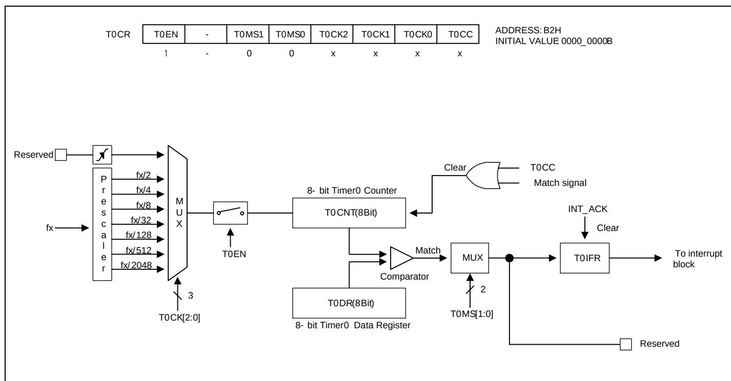
Figure 11.7 8-bit Timer/Counter Mode for Timer 0
