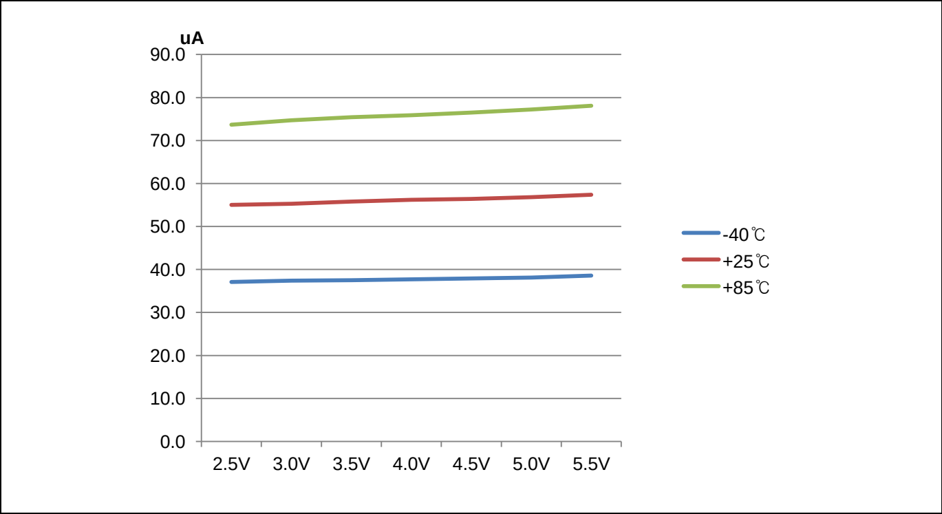
Figure 7.14 SUB RUN (IDD3) Current
