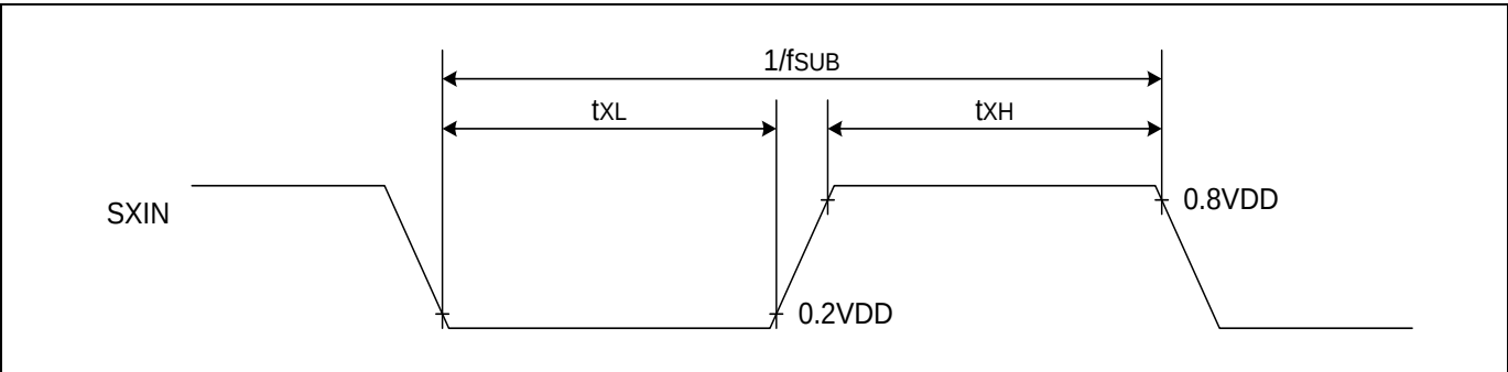
Figure 7.8 Clock Timing Measurement at SXIN
