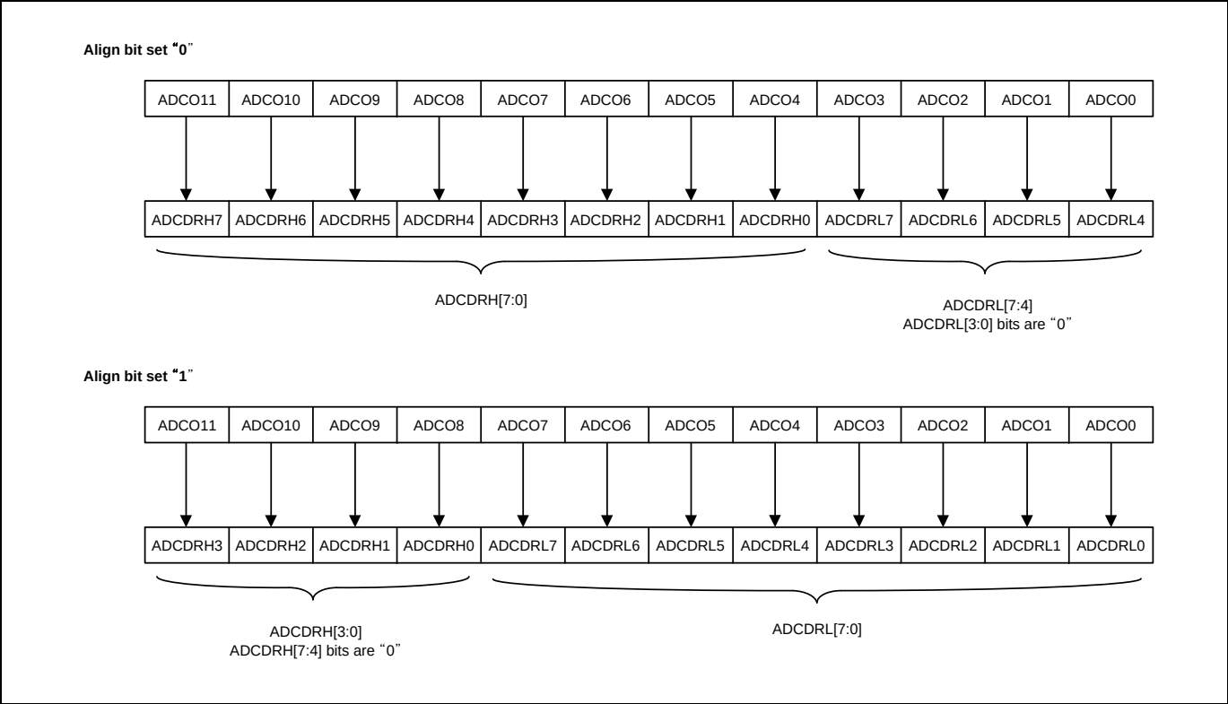
Figure 11.31 ADC Operation for Align Bit
