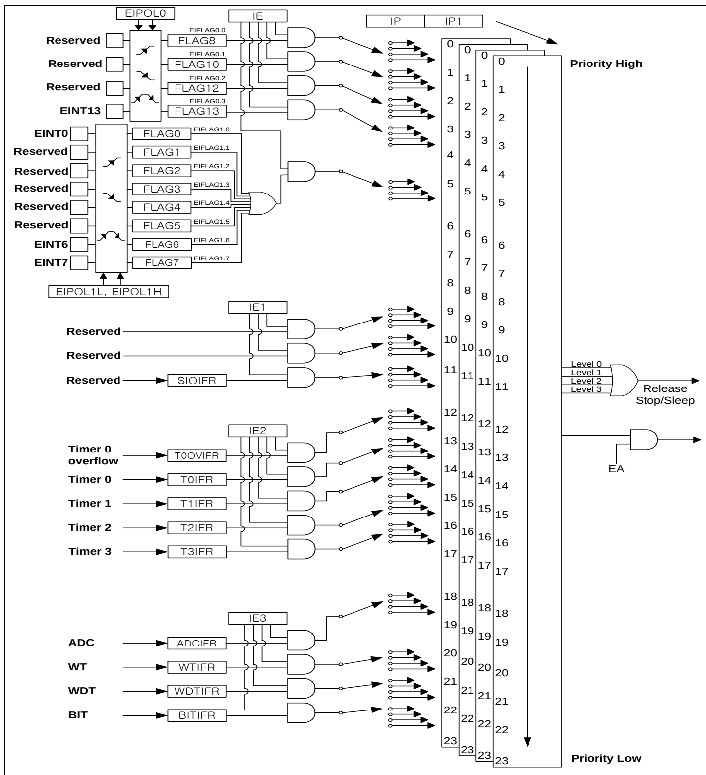
Figure 10.2 Block Diagram of Interrupt
