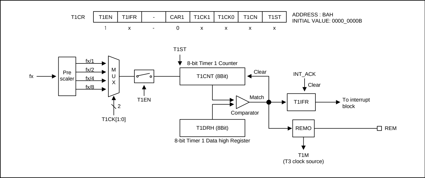
Figure 11.12 8-bit Timer/Counter Mode for Timer 1
