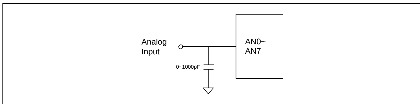
Figure 11.29 A/D Analog Input Pin with Capacitor
