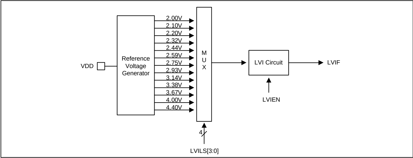
Figure 13.10 LVI Diagram
