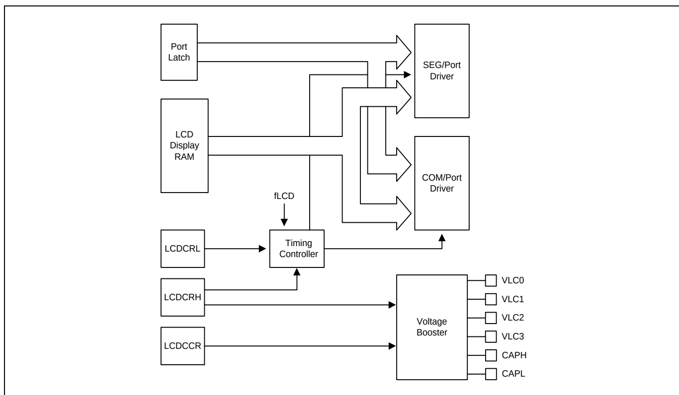
Figure 11.42 Capacitor Bias Connection
