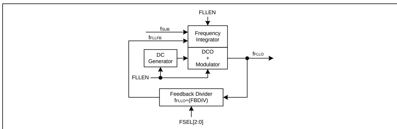
Figure 11.2 Frequency Locked-Loop Block Diagram
