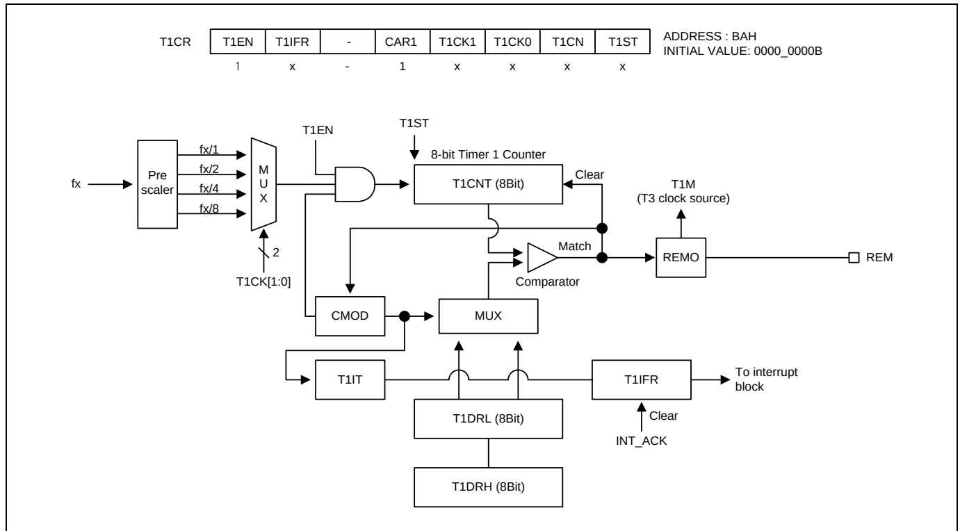
Figure 11.15 Carrier Mode for Timer 1
