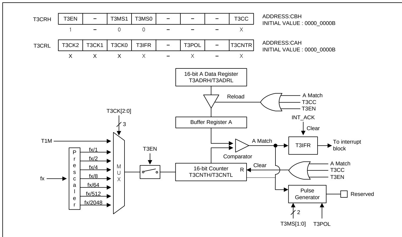
Figure 11.21 16-bit Timer/Counter Mode for Timer 3
