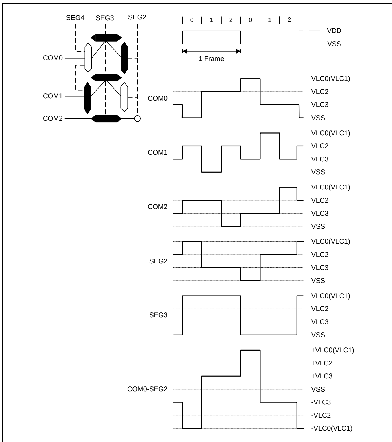
Figure 11.36 LCD Signal Waveforms (1/3Duty, 1/3Bias)
