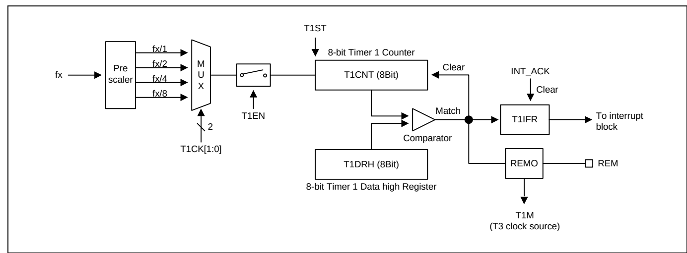
Figure 11.17 8-bit Timer 1 Block Diagram
