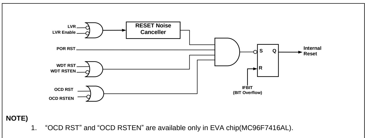
Figure 13.1 RESET Block Diagram
