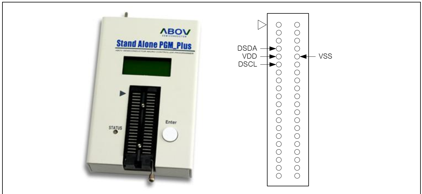
Figure 1.2 Standalone PGMplus(Single writer)
