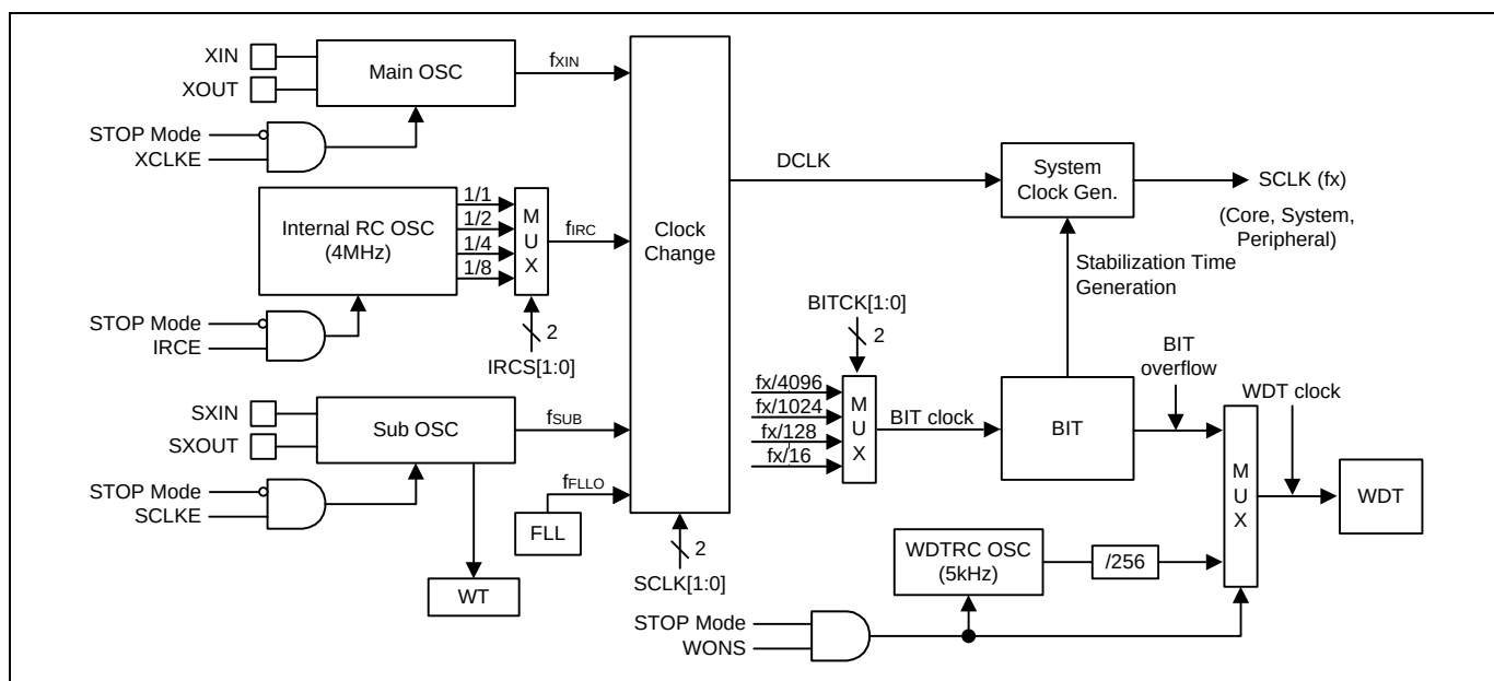
Figure 11.1 Clock Generator Block Diagram
