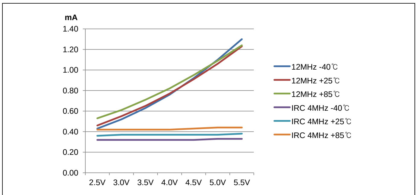
Figure 7.13 IDLE (IDD2) Current
