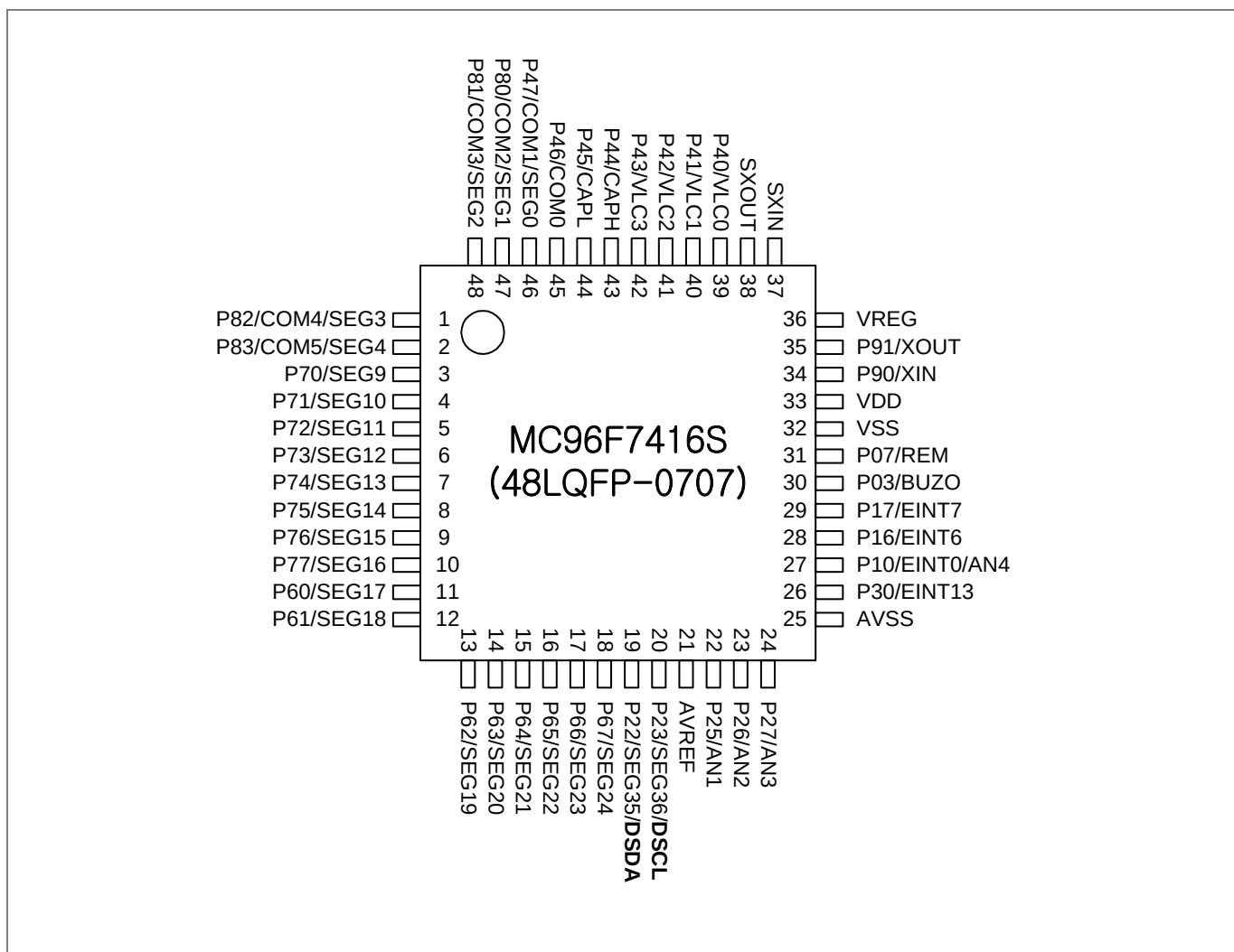
Figure 3.1 MC96F7416S Pin Assignment
