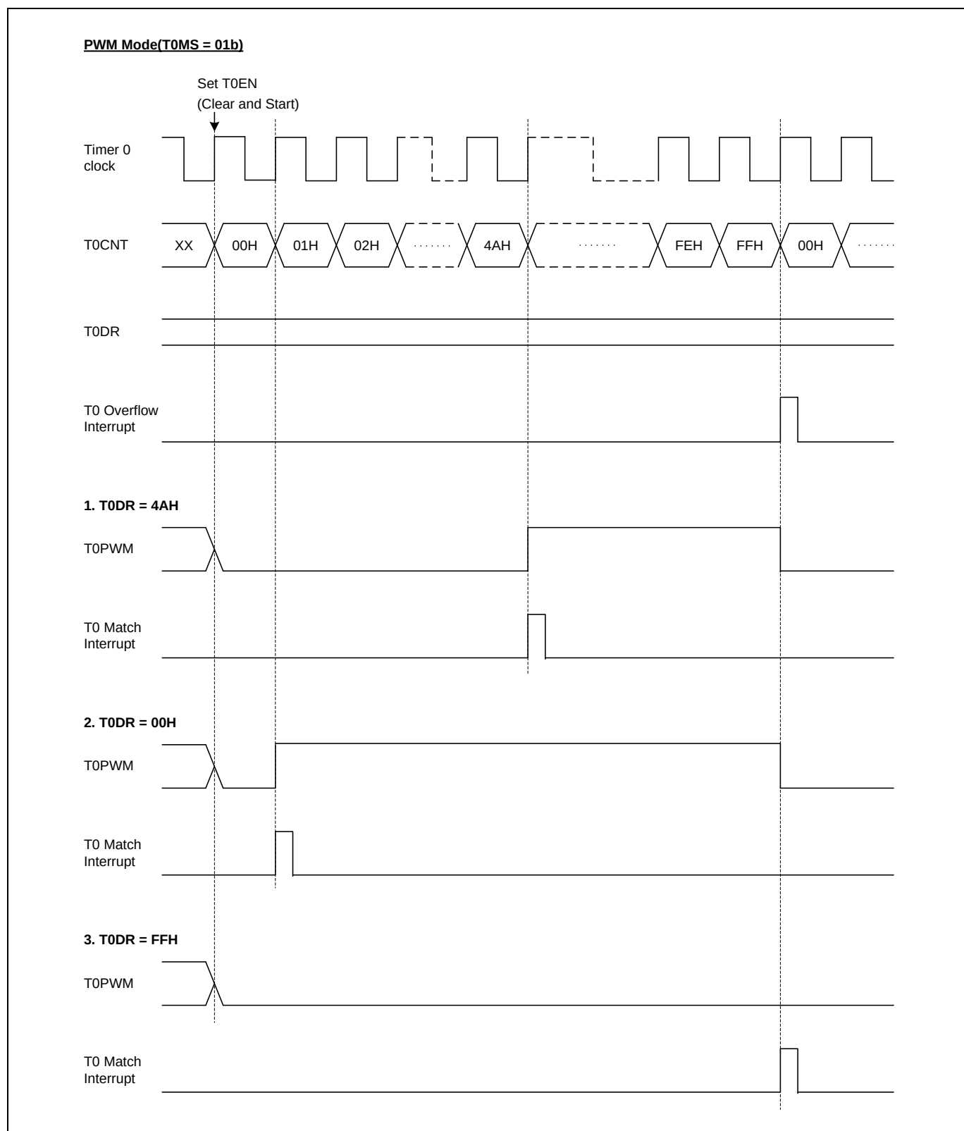
Figure 11.10 PWM Output Waveforms in PWM Mode for Timer 0
