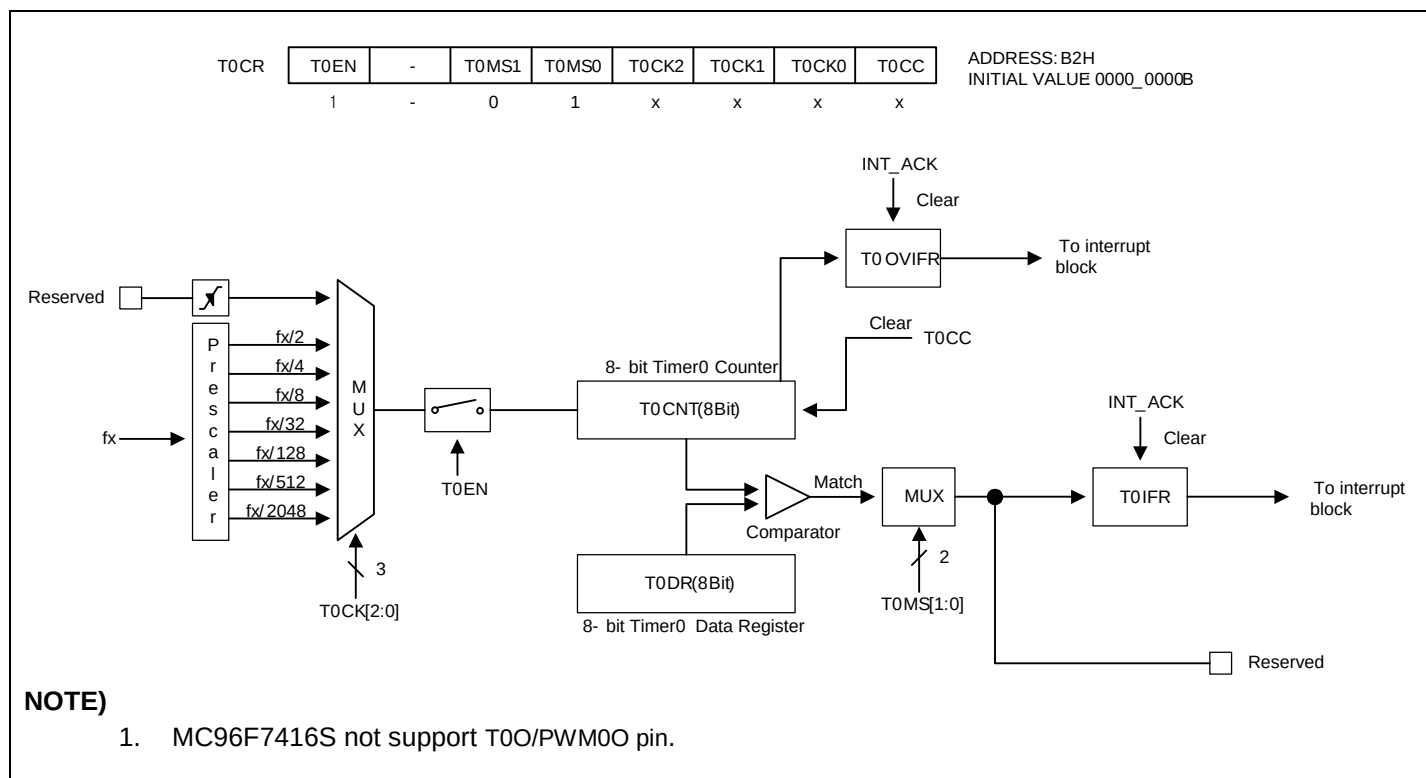
Figure 11.9 8-bit PWM Mode for Timer 0
