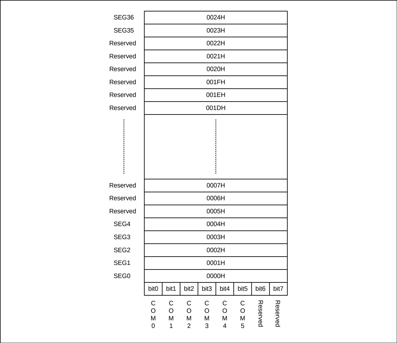
Figure 11.33 LCD Display Data Ram Organization
