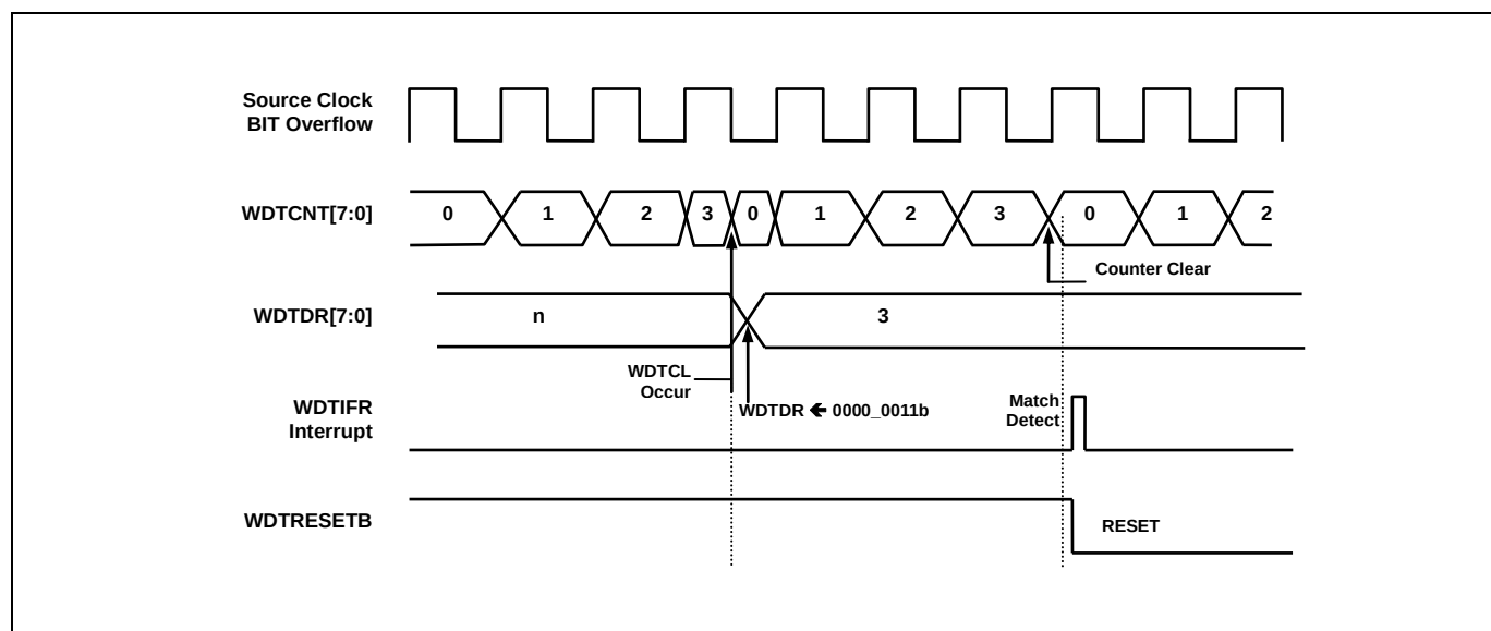
Figure 11.4 Watch Dog Timer Interrupt Timing Waveform
