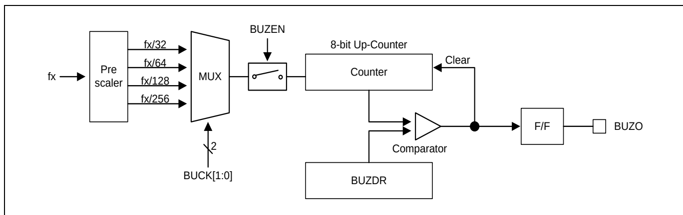
Figure 11.27 Buzzer Driver Block Diagram
