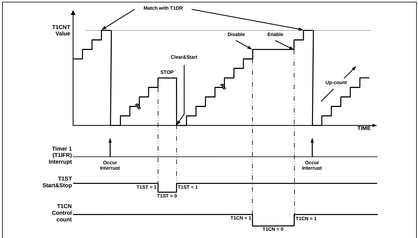
Figure 11.14 8-bit Timer/Counter 1 Counter Operation
