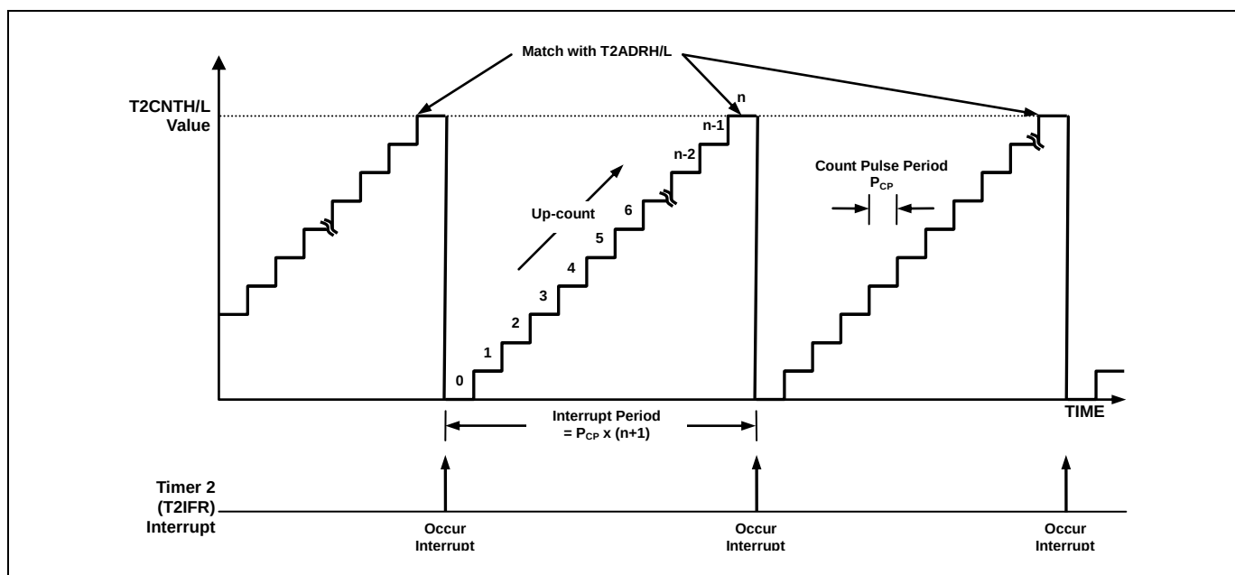
Figure 11.19 16-bit Timer/Counter 2 Example
