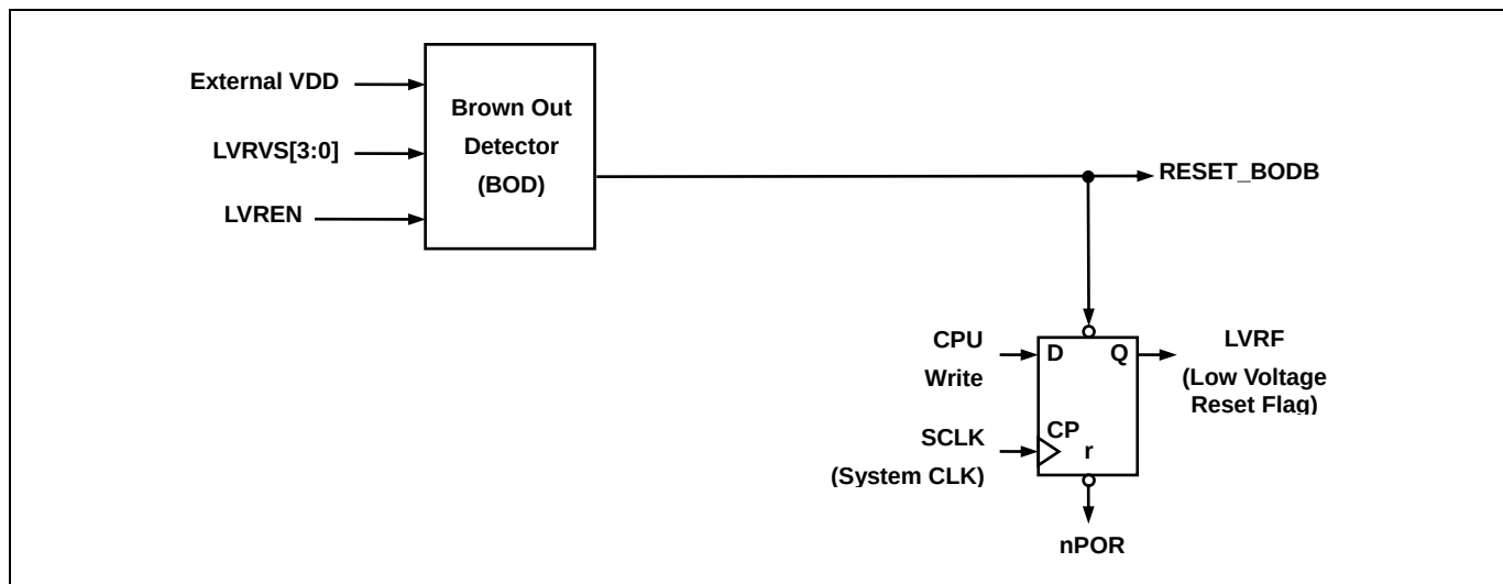
Figure 13.7 Block Diagram of BOD
