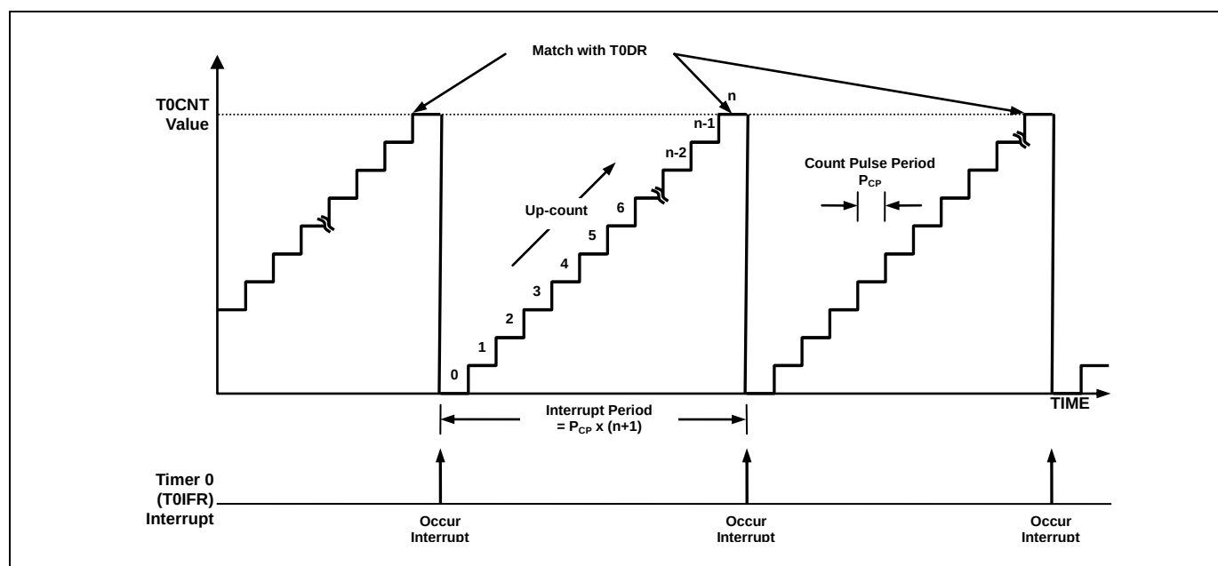
Figure 11.8 8-bit Timer/Counter 0 Example
