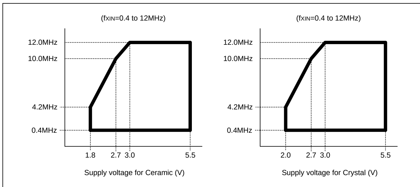
Figure 7.9 Operating Voltage Range (Main OSC)
