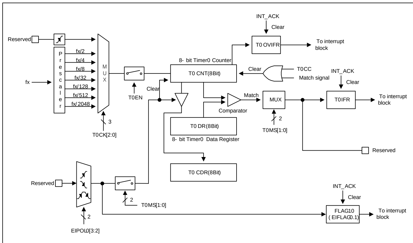
Figure 11.11 8-bit Timer 0 Block Diagram
