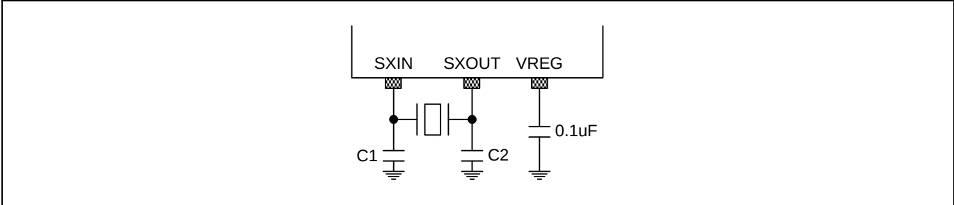
Figure 7.5 Crystal Oscillator
