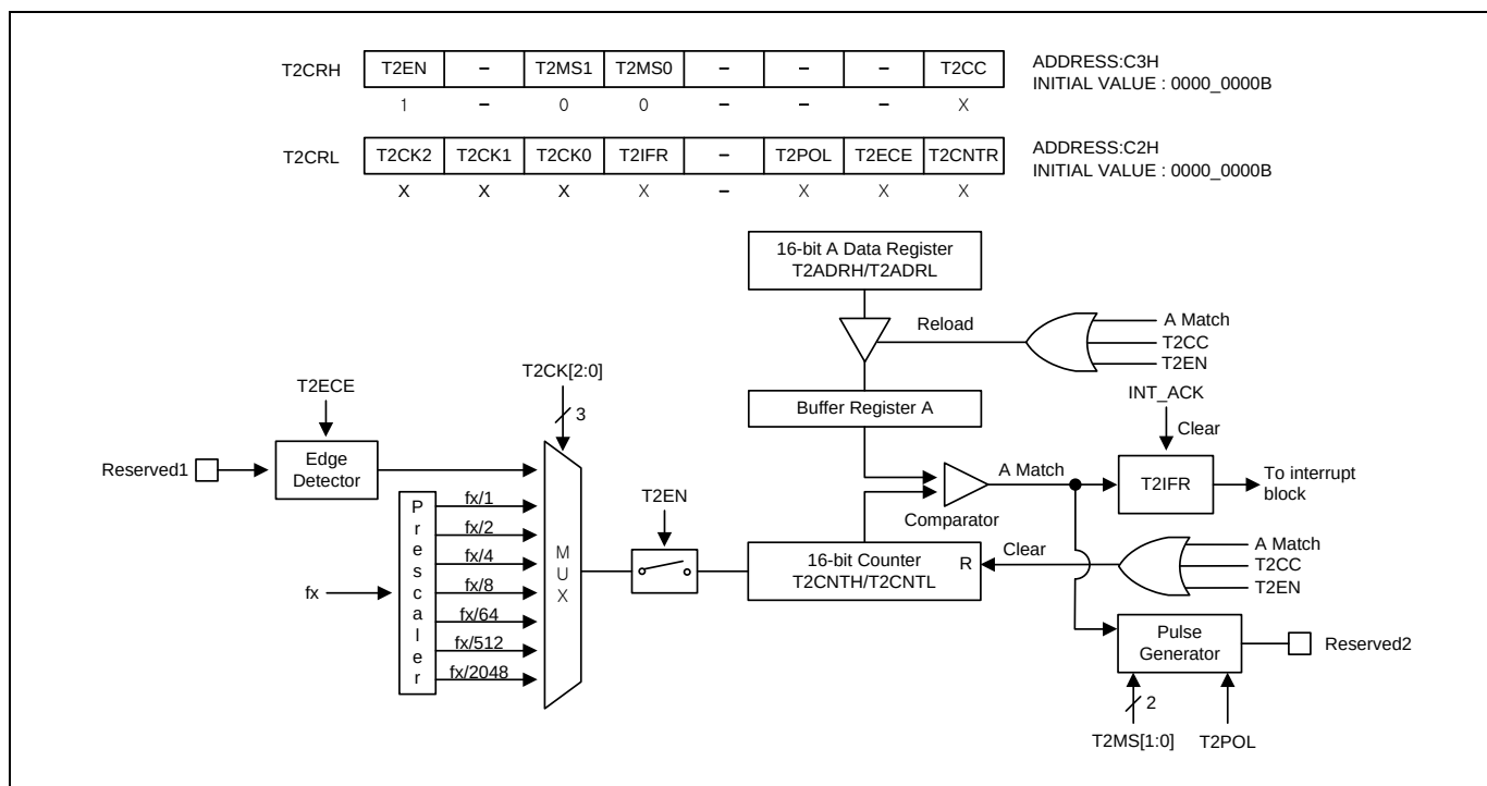
Figure 11.18 16-bit Timer/Counter Mode for Timer 2
