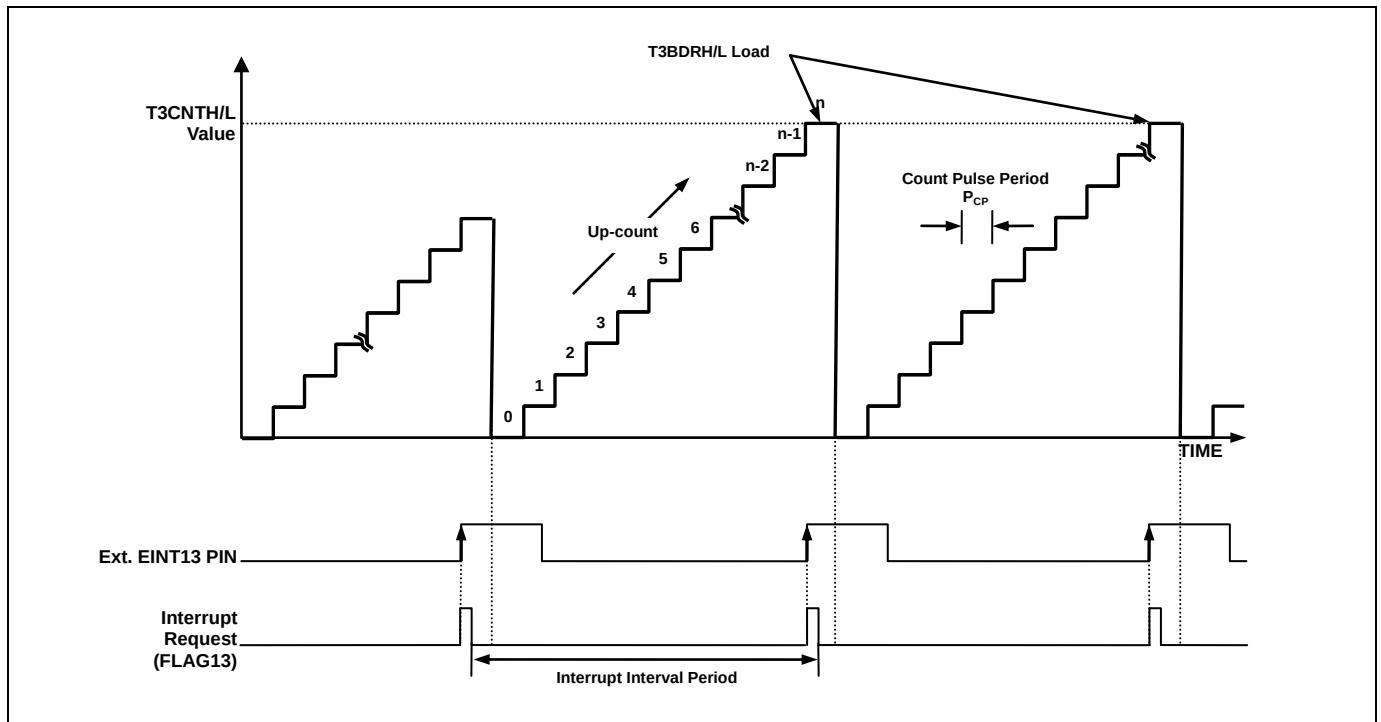
Figure 11.24 Input Capture Mode Operation for Timer 3
