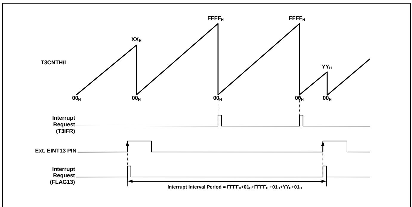
Figure 11.25 Express Timer Overflow in Capture Mode
