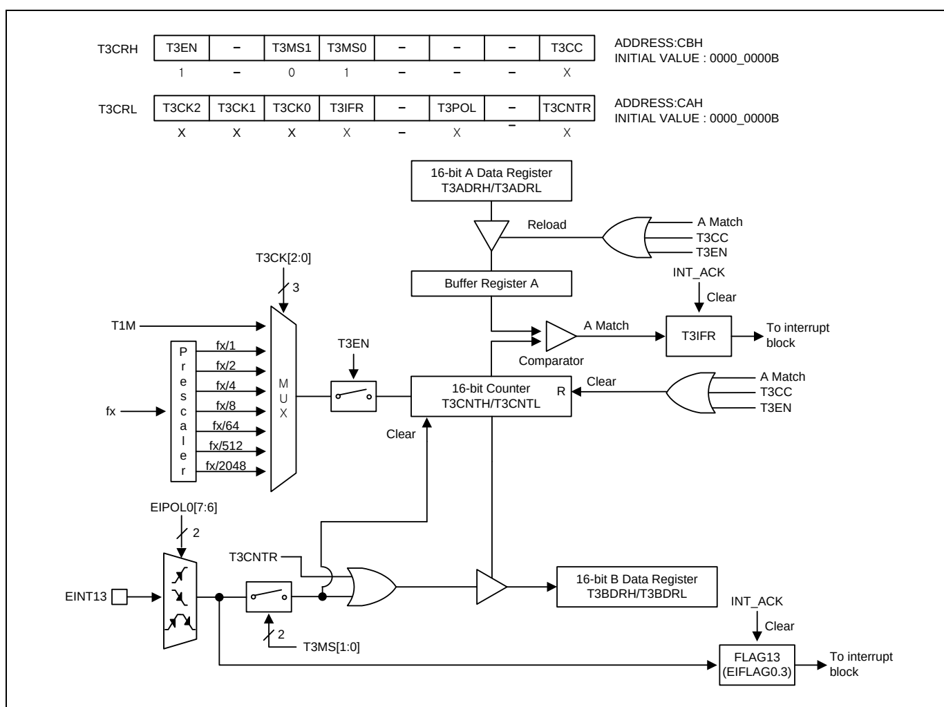
Figure 11.23 16-Bit Capture Mode for Timer 3
