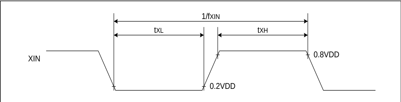
Figure 7.7 Clock Timing Measurement at XIN
