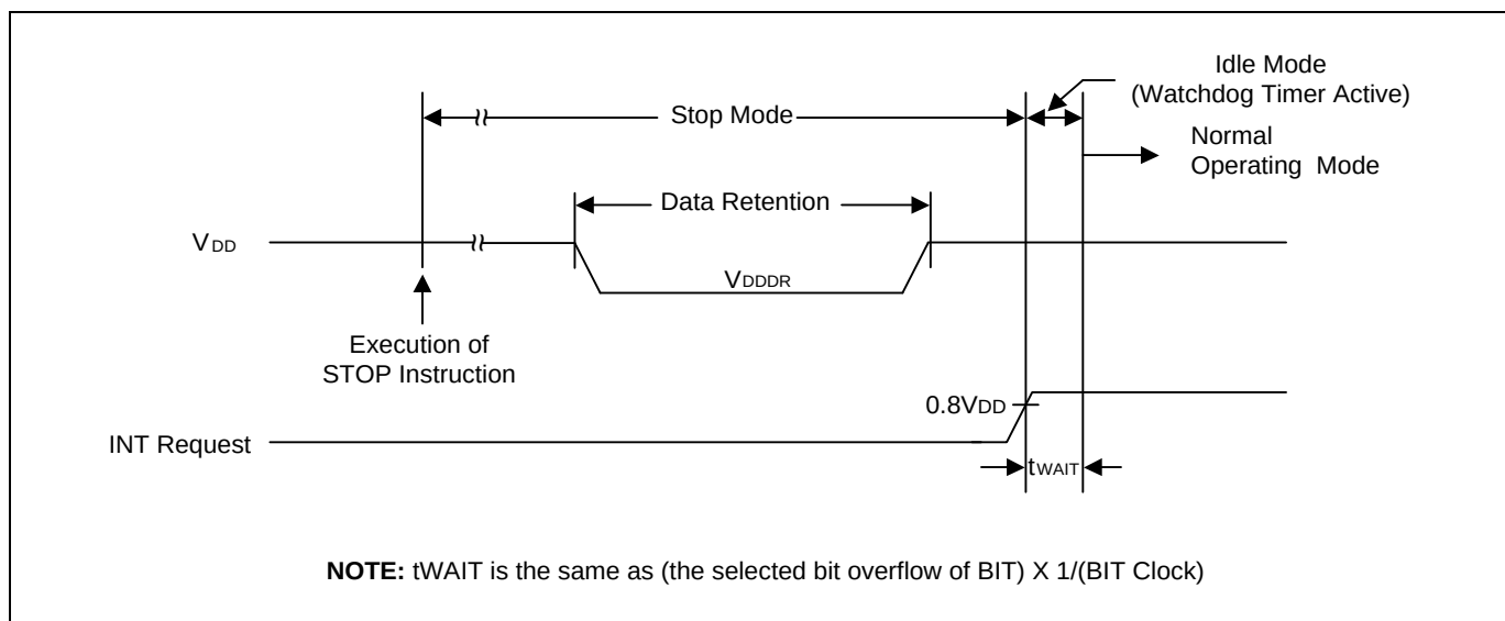
Figure 7.2 Stop Mode Release Timing when Initiated by an Interrupt
