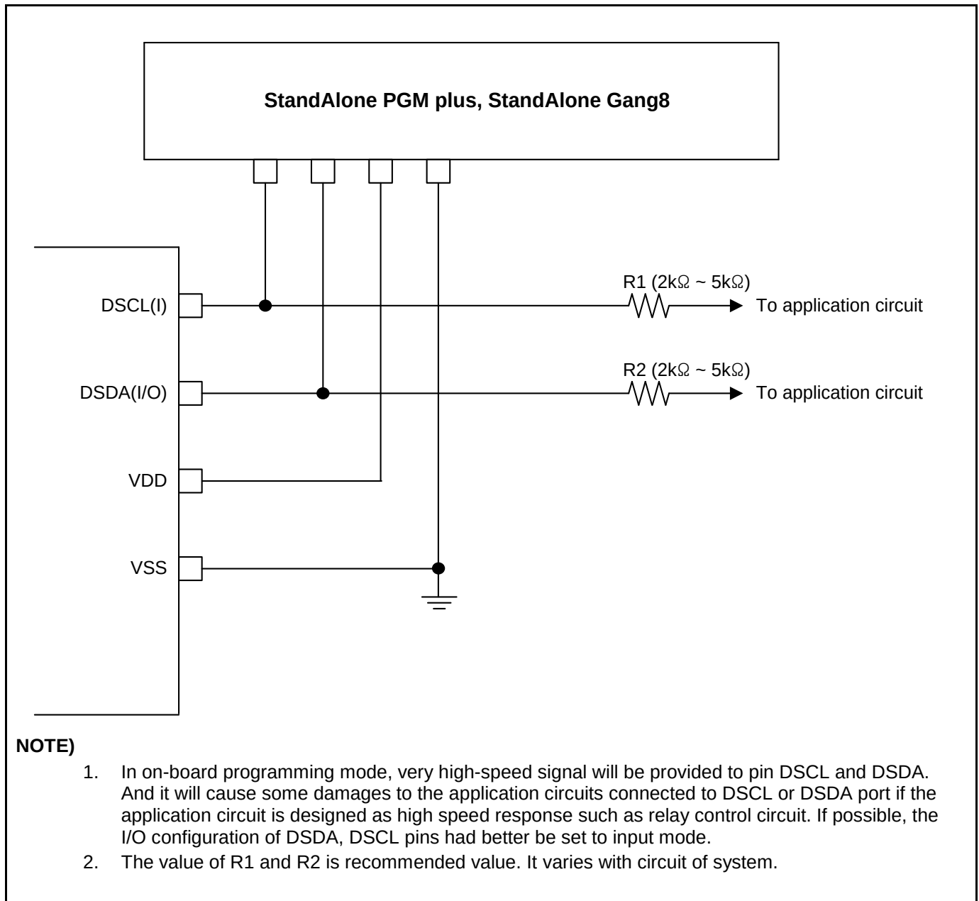
Figure 1.4 PCB design guide for on board programming
