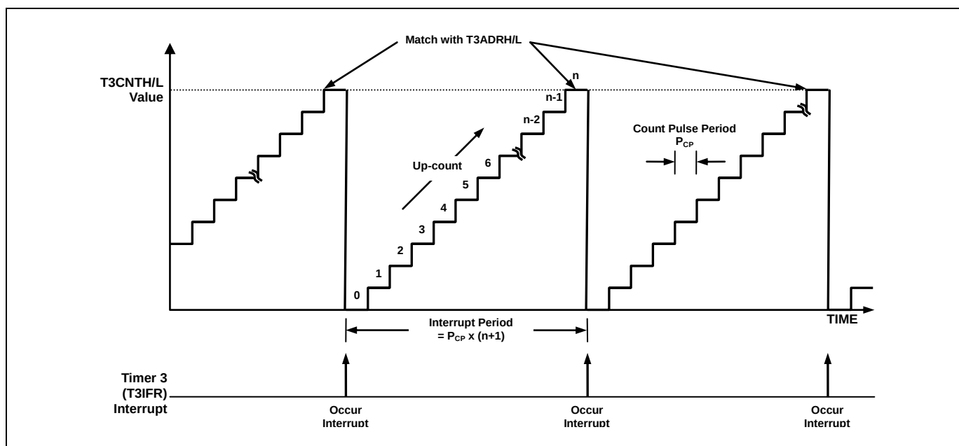
Figure 11.22 16-bit Timer/Counter 3 Example
