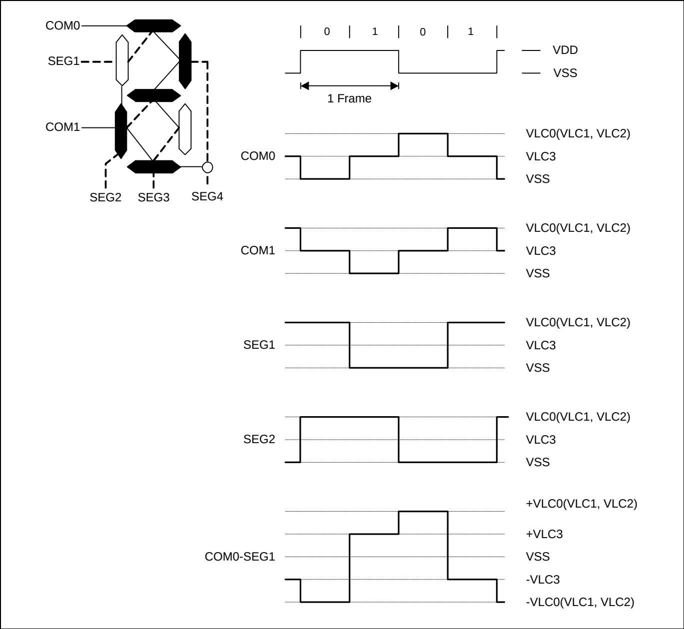
Figure 11.35 LCD Signal Waveforms (1/2Duty, 1/2Bias)
