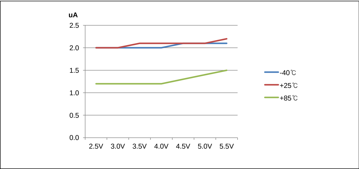
Figure 7.15 SUB IDLE (IDD4) Current
