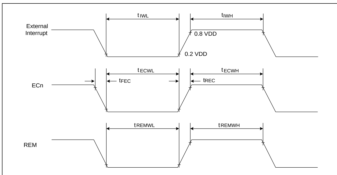
Figure 7.1 AC Timing
