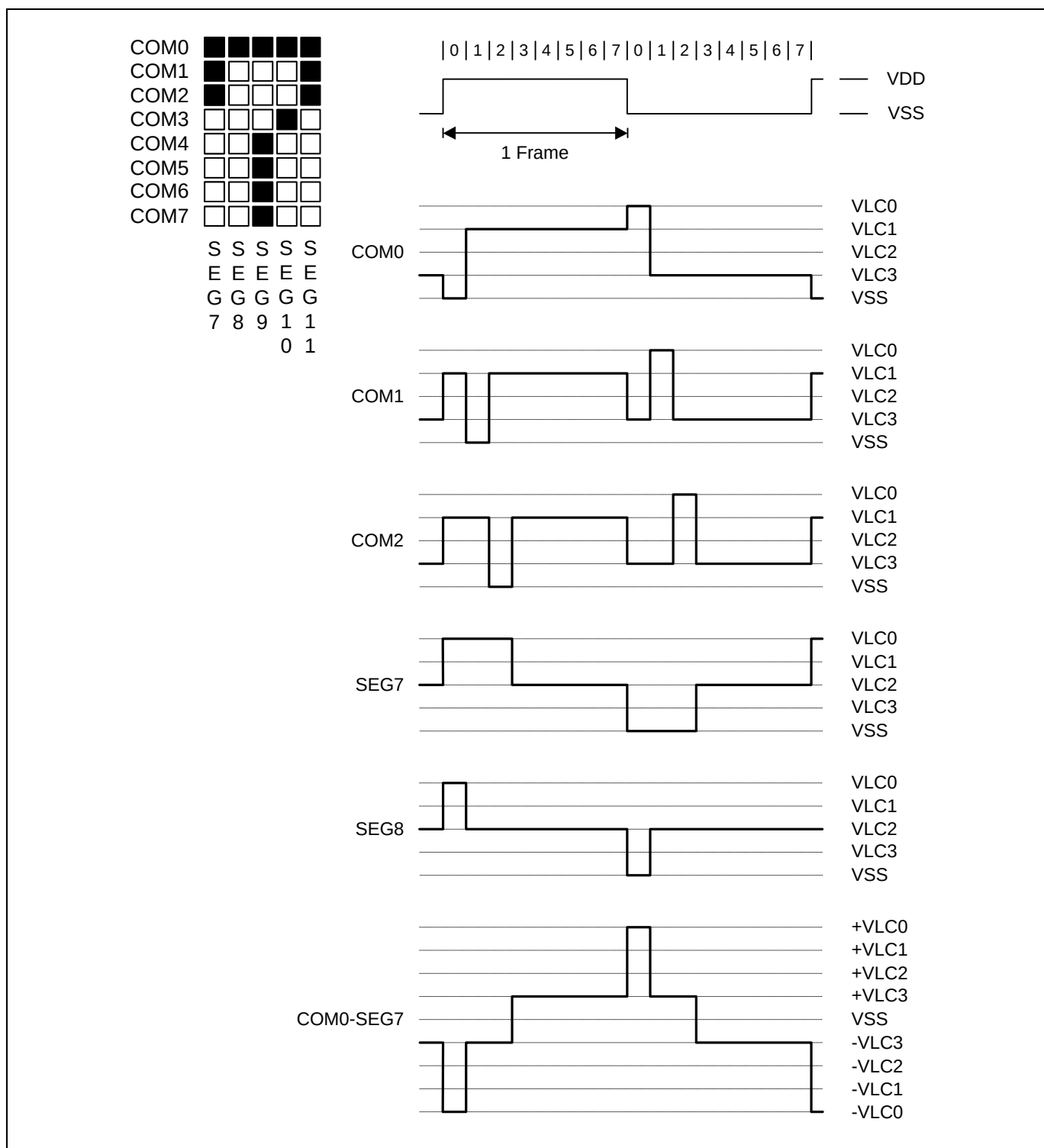
Figure 11.38 LCD Signal Waveforms (1/8Duty, 1/4Bias)
