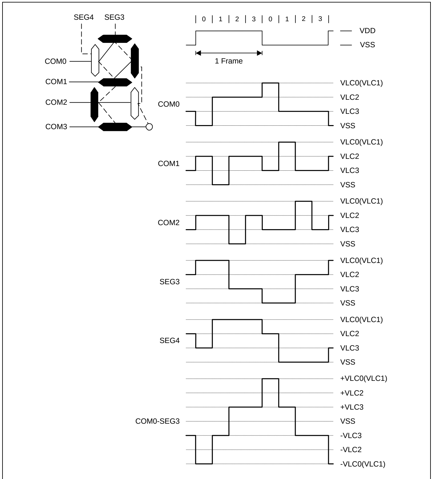
Figure 11.37 LCD Signal Waveforms (1/4Duty, 1/3Bias)
