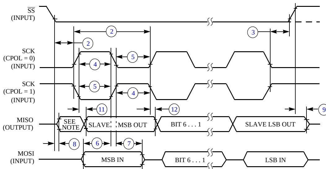
Figure 14. SPI Slave Timing (CPHA = 0)
