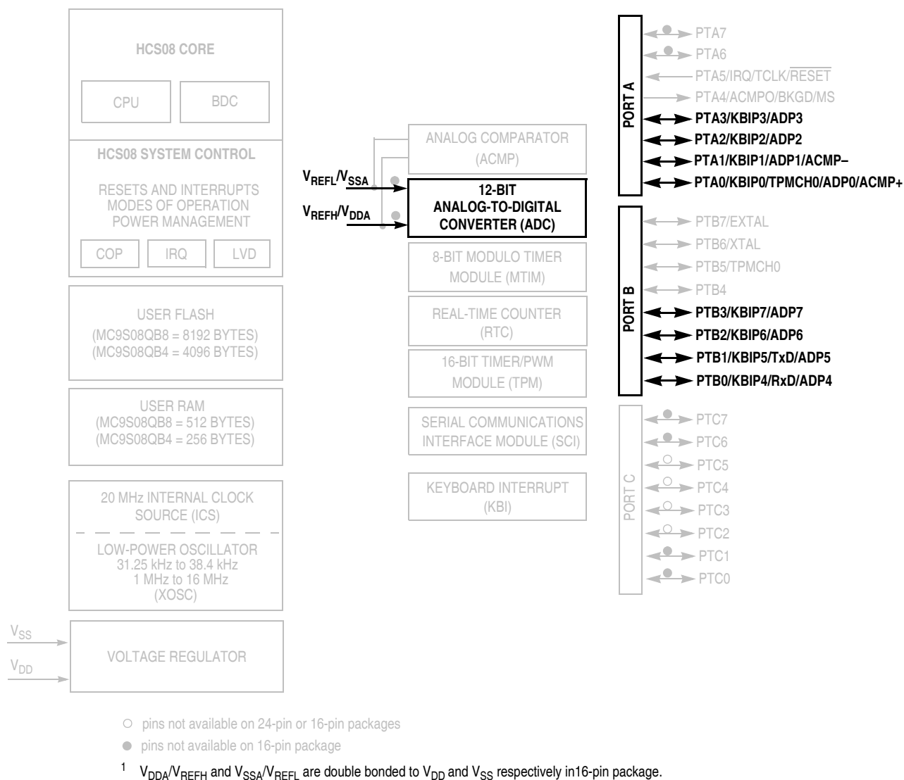
Figure 10-1. MC9S08QB8 Series Block Diagram Highlighting ADC Block and Pins
