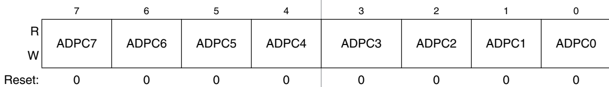
Figure 8-11. Pin Control 1 Register (APCTL1)
