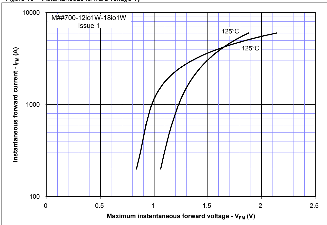
Figure 19 – Instantaneous forward voltage V_F
