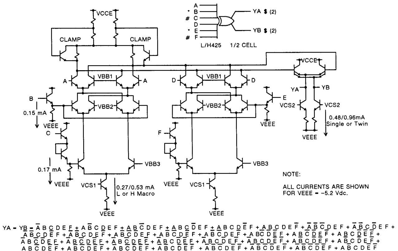
FIGURE 8 — SCHEMATIC OF 6-INPUT EXCLUSIVE OR GATE
