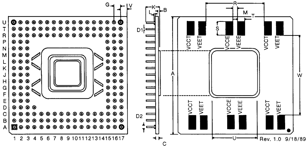
FIGURE 20 — 169 PIN GRID ARRAY PACKAGE
