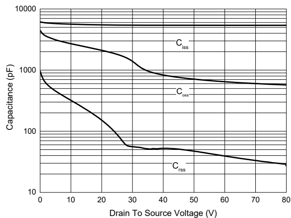
Fig.5 Capacitance Characteristics
