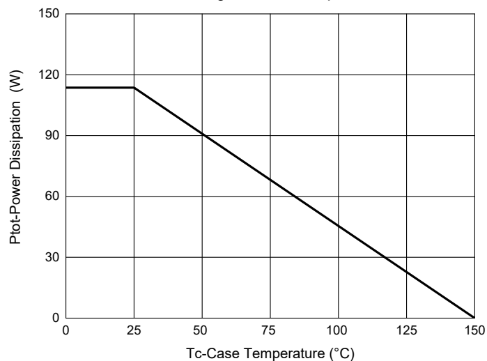
Fig. 11 - PD dissipation
