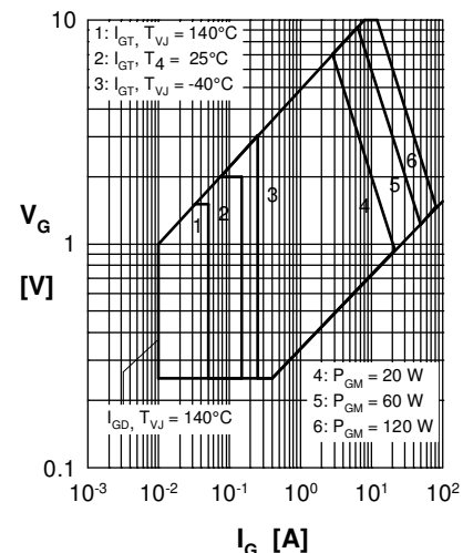
Fig. 5 Gate voltage and current
