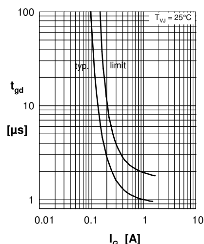
Fig. 7 Gate trigger characteristics
