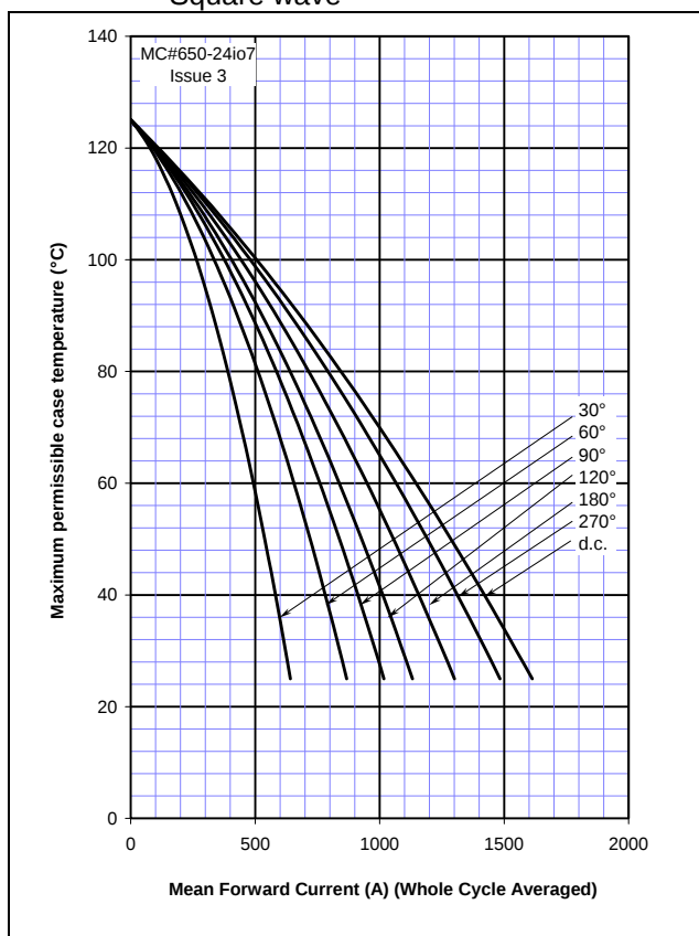
Figure 11 – On-state current vs. case temperature – Square wave
