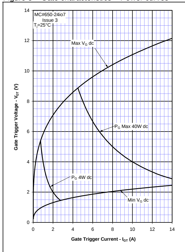
Figure 3 – Gate characteristics – Power curves
