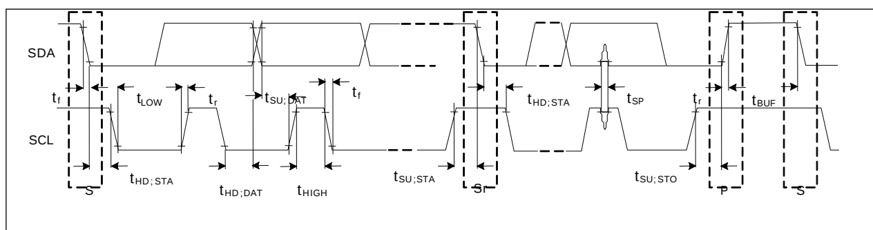
Figure 12. I2C timing
