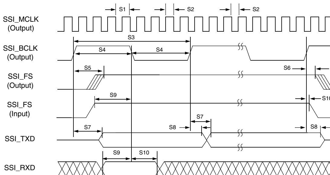
Figure 23. SSI Timing—Master Modes
