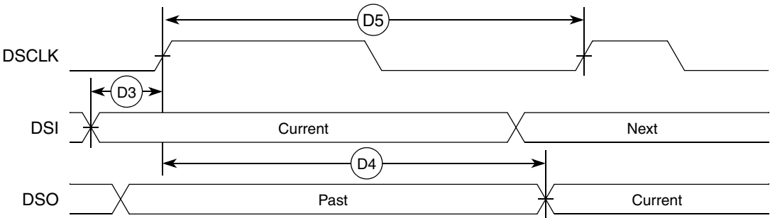
Figure 34. BDM Serial Port AC Timing
