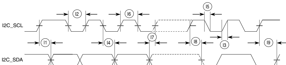
Figure 25. I 2 C Input/Output Timings
