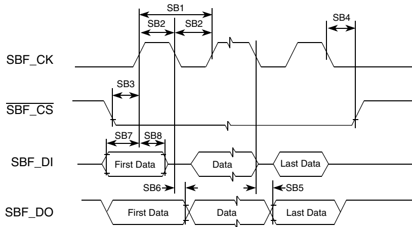
Figure 28. SBF Timing
