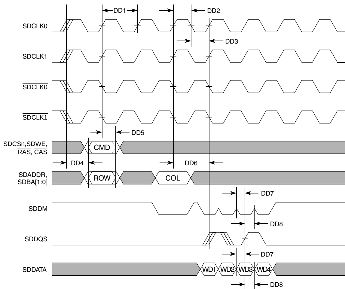
Figure 16. DDR Write Timing
