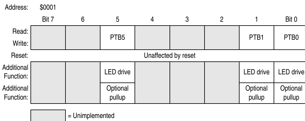
Figure 13-5. Port B Data Register (PTB)
