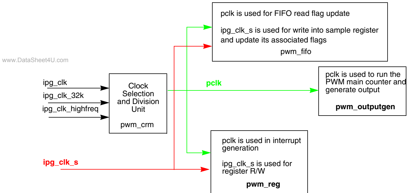
Figure 32-11. Clock Distribution Inside PWM
