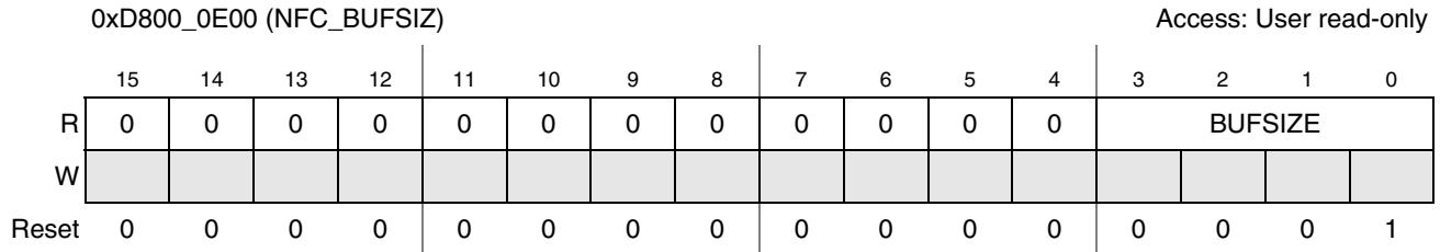
Figure 19-4. NFC_BUFSIZE Register
