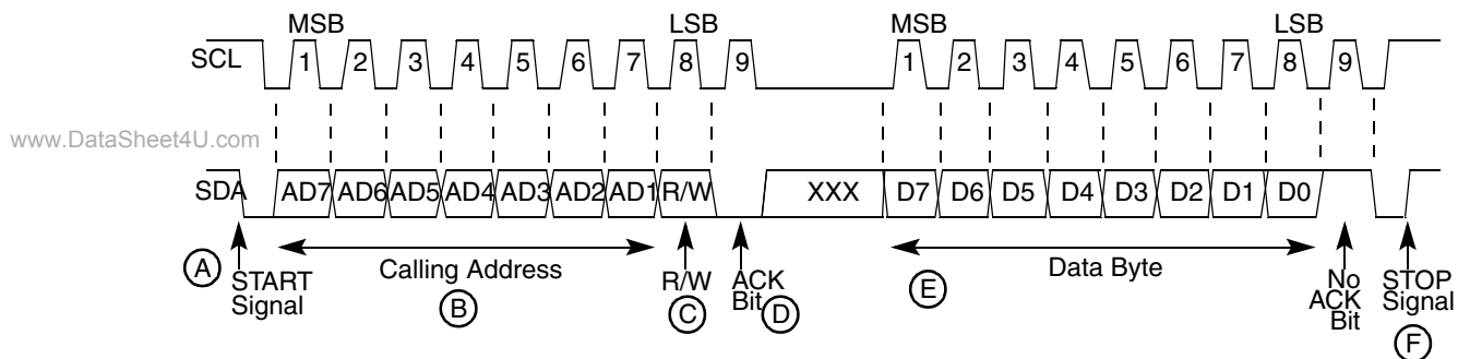
Figure 24-11. I 2 C Standard Communication Protocol
