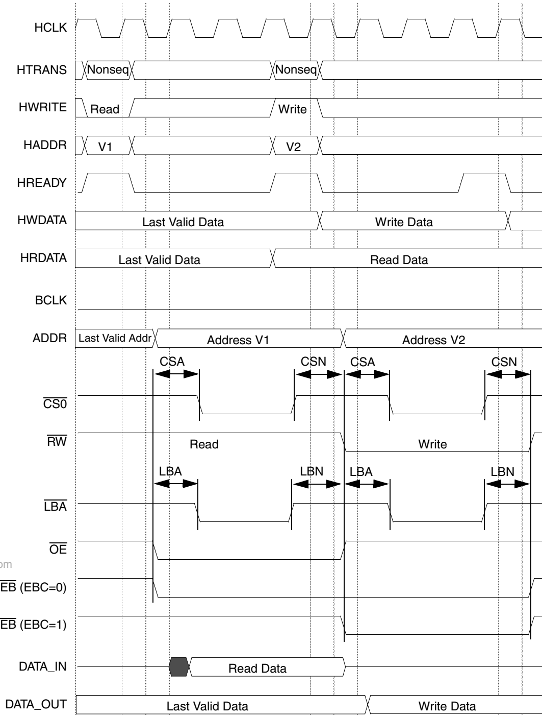
Figure 17-11. Read and Write Accesses, WSC=3, CSA=1, CSN=1, LBA=1, LBN=1
