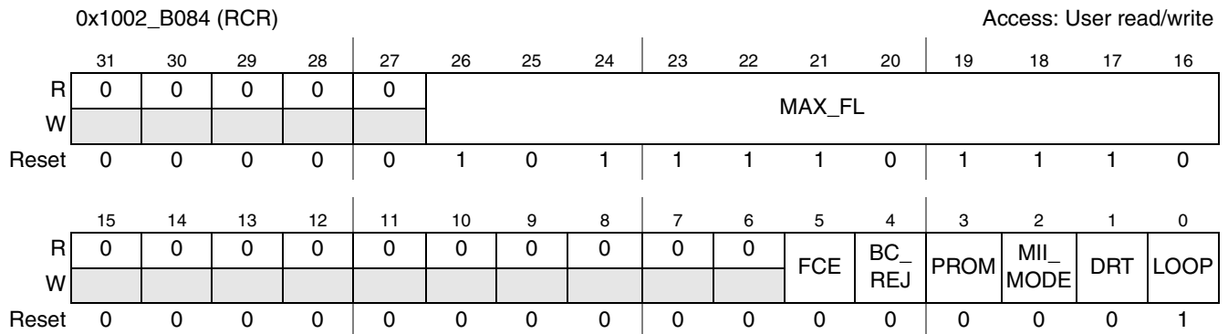
Figure 29-12. RCR Register
