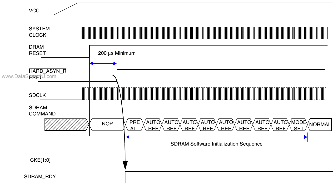
Figure 18-80. SDR SDRAM Initialization and Load Mode Register Sequence
