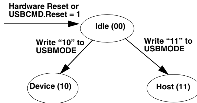
Figure 30-42. Controller Mode
