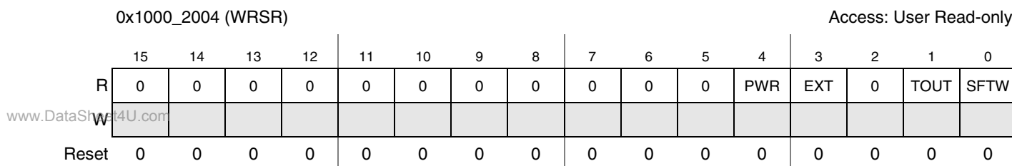
Figure 34-5. Watchdog Reset Status Register (WRSR)
