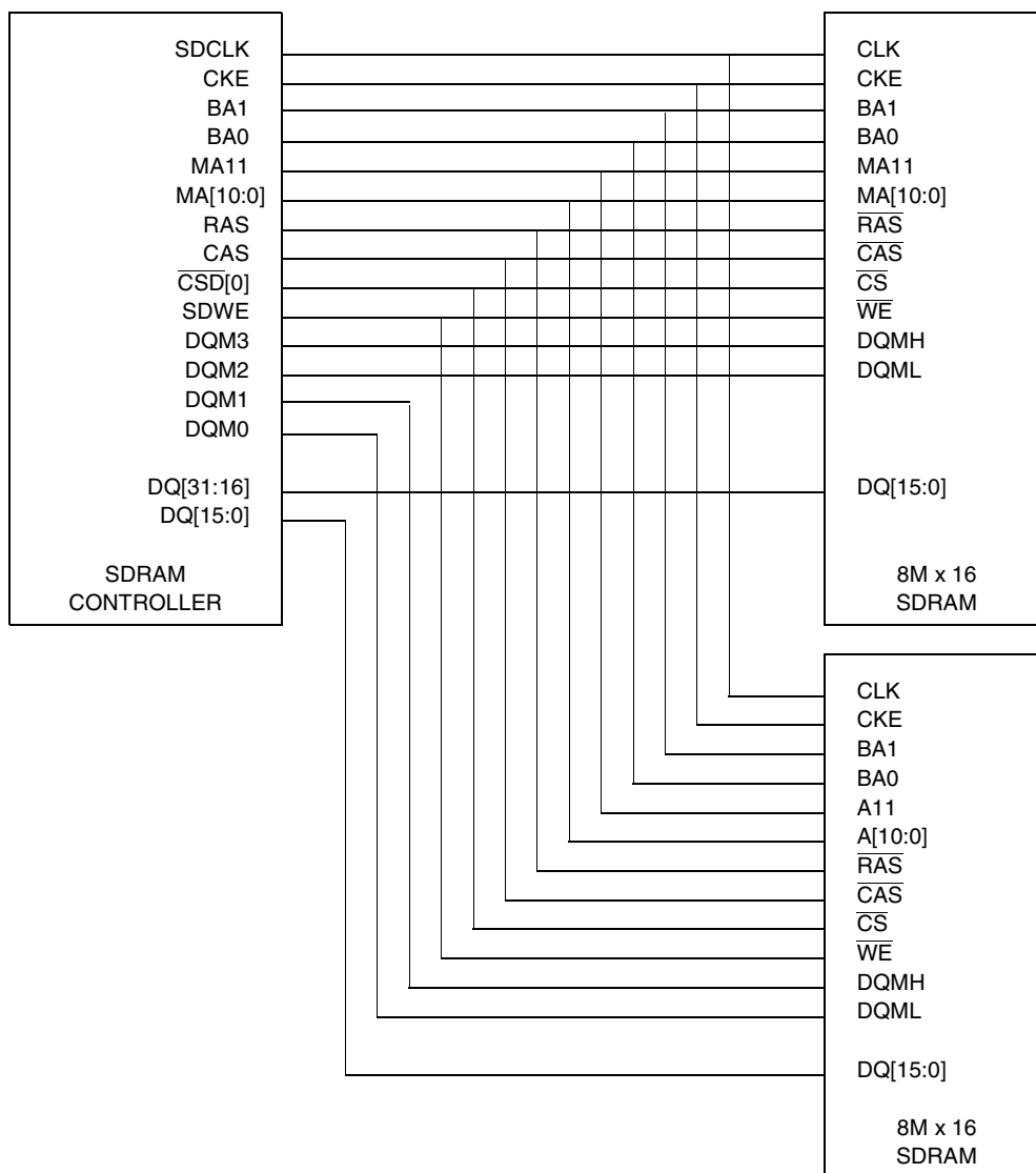
Figure 18-89. Dual 128 Mb (8M x 16 x 2) SDRAM Connection Diagram
