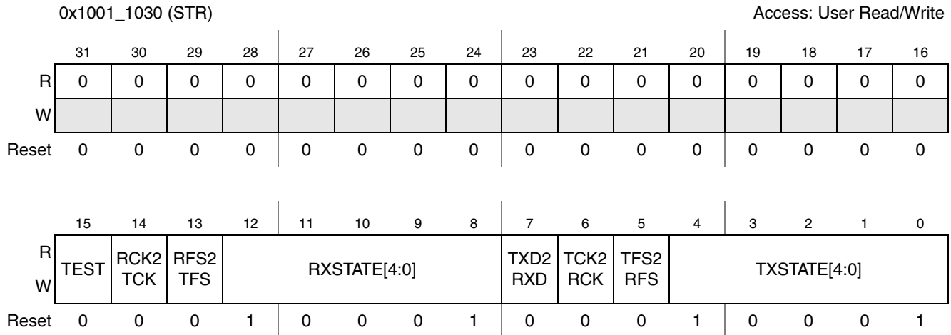
Figure 42-33. SSI Test Register
