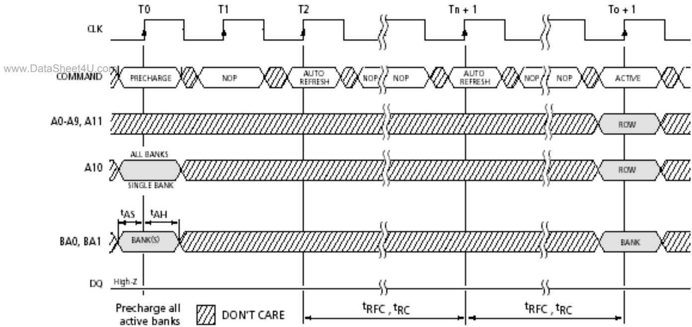
Figure 18-18. t_{RC} —Row Cycle Timing
