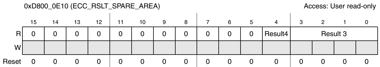
Figure 19-13. ECC_Rslt_Spare_Area Register
