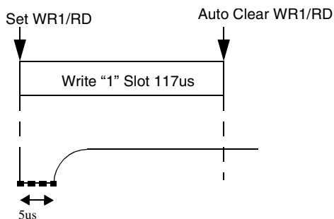
Figure 21-5. Write 1 Timing
