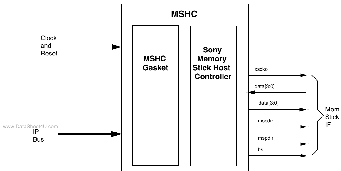
Figure 26-1. Memory Stick Controller Block Diagram
