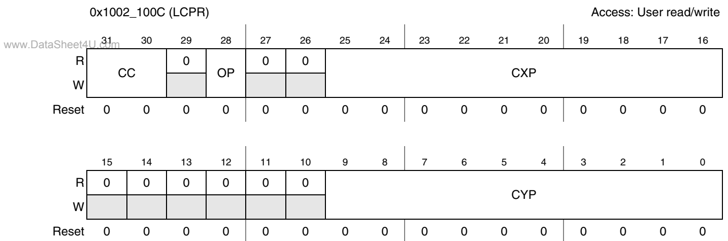
Figure 43-26. LCDC Cursor Position Register (LCPR)
