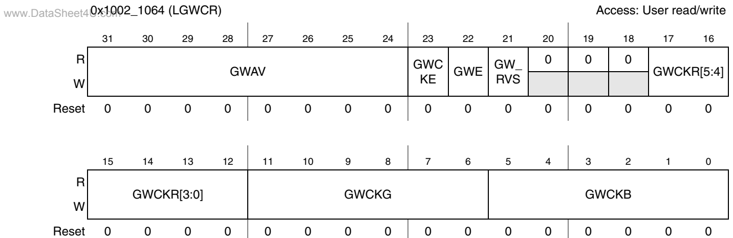
Figure 43-46. LCDC Graphic Window Control Register (LGWCR)
