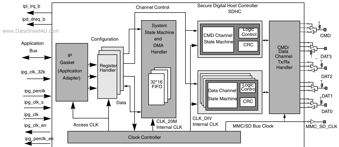
Figure 27-1. Secure Digital Host Controller Block Diagram
