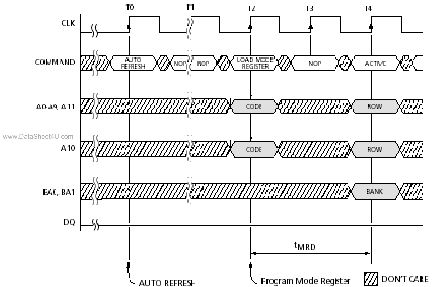
Figure 18-10. tMRD—SDRAM Load Mode Register to Active Command Timing Diagram
