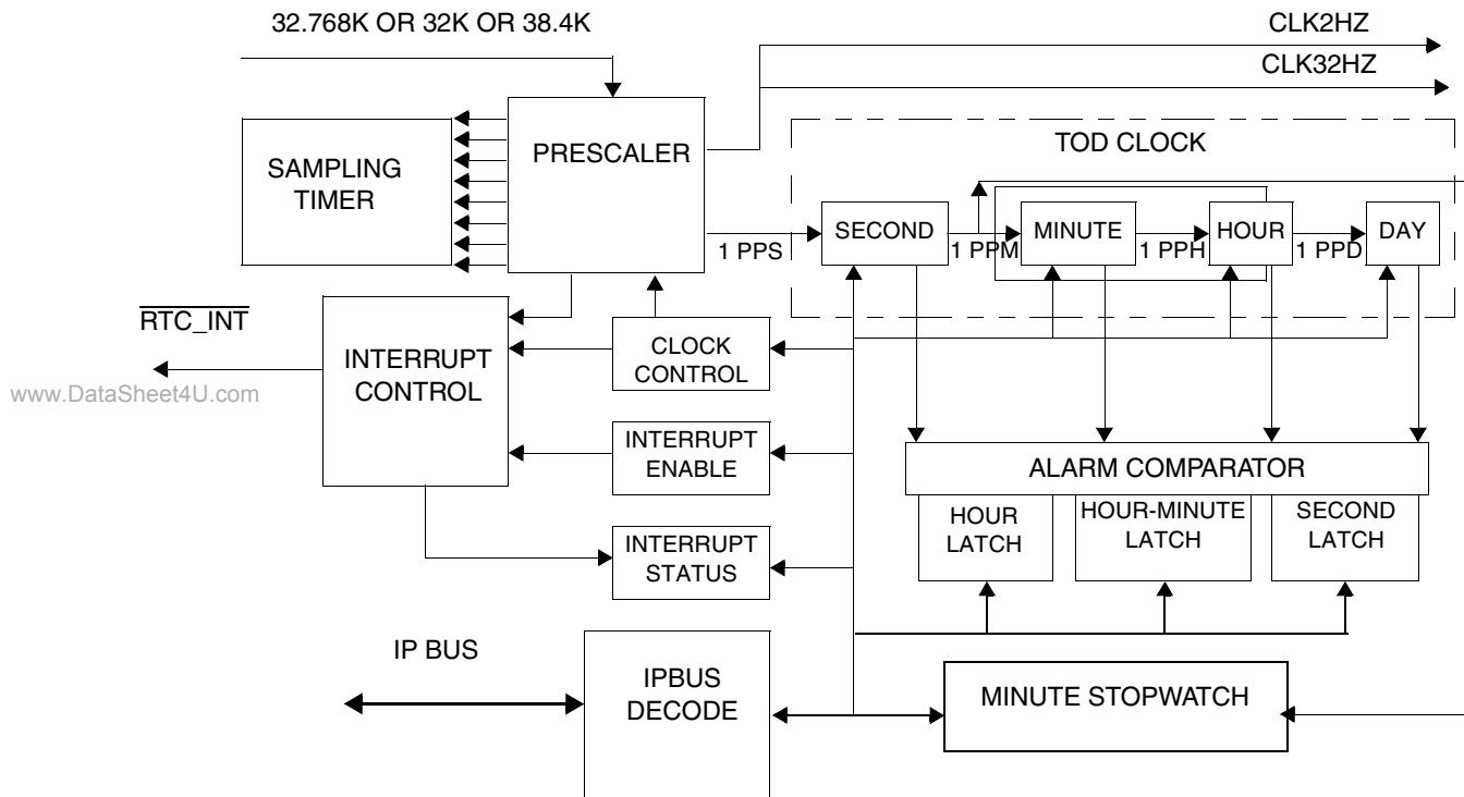
Figure 33-1. Real Time Clock Block Diagram
