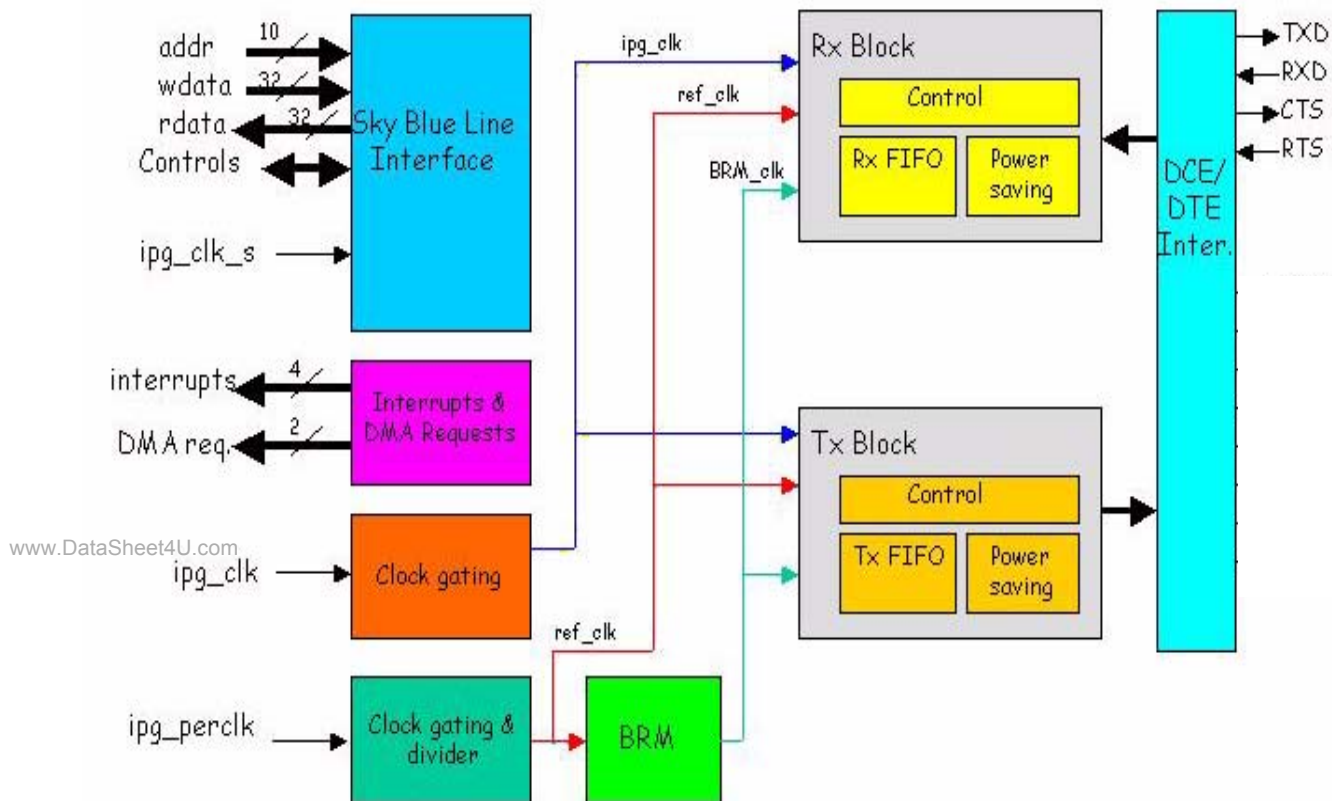
Figure 28-1. UART Block Diagram
