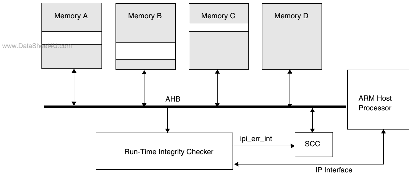
Figure 13-2. System Diagram
