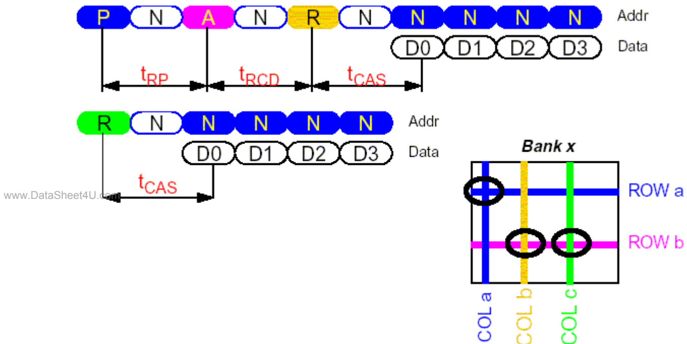
Figure 18-27. SDR SDRAM Read Burst Command Sequence Example
