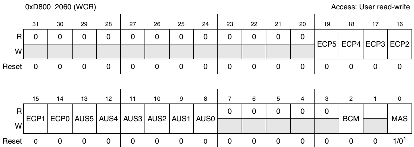
Figure 17-6. WCR Register
