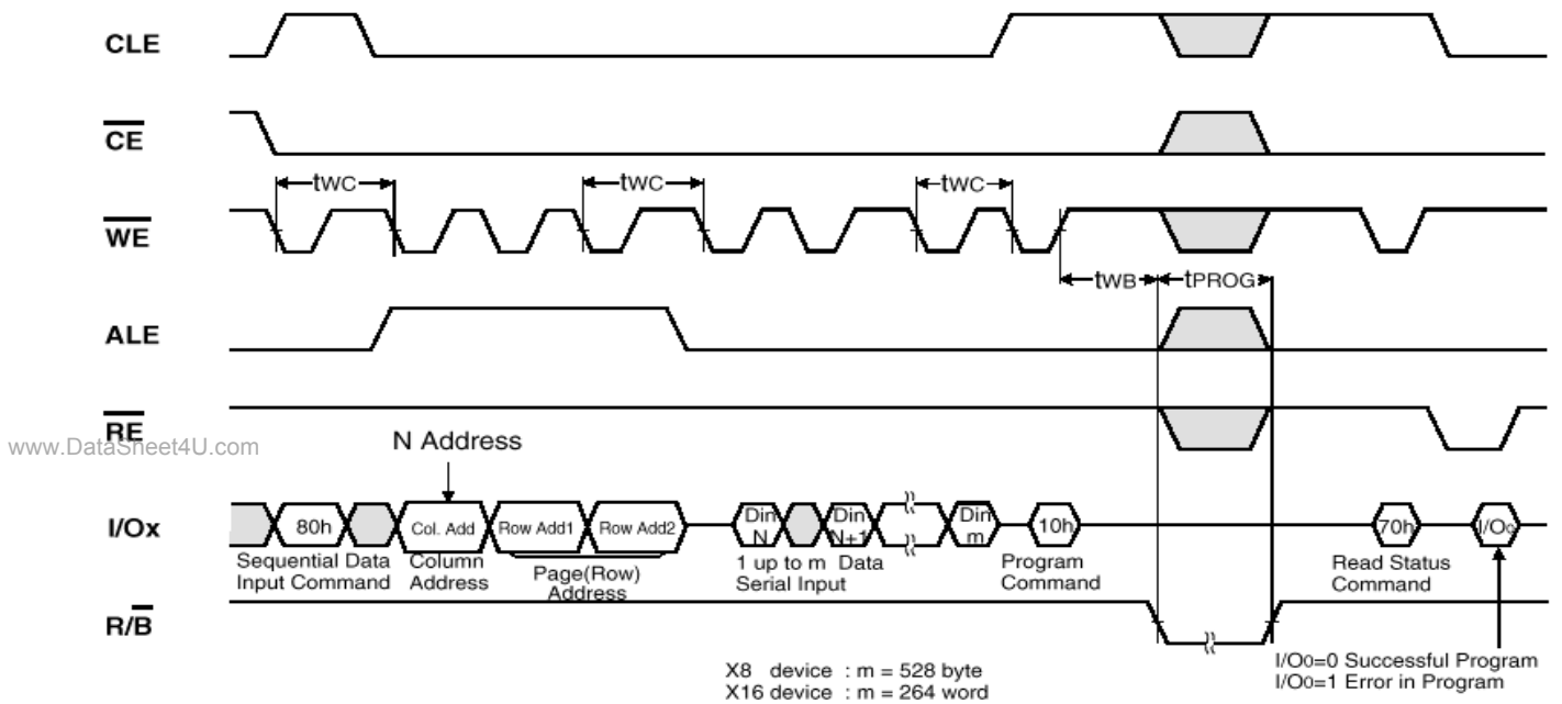
Figure 19-22. Program Operation
