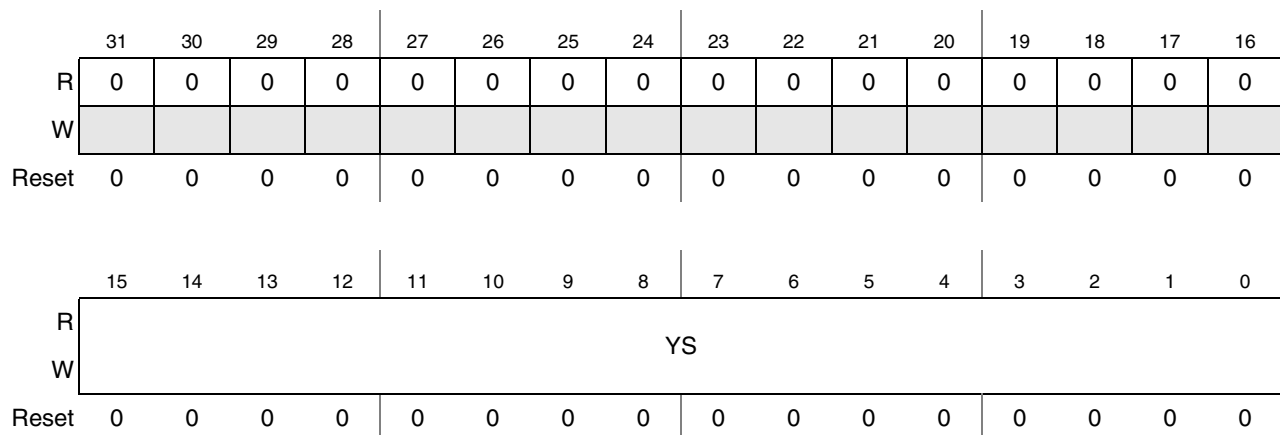
Figure 37-17. Y Size Registers (YSRA, YSRB)
