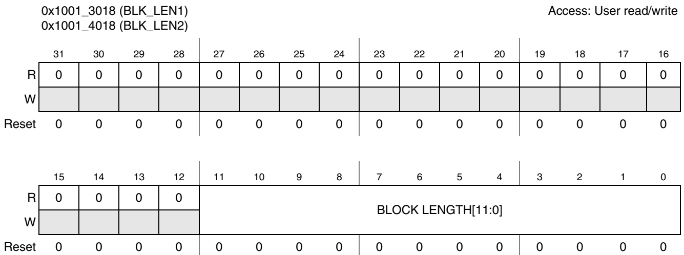
Figure 27-10. SDHC Block Length Register
