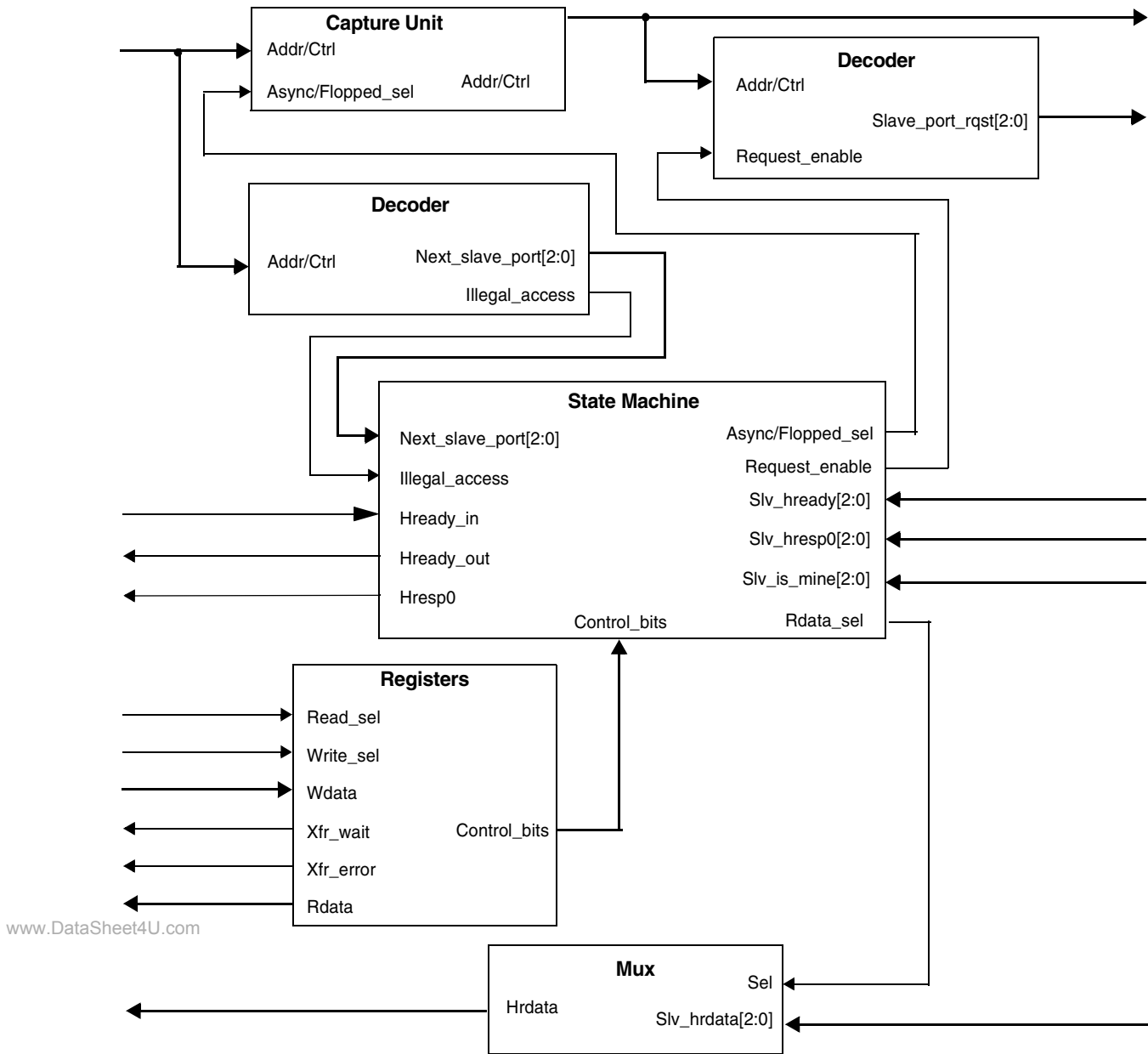
Figure 36-6. MAX Master Port Block Diagram
