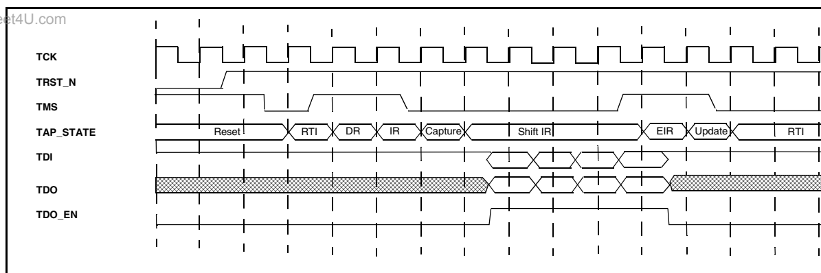
Figure 7-1. JTAG Signals Timing Diagram
