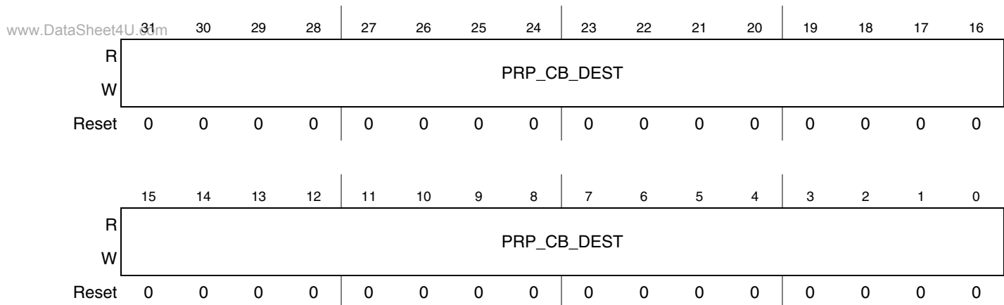
Figure 41-37. PrP Destination Cb Address Register
