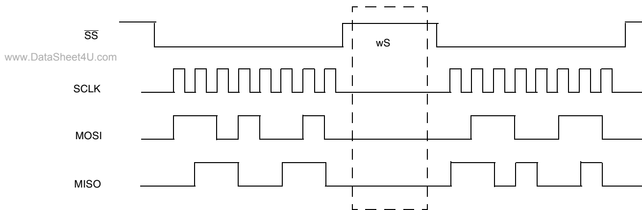
Figure 23-6. SPI Transfers with Wait States
