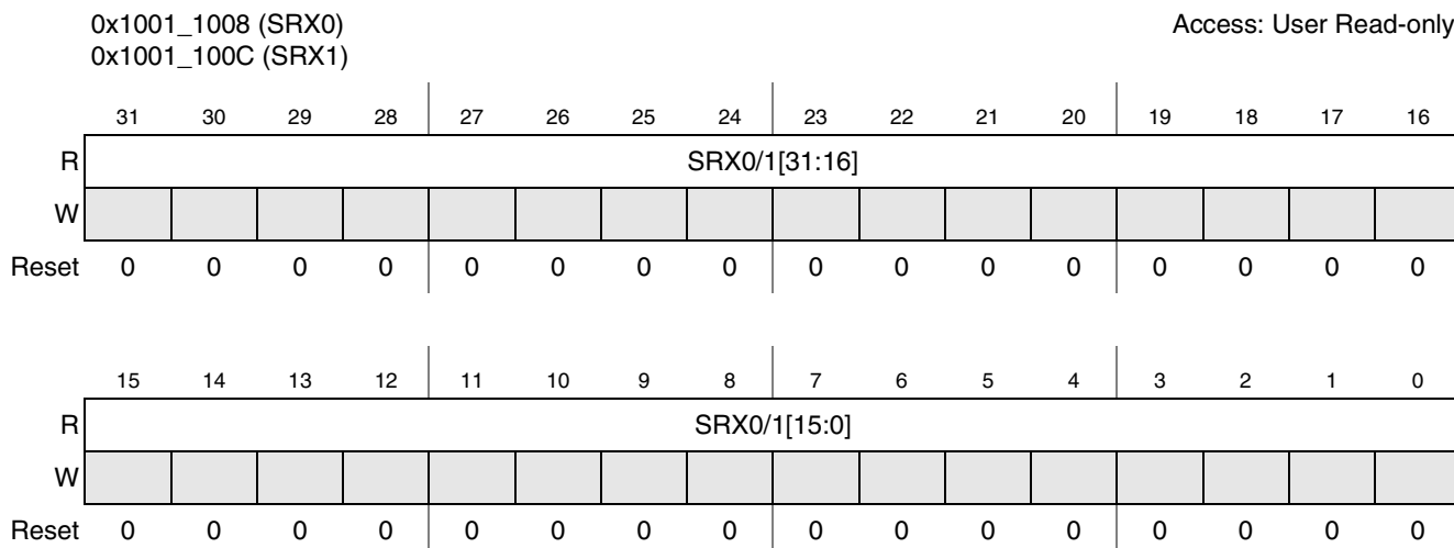
Figure 42-20. SSI Receive Data Registers
