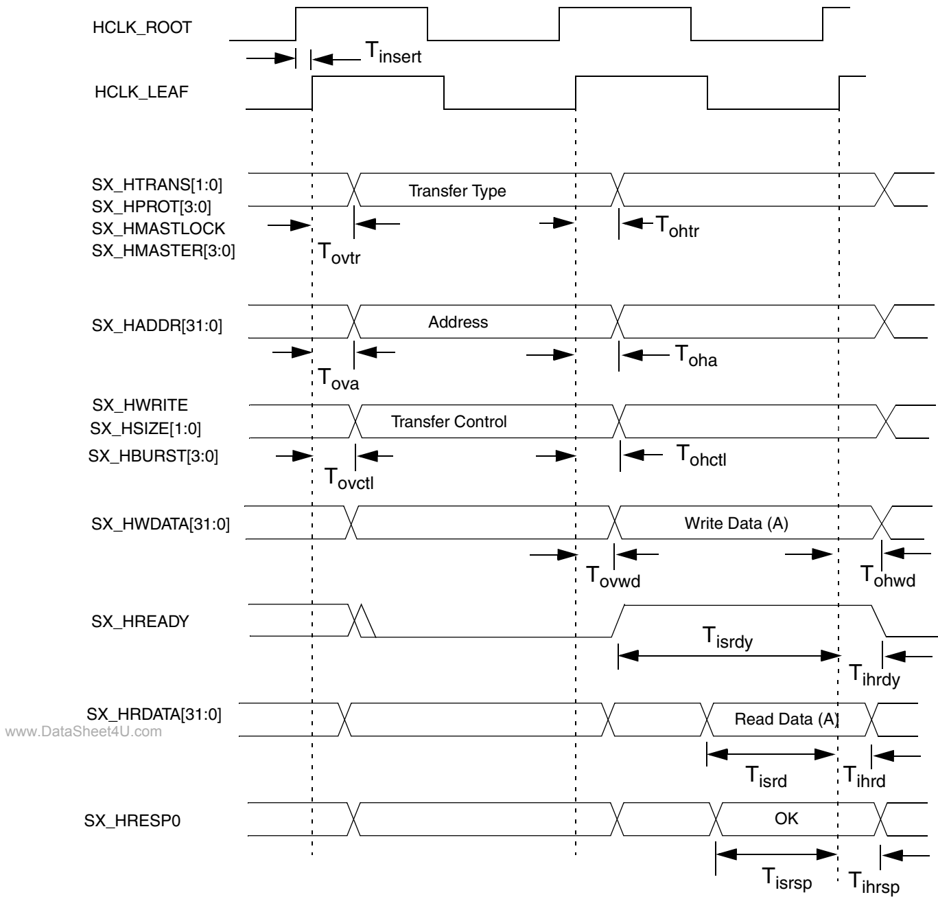
Figure 9-12. Secondary AHB AC Timing Parameters
