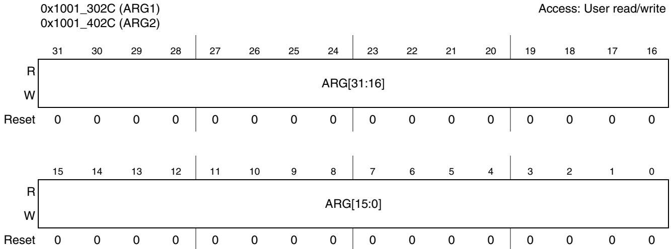
Figure 27-15. SDHC Command Argument Register
