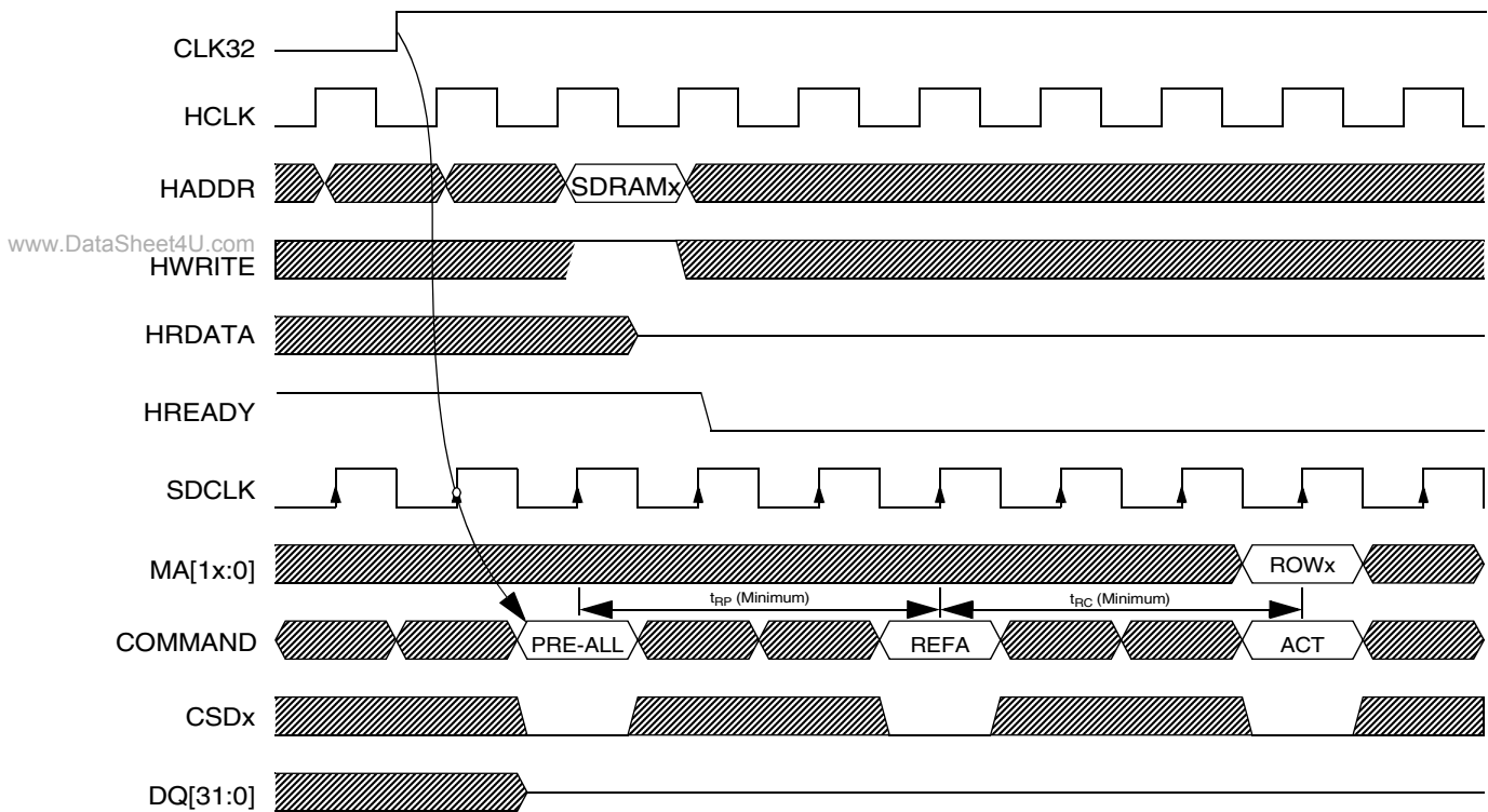
Figure 18-36. Hardware Refresh with Pending Bus Cycle Timing Diagram
