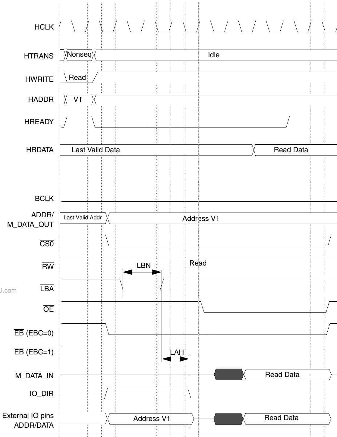
Figure 17-43. Read Access, WSC=7, LBA=1, LBN=1, LAH=1, OEA=7
