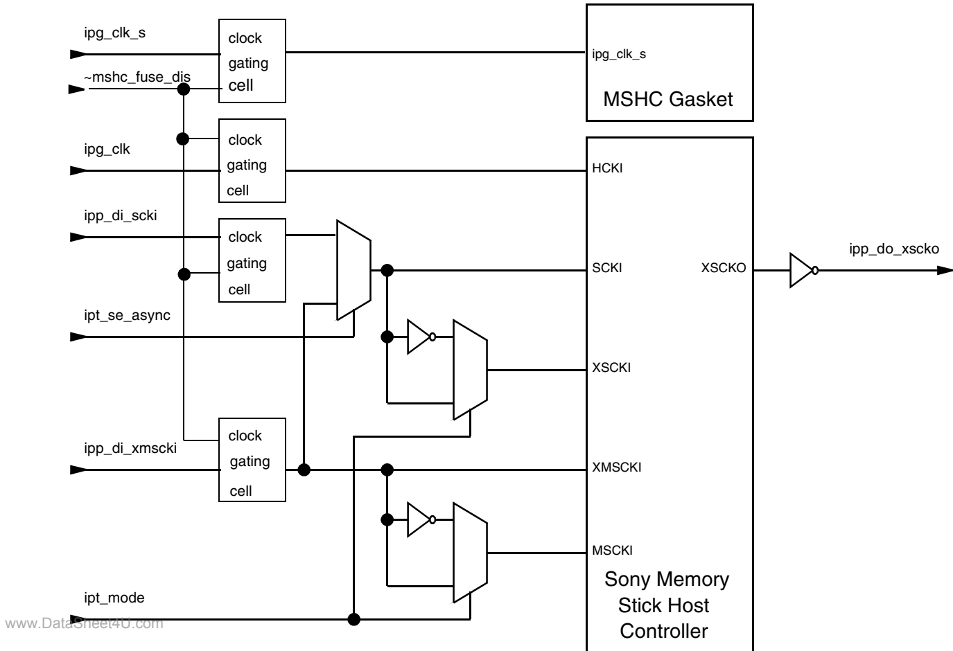
Figure 26-2. MSHC Clock Structure
