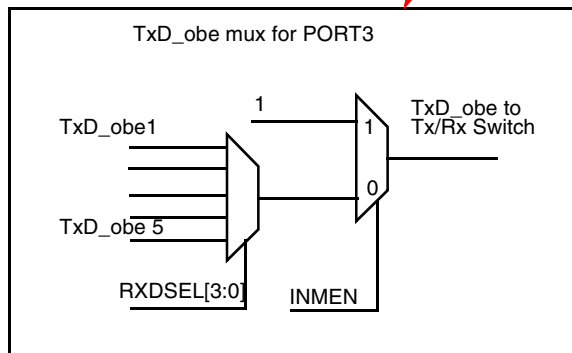
Figure 38-1. AUDMUX Block Diagram
