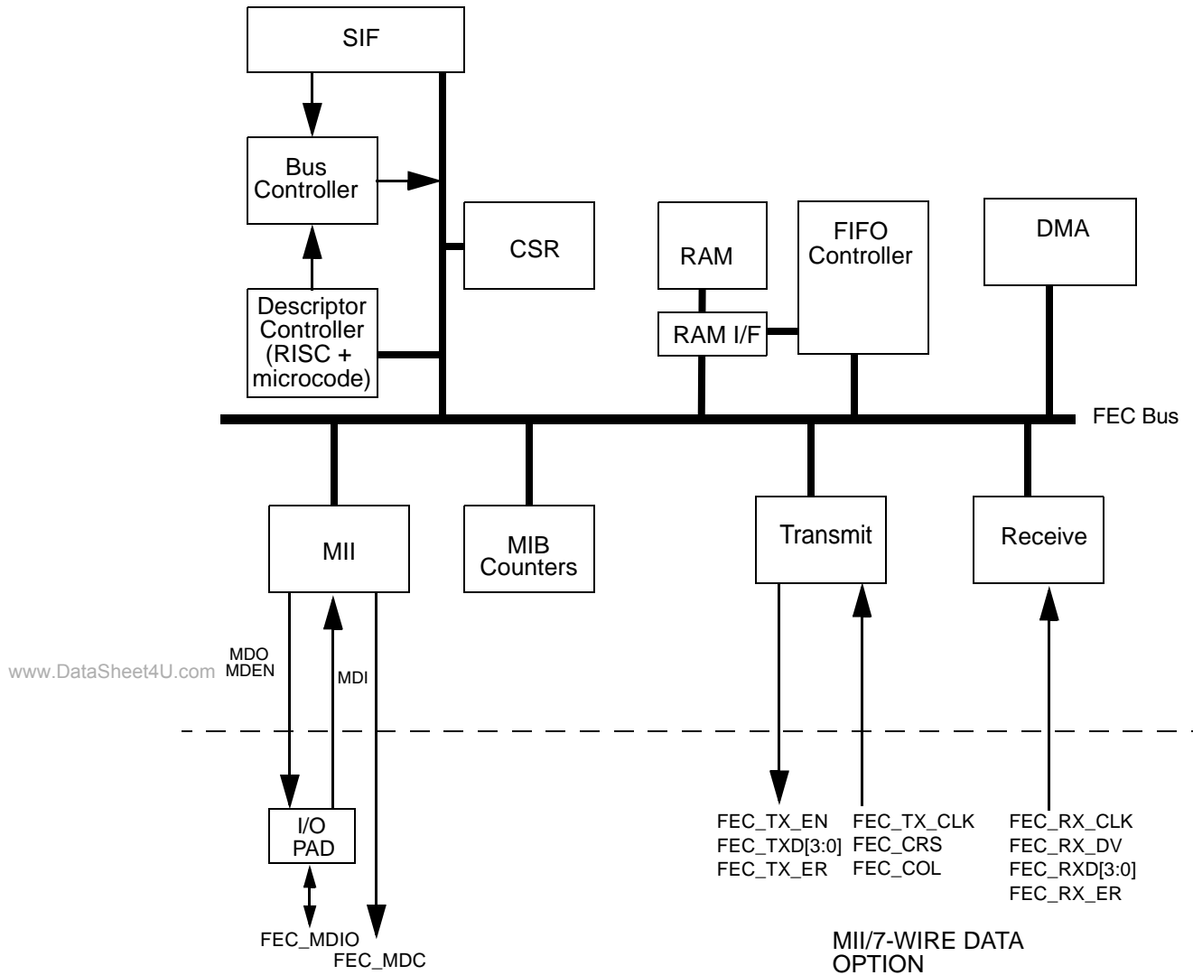
Figure 29-1. FEC Block Diagram
