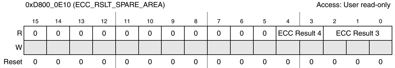
Figure 19-12. ECC_Rslt_Spare_Area Register
