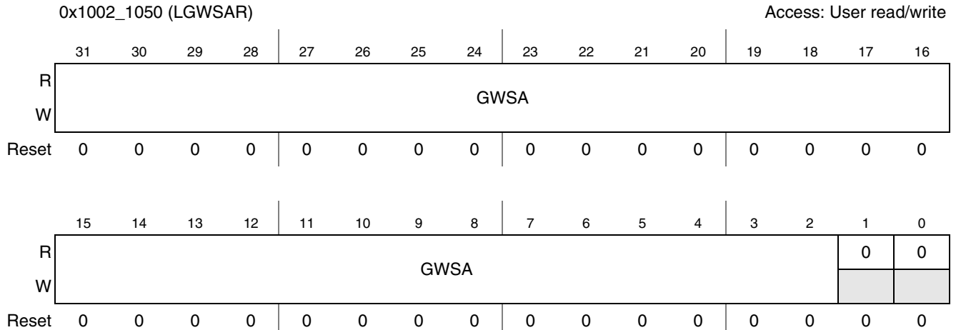
Figure 43-41. LCDC Graphic Window Start Address Register (LGWSAR)
