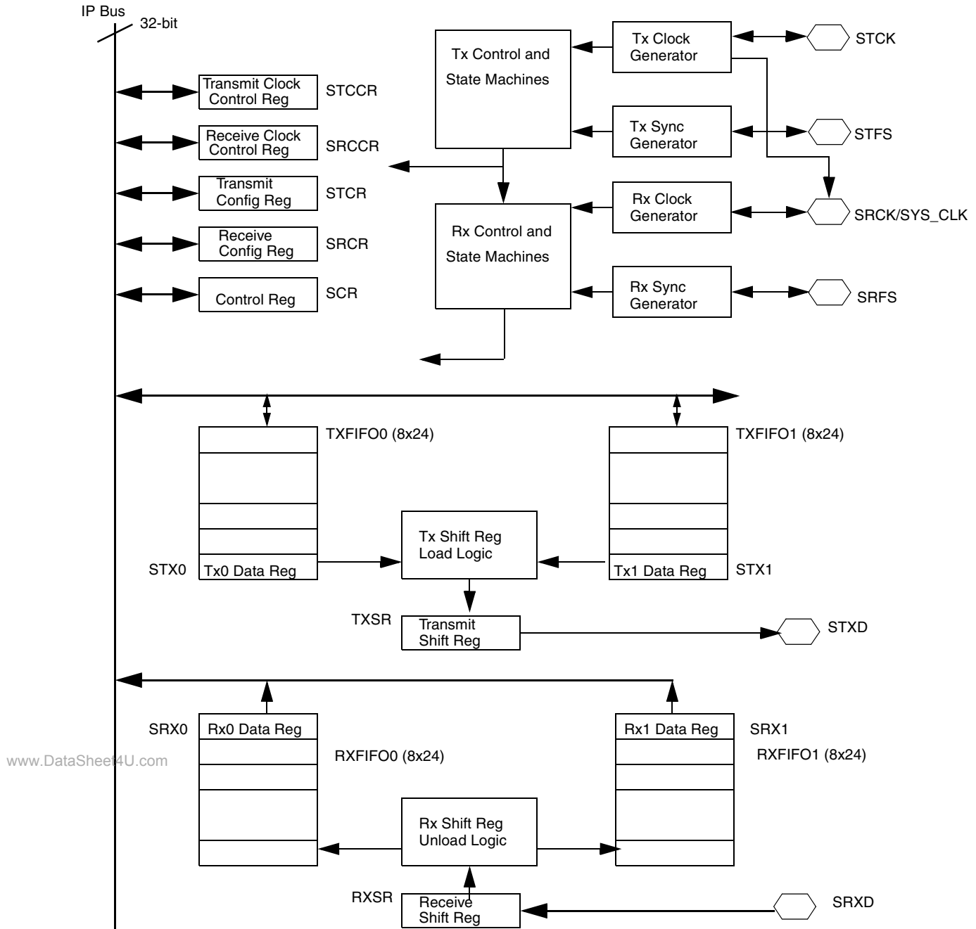
Figure 42-1. SSI Block Diagram
