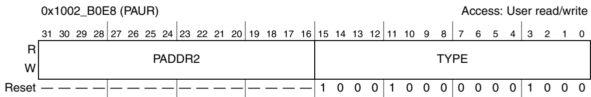
Figure 29-15. PAUR Register
