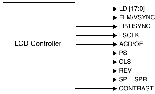
Figure 43-11. LCDC Interface Signals
