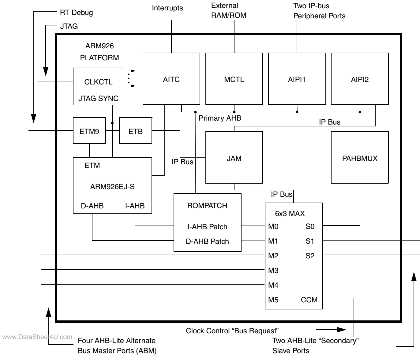
Figure 9-1. ARM9 Platform Block Diagram
