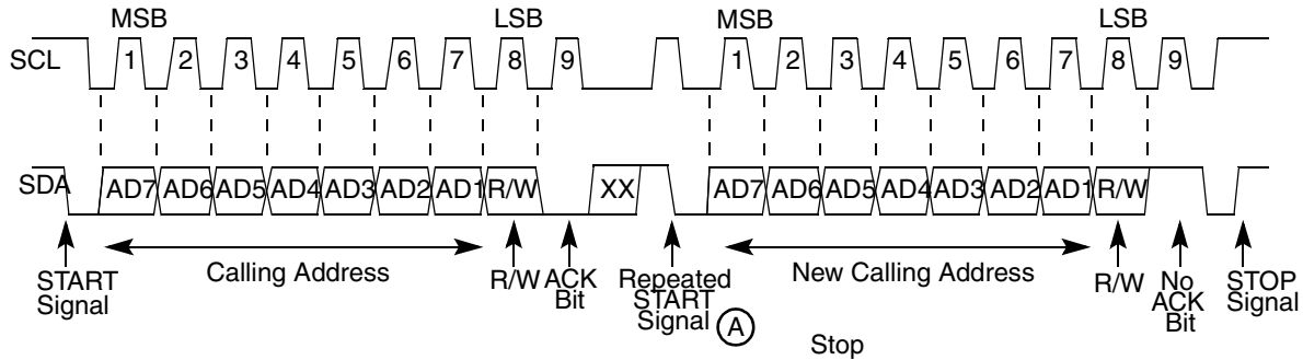
Figure 24-12. Repeated START
