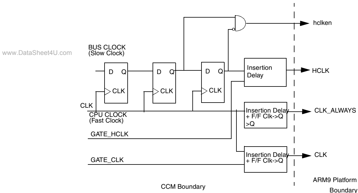
Figure 9-4. Example hclk to clk Synchronization When clk Is Faster
