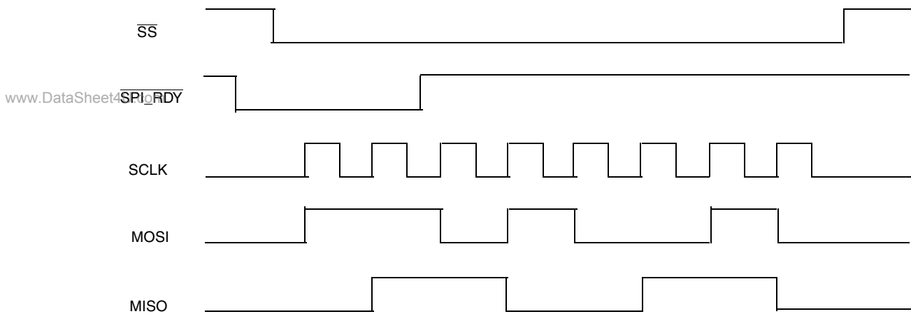
Figure 23-4. Relationship between a SPI transfer and the Falling Edge of \overline{SPI\_RDY}
