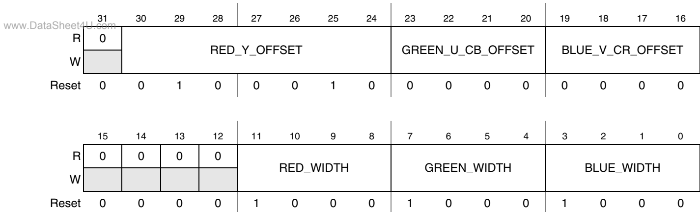
Figure 41-41. PrP Source Pixel Format Control Register
