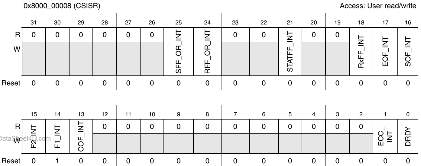
Figure 39-12. CSI Status Register (CSISR)
