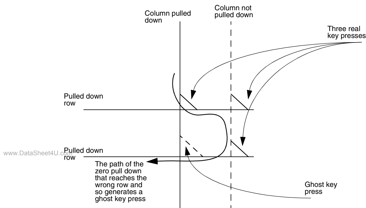
Figure 25-10. Decoding Wrong Three-Key Presses
