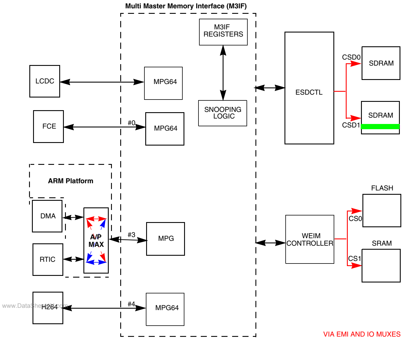
Figure 16-29. M3IF System Example
