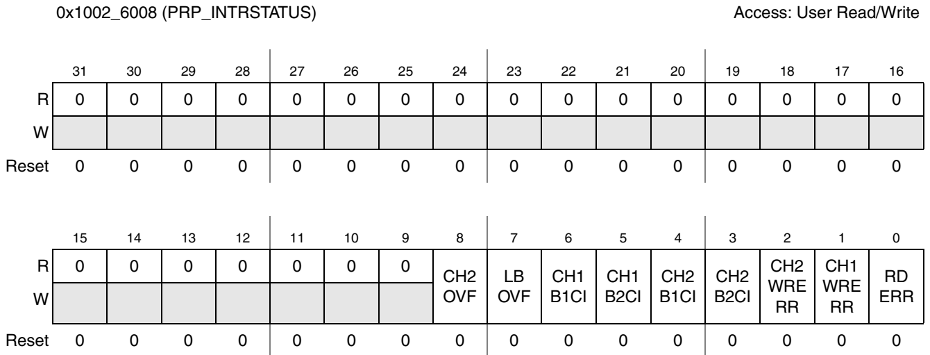
Figure 41-30. PrP Interrupt Status Register
