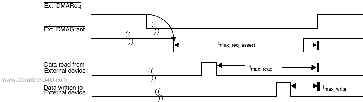
Figure 37-3. Safe Maximum Timings for External Request De-Assertion
