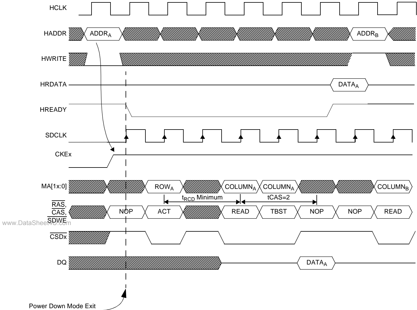
Figure 18-42. SDR SDRAM Precharge Power Down Mode Exit Timing Diagram
