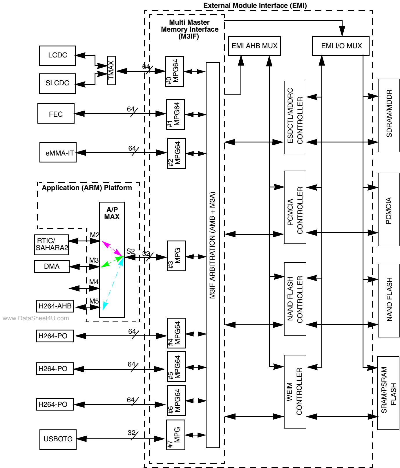
Figure 15-1. M3IF System Block Diagram
