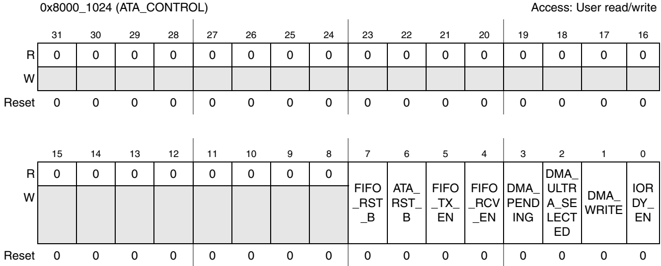
Figure 22-12. ATA_CONTROL Register
