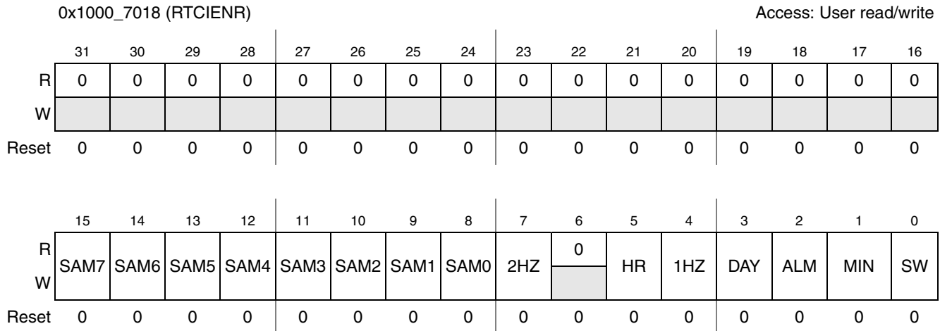
Figure 33-9. RTC Interrupt Enable Register
