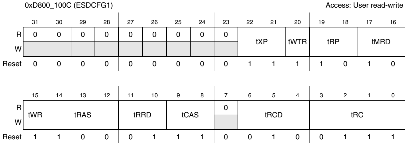
Figure 18-7. Enhanced SDRAM Configuration Register 1 (ESDCFG1)
