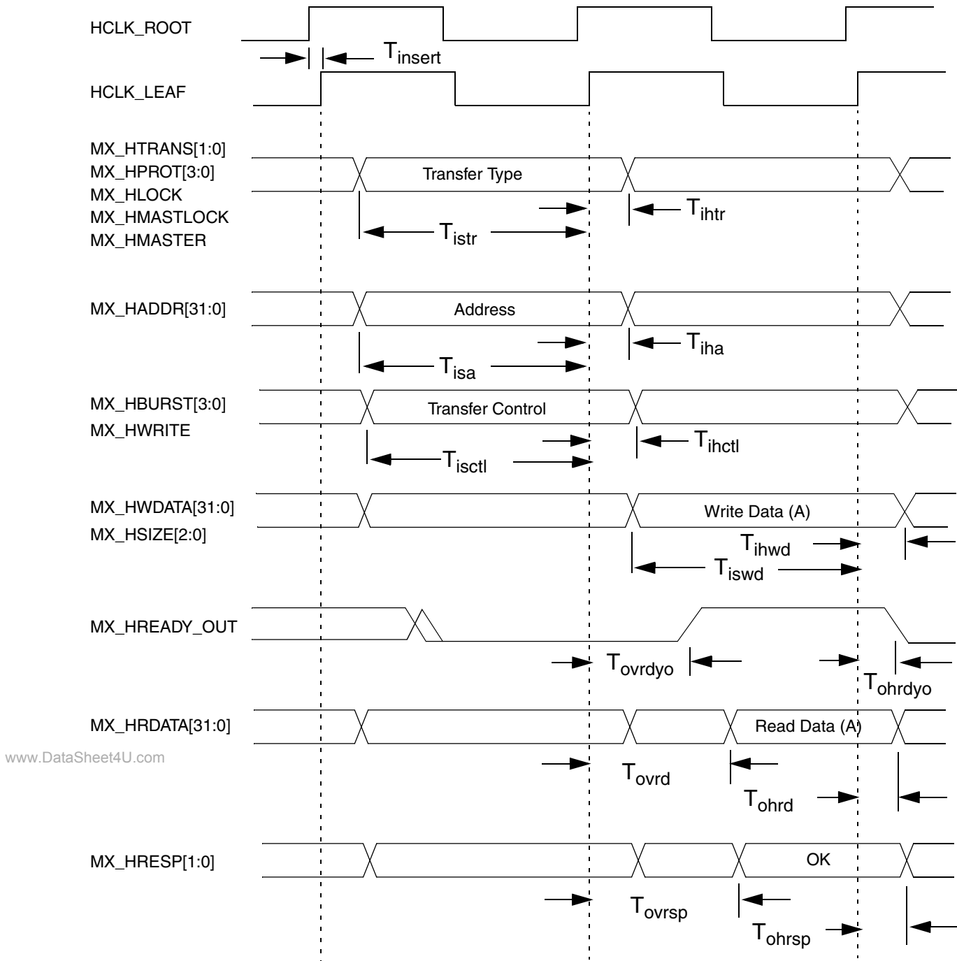
Figure 9-11. Alternate Bus Master Timing Parameters
