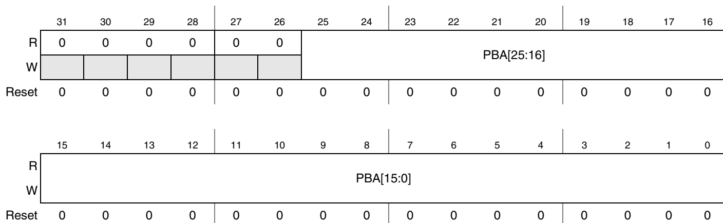
Figure 20-6. PCMCIA Base Registers 0–4 (PBR0–PBR4)
