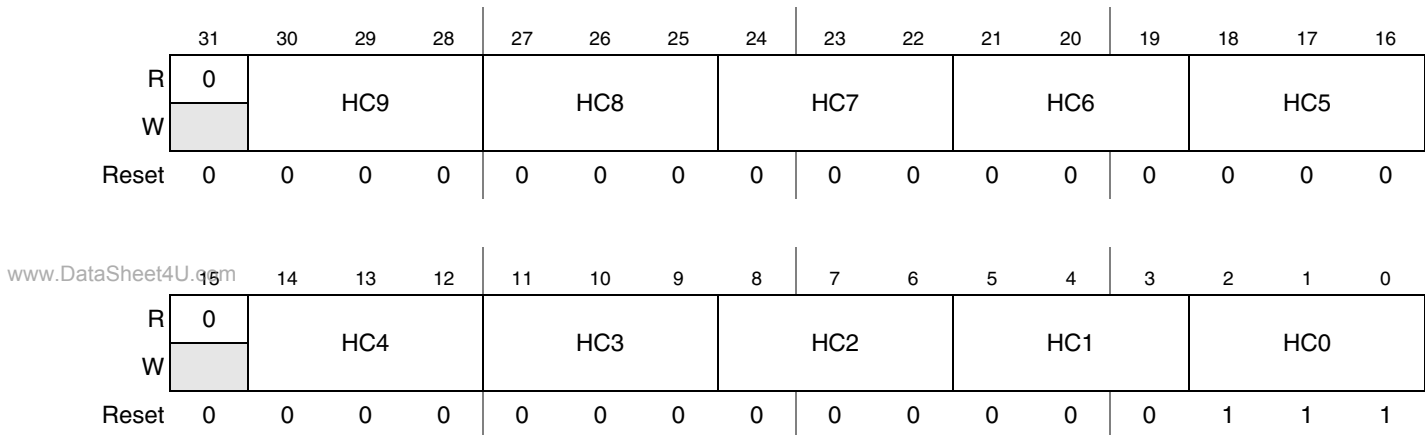
Figure 41-55. PrP Channel-2 Horizontal Resize Coefficient 1
