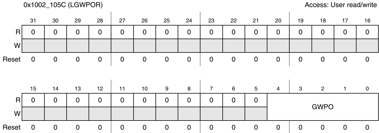
Figure 43-44. LCDC Graphic Window Panning Offset Register (LGWPOR)
