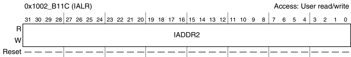
Figure 29-18. IALR Register
