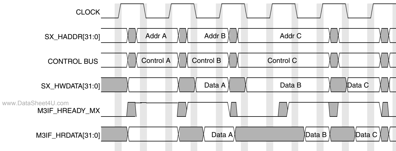
Figure 16-14. MPG Multiple Transfers
