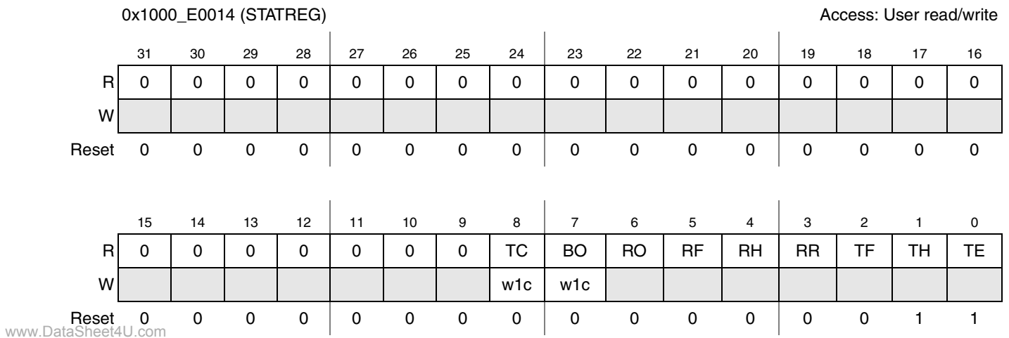
Figure 23-20. Status Register Diagram
