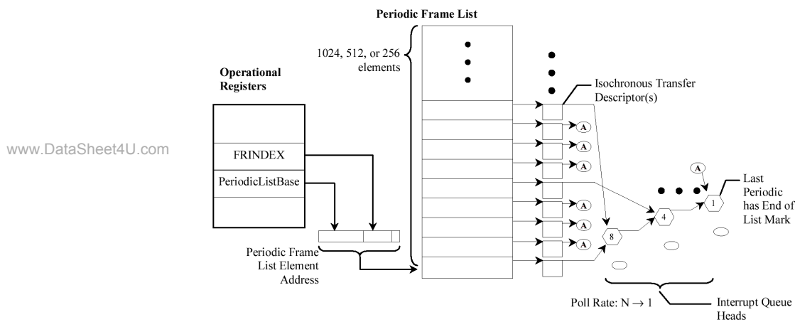
Figure 30-43. Periodic Schedule Organization
