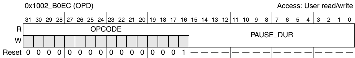
Figure 29-16. OPD Register
