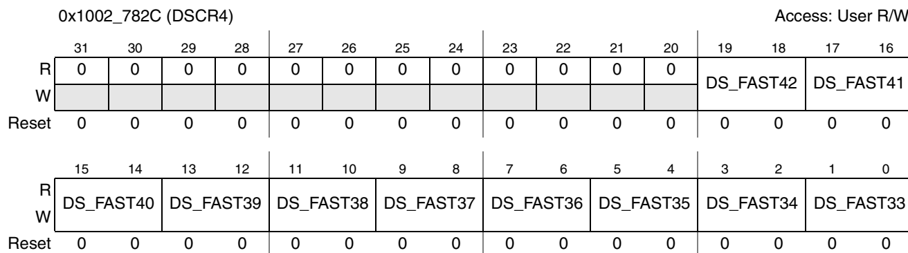
Figure 4-9. Drive Strength Control Register 4 (DSCR4)
