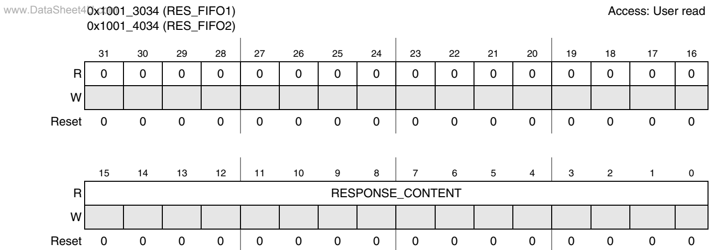
Figure 27-16. SDHC Response FIFO Register
