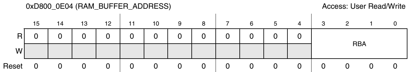
Figure 19-5. RAM Buffer Address Register
