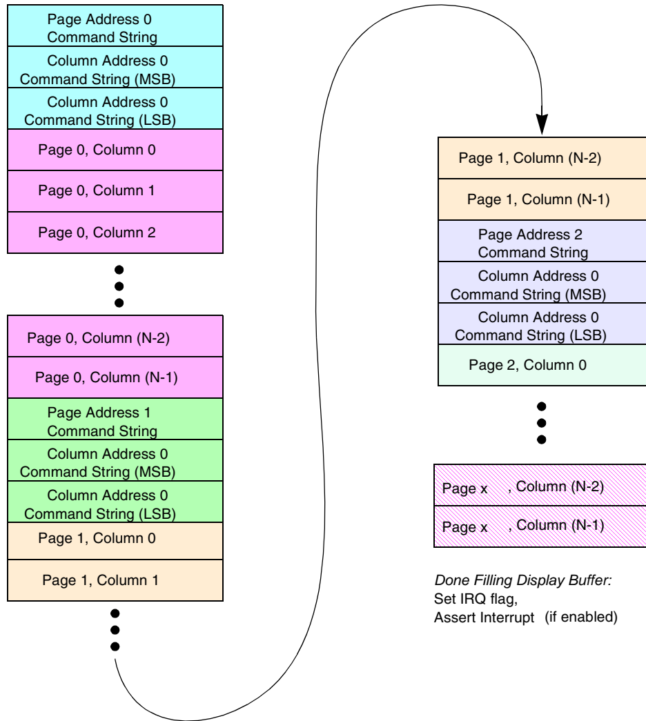
www.DataSheet4U.com Figure 44-9. SLCDC Automatic Mode Write Sequence (Monochrome Display)
