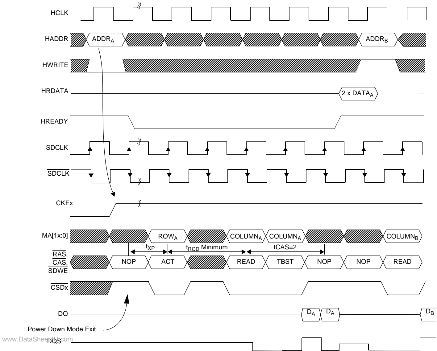
Figure 18-44. Mobile DDR SDRAM Precharge Power Down Mode Exit Timing Diagram
