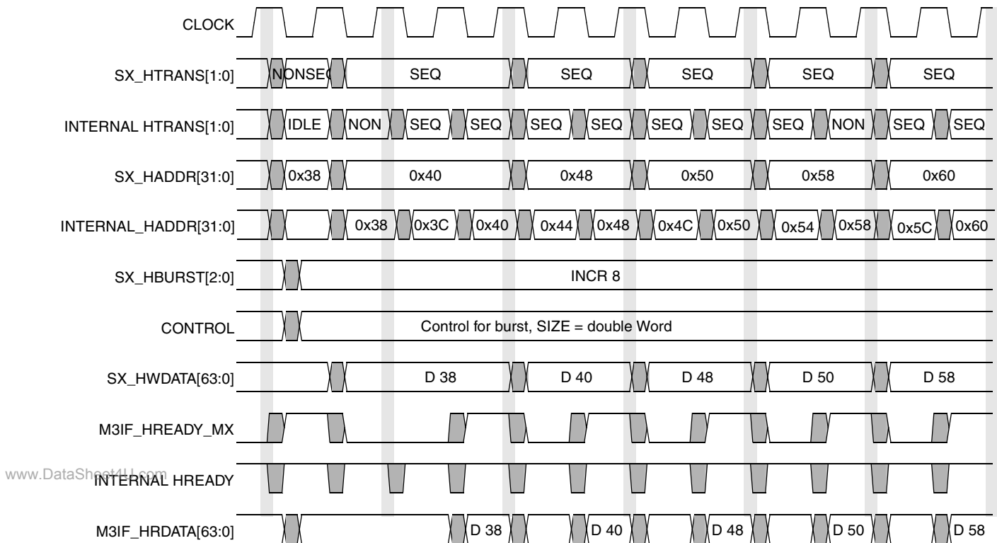
Figure 16-21. MPG64—8 Beat Incremental Burst of Double Words to 32-bit SDRAM
