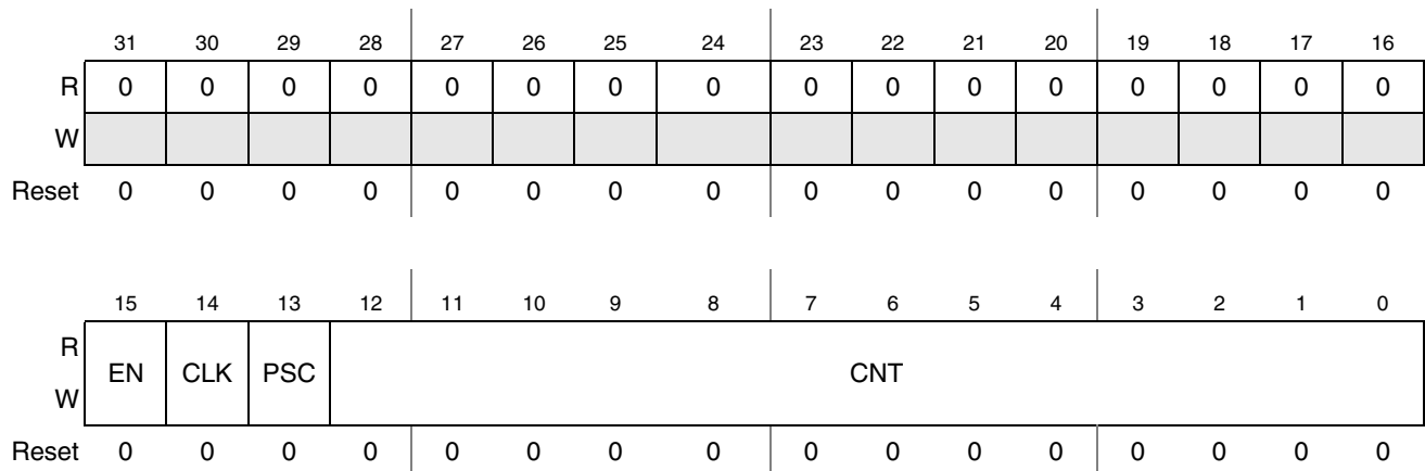
Figure 37-24. Channel Request Time-Out Registers (RTOR0-RTOR15)
