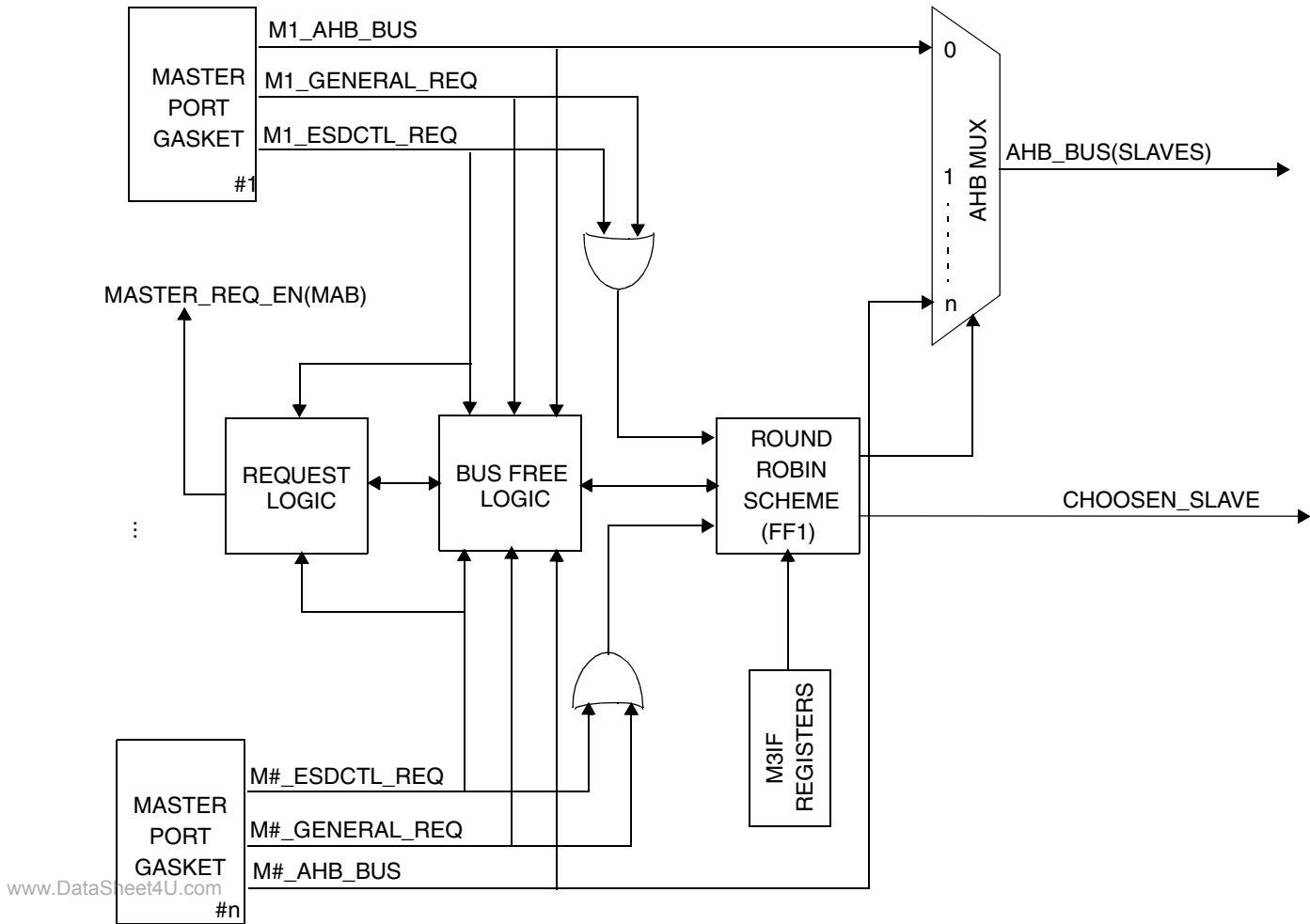
Figure 16-22. M3A Block Diagram
