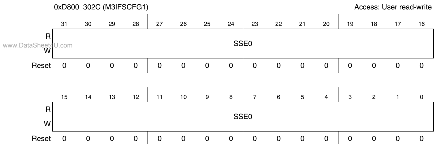
Figure 16-6. M3IF Snooping Configuration Register 1 (M3IFSCFG1)
