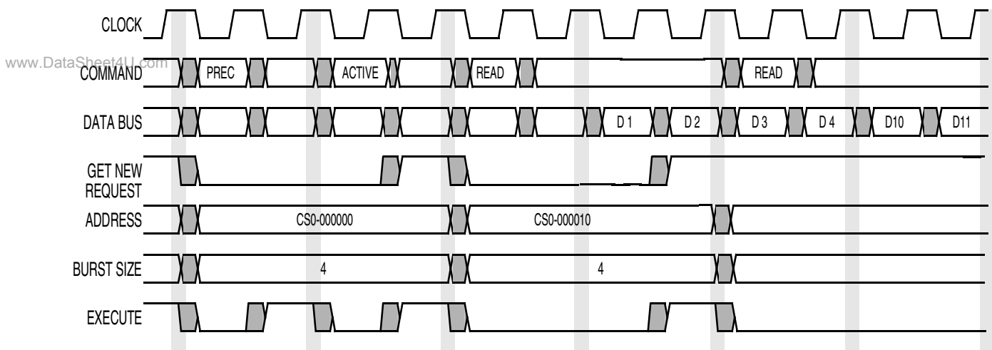
Figure 18-31. SDR Simple Read after Read Latency Hiding Timing Diagram
