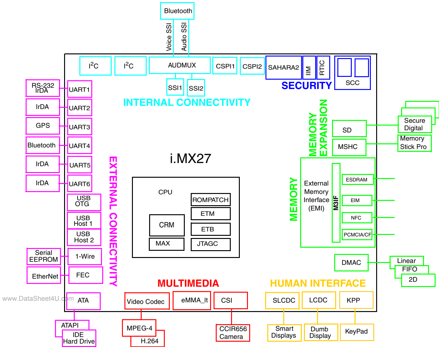
Figure 1-2. i.MX27 Connectivity Example
