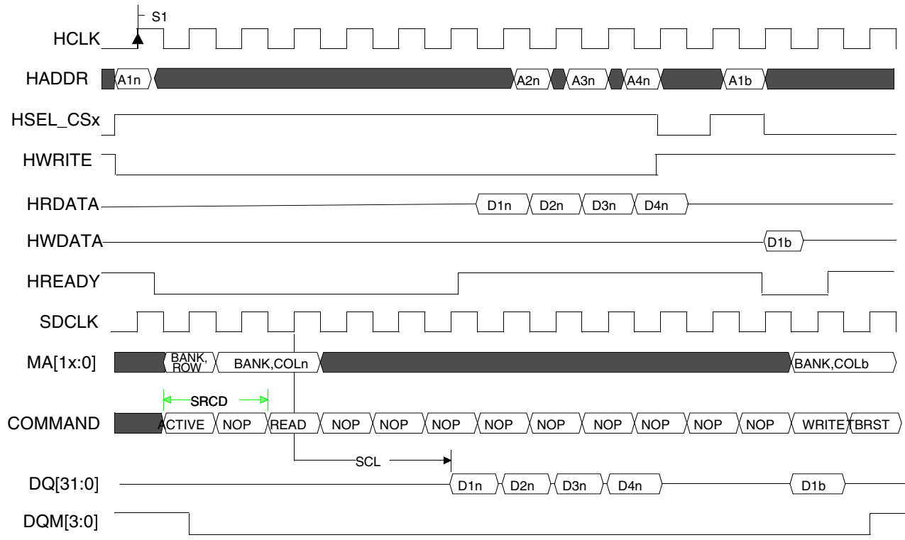
Figure 18-68. SDR Burst Read Followed by On-Page Write Timing Diagram
