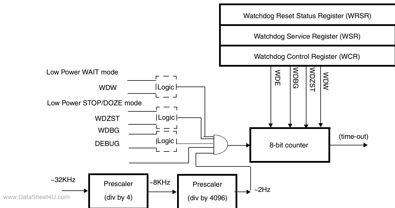
Figure 34-1. WDOG Block Diagram
