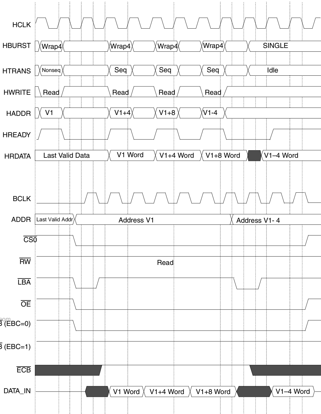
Figure 17-38. Wrap 4 AHB Read Access, WSC=2, SYNC=1, DOL=1, WRAP=0
