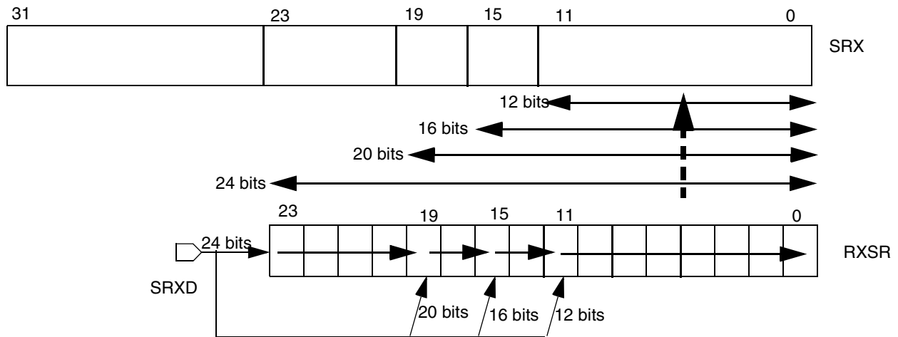
Figure 42-24. Receive Data Path (RXBIT0=1, RSHFD=1) (LSB Alignment)
