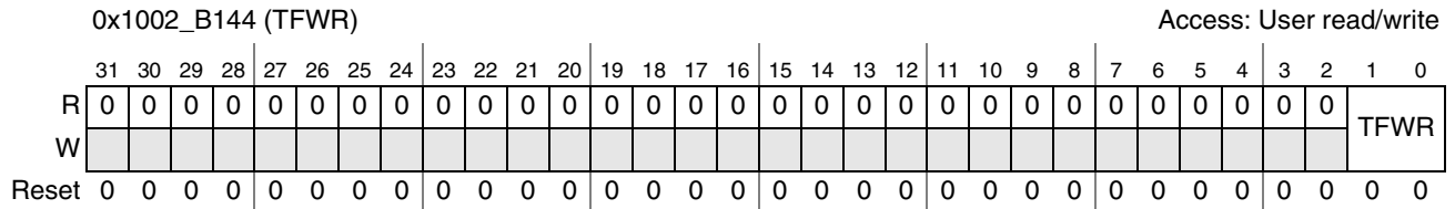
Figure 29-21. TFWR Register
