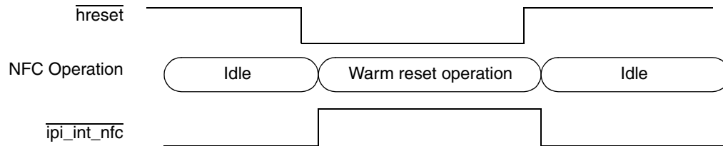
Figure 19-2. Warm Reset Operation
