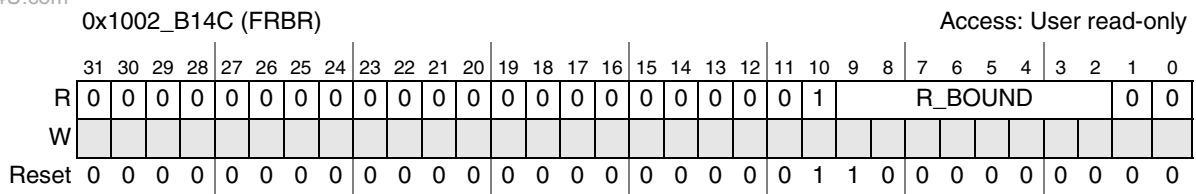
Figure 29-22. FRBR Register
