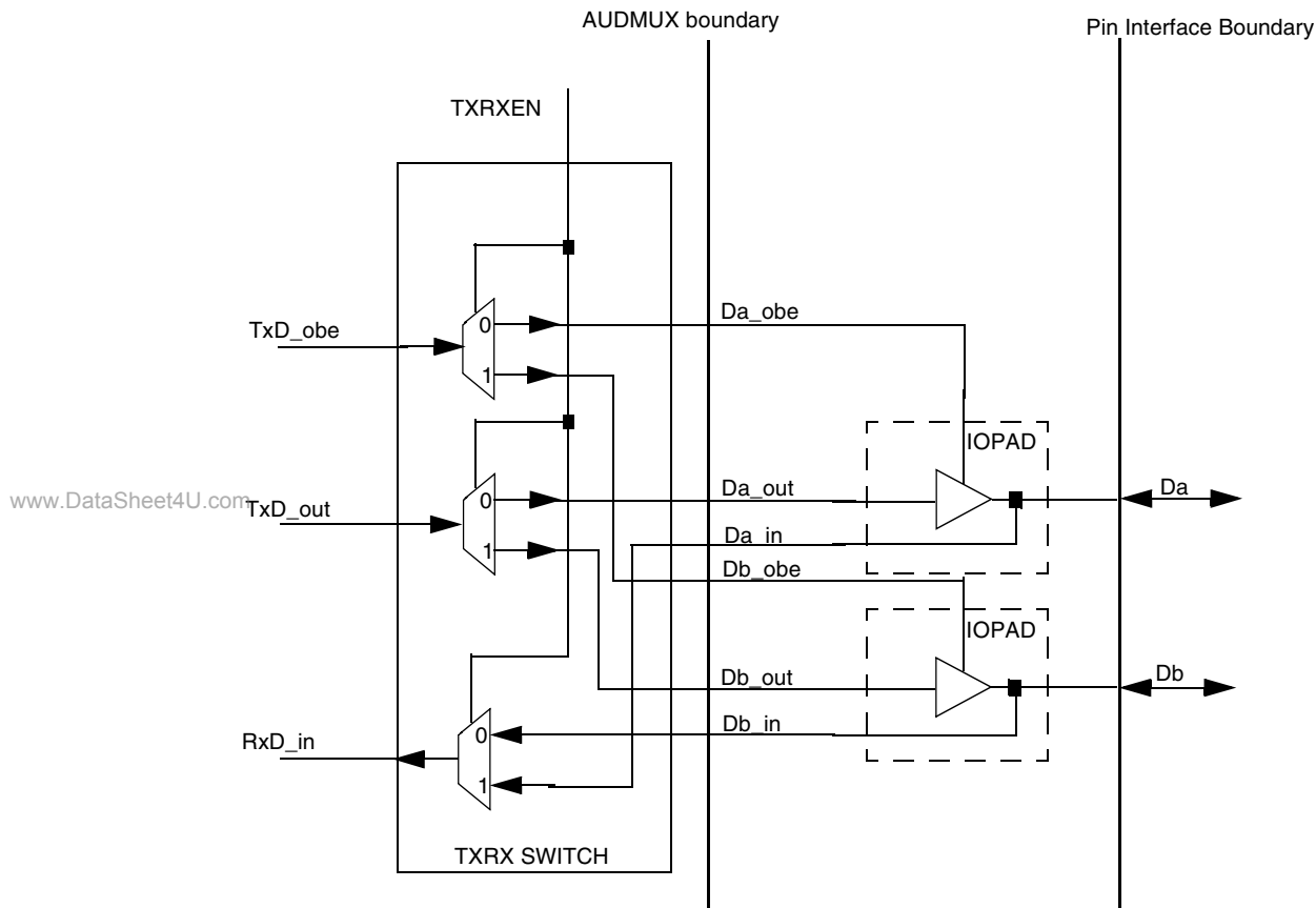
Figure 38-3. Tx/Rx Switch
