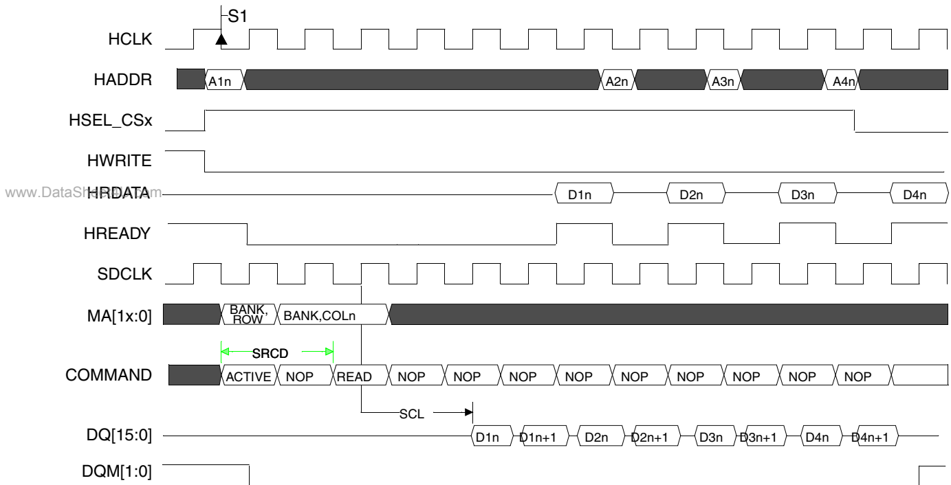
Figure 18-55. Off-Page Burst Read Timing Diagram (16-Bit Memory, LPDDR 8-Bit Is Not Supported)
