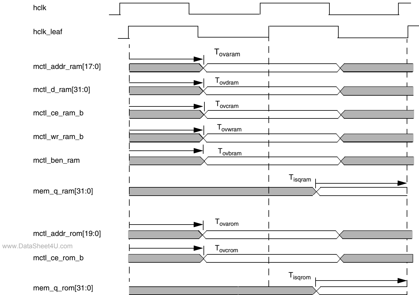
Figure 9-13. RAM and ROM Interface AC Timing Parameters
