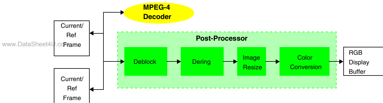
Figure 1-6. Post-Processor
