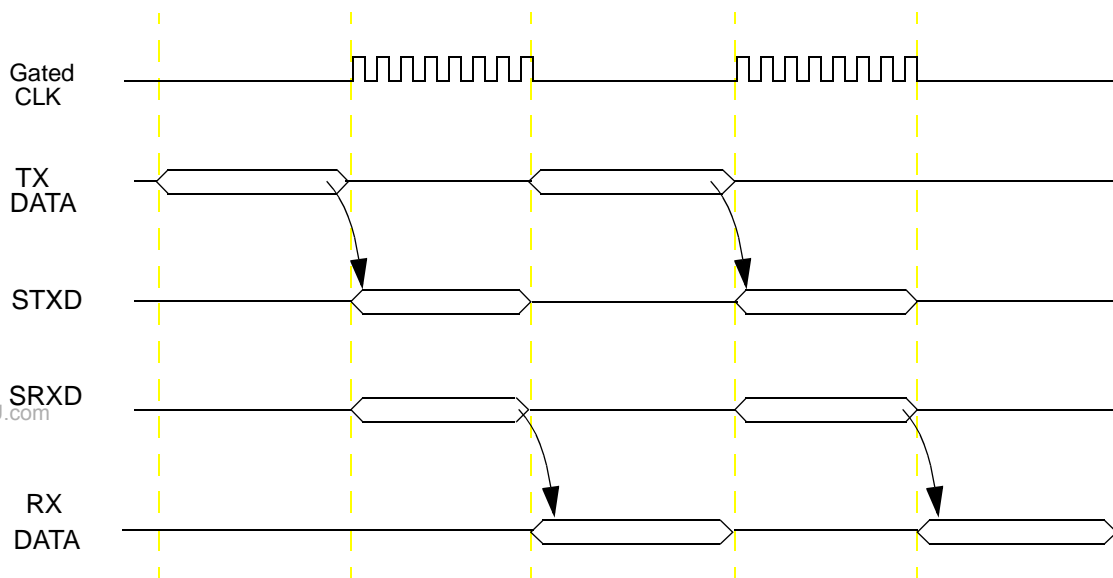
Figure 42-4. Normal Mode Timing—External Gated Clock
