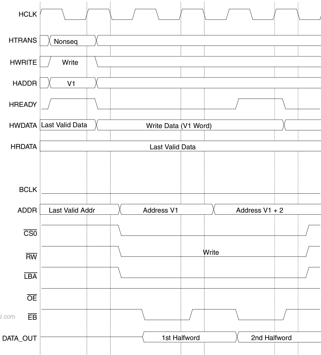
Figure 17-15. Write Access, WSC=1, EBWA=1, EBWN=1
