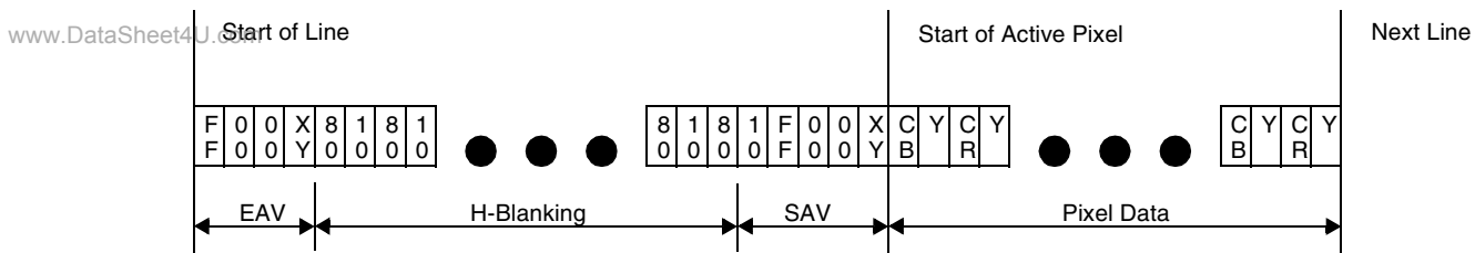
Figure 39-4. CCIR656 General Line Timing
