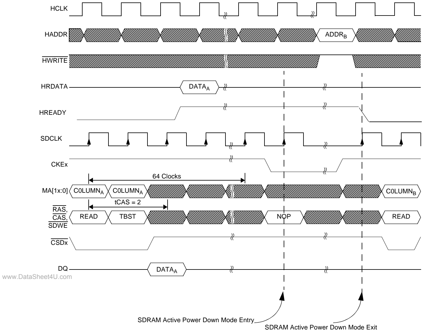
Figure 18-45. SDR SDRAM Active Power Down Mode Timing Diagram
