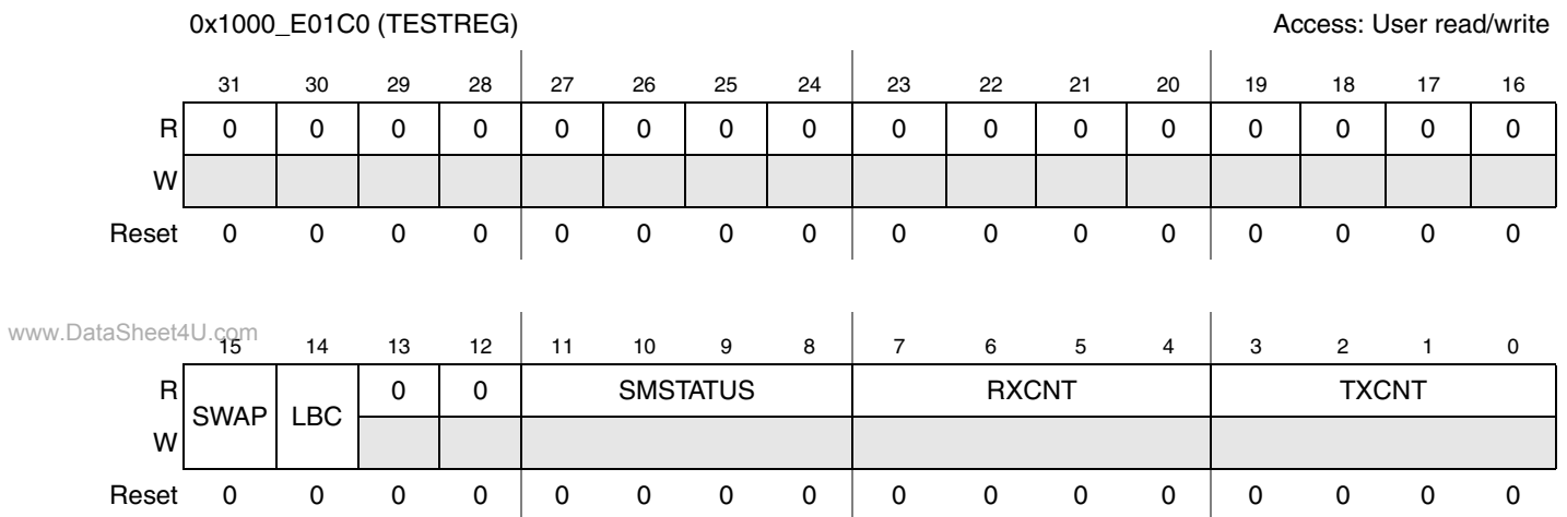
Figure 23-22. Test Control Register Diagram
