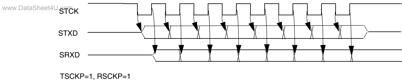
Figure 42-7. Internal Gated Mode Timing—Falling Edge Clocking/Rising Edge Latching
