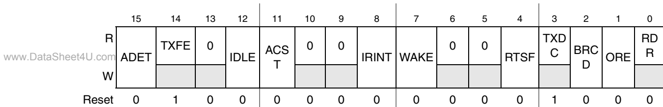
Figure 28-12. UART Status Register 2 (USR2) Summary
