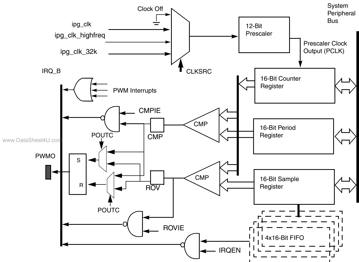
Figure 32-1. Pulse-Width Modulator Block Diagram
