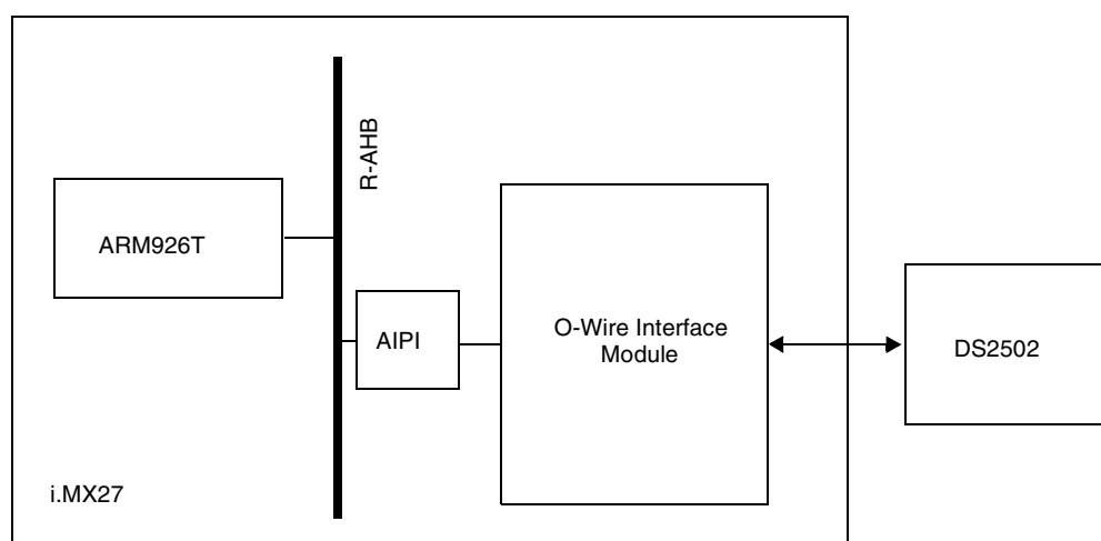
Figure 21-1. 1-Wire Connection
