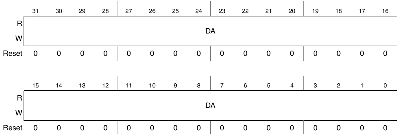
Figure 37-19. Channel Destination Address Registers (DAR0–DAR15)
