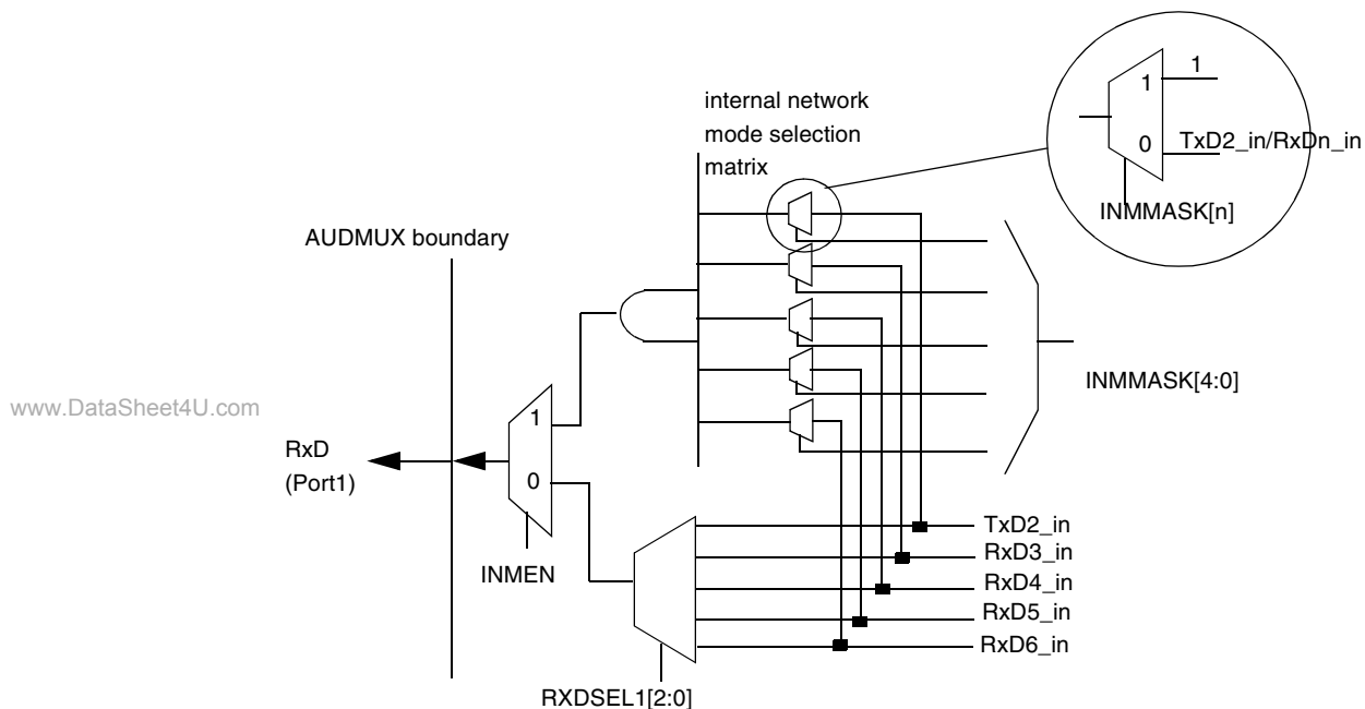
Figure 38-2. Internal Network Mode
