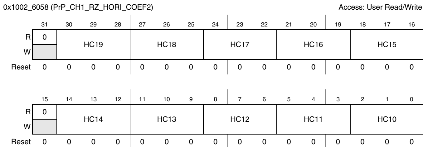
Figure 41-50. PrP Channel-1 Horizontal Resize Coefficient 2
