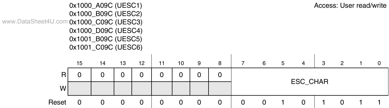
Figure 28-13. UART Escape Character Register Summary (UESC)
