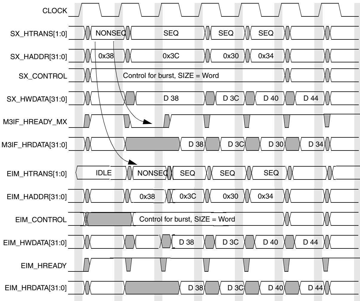
Figure 16-23. M3A Simple Transfer Timing Diagram
