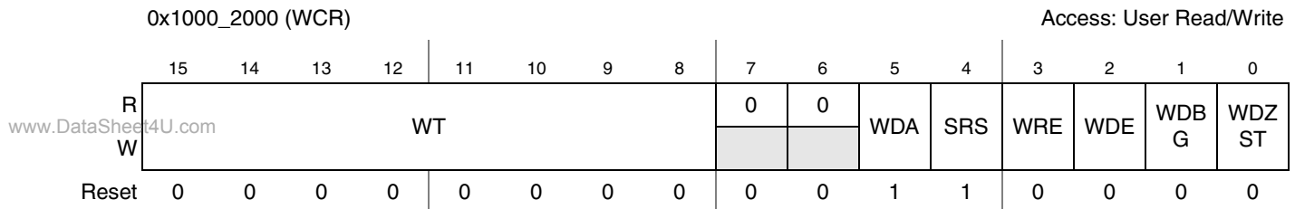
Figure 34-3. Watchdog Control Register
