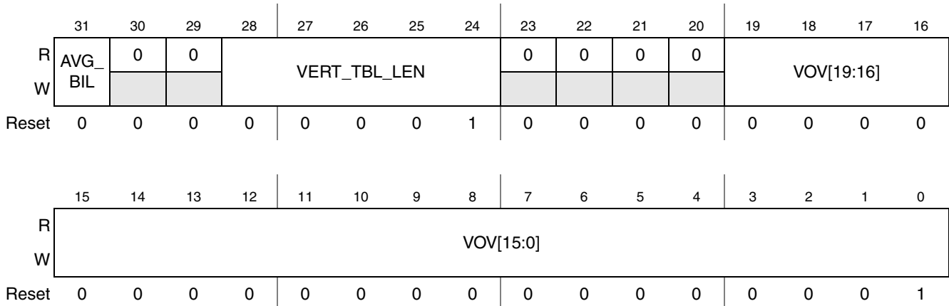
Figure 41-54. PrP Channel1 Vertical Resize Valid
