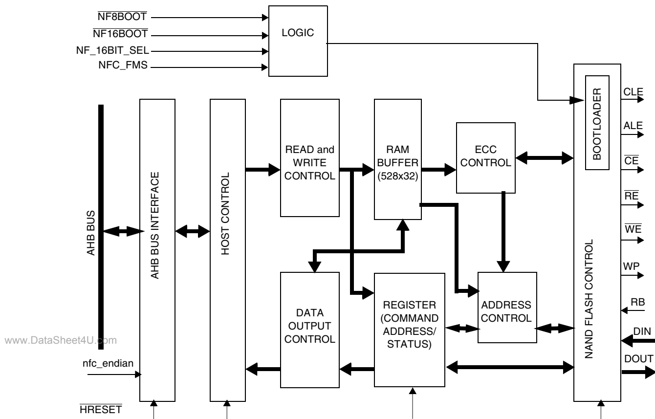
Figure 19-1. NAND Flash Controller Block Diagram
