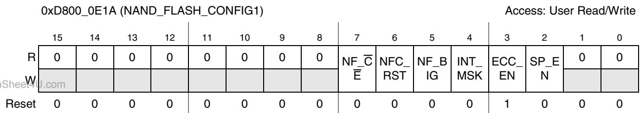
Figure 19-18. NAND_FLASH_CONFIG1 Register
