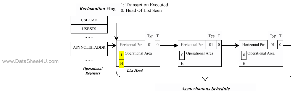
Figure 30-60. Asynchronous Schedule List w/Annotation to Mark Head of List
