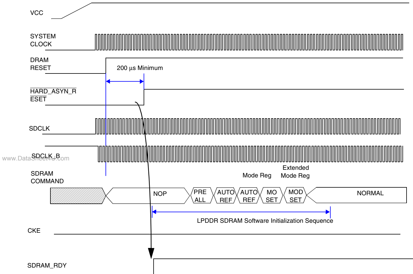
Figure 18-81. Simplified LPDDR SDRAM Initialization and Load Mode Register Sequence
