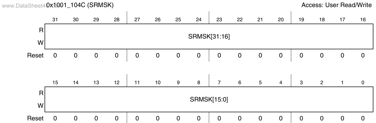
Figure 42-40. SSI Receive Time Slot Mask Register
