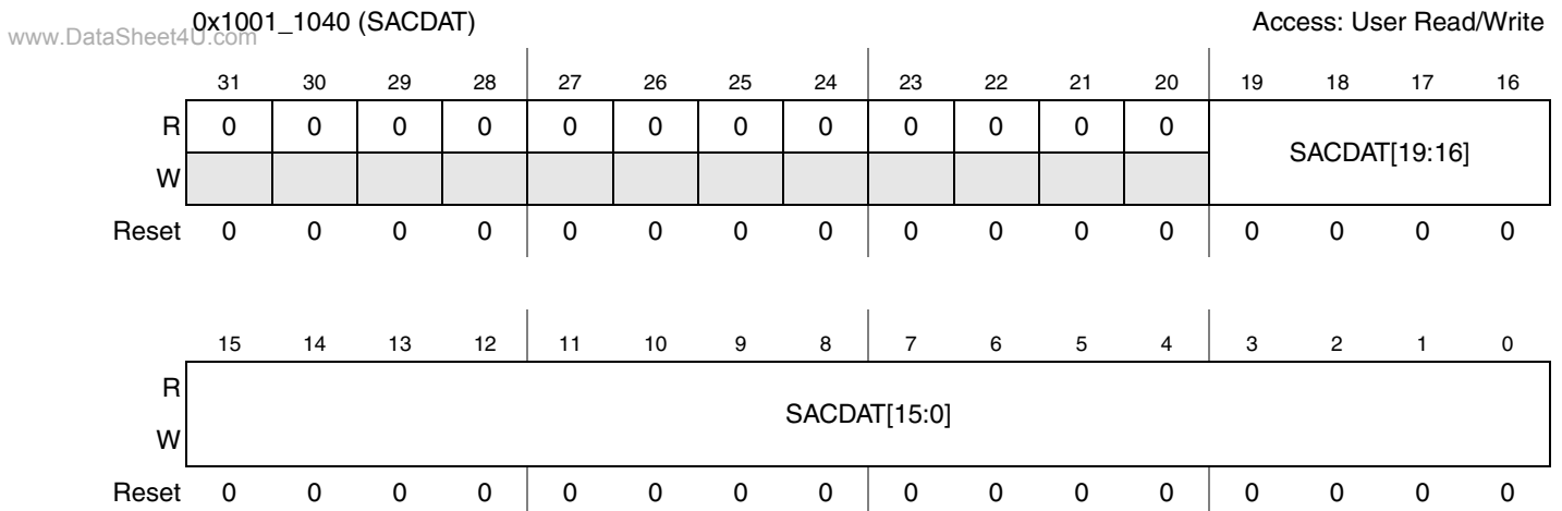
Figure 42-37. SSI AC97 Command Data Register
