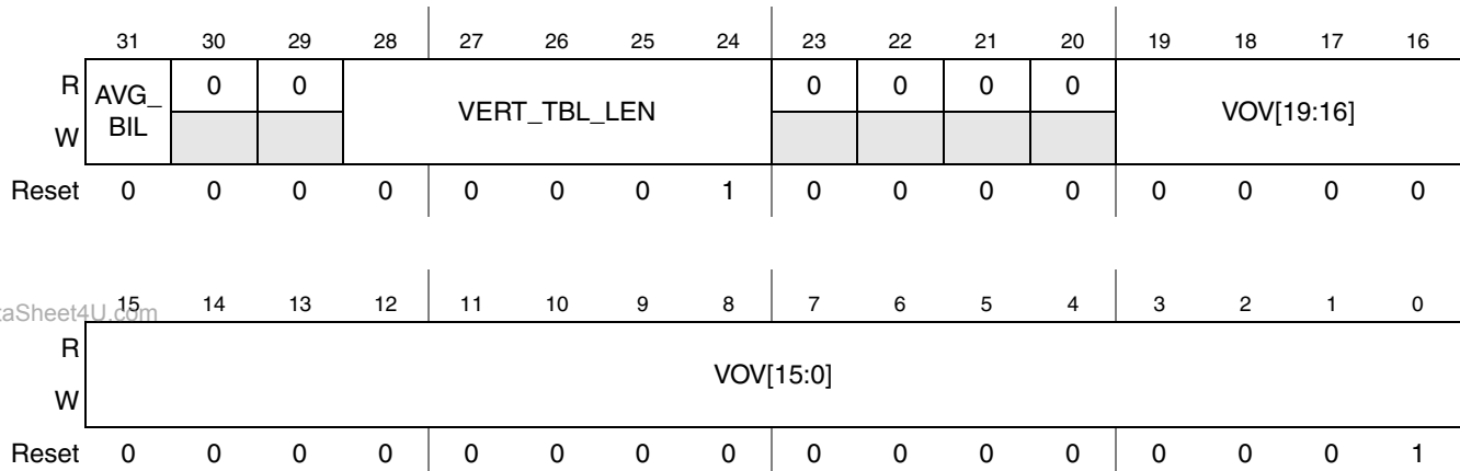
Figure 41-60. PrP Channel2 Vertical Resize Valid
