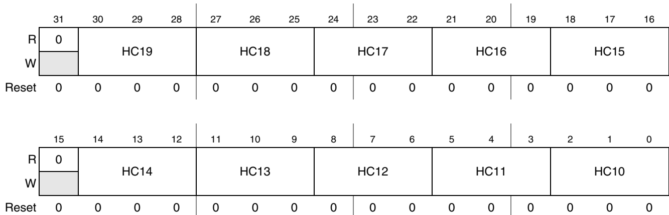
Figure 41-56. PrP Channel-2 Horizontal Resize Coefficient 2
