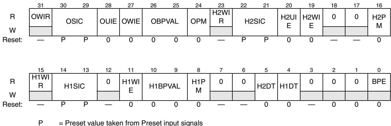
Figure 30-2. USB Control Register
