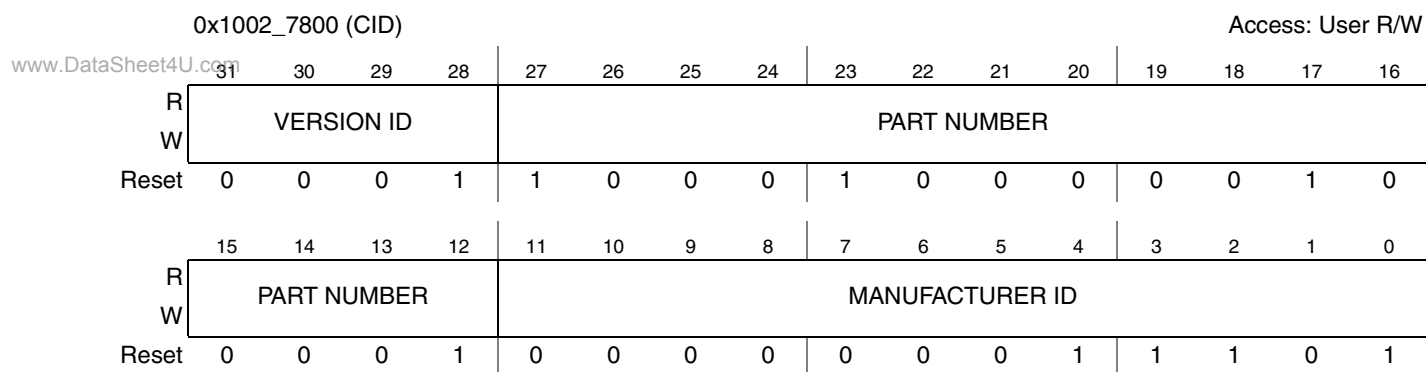
Figure 4-2. Chip ID Register (CID)
