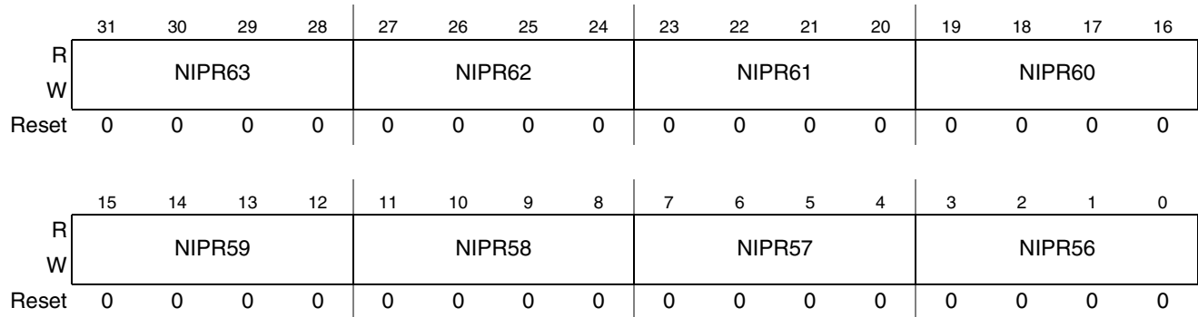
Figure 10-11. Normal Interrupt Priority Level 7 Register Format
