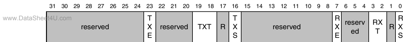
Figure 30-40. ENDPTCTRL0—Endpoint Control 0
