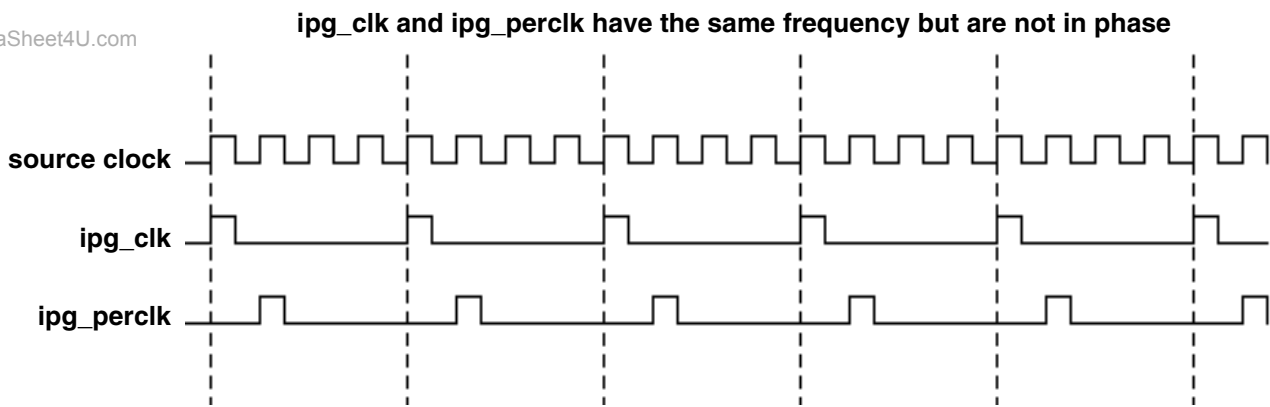
Figure 28-20. Examples of Working Relationships Between ipg_clk and ipg_perclk
