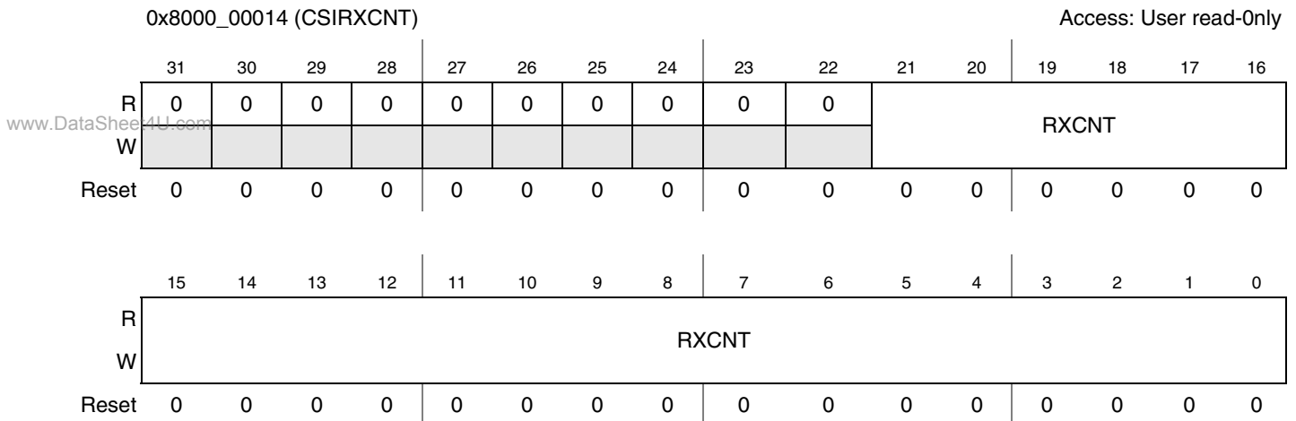
Figure 39-15. CSI RX Count Register (CSIRXCNT)
