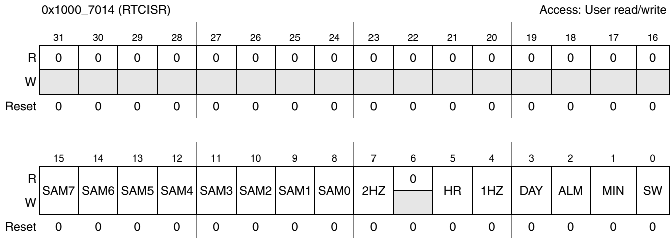
Figure 33-8. RTC Interrupt Status Register
