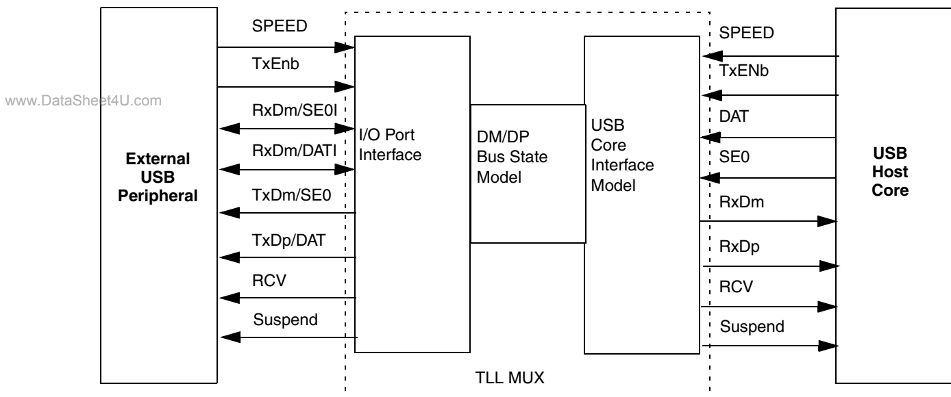
Figure 30-4. TLL Mux Functional Diagram
