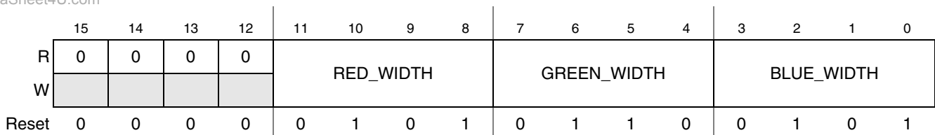
Figure 41-42. PrP CH1 Pixel Format Control Register
