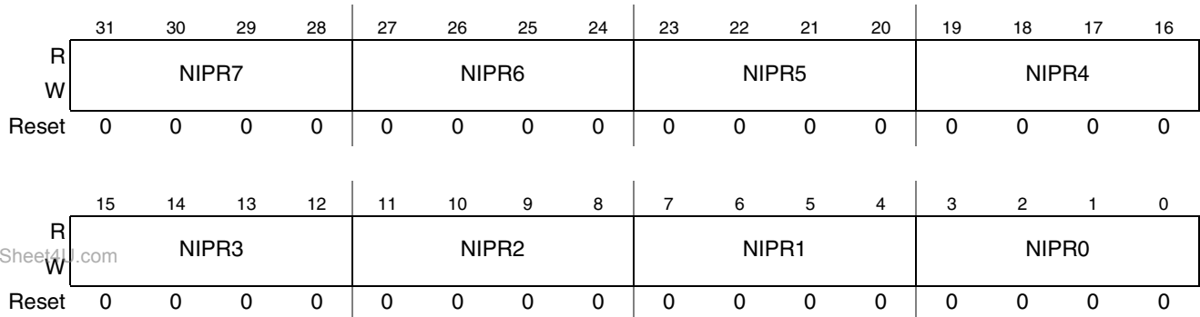
Figure 10-18. Normal Interrupt Priority Level 1 Register Format
