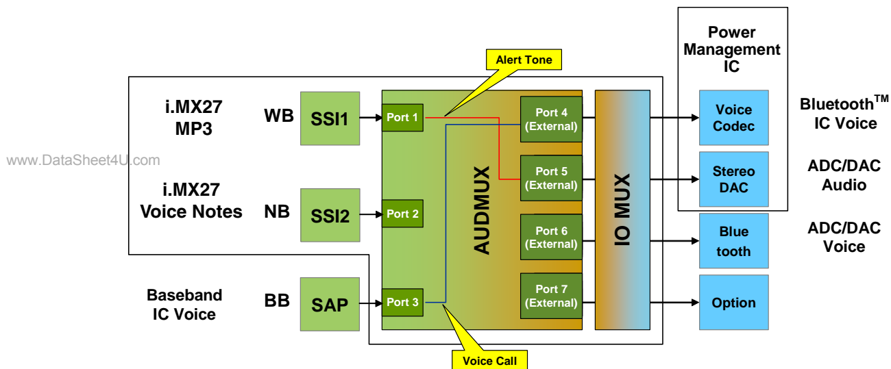
Figure 1-7. Typical AUDMUX Application
