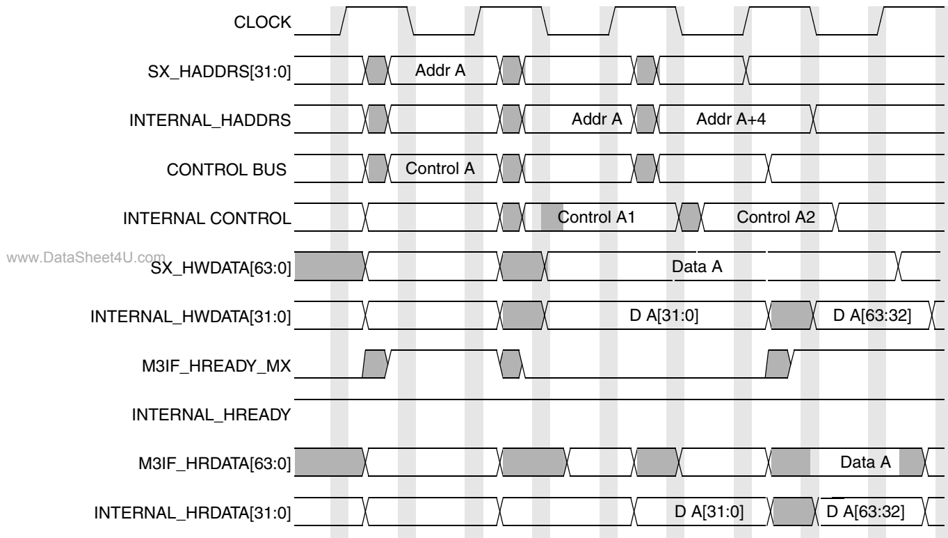
Figure 16-20. MPG64 Simple Double Word Transfer
