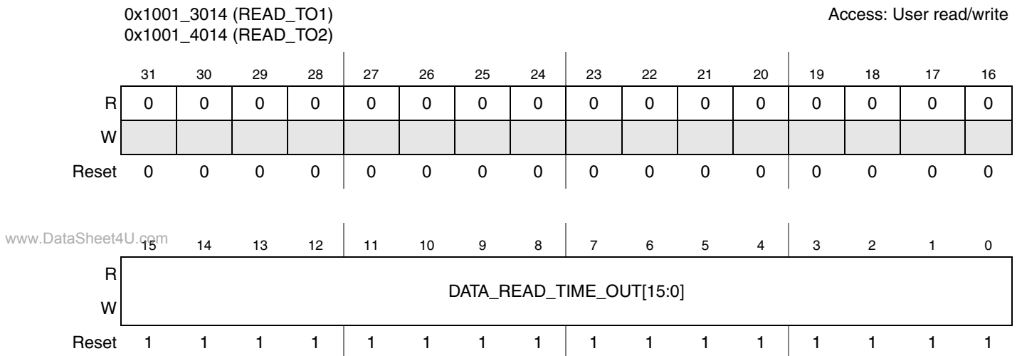
Figure 27-9. SDHC Read Time Out Register
