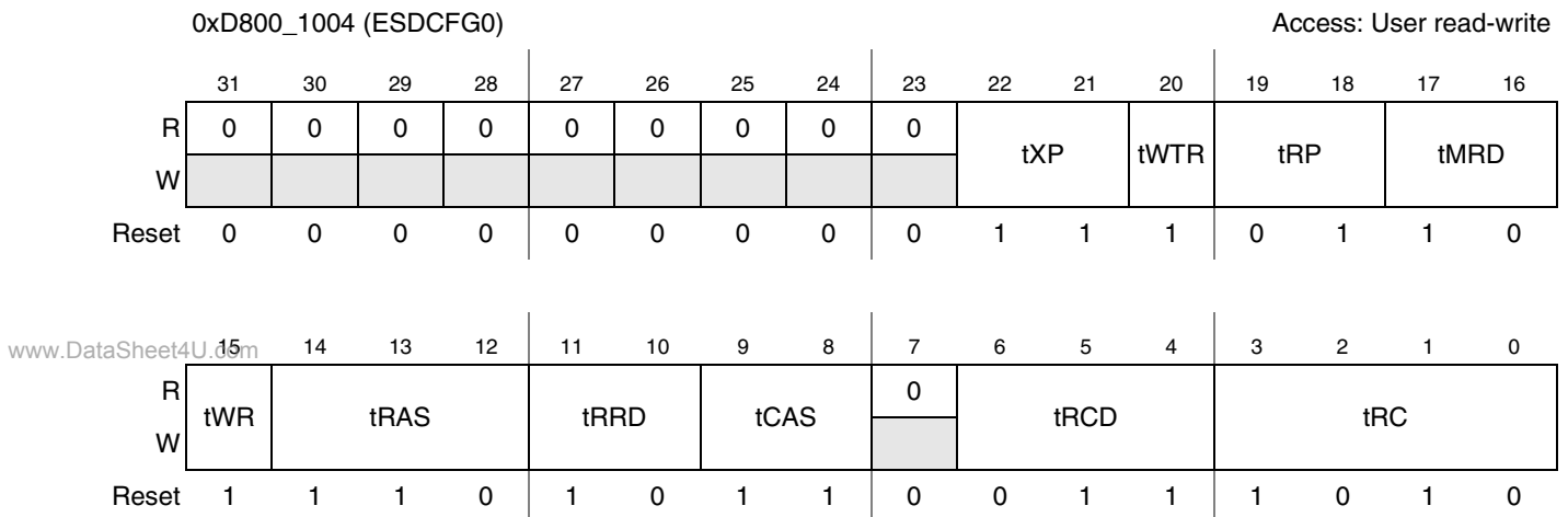
Figure 18-6. Enhanced SDRAM Configuration Register 0 (ESDCFG0)
