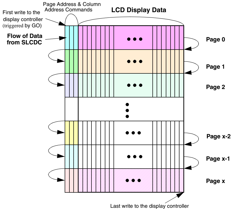
Figure 44-10. SLCDC Automatic Mode Data Flow (AUTOMODE[1:0] = 10)
