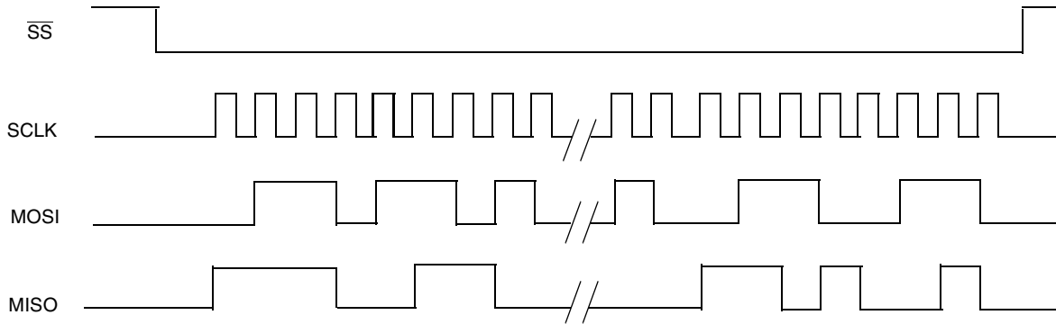
Figure 23-7. SPI continuous transfer with BURST=1
