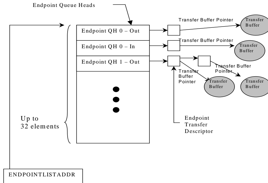
Figure 30-76. End Point Queue Head Diagram
