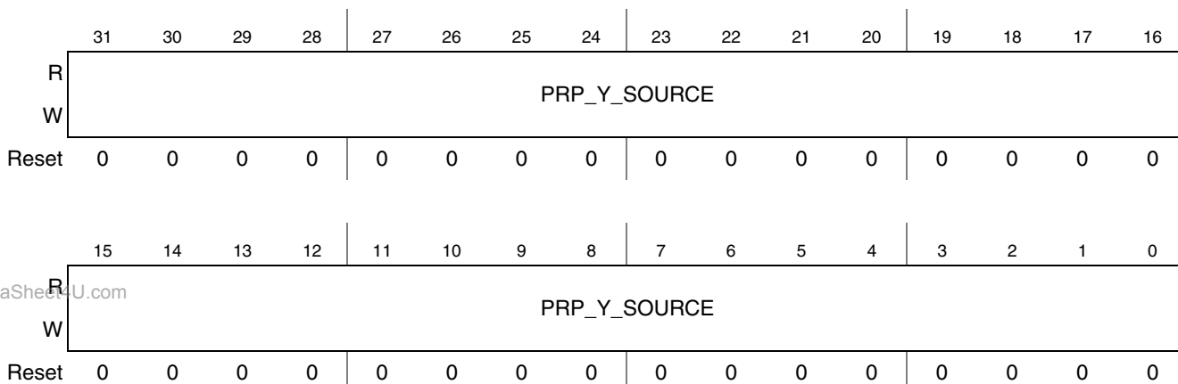
Figure 41-31. PrP Source Y Address Register
