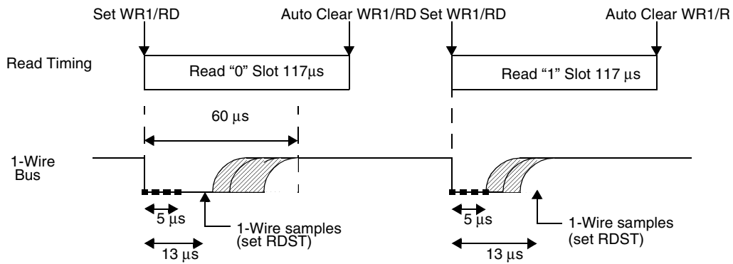
Figure 21-6. Read Timing
