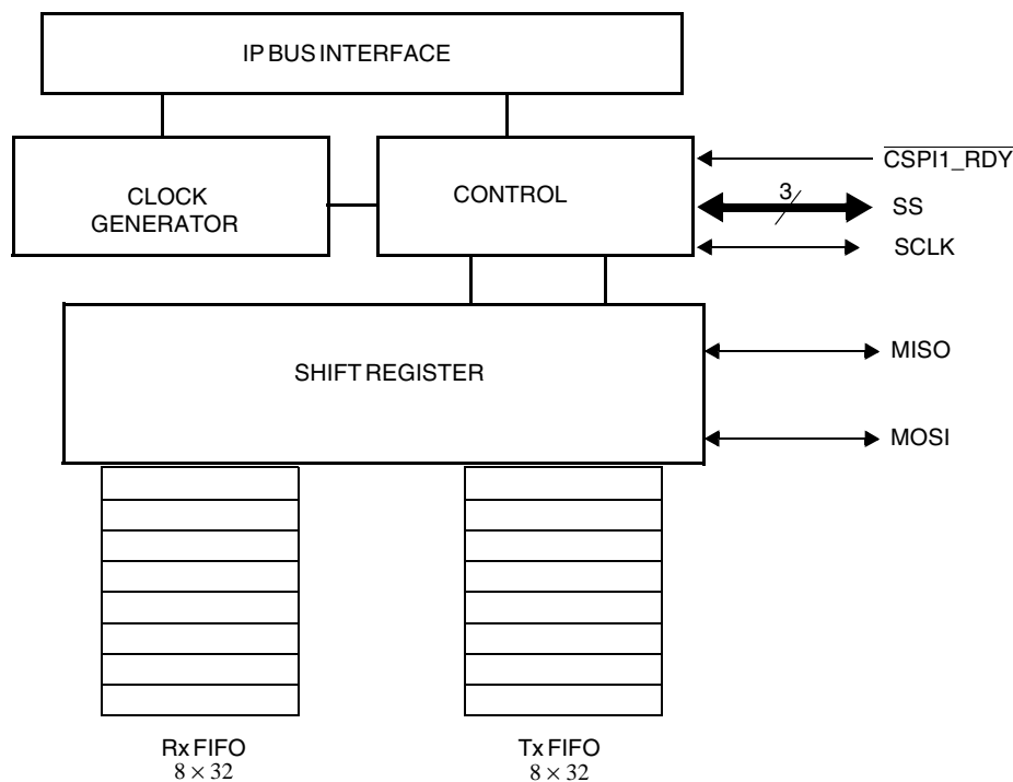
Figure 23-1. Configurable Serial Peripheral Interface Block Diagram
