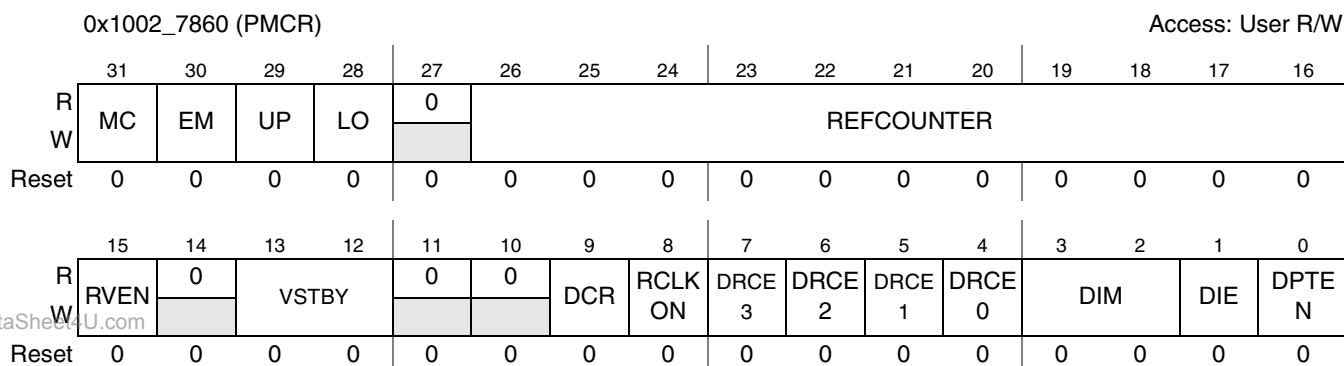
Figure 4-21. Power Management Control Register (PMCR)
