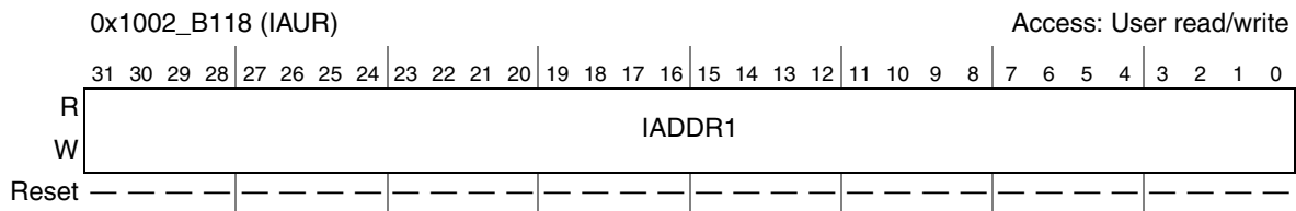
Figure 29-17. IAUR Register
