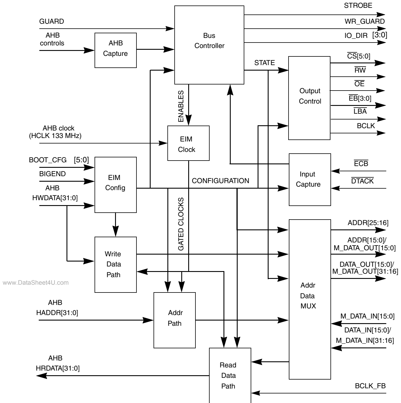
Figure 17-1. WEIM Block Diagram
