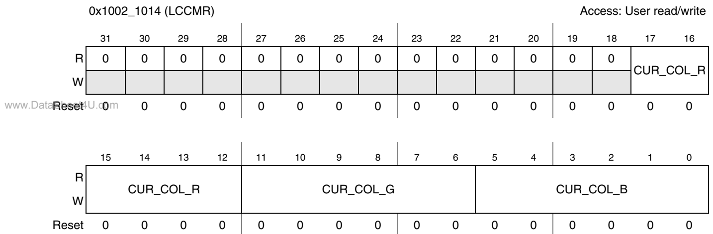
Figure 43-28. LCDC Color Cursor Mapping Register (LCCMR)
