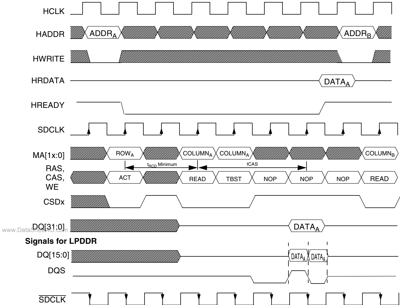
Figure 18-48. SDR and LPDDR Off-Page Single Read Timing Diagram (32-Bit Memory for SDR and 16-Bit for LPDDR)
