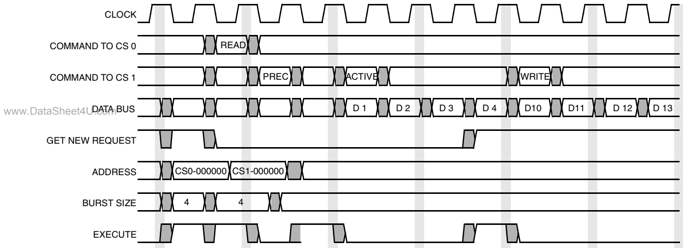
Figure 18-33. SDR Miss Write to CSD1 after Read from CSD0
