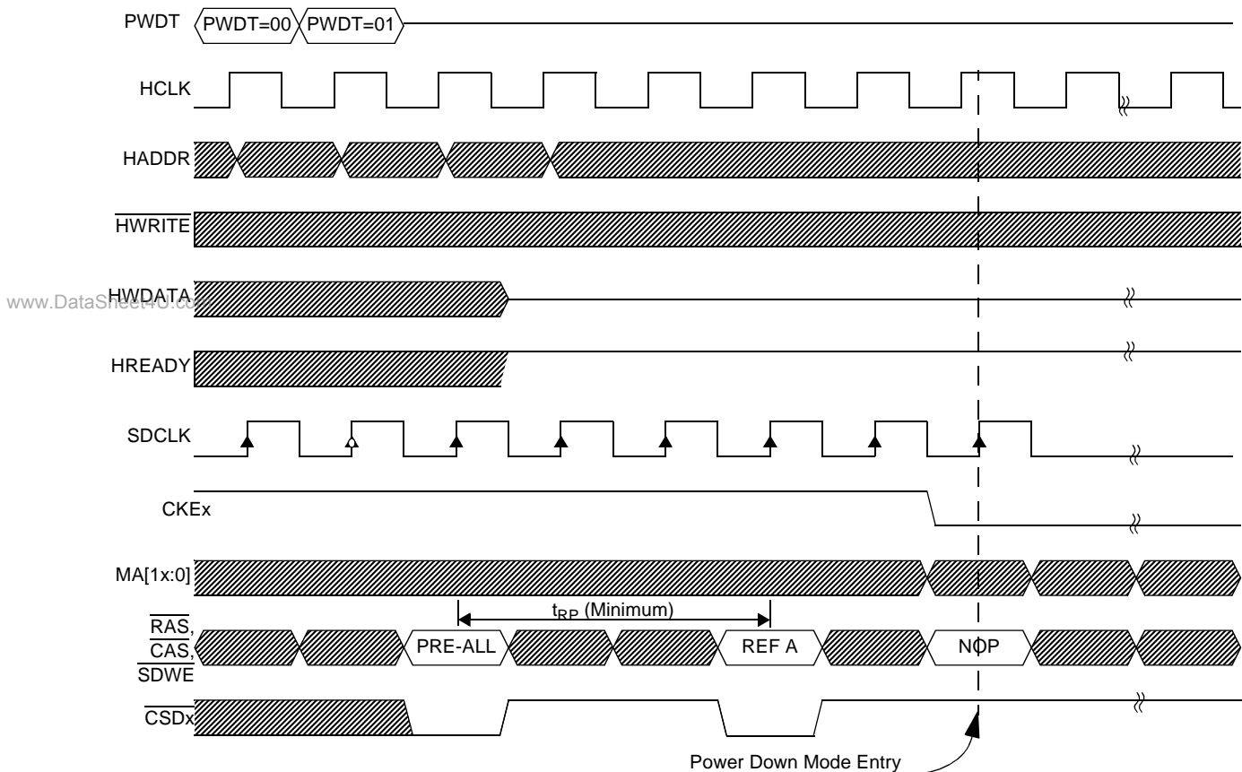
Figure 18-41. SDR SDRAM Precharge Power Down Mode Entry Timing Diagram
