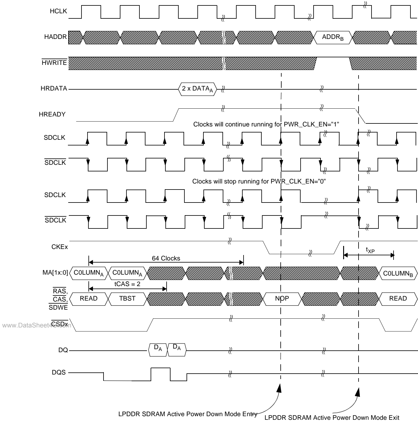
Figure 18-46. Mobile DDR SDRAM Active Power Down Mode Timing Diagram
