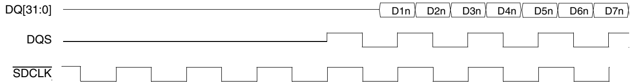
Figure 18-59. AHB 64-Bit Write to LPDDR: Off-Page Burst Write Timing Diagram (32-Bit Memory)
