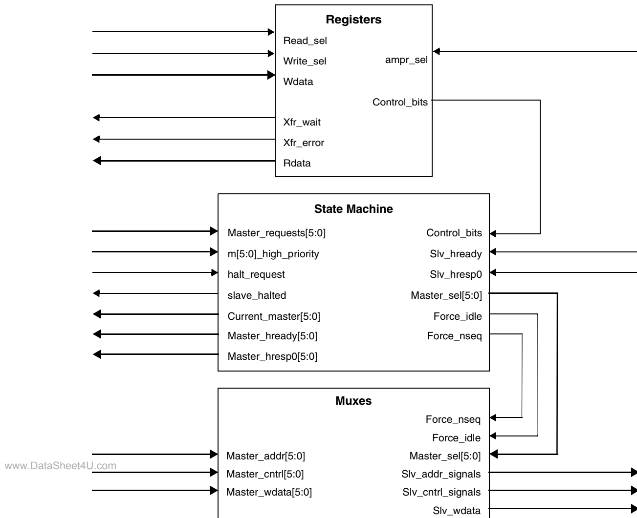
Figure 36-7. MAX Slave Port Block Diagram
