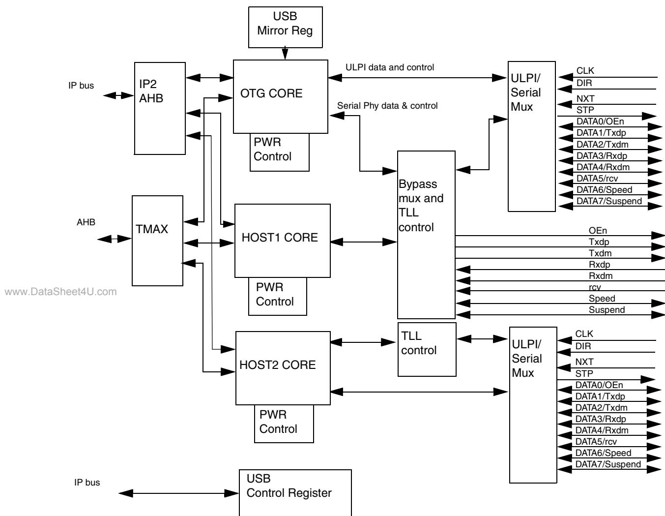
Figure 30-1. USB Block Diagram
