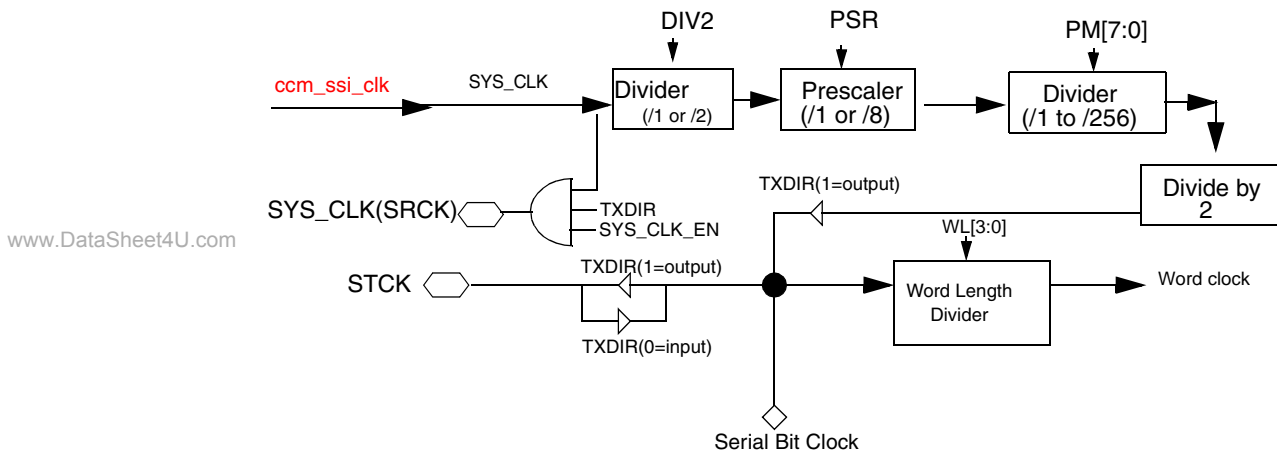
Figure 42-45. SSI Transmit Clock Generator Block Diagram
