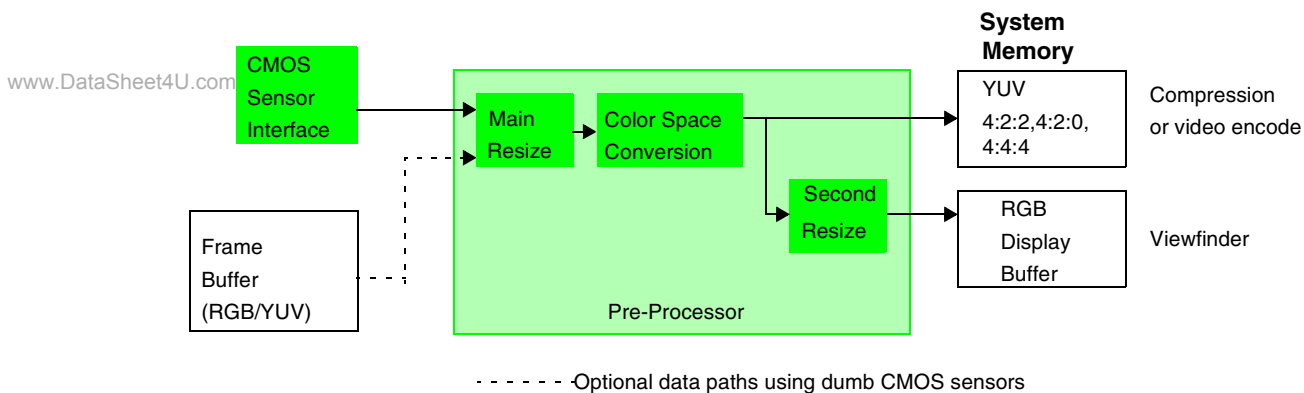
Figure 1-5. Pre-Processor Data Flow
