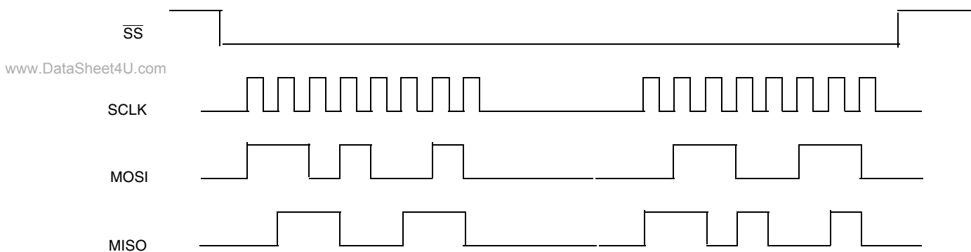
Figure 23-8. SPI Transfer while SSCTL is Clear
