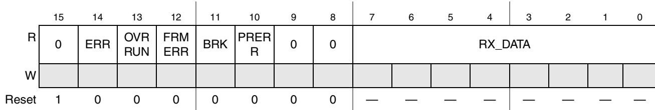
Figure 28-4. UART Receiver Register (URXD)
