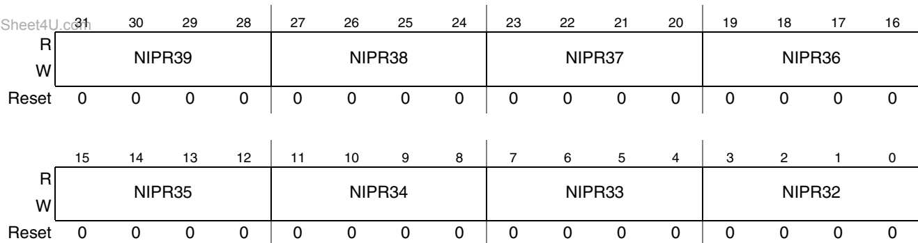
Figure 10-14. Normal Interrupt Priority Level 4 Register Format
