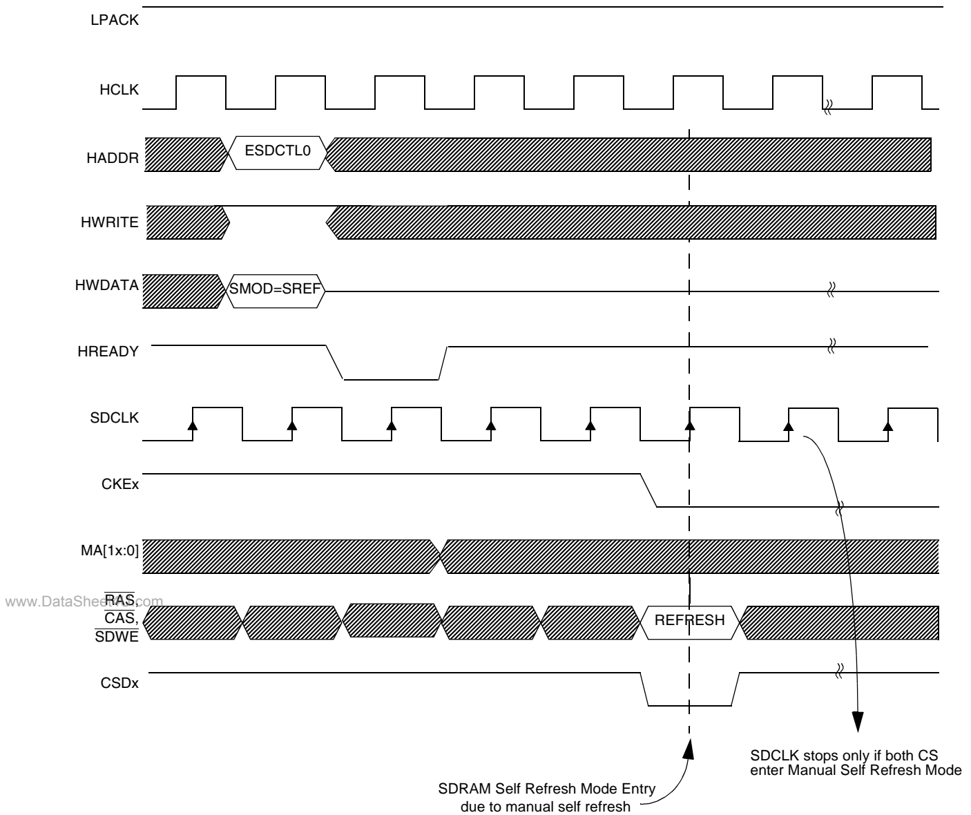
Figure 18-39. Manual Self Refresh Entry Timing Diagram
