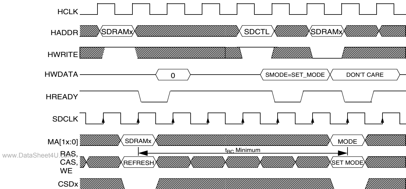
Figure 18-78. Set Mode Register State Diagram
