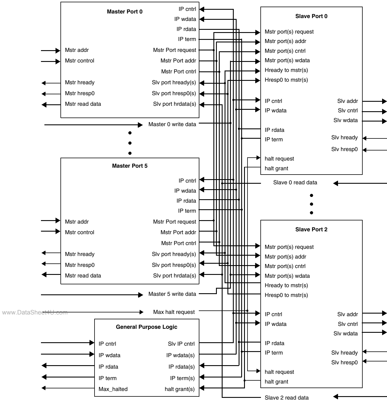
Figure 36-1. MAX Block Diagram
