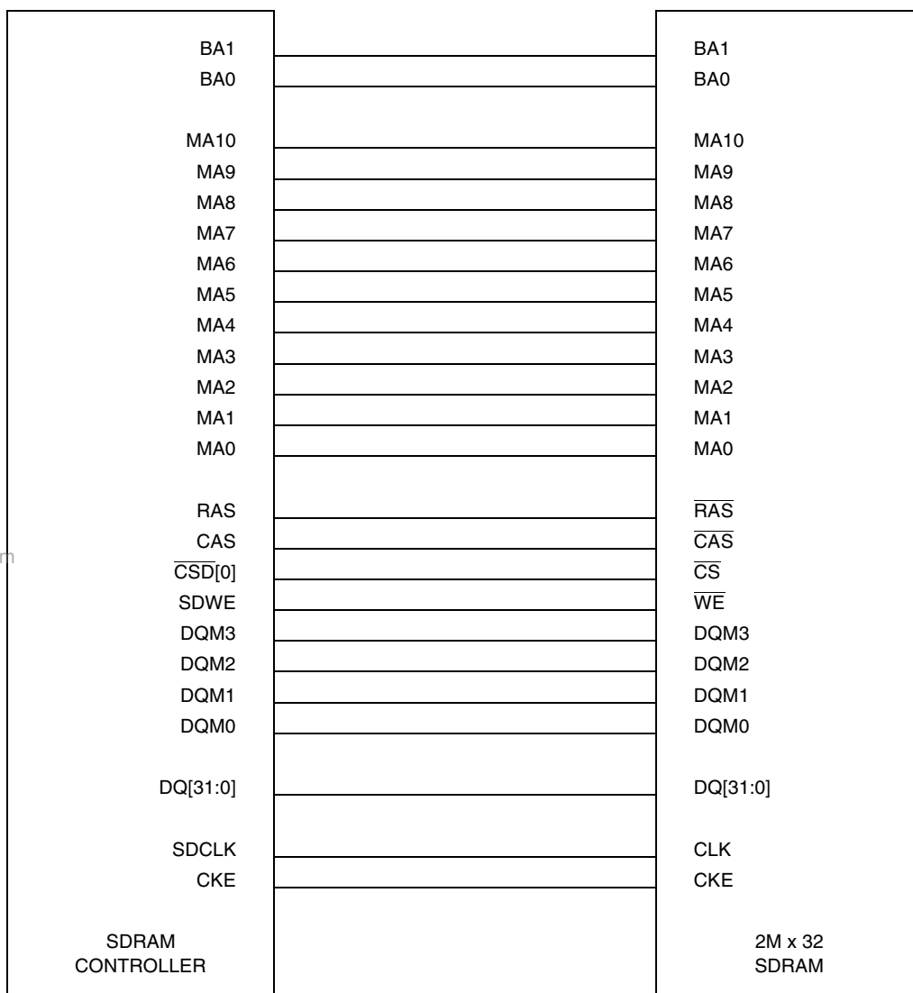
Figure 18-91. Single 64-Mbyte (2MBx32) SDRAM Connection Diagram
