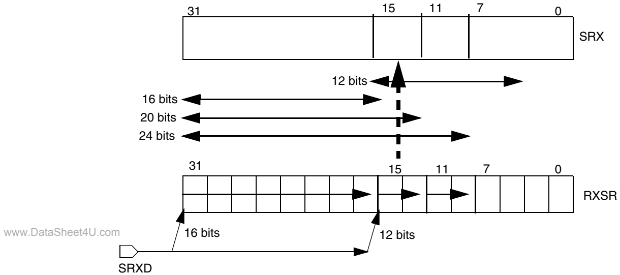
Figure 42-22. Receive Data Path (RXBIT0=0, RSHFD=1) (MSB Alignment)
