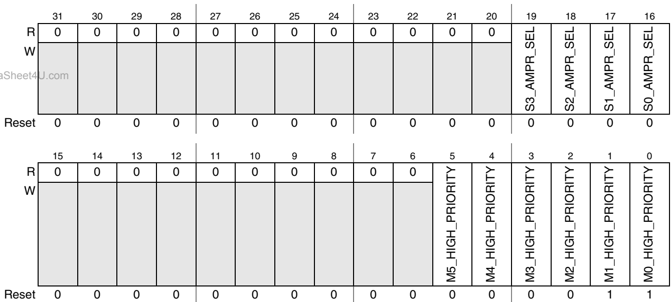
Figure 4-20. Priority Control and Select Register (PCSR)
