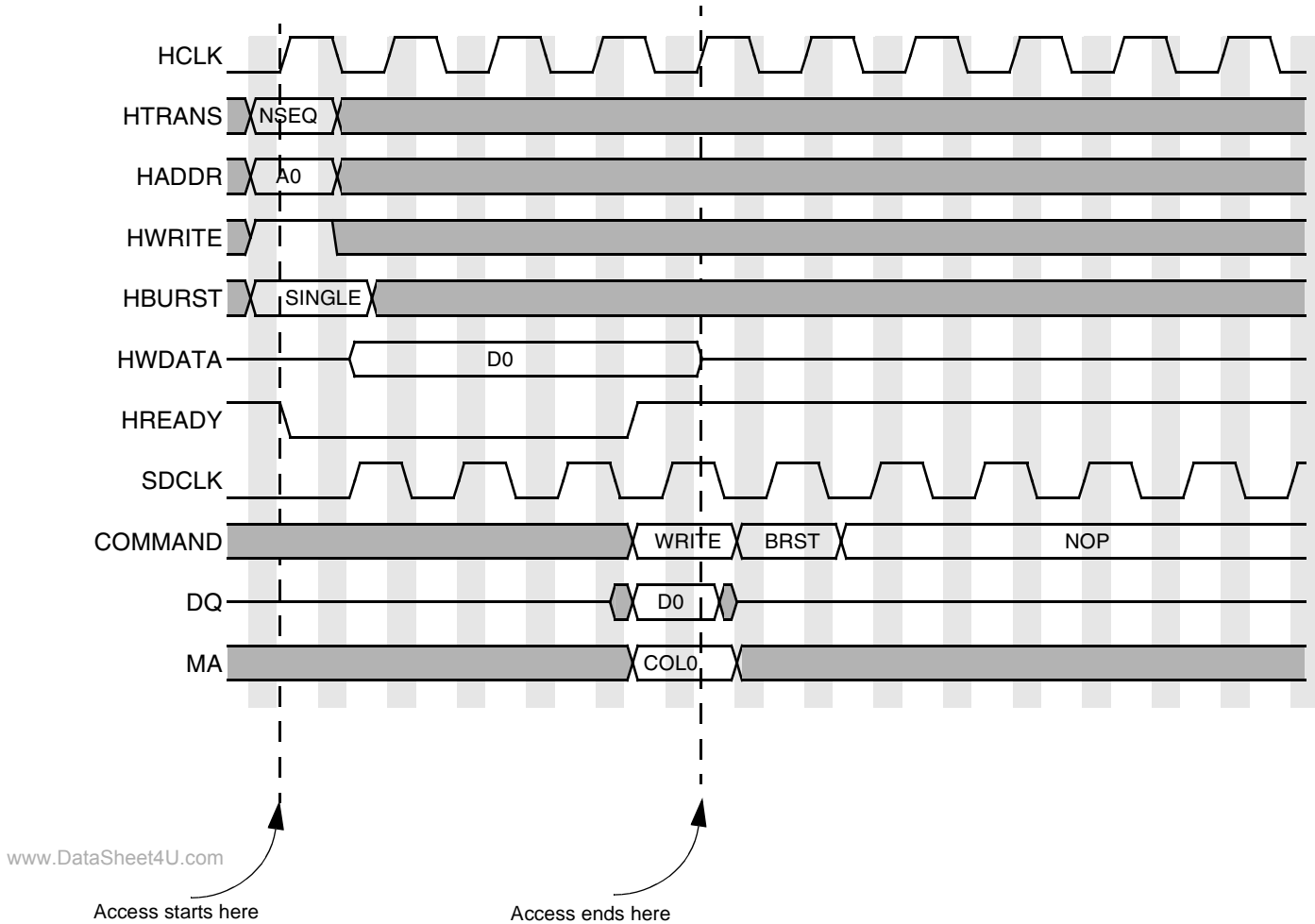
Figure 18-73. Single on Page Write—Word Access to 32-Bit Memory (Cycle Accurate)
