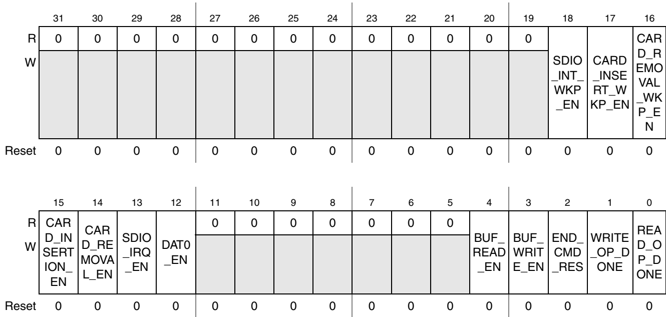
Figure 27-13. SDHC Interrupt Control Register
