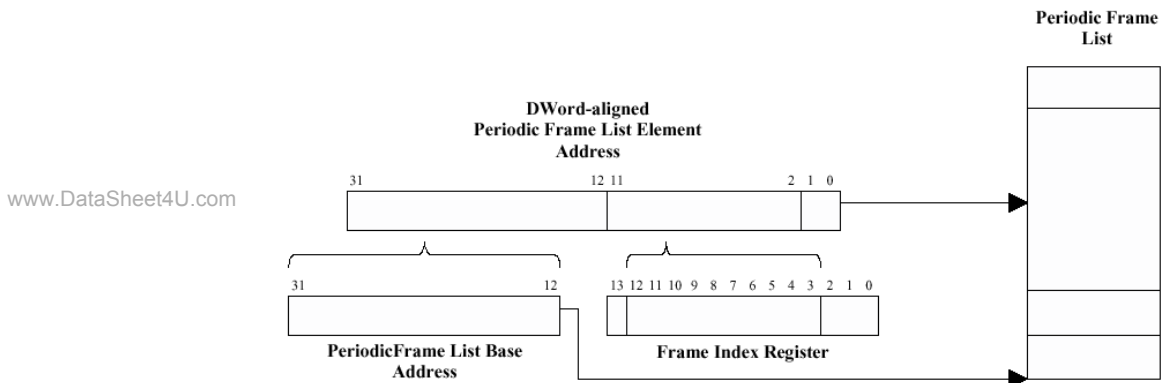
Figure 30-52. Derivation of Pointer into Frame List Array
