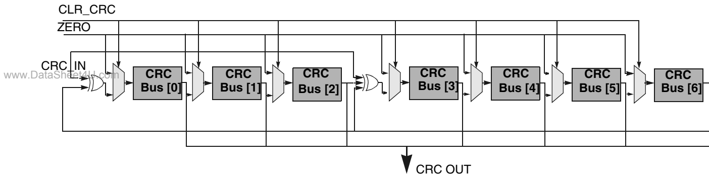
Figure 27-25. Command CRC Shift Register (DATs Has Similar Structure)
