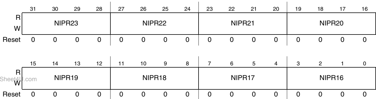
Figure 10-16. Normal Interrupt Priority Level 2 Register Format
