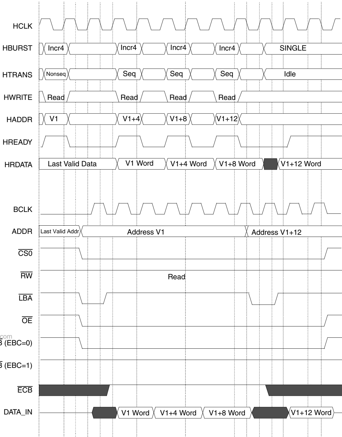
Figure 17-37. Increment 4 AHB Read Access, WSC=2, SYNC=1, DOL=1, WRAP=1, PSZ=0
