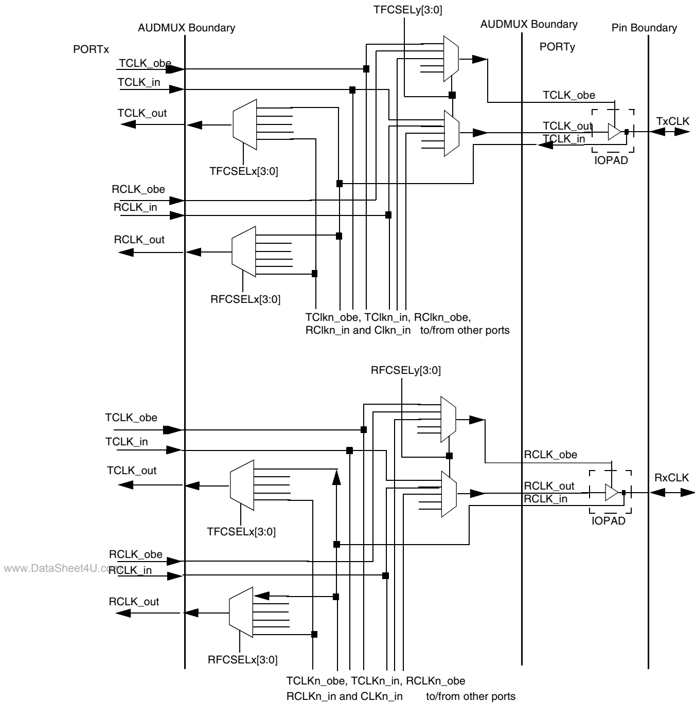
Figure 38-6. Clock Routing when Peripheral Port is 6-Wired
