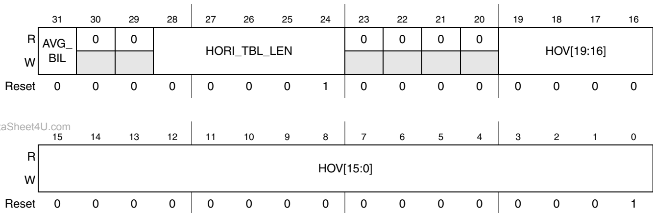
Figure 41-51. PrP Channel-1 Resize Horizontal Valid
