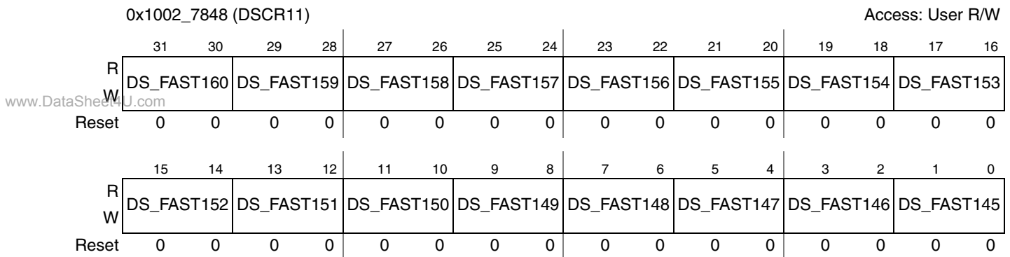
Figure 4-16. Drive Strength Control Register 11 (DSCR11)
