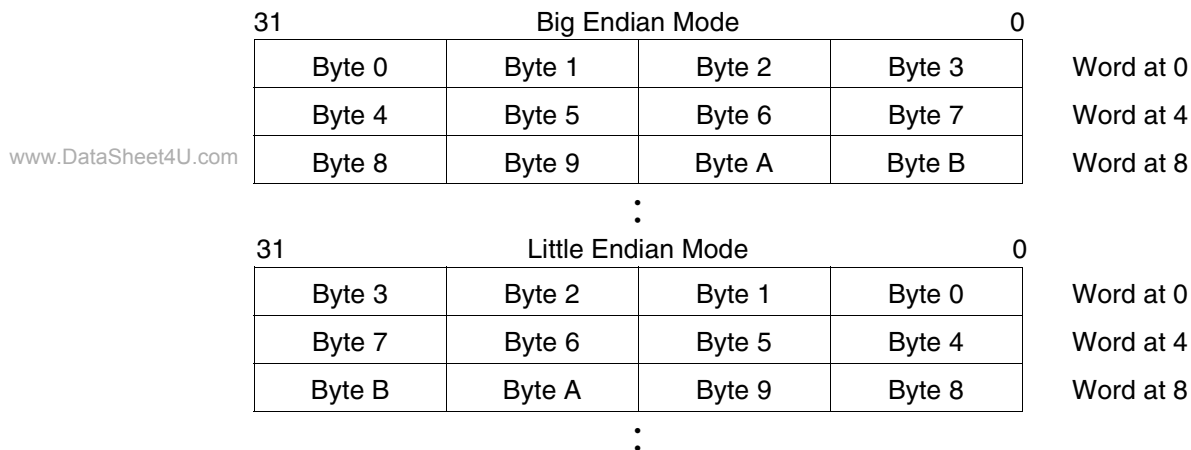
Figure 18-3. Data Organization in Memory
