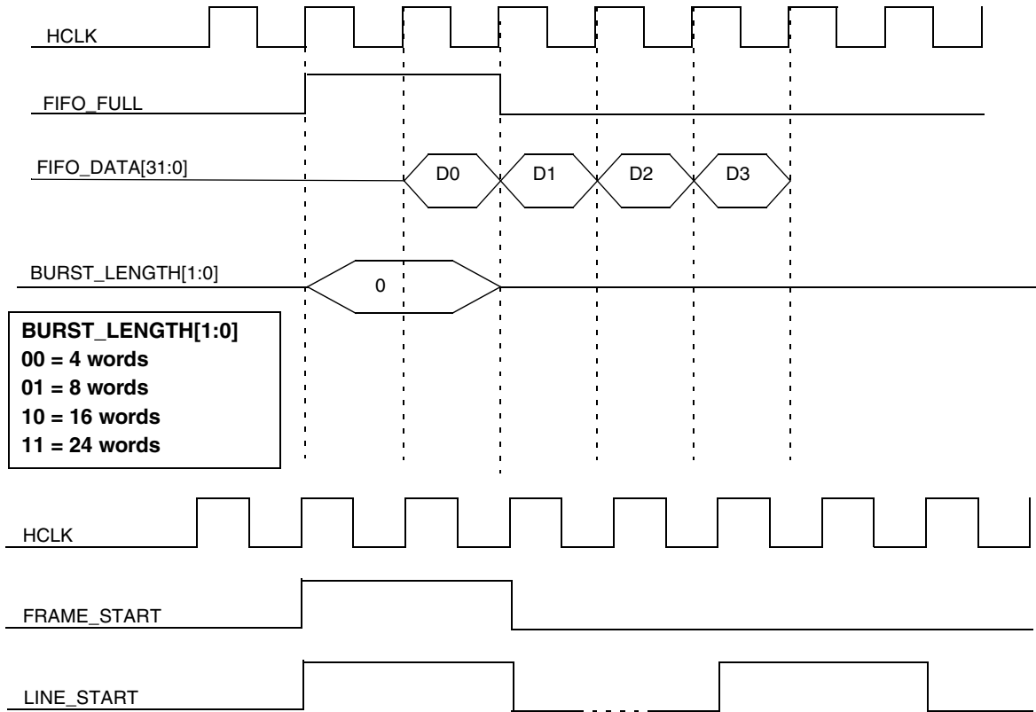
Figure 41-27. CSI-PrP Link
