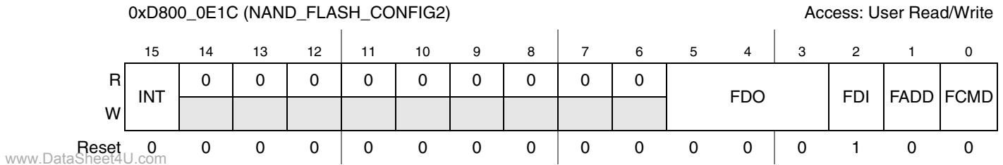
Figure 19-19. NAND_FLASH_CONFIG2 Register
