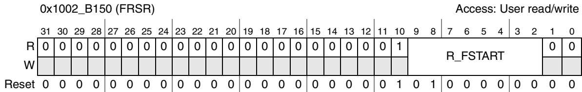
Figure 29-23. FRSR Register
