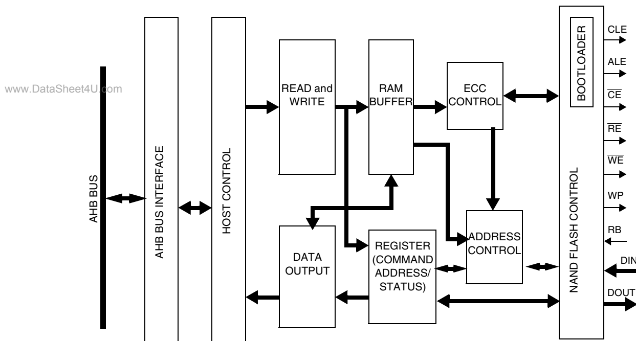
Figure 15-3. NAND Flash Controller Simplified Block Diagram
