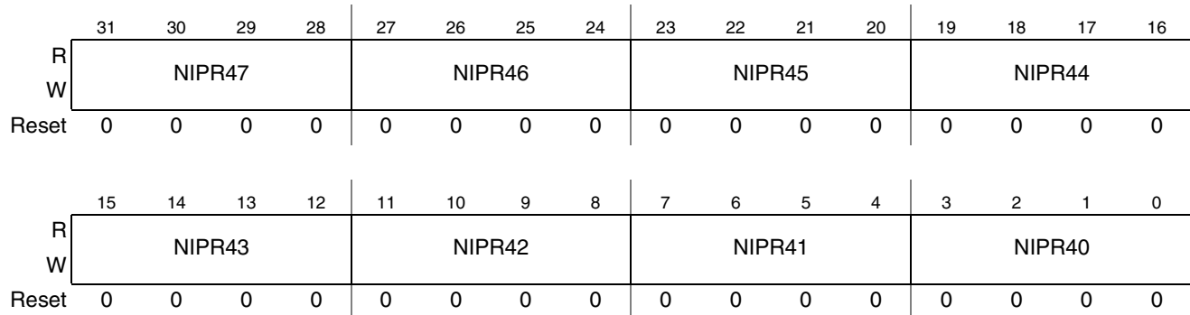
Figure 10-13. Normal Interrupt Priority Level 5 Register Format
