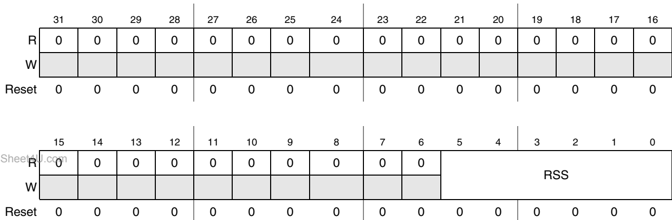
Figure 37-22. Channel Request Source Select Registers (RSSR0–RSSR15)
