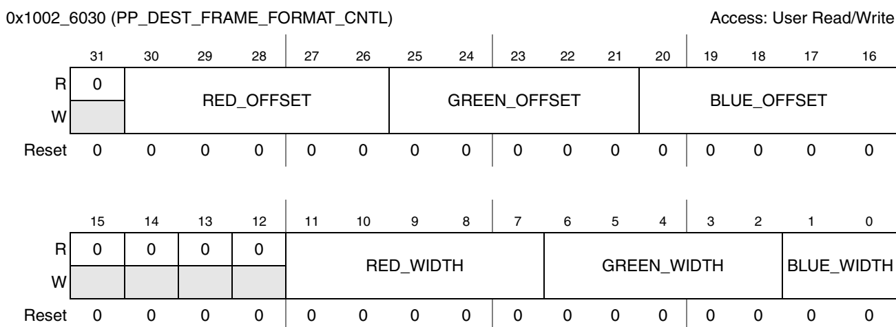
Figure 41-19. PP Destination Frame Format Control Register
