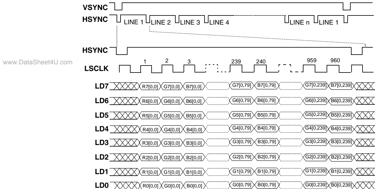
Figure 43-18. LCDC Interface 24-bpp Timing For AUS Mode
