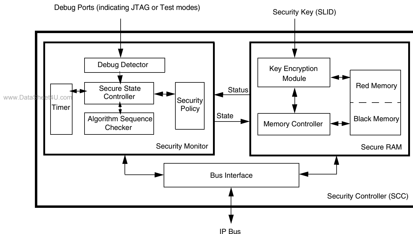
Figure 11-1. Security Controller Block Diagram
