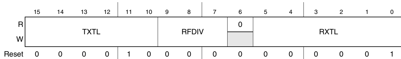
Figure 28-10. UART FIFO Control Register (UFCR) Summary
