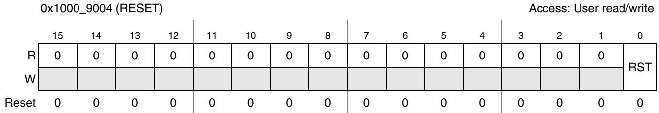
Figure 21-10. Reset Register
