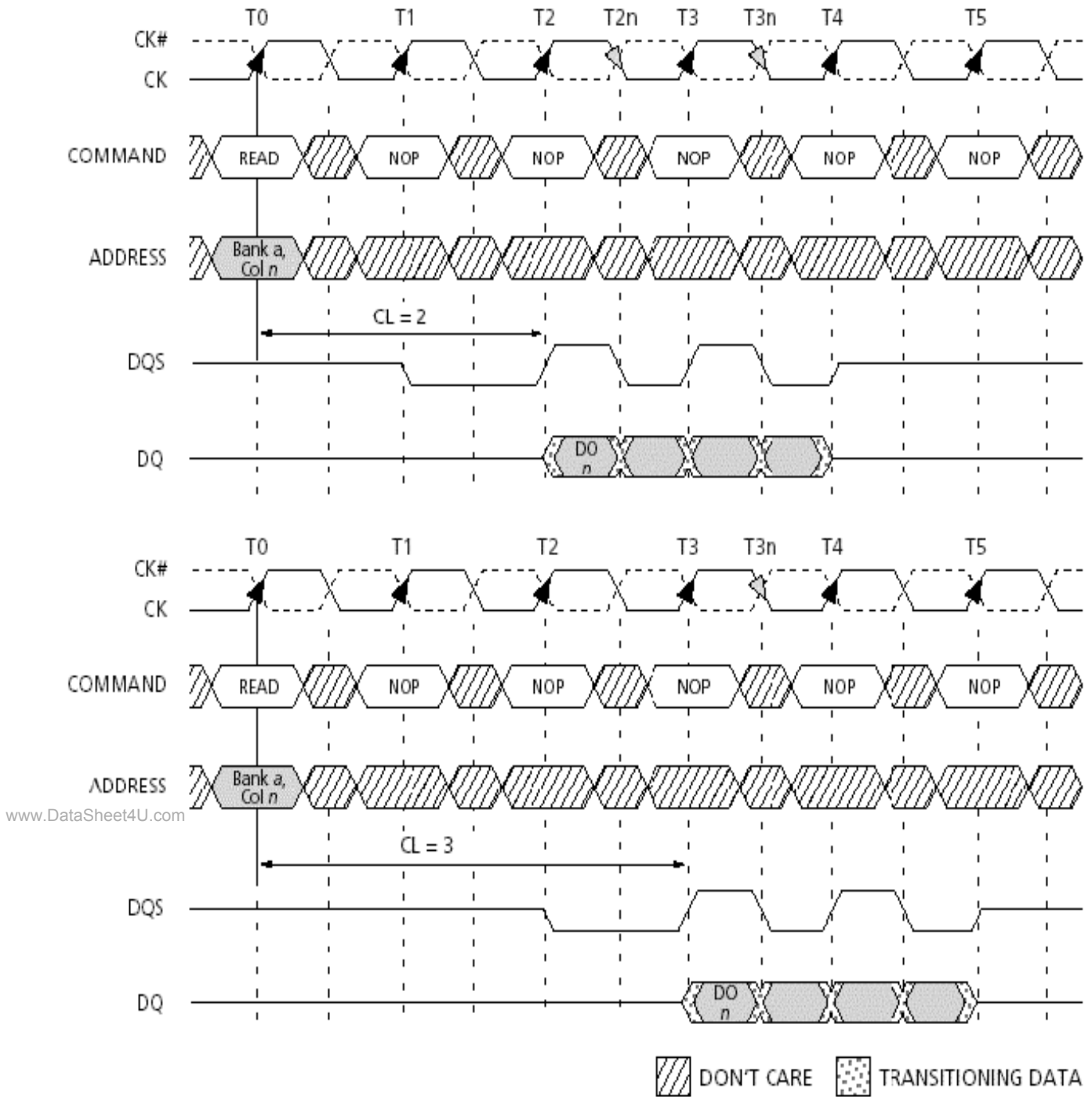
Figure 18-16. Mobile LPDDR CAS Latency Timing
