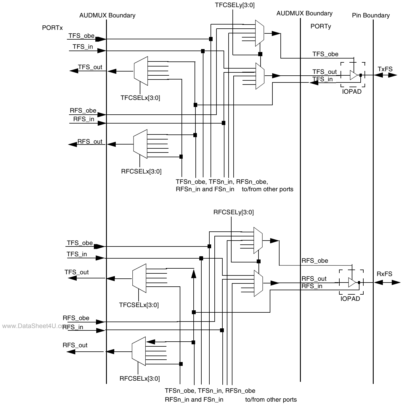
Figure 38-5. Frame Sync Routing when Peripheral Port is 6-Wired
