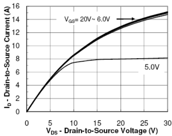
Figure1.Output Characteristic
