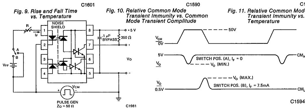
Fig. 12. Test Circuit for Transient Immunity and Typical Waveforms
