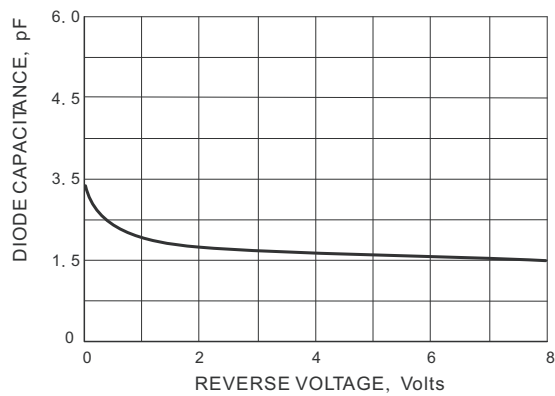
Fig.3-TYPICALCAPATICANCE
