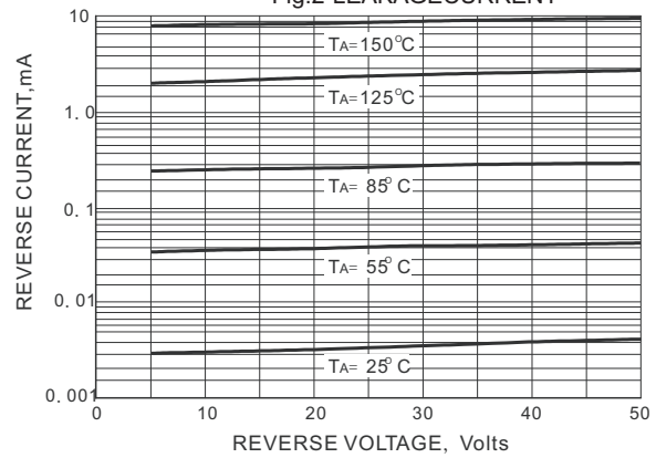
Fig.2-LEAKAGECURRENT
