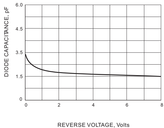
TYPICAL CAPATICANCE
