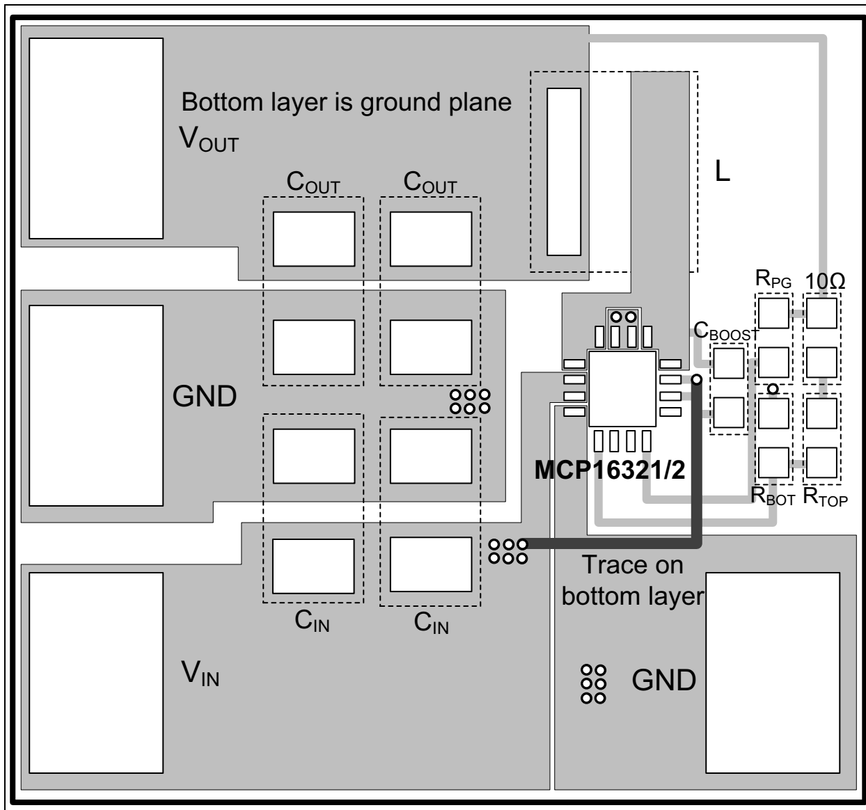
FIGURE 5-1: Recommended Layout.
