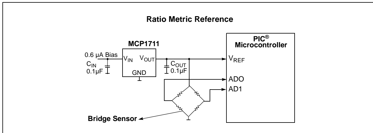
FIGURE 5-2: Using the MCP1711 as a Voltage Reference.
