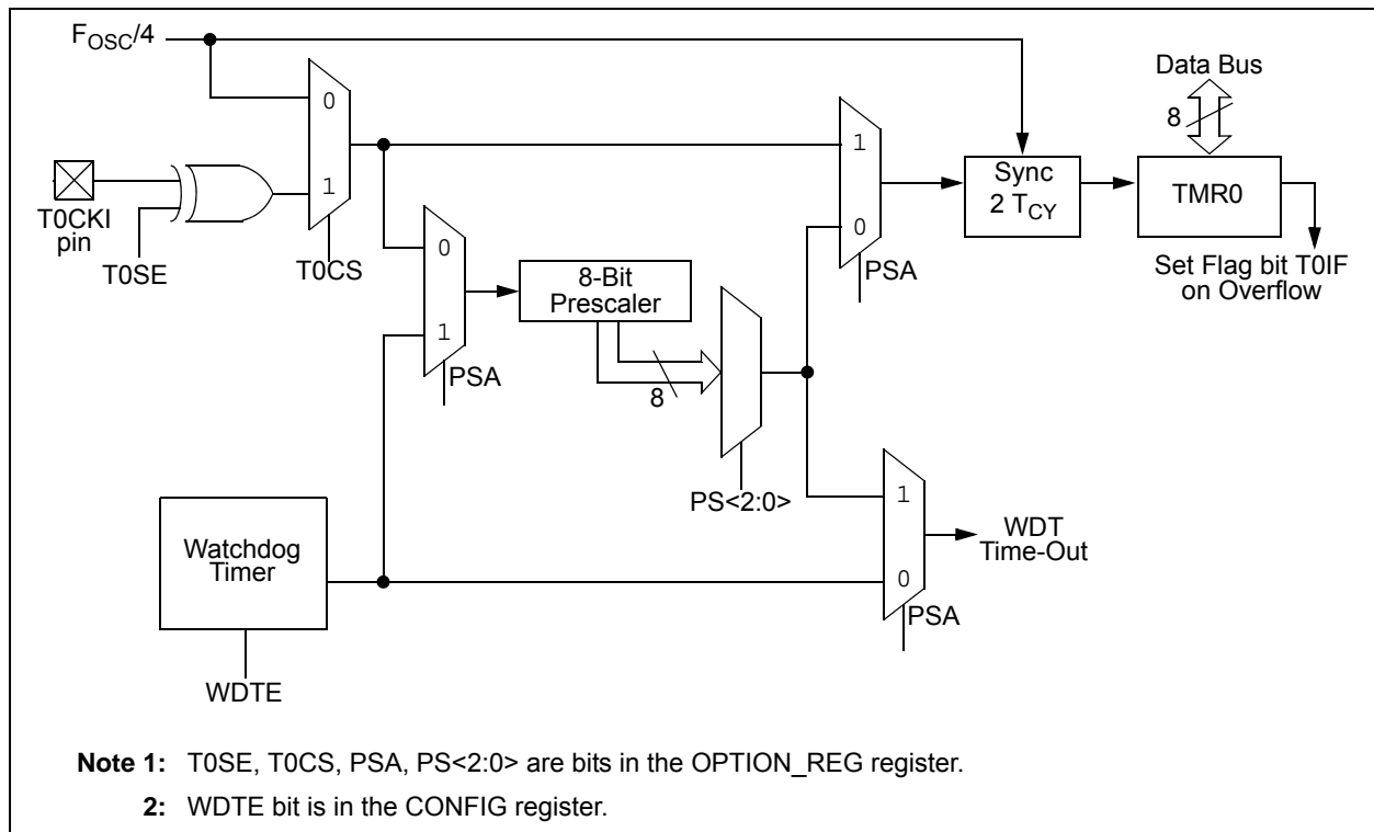
FIGURE 14-1: WATCHDOG TIMER WITH SHARED PRESCALE BLOCK DIAGRAM
