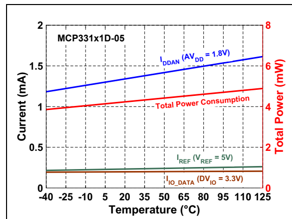
FIGURE 3-36: Power Consumption vs. Temperature.
