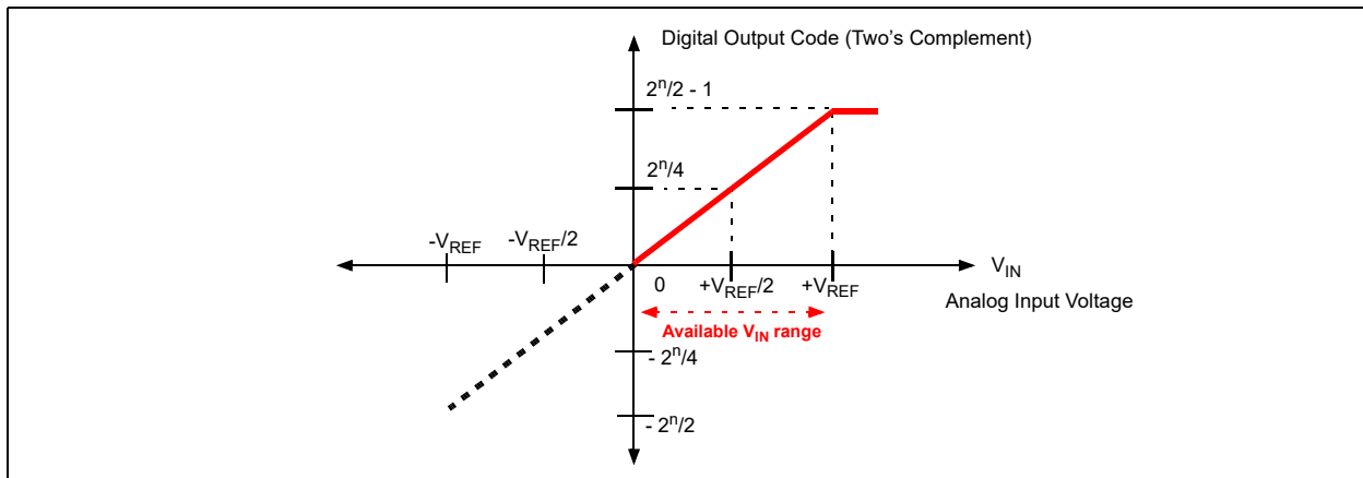
FIGURE 6-8: Transfer Function for Figure 6-7. See the output code example in Table 6-8.
