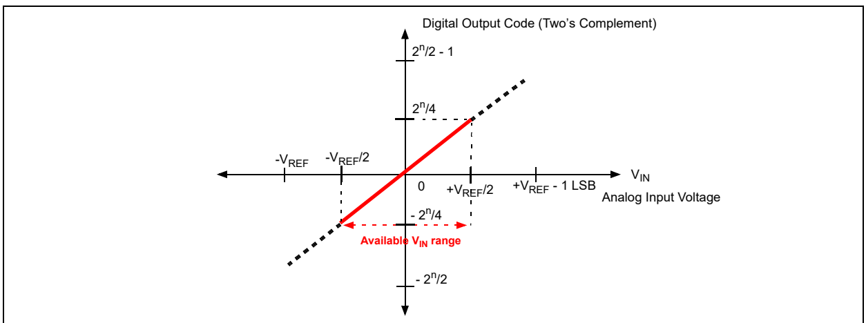
FIGURE 6-6: Transfer Function for Figure 6-5. See the output code example in Table 6-7.
