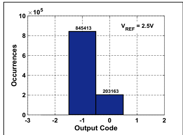
FIGURE 4-29: Shorted Input Histogram: V_{REF} = 2.5\text{V} .
