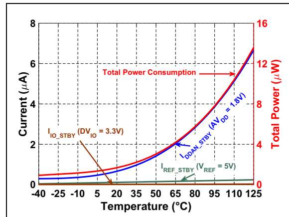
FIGURE 3-34: Power Consumption vs. Temperature during Shutdown.
