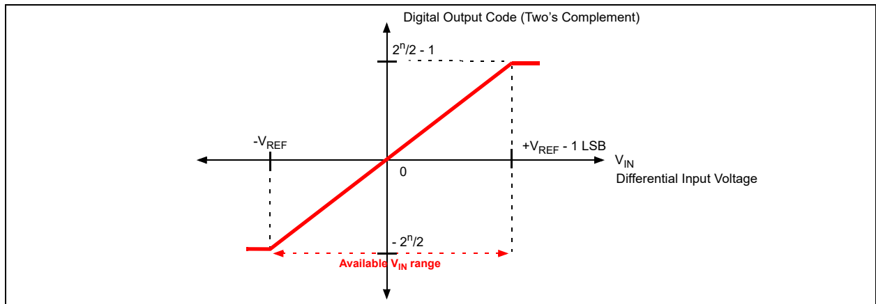
FIGURE 6-3: Transfer Function for Figure 6-7. See the output code example in Table 6-7.
