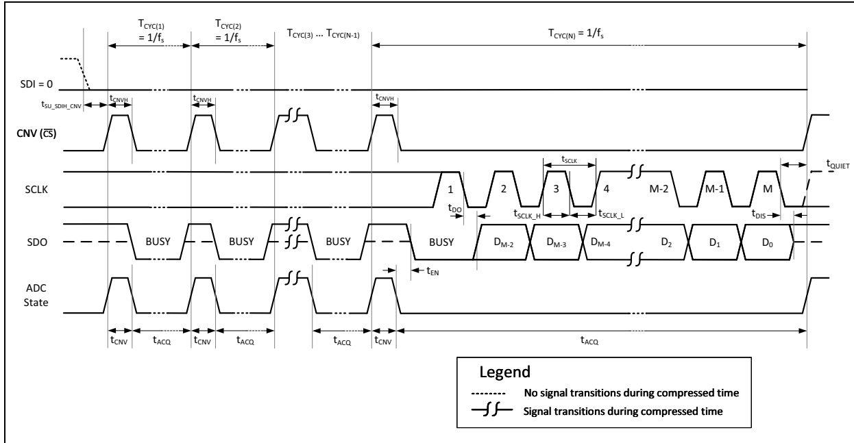
FIGURE 6-6: Timing Diagram for 3-Wire \overline{CS} Mode with BUSY Status indicator Output Bit, Early CNV (Recommended).
