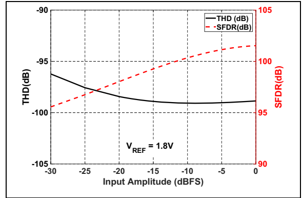
FIGURE 3-28: THD/SFDR vs. Input Amplitude: V_{REF} = 1.8\text{V} .
