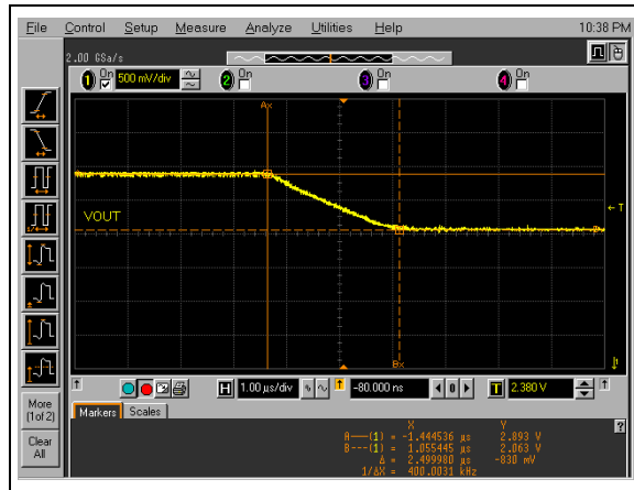
FIGURE 2-92: Half-Scale Settling Time (50h to 30h), V_{DD} = 5.0\text{V} , V_{REF} = 5.0\text{V} , R_L = 5\text{k}\Omega , C_L = 1\text{nF} .
