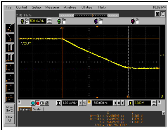
FIGURE 2-90: Full-Scale to Zero-Scale Settling Time (60h to 20h), V_{DD} = 5.0\text{V} , V_{REF} = 5.0\text{V} , R_L = 5\text{k}\Omega , C_L = 1\text{nF} .
