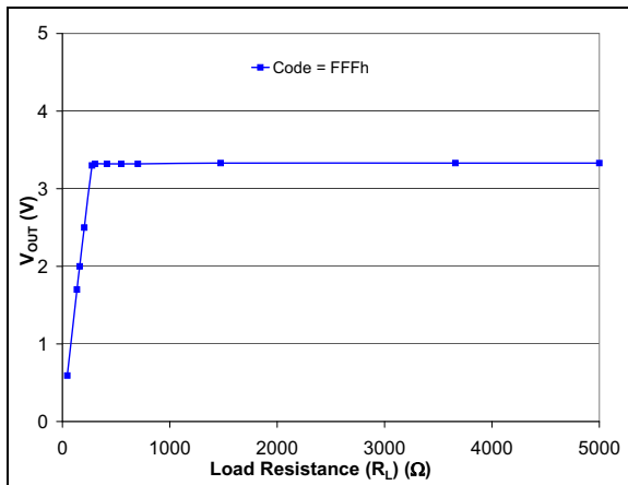
FIGURE 2-84: V_{OUT} vs. Resistive Load. V_{DD} = 5.0\text{V} .
