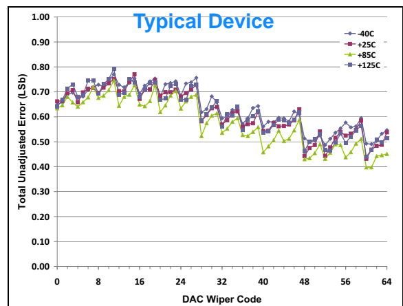
FIGURE 2-50: Total Unadjusted Error vs. Code and Temperature. V_{DD} = 3.6\text{V} , V_{REF} = 1.0\text{V} .
