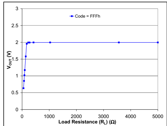
FIGURE 2-87: V_{OUT} vs. Resistive Load. V_{DD} = 3.0\text{V} .
