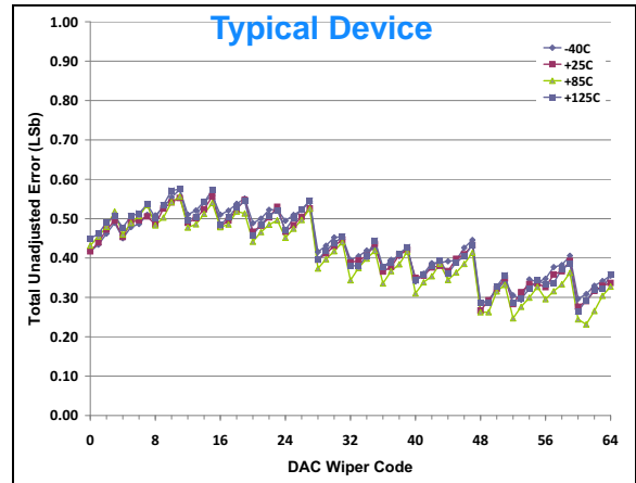
FIGURE 2-49: Total Unadjusted Error vs. Code and Temperature. V_{DD} = 3.6\text{V} , V_{REF} = 1.65\text{V} .
