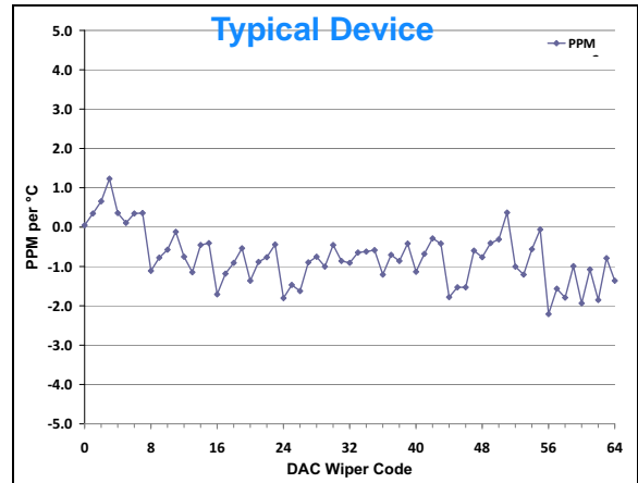
FIGURE 2-59: V_{OUT} Tempco vs. Code \left( \left( \frac{V_{OUT(+125C)} - V_{OUT(-40C)}}{V_{OUT(+25C, Code=FS)}} \right) / 165 \right) * 1,000,000 , V_{DD} = 3.6\text{V} , V_{REF} = 3.6\text{V} .
