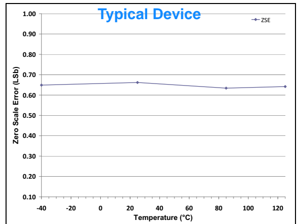
FIGURE 2-39: Zero Scale Error (ZSE) vs. Temperature. V_{DD} = 3.6\text{V} , V_{REF} = 1.0\text{V}
