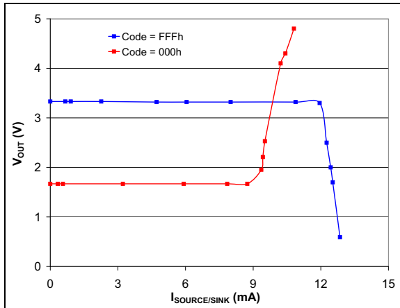
FIGURE 2-83: V_{OUT} vs. Source / Sink Current. V_{DD} = 5.0\text{V} .
