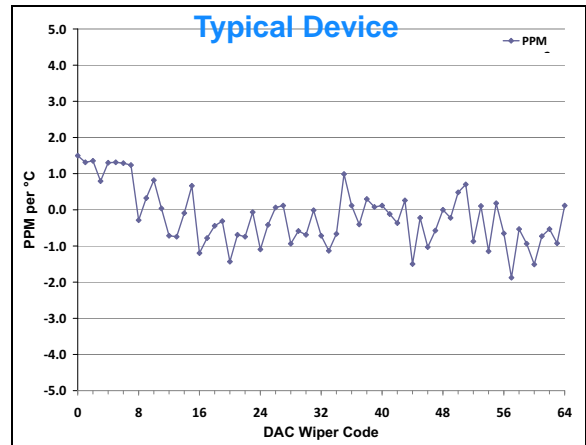
FIGURE 2-60: V_{OUT} Tempco vs. Code \left( \left( \frac{V_{OUT(+125C)} - V_{OUT(-40C)}}{V_{OUT(+25C, Code=FS)}} \right) / 165 \right) * 1,000,000 , V_{DD} = 3.6\text{V} , V_{REF} = 1.65\text{V} .
