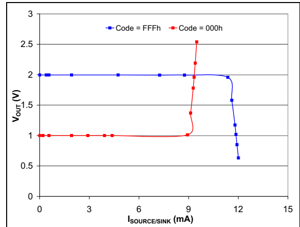
FIGURE 2-86: V_{OUT} vs. Source / Sink Current. V_{DD} = 3.0\text{V} .
