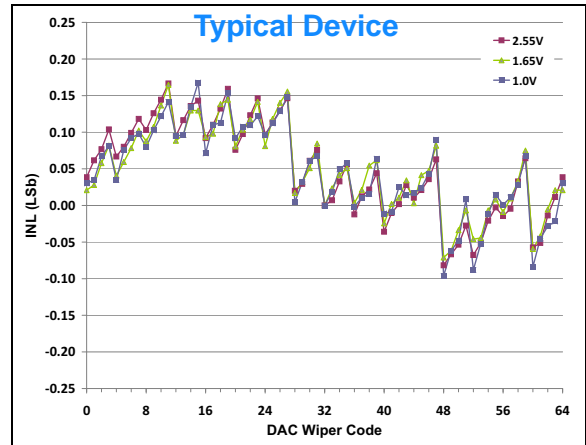
FIGURE 2-70: INL vs. Code and V_{REF} V_{DD} = 2.7\text{V} , V_{REF} = 1\text{V} , 1.65\text{V} , and 2.55\text{V} , \text{Temp} = +25^\circ\text{C} .
