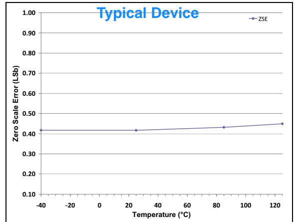
FIGURE 2-38: Zero Scale Error (ZSE) vs. Temperature. V_{DD} = 3.6\text{V} , V_{REF} = 1.65\text{V}
