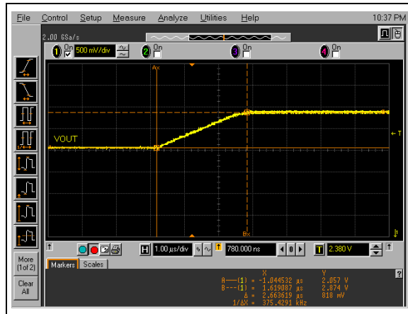
FIGURE 2-91: Half-Scale Settling Time (30h to 50h), V_{DD} = 5.0\text{V} , V_{REF} = 5.0\text{V} , R_L = 5\text{k}\Omega , C_L = 1\text{nF} .
