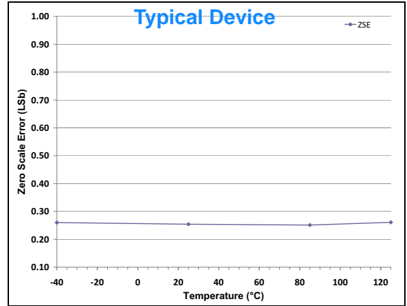
FIGURE 2-37: Zero Scale Error (ZSE) vs. Temperature. V_{DD} = 3.6\text{V} , V_{REF} = 3.6\text{V}
