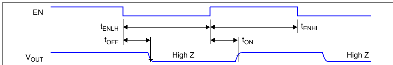
FIGURE 1-6: EN Timing Diagram.
