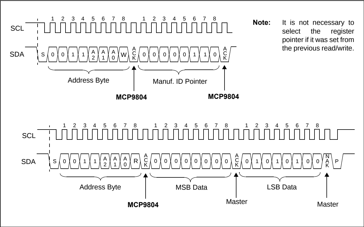
FIGURE 5-7: Timing Diagram for Reading the Manufacturer ID Register (See Section 4.0).
