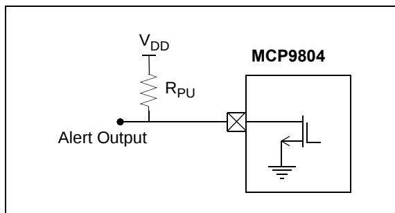
FIGURE 5-10: Active-Low Alert Output Configuration.
