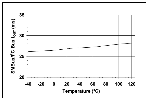
FIGURE 2-16: SMBus Timeout vs. Temperature.
