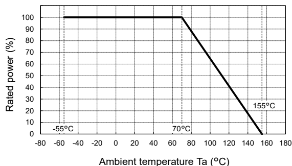
Fig.1< Ambient temperature>
