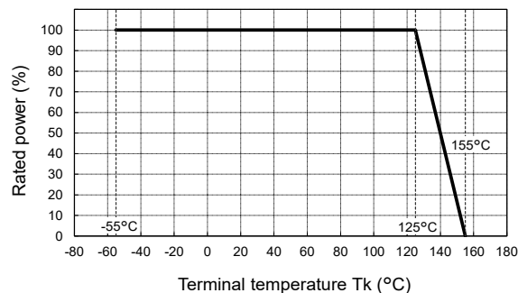
Fig.2< Terminal temperature>
