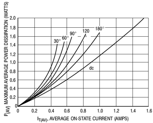
Figure 8. Power Dissipation
