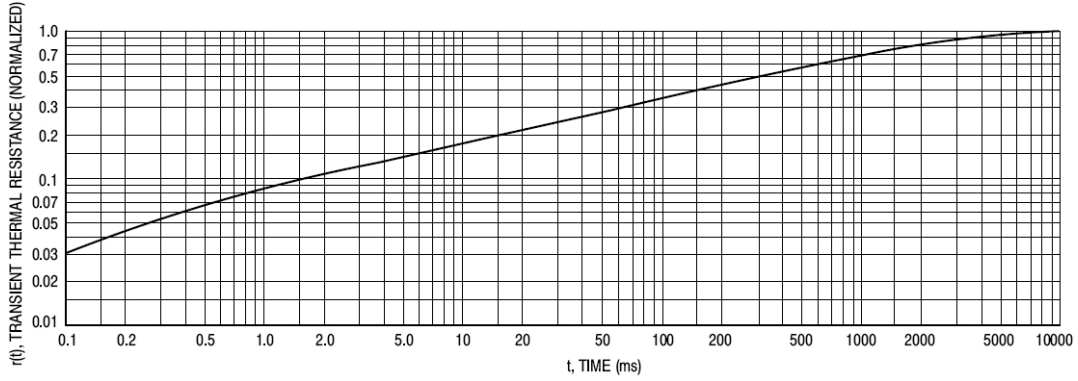
Figure 4. Thermal Response
