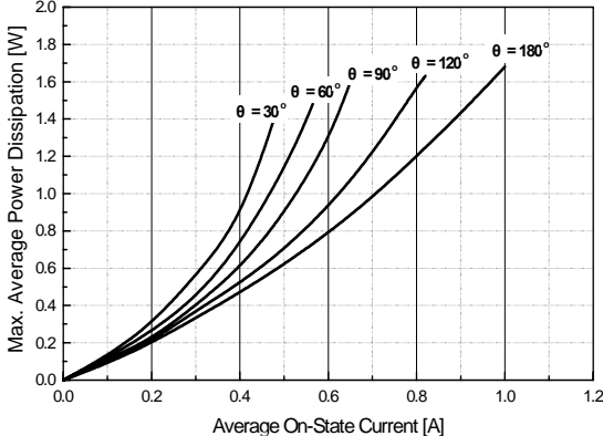
Fig 8. Power Dissipation
