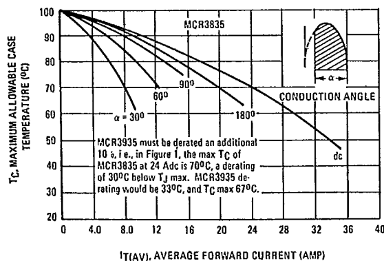
FIGURE 1 — CURRENT DERATING
