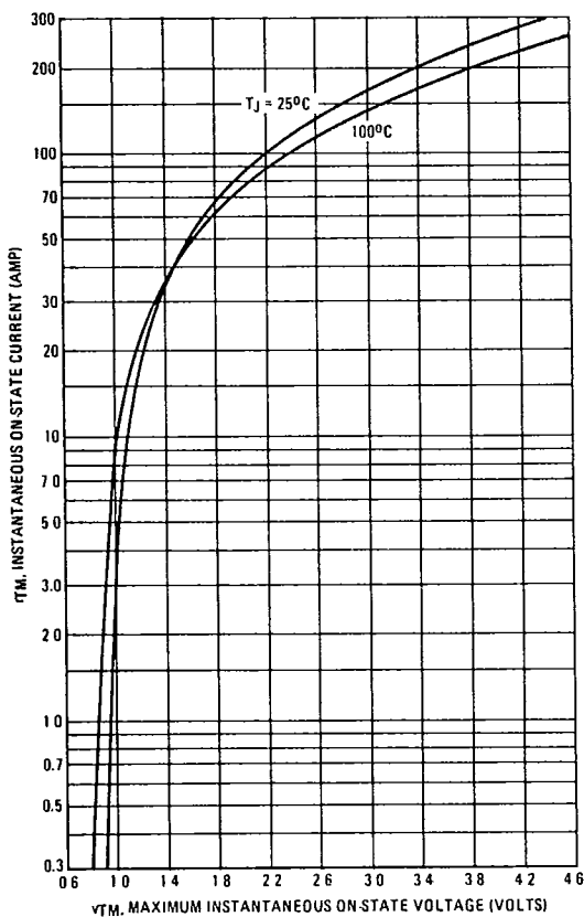
FIGURE 3 - ON-STATE CHARACTERISTICS
