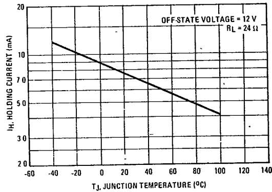
FIGURE 9 - HOLDING CURRENT
