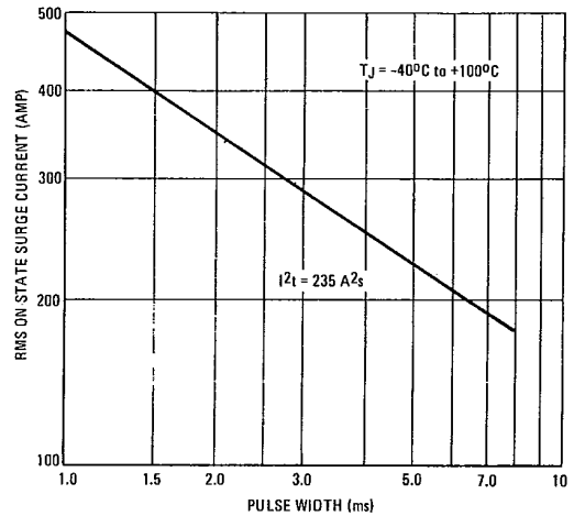
FIGURE 4 – SUB-CYCLE SURGES
