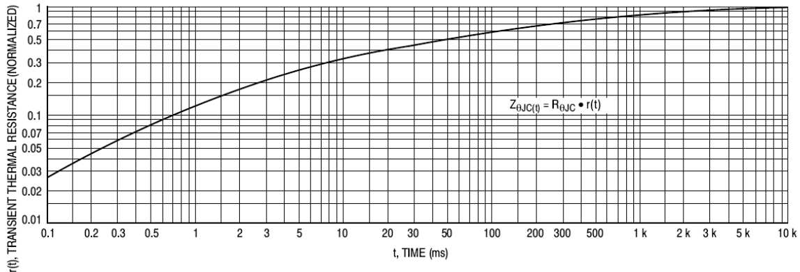
Figure 5. Thermal Response
