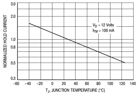
Figure 8. Holding Current
