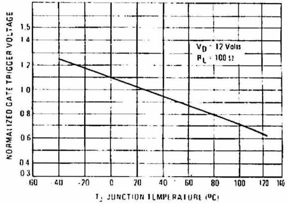
FIGURE 9 – GATE TRIGGER VOLTAGE
