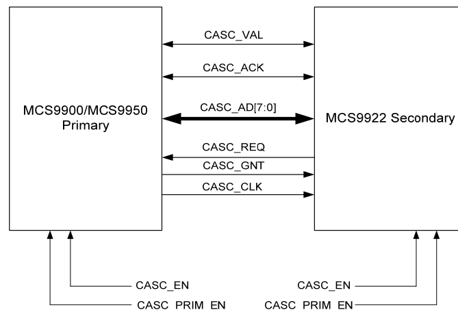
Cascade Interface between Primary and Secondary Devices
