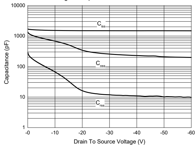
Fig. 9 - Capacitance Characteristics
