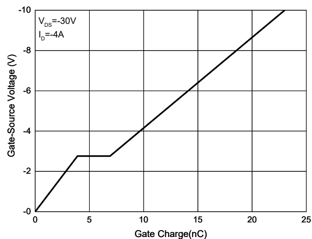
Fig. 8 - Gate Charge
