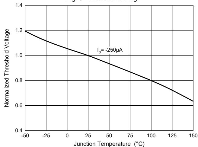
Fig. 6 - Threshold Voltage
