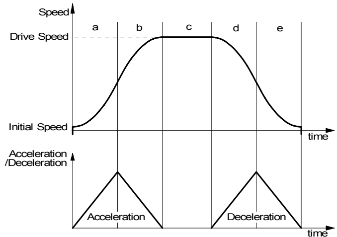
Fig. 2.13 Symmetrical S-Curve Acceleration/Deceleration Driving
