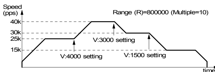
Fig. 2.5 Example of Drive Speed Change During Driving
