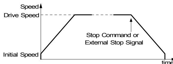
Fig. 2.7 Continuous Pulse Driving
