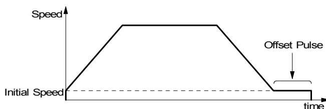
Fig. 2.6 Offset for Deceleration
