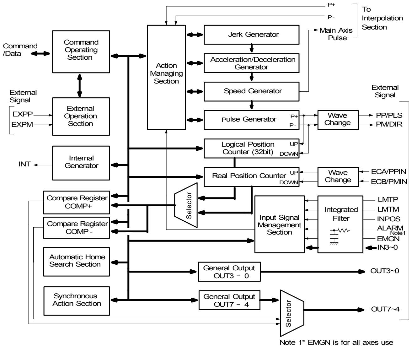
Fig.1.2 Block Diagram of the X,Y,Z and U -axis Control Section ( for One Axis Only)
