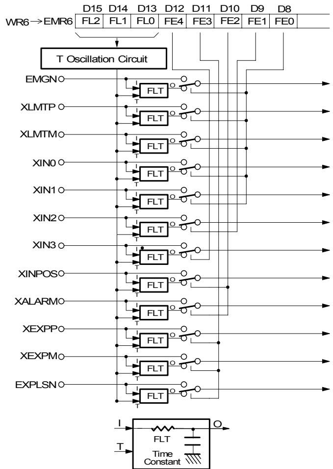
Fig. 2.43 Concept of Input Signal Filter Circuit
