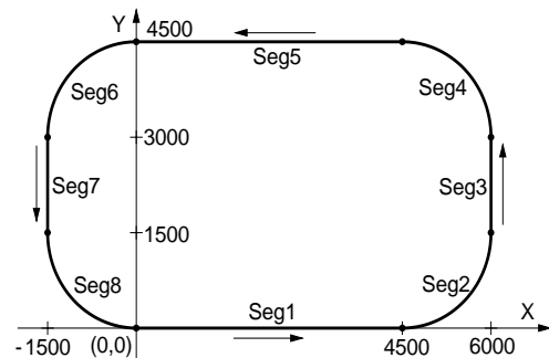
Fig. 2.37 The Example of Continuous Interpolation Axis
