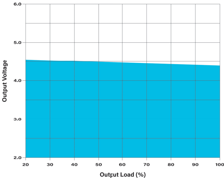
Output Load vs Output Voltage: MD124, Low Line
