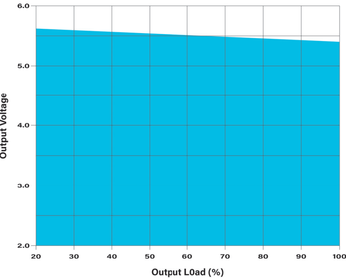
Output Load vs Output Voltage: MD112, Low Line
