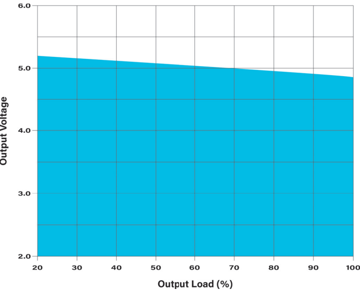
Output Load vs Output Voltage: MD112, High Line
