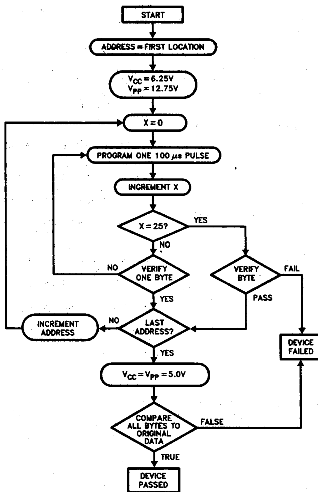
Figure 3. Quick-Pulse Programming Algorithm
