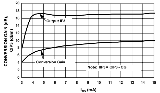
Conversion Gain & OIP 3 vs. DC Current
