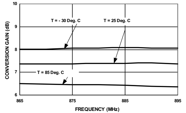
Conversion Gain vs. Temperature I_{DD} = 4.9 mA , R_{F IN} = -27 dBm
